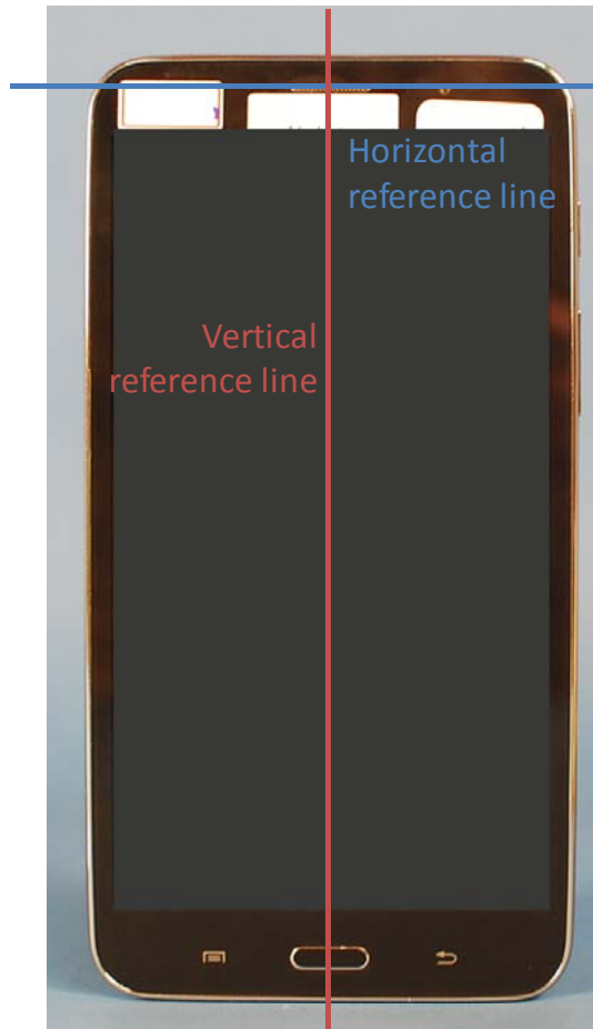
SAR Test Setup Photo 13- Horizontal and Vertical Reference Lines
