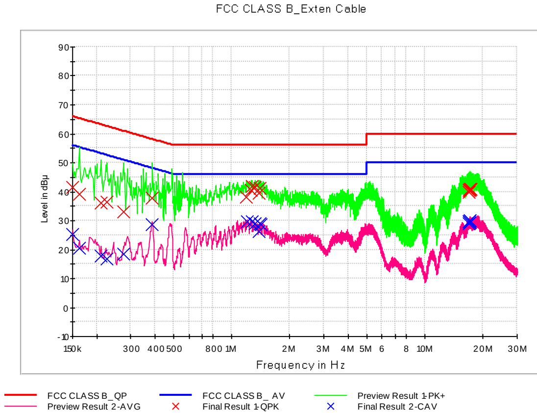
Figure 12: [EUT&amp;TA] MP4 Play Mode, Line (N)
