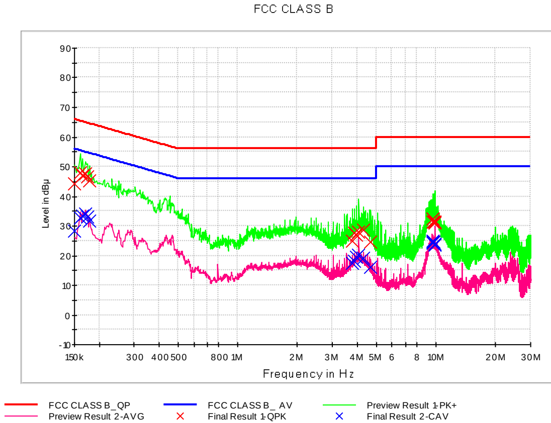
Figure 1: [EUT&amp;PC] DATA Communication Mode, Line (L1)
