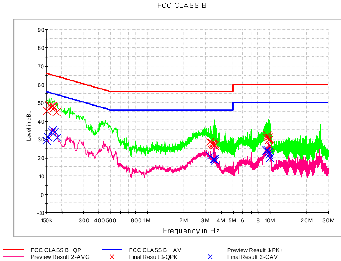
Figure 2: [EUT&amp;PC] DATA Communication Mode, Line (N)
