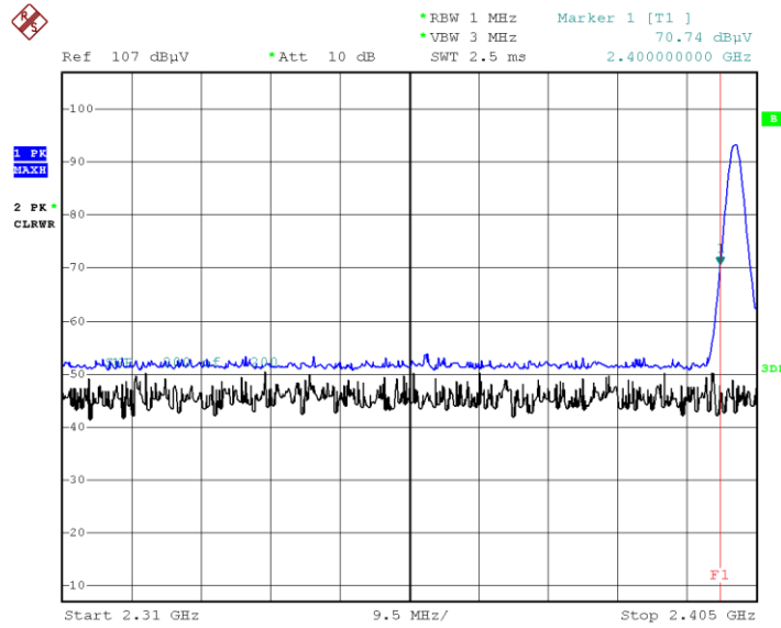
Radiated Band Edges plot – Average & Peak Reading (Ch.0)
