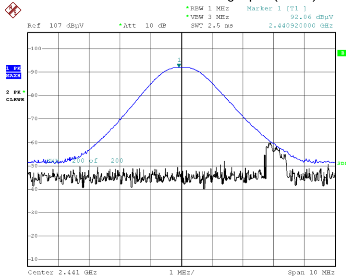
Fundamental Field Strength plot (Ch.39)
