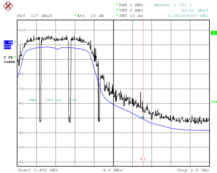
Radiated Restricted Band Edges plot – Average Reading (802.11g_6Mbps Ch.11)
