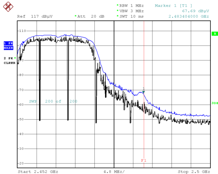
Radiated Restricted Band Edges plot – Peak Reading (802.11g_6Mbps Ch.11)
