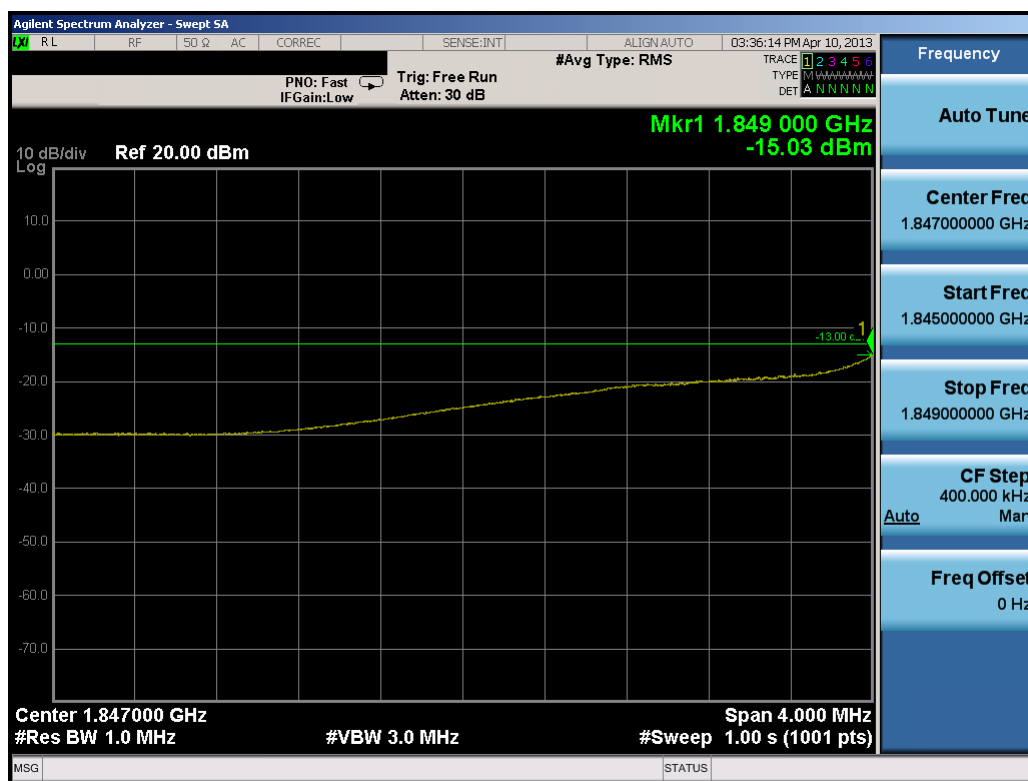
Plot 7-38. 4MHz Span Plot (PCS WCDMA Mode – Ch. 9262)
