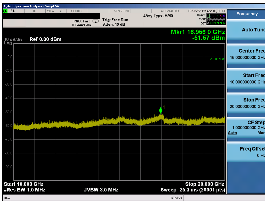
Plot 7-36. Conducted Spurious Plot (PCS WCDMA Mode – Ch. 9262)
