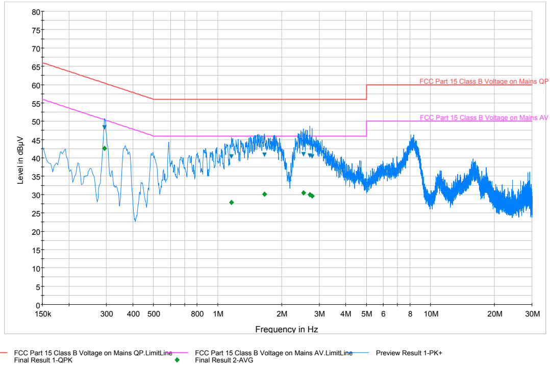
Plot 6-45. Line-Conducted Test Plot (N)
