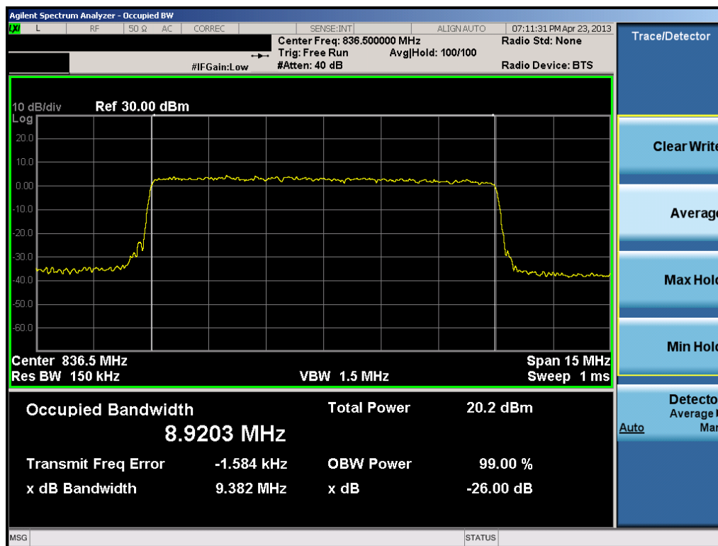
Plot 7-15. Occupied Bandwidth Plot (10.0MHz 16-QAM – RB Size 50)
