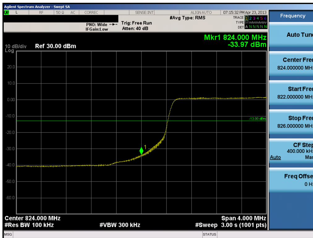
Plot 7-13. Lower Band Edge Plot (10.0MHz QPSK – RB Size 50)
