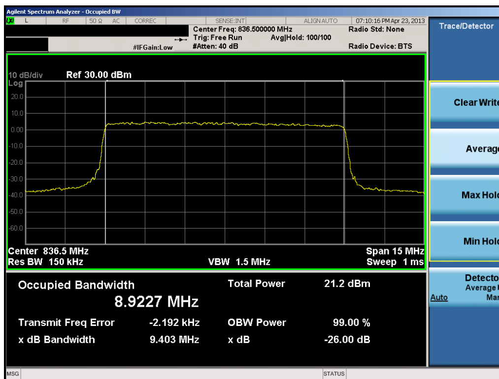
Plot 7-14. Occupied Bandwidth Plot (10.0MHz QPSK – RB Size 50)
