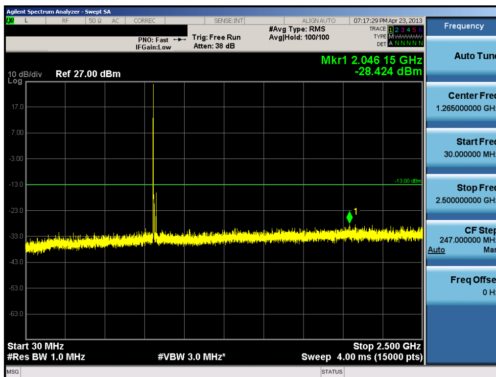
Plot 7-16. Conducted Spurious Plot (10.0MHz QPSK – RB Size 1, RB Offset 0 – Low Channel)
