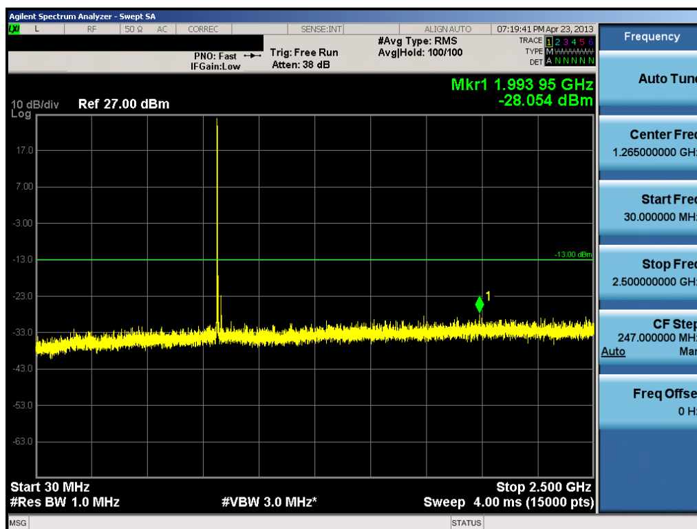
Plot 7-18. Conducted Spurious Plot (10.0MHz QPSK – RB Size 1, RB Offset 0 – Mid Channel)
