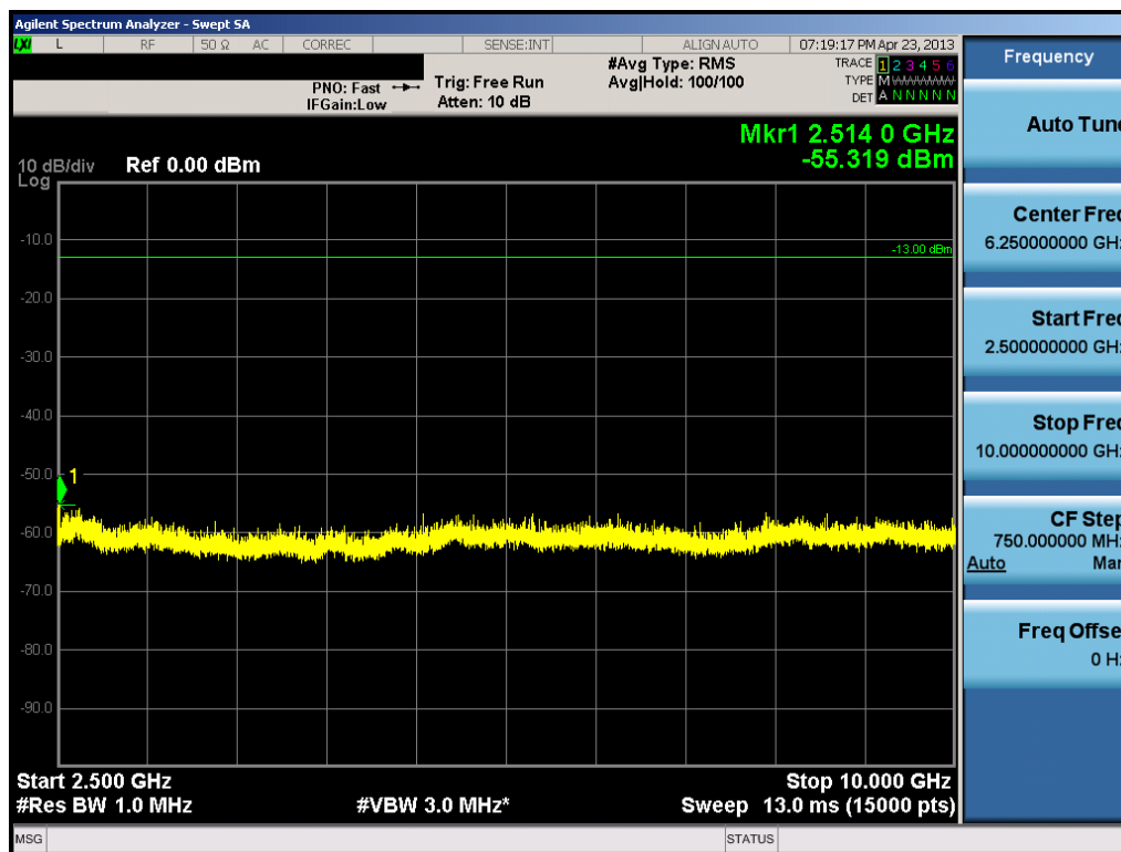
Plot 7-19. Conducted Spurious Plot (10.0MHz QPSK – RB Size 1, RB Offset 0 – Mid Channel)
