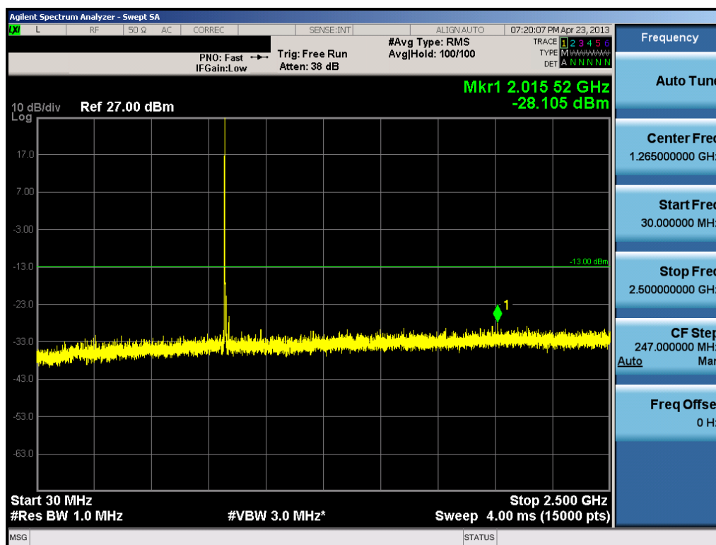
Plot 7-20. Conducted Spurious Plot (10.0MHz QPSK – RB Size 1, RB Offset 0 – High Channel)
