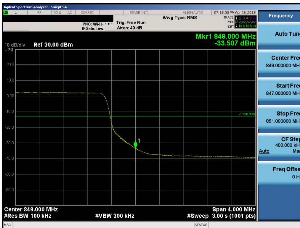
Plot 7-22. Upper Band Edge Plot (10.0MHz QPSK – RB Size 50)
