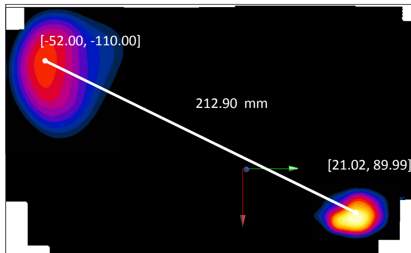
Figure 11-2 Peak SAR Locations of 2.4 GHz WLAN and UMTS 850
