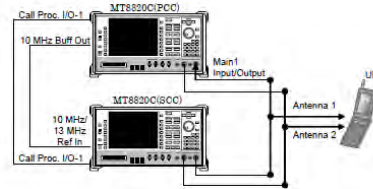
Figure 8-2 Power Measurement Setup
