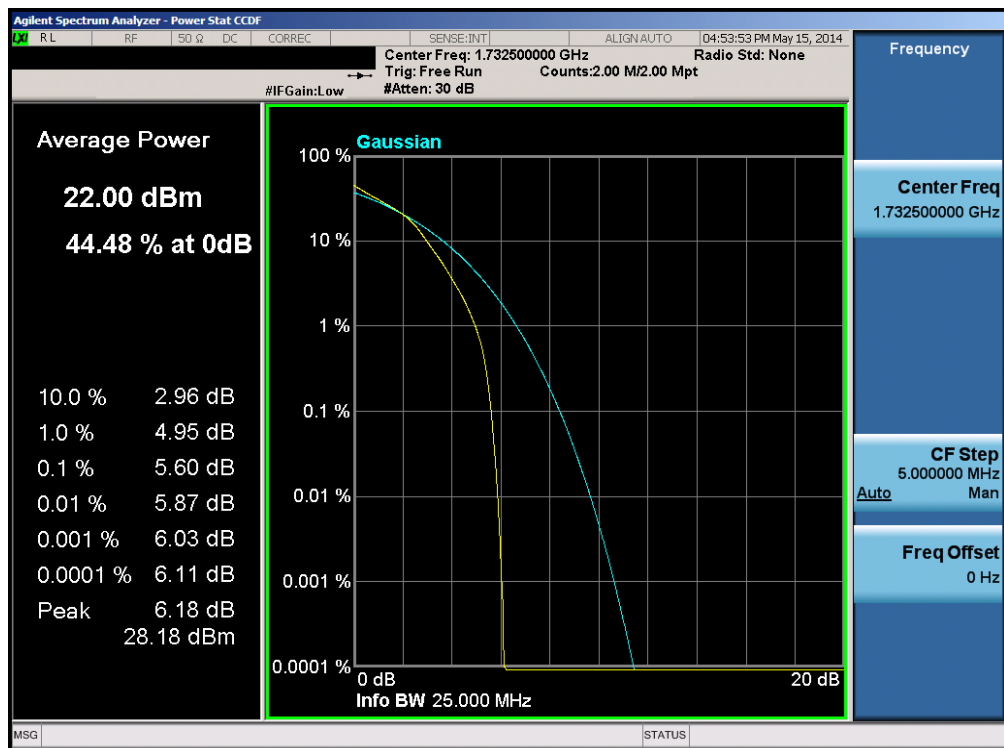
Plot 6-140. PAR Plot (Band 4 – 20.0MHz 16-QAM – RB Size 100)
