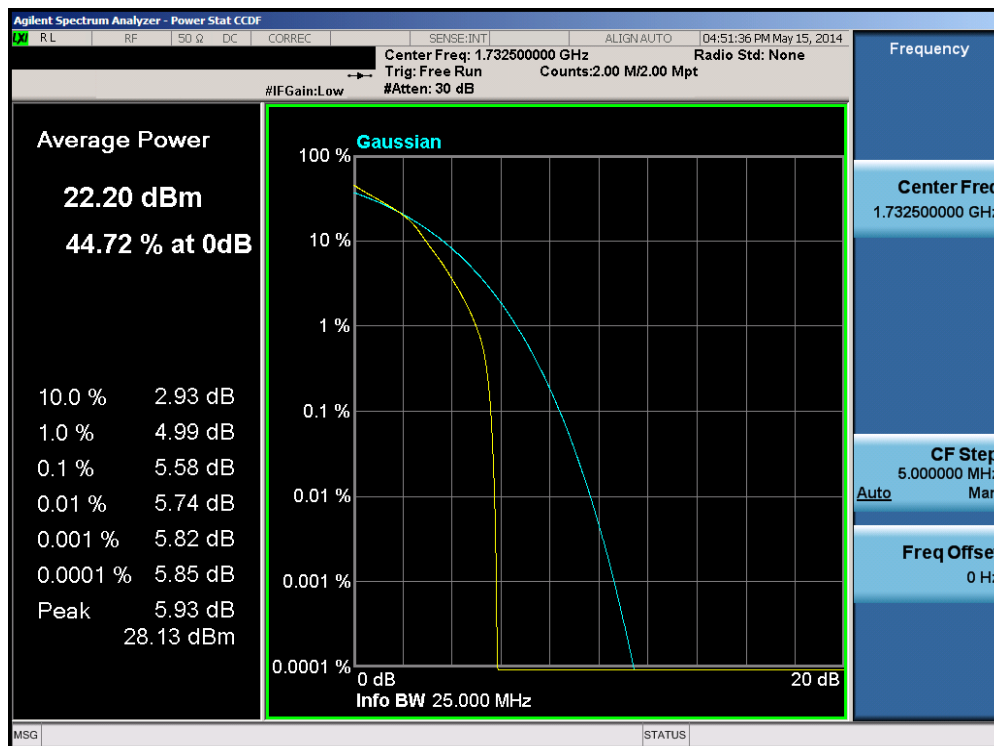
Plot 6-138. PAR Plot (Band 4 – 15.0MHz 16-QAM – RB Size 75)
