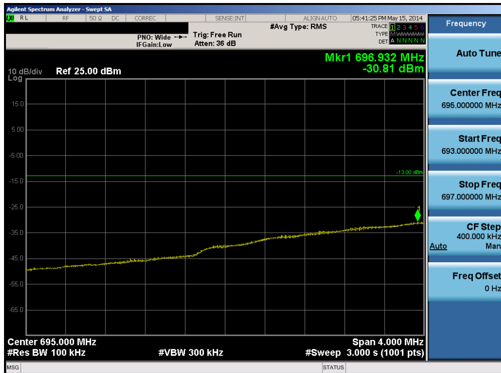
Plot 6-62. Lower Extended Band Edge Plot (Band 12 – 5.0MHz QPSK – RB Size 25)
