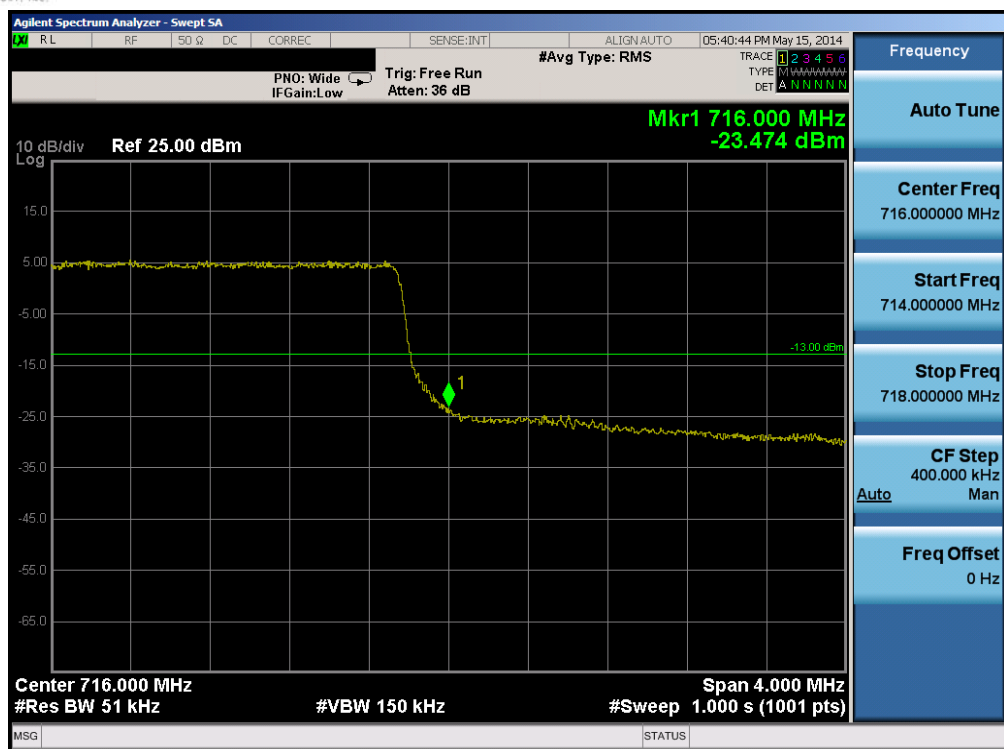
Plot 6-63. Upper Band Edge Plot (Band 12 – 5.0MHz QPSK – RB Size 25)
