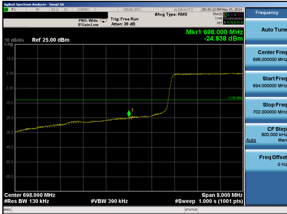
Plot 6-65. Lower Band Edge Plot (Band 12 – 10.0MHz QPSK – RB Size 50)
