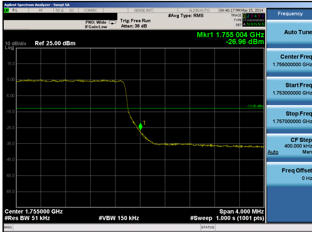
Plot 6-91. Upper Band Edge Plot (Band 4 – 5.0MHz QPSK – RB Size 25)
