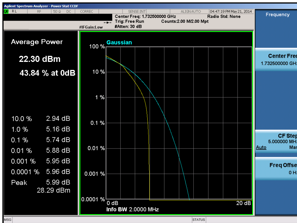
Plot 6-130. PAR Plot (Band 4 – 1.4MHz 16-QAM – RB Size 6)
