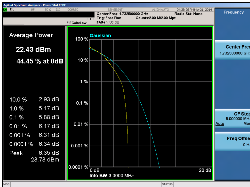
Plot 6-132. PAR Plot (Band 4 – 3.0MHz 16-QAM – RB Size 15)
