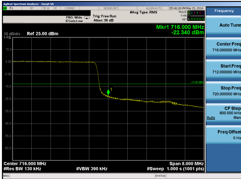
Plot 6-66. Upper Band Edge Plot (Band 12 – 10.0MHz QPSK – RB Size 50)
