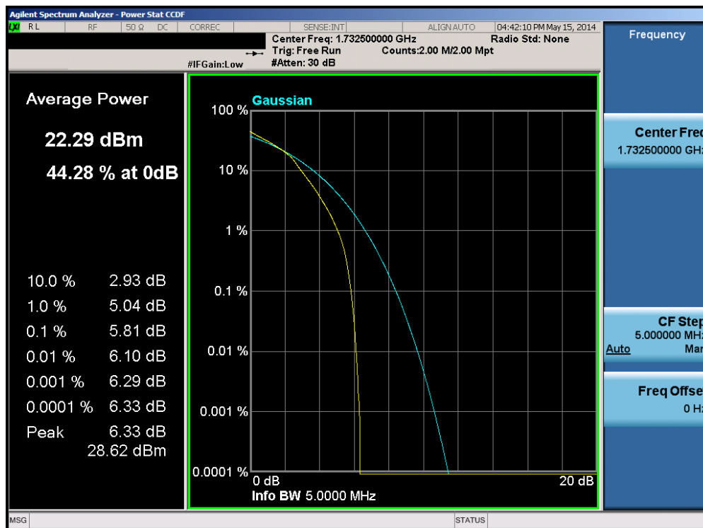
Plot 6-134. PAR Plot (Band 4 – 5.0MHz 16-QAM – RB Size 25)
