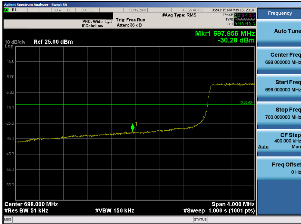
Plot 6-61. Lower Band Edge Plot (Band 12 – 5.0MHz QPSK – RB Size 25)
