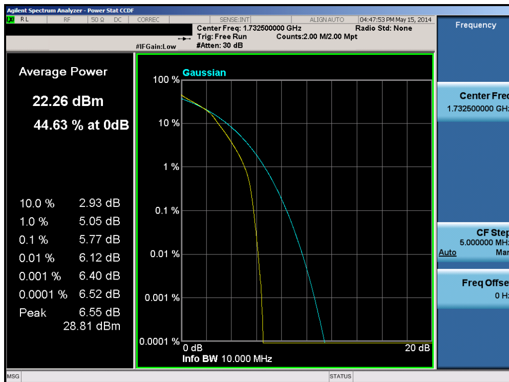
Plot 6-136. PAR Plot (Band 4 – 10.0MHz 16-QAM – RB Size 50)
