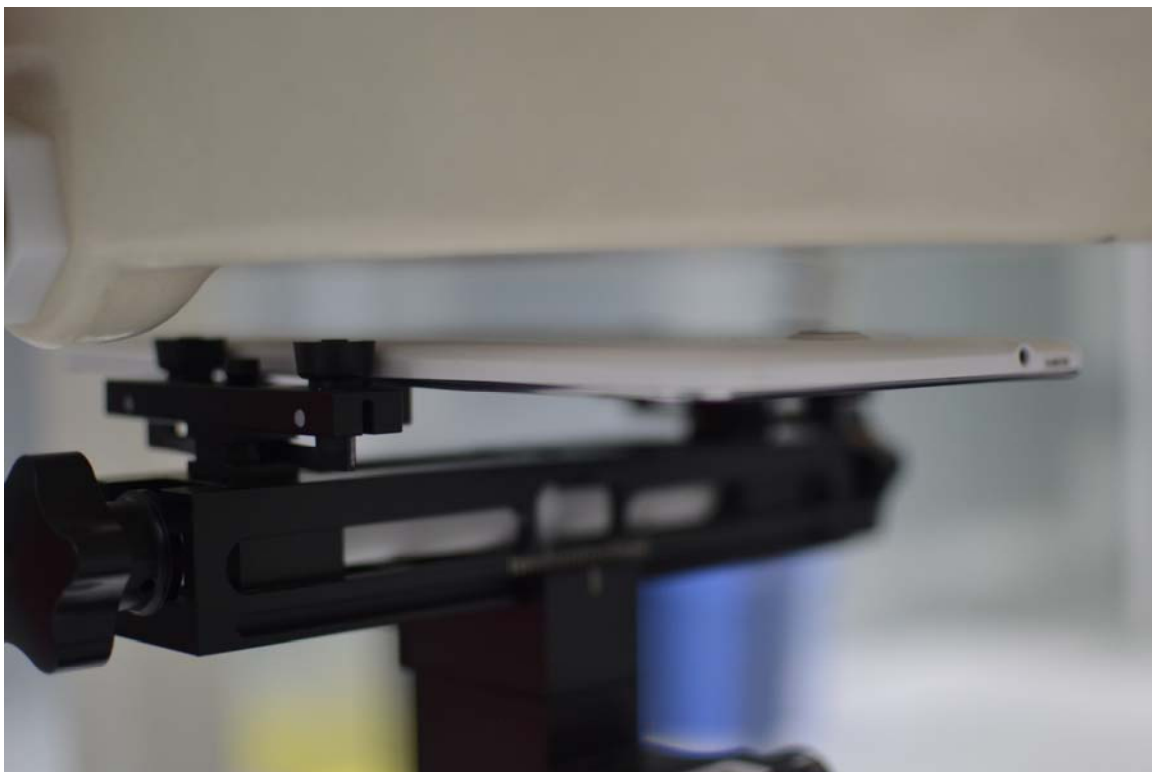
SAR Test Setup Photo 1 – Back Side at 17 mm
