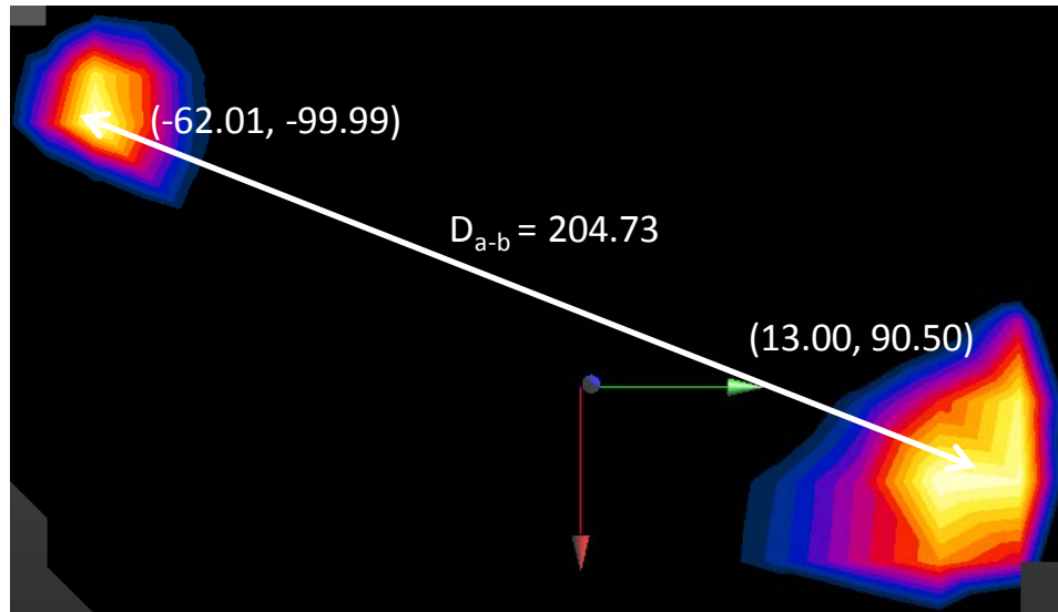
Figure 11-5 Peak SAR Location of 5 GHz WLAN and UMTS 1900 MHz
