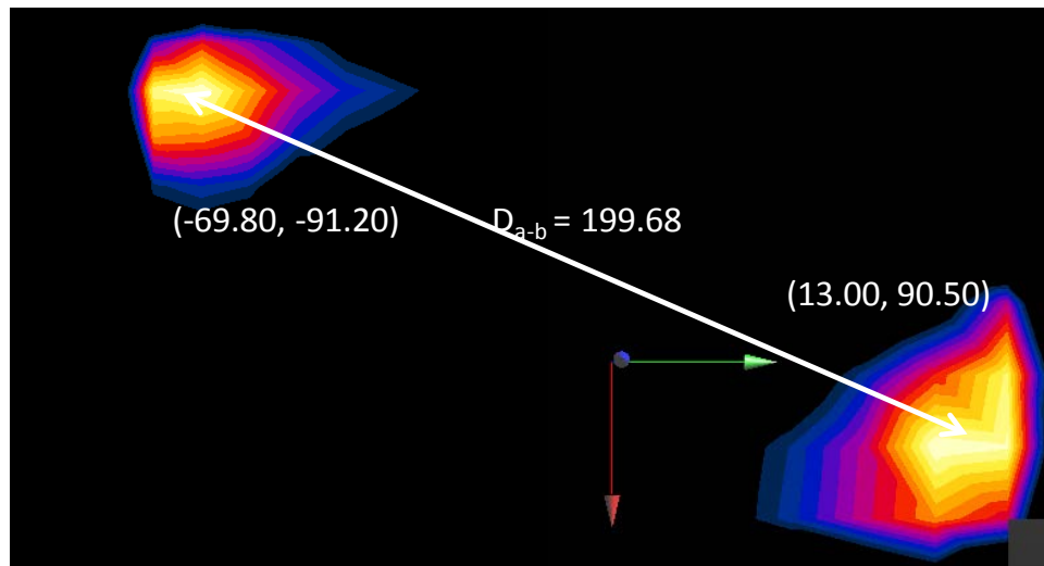
Figure 11-4 Peak SAR Location of 2.4 GHz WLAN and UMTS 1900 MHz
