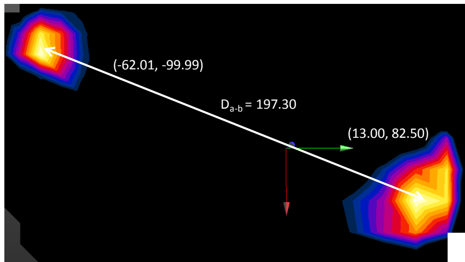
Figure 11-3 Peak SAR Location of 5 GHz WLAN and GPRS 1900
