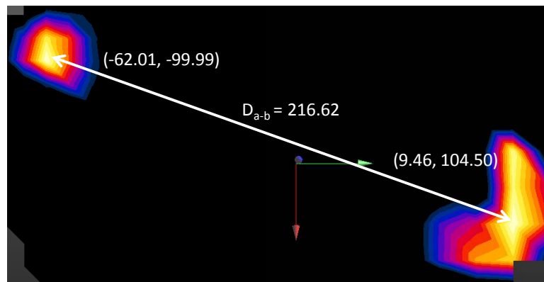
Figure 11-1 Peak SAR Location of 5 GHz WLAN and GPRS 850 MHz
