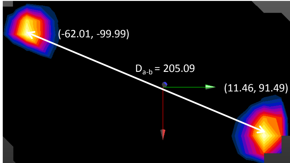
Figure 11-5 Peak SAR Location of 5 GHz WLAN and LTE B4
