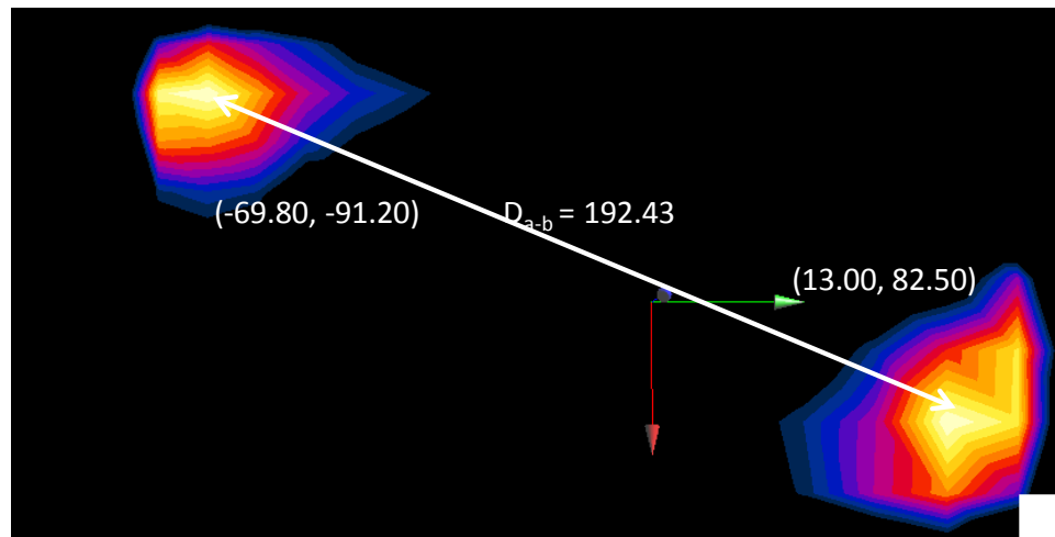
Figure 11-2 Peak SAR Location of 2.4 GHz WLAN and GPRS 1900 MHz
