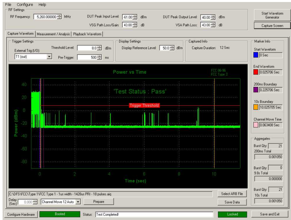
Figure 5-1. Band 2A Move Time and Aggregate Time
