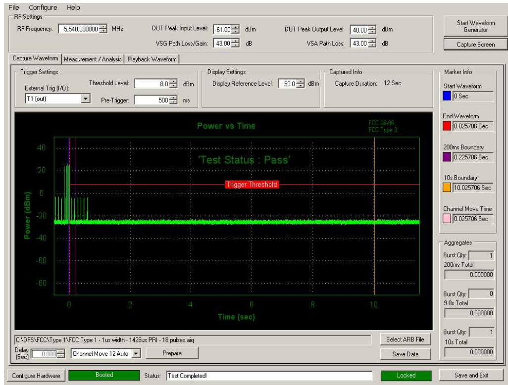
Figure 5-3. Band 2C Move Time and Aggregate Time
