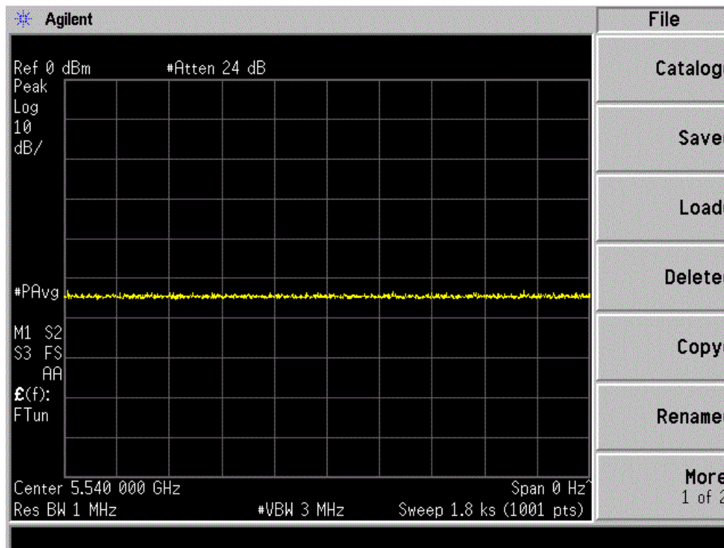
Figure 5-4 Non-occupancy Period - Monitoring live spectrum - Elapse time 30 minutes
