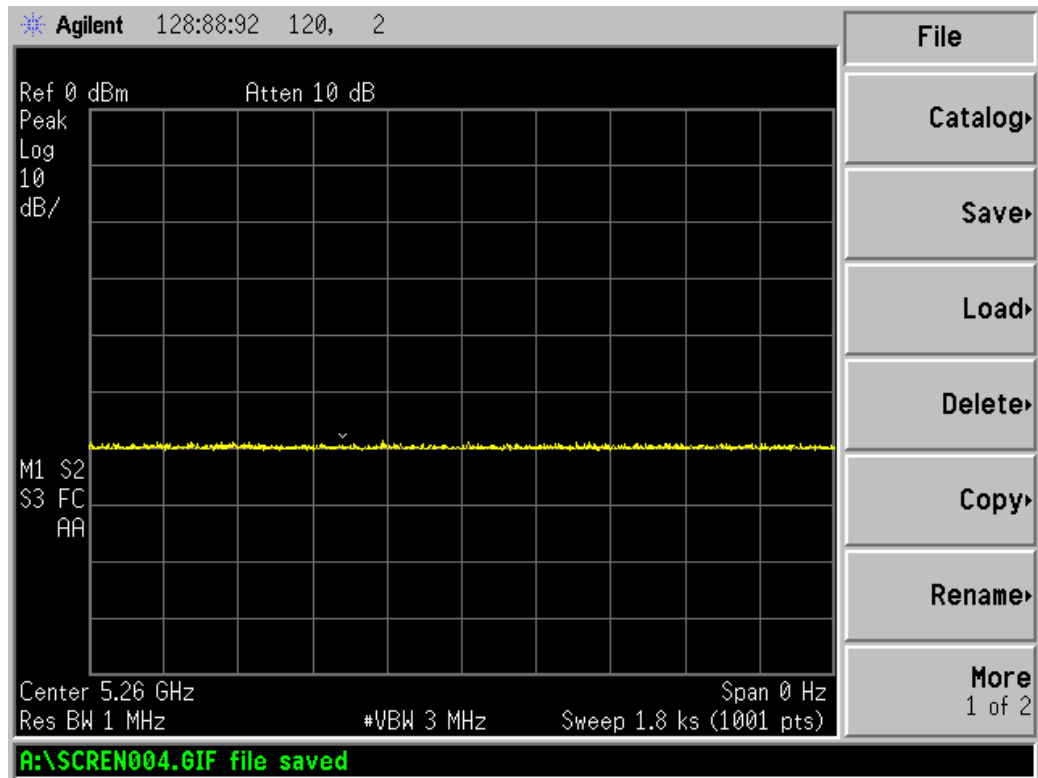
Figure 5-2 Band 2A Non-occupancy Period - Monitoring live spectrum - Elapse time 30 minutes
