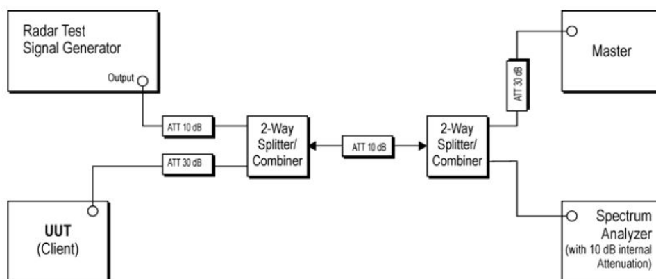
Figure 3-1. Conducted Test Setup for DFS
