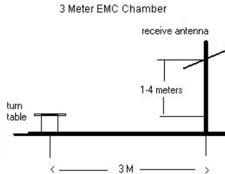
Figure 6-6. Test Instrument & Measurement Setup
