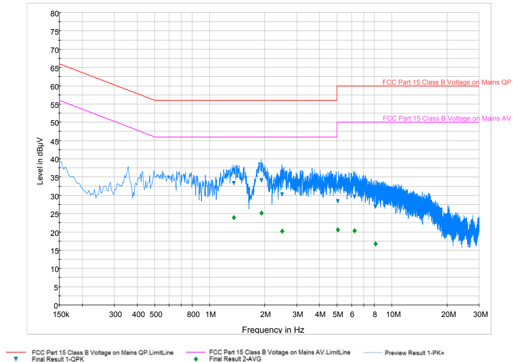
Plot 6-44. Line-Conducted Test Plot (L1)
