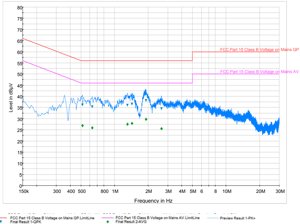
Plot 6-45. Line-Conducted Test Plot (N)
