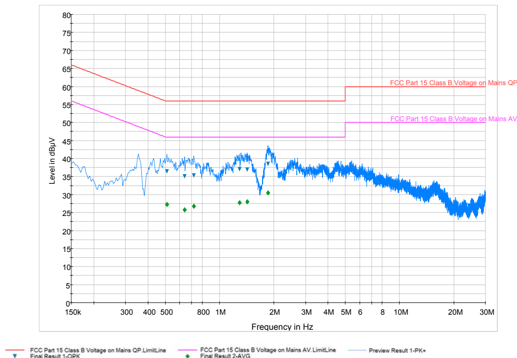
Plot 6-6. Line Conducted Plot with ANT+ (N)
