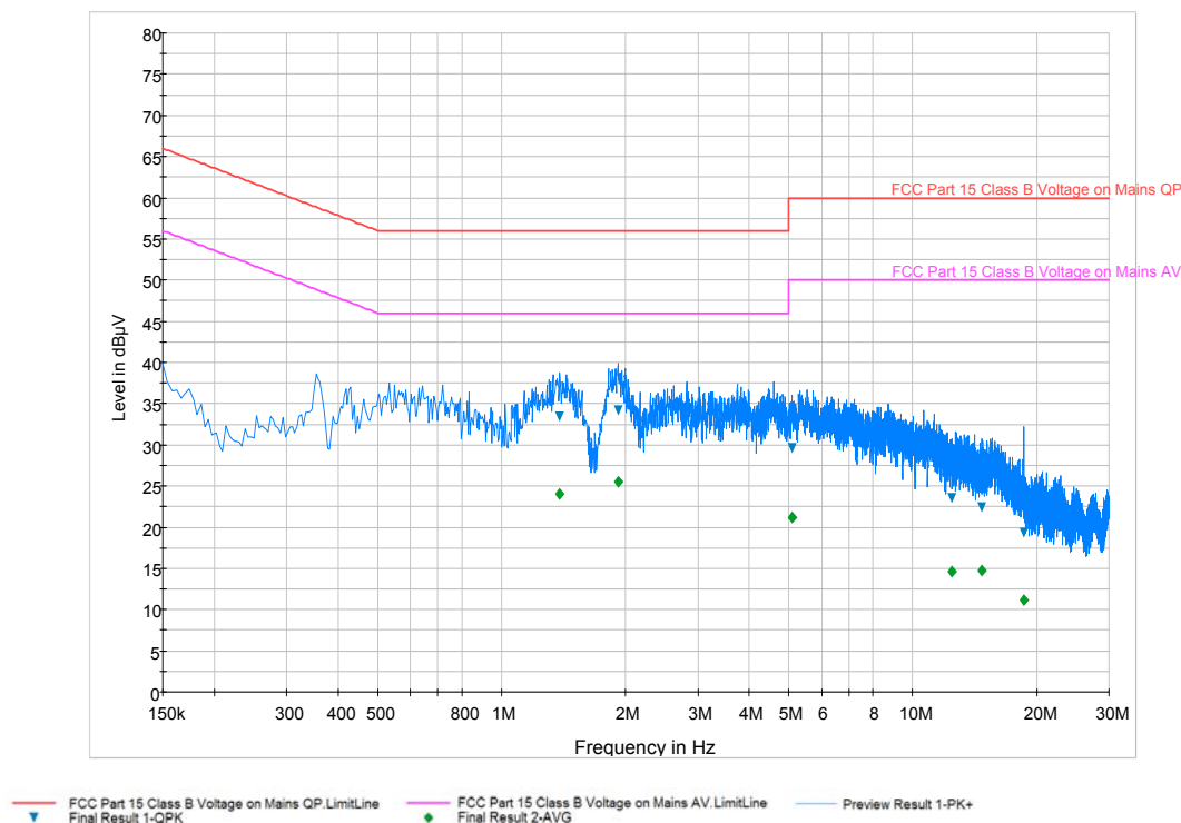
Plot 6-5. Line Conducted Plot with ANT+ (L1)
