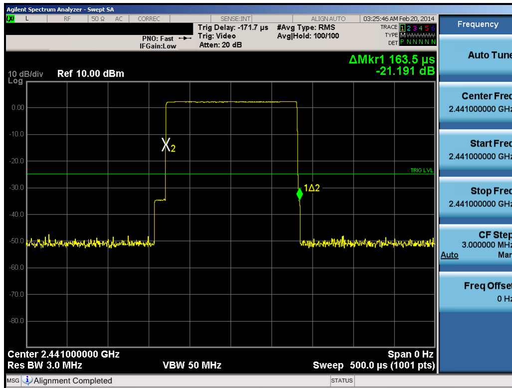
Plot 6-1. Pulse Width
