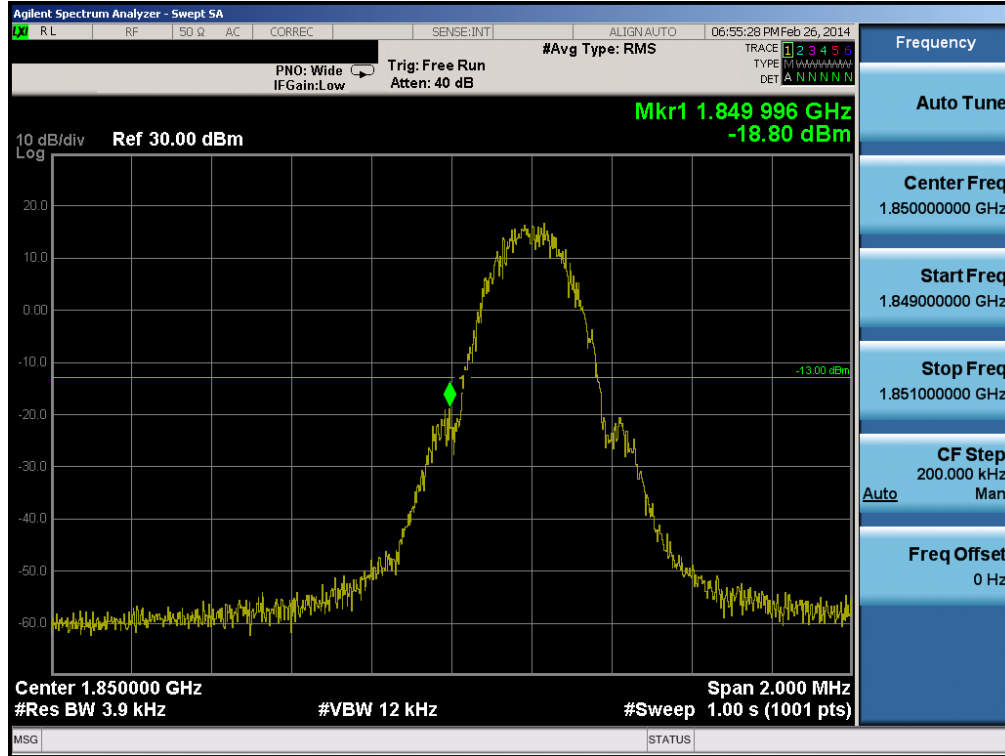
Plot 6-36. Band Edge Plot (PCS GPRS Mode – Ch. 512)
