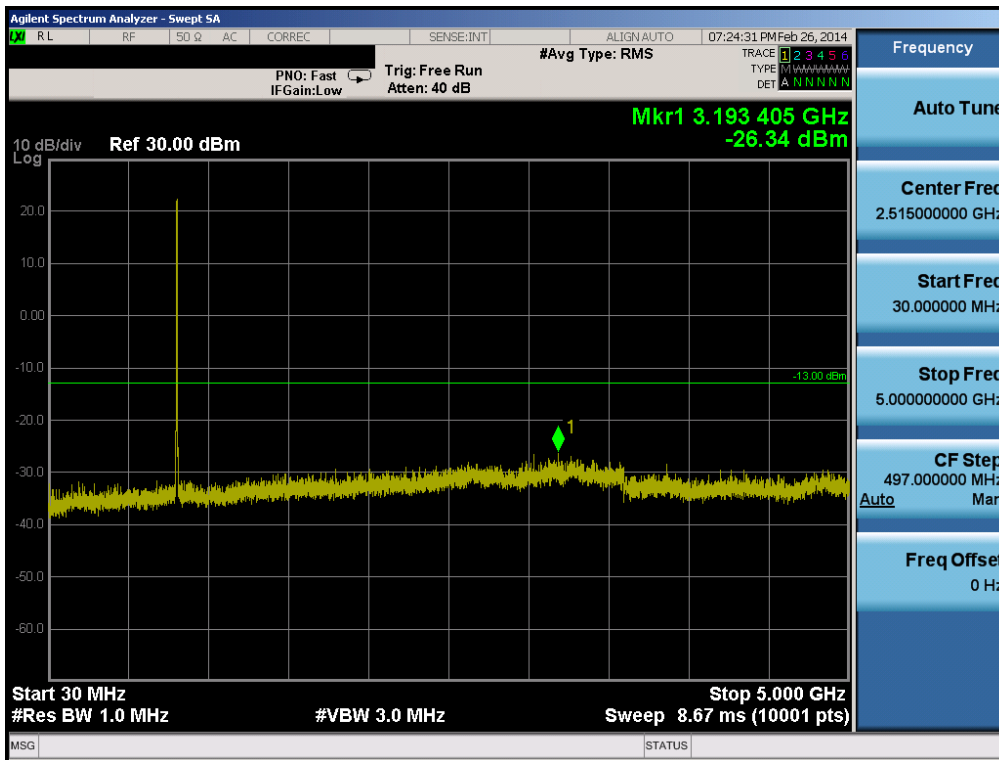
Plot 6-22. Conducted Spurious Plot (Cellular WCDMA Mode – Ch. 4132)
