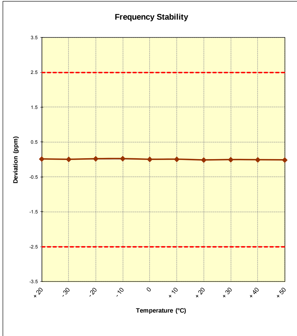
Figure 6-7. Frequency Stability Graph (Cellular GPRS Mode – Ch. 190)
