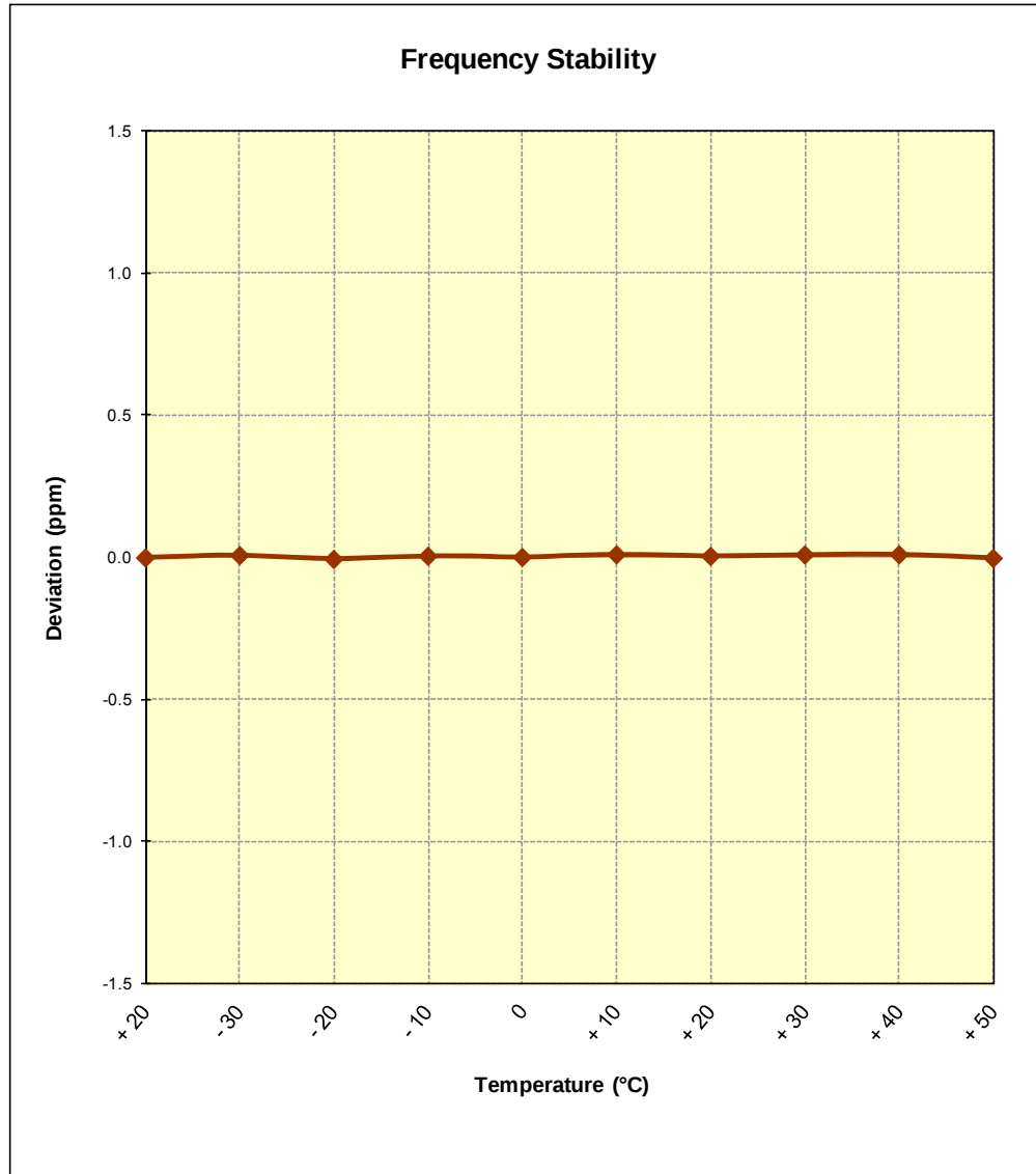
Figure 6-9. Frequency Stability Graph (PCS GPRS Mode – Ch. 661)
