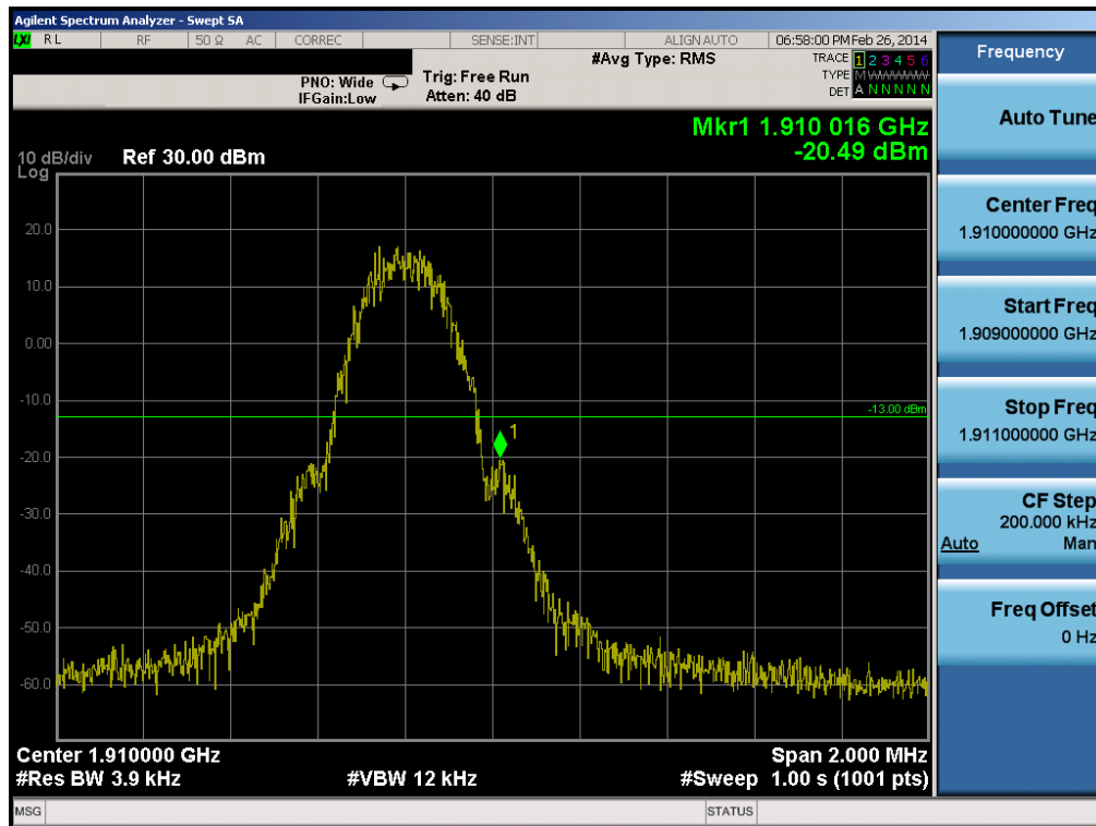
Plot 6-37. Band Edge Plot (PCS GPRS Mode – Ch. 810)
