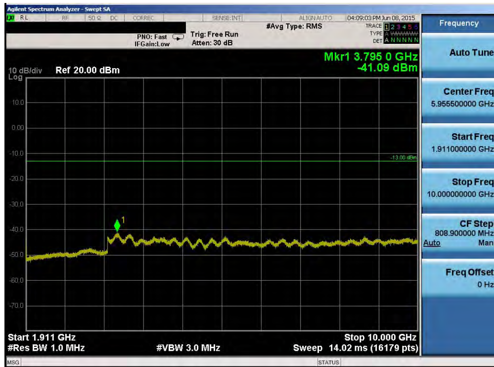
Plot 6-54. Conducted Spurious Plot (Band 2 – 15.0MHz QPSK – RB Size 1, RB Offset 0 – High Channel)
