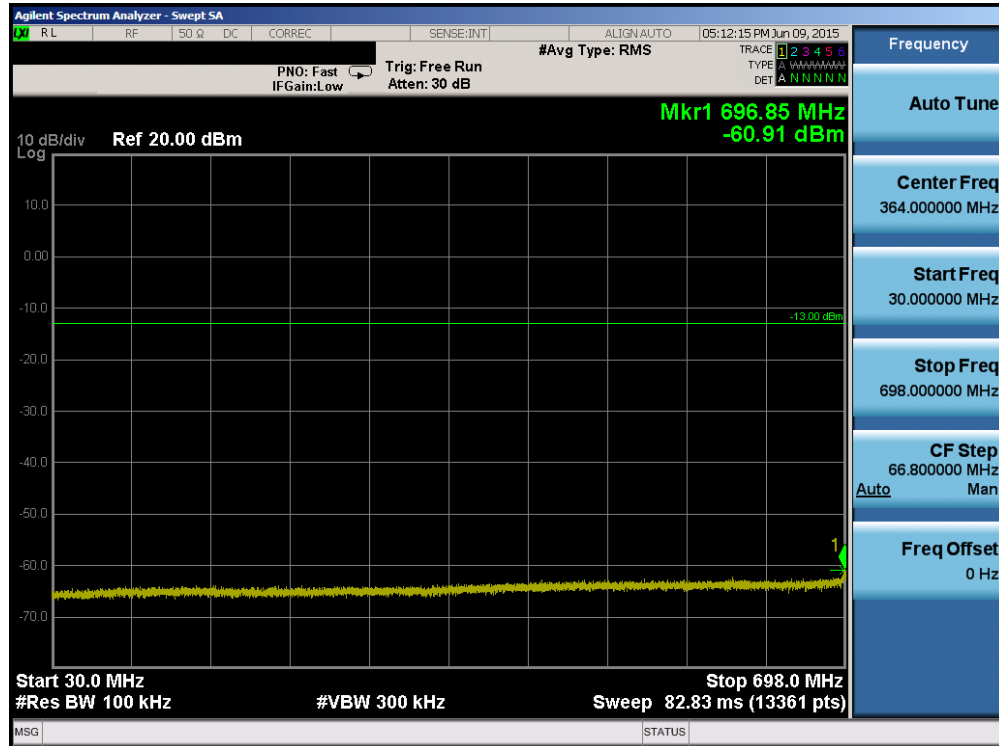
Plot 6-35. Conducted Spurious Plot (Band 12 – 5.0MHz QPSK – RB Size 1, RB Offset 0 – High Channel)
