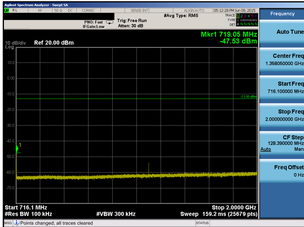
Plot 6-36. Conducted Spurious Plot (Band 12 – 5.0MHz QPSK – RB Size 1, RB Offset 0 – High Channel)
