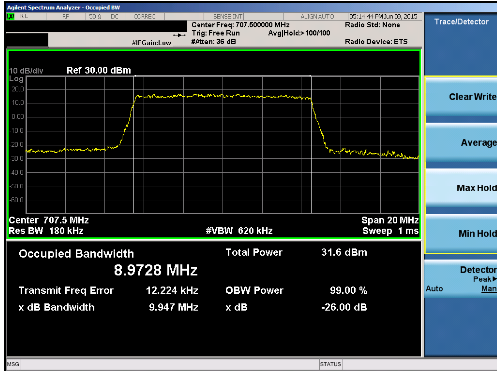
Plot 6-3. Occupied Bandwidth Plot (Band 12 – 10.0MHz QPSK – RB Size 50)
