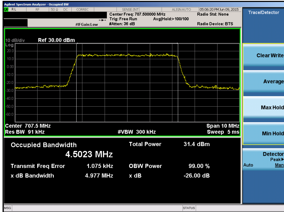
Plot 6-1. Occupied Bandwidth Plot (Band 12 – 5.0MHz QPSK – RB Size 25)
