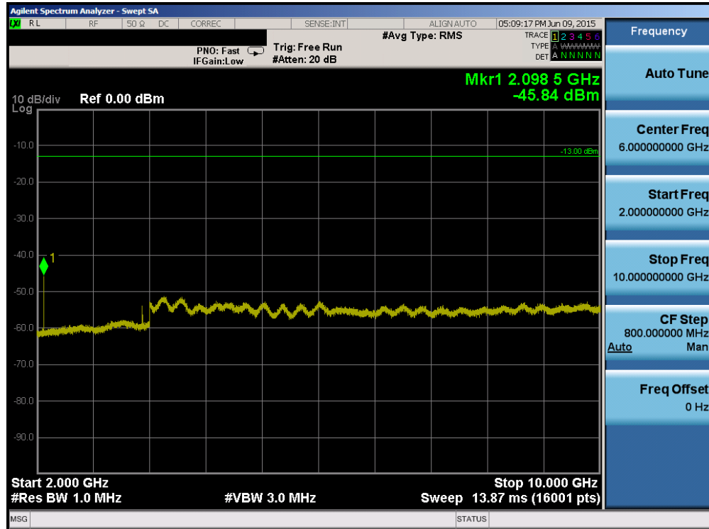
Plot 6-31. Conducted Spurious Plot (Band 12 – 5.0MHz QPSK – RB Size 1, RB Offset 0 – Low Channel)
