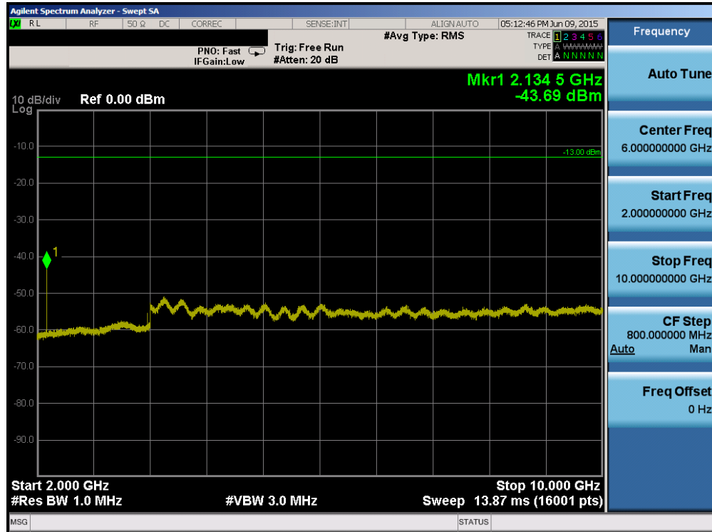
Plot 6-37. Conducted Spurious Plot (Band 12 – 5.0MHz QPSK – RB Size 1, RB Offset 0 – High Channel)
