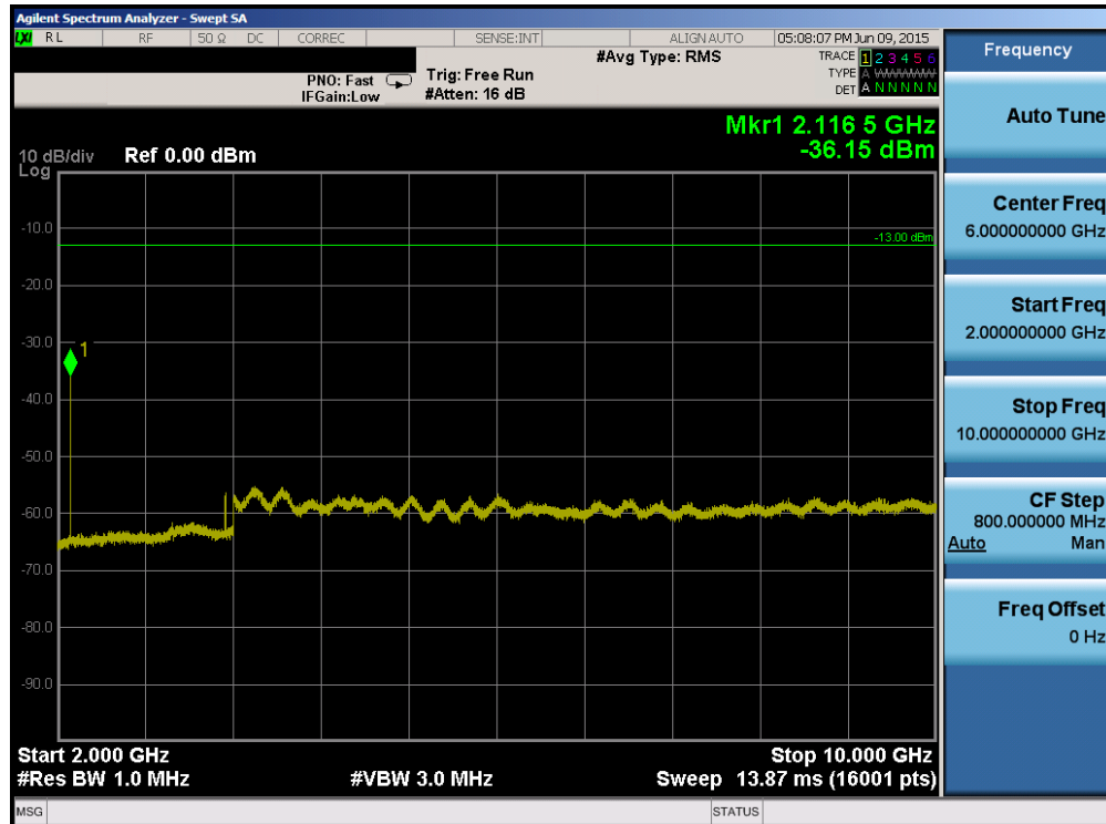
Plot 6-34. Conducted Spurious Plot (Band 12 – 5.0MHz QPSK – RB Size 1, RB Offset 0 – Mid Channel)
