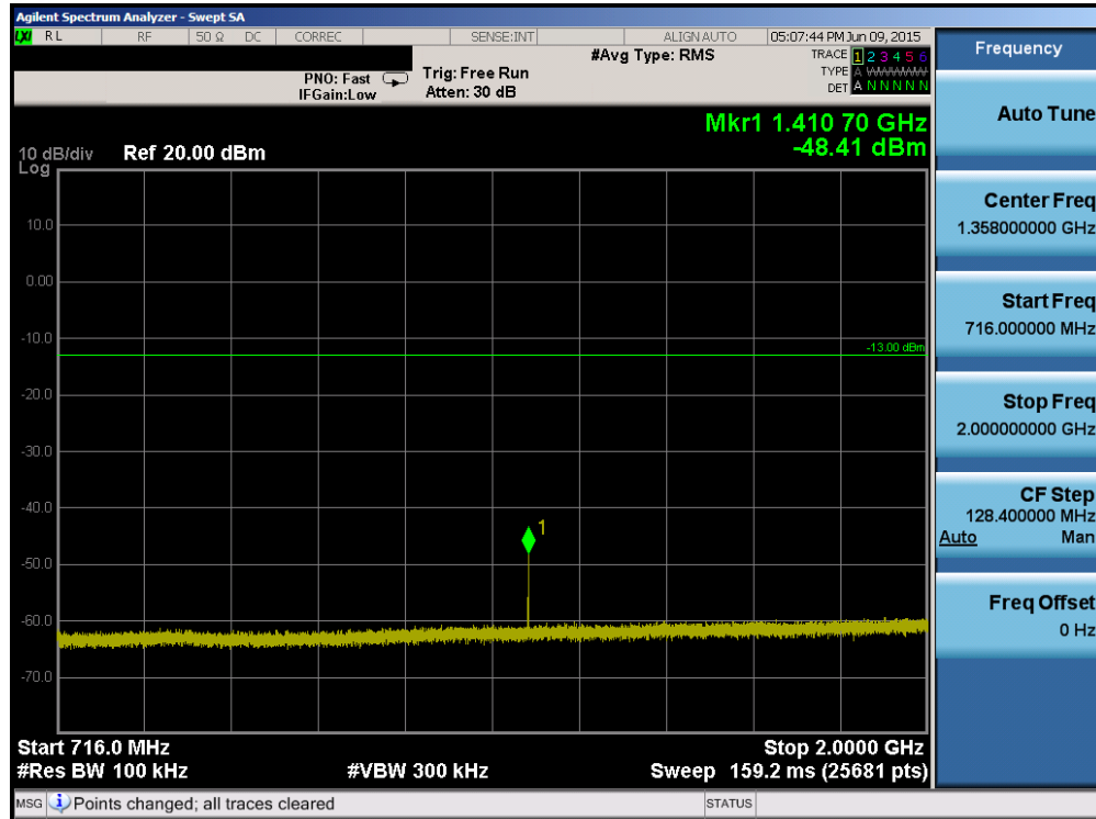
Plot 6-33. Conducted Spurious Plot (Band 12 – 5.0MHz QPSK – RB Size 1, RB Offset 0 – Mid Channel)
