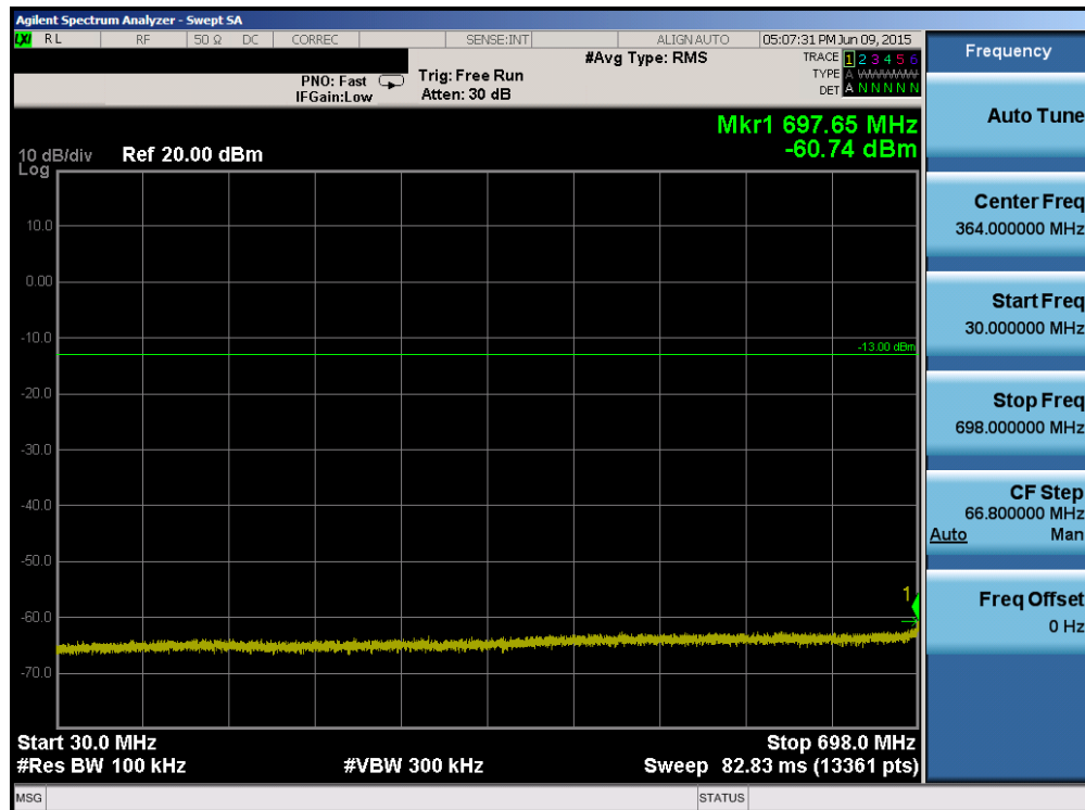
Plot 6-32. Conducted Spurious Plot (Band 12 – 5.0MHz QPSK – RB Size 1, RB Offset 0 – Mid Channel)
