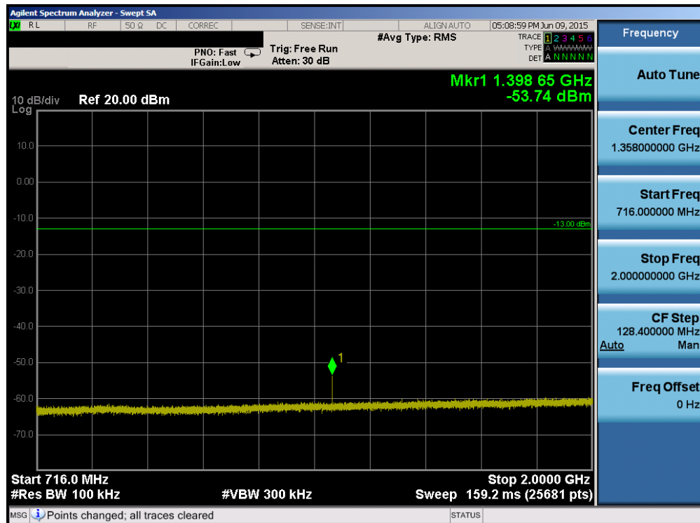
Plot 6-30. Conducted Spurious Plot (Band 12 – 5.0MHz QPSK – RB Size 1, RB Offset 0 – Low Channel)
