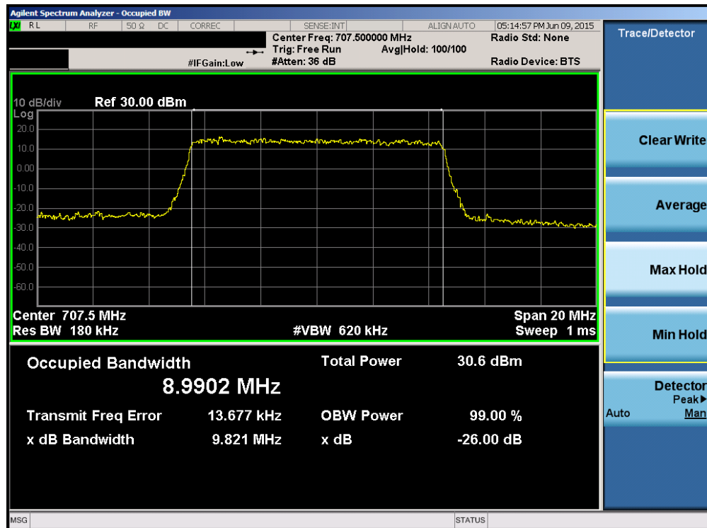
Plot 6-4. Occupied Bandwidth Plot (Band 12 – 10.0MHz 16-QAM – RB Size 50)
