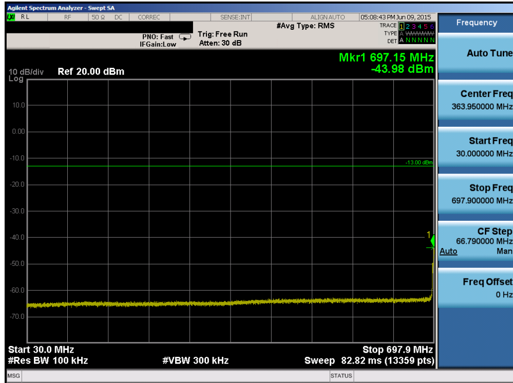
Plot 6-29. Conducted Spurious Plot (Band 12 – 5.0MHz QPSK – RB Size 1, RB Offset 0 – Low Channel)
