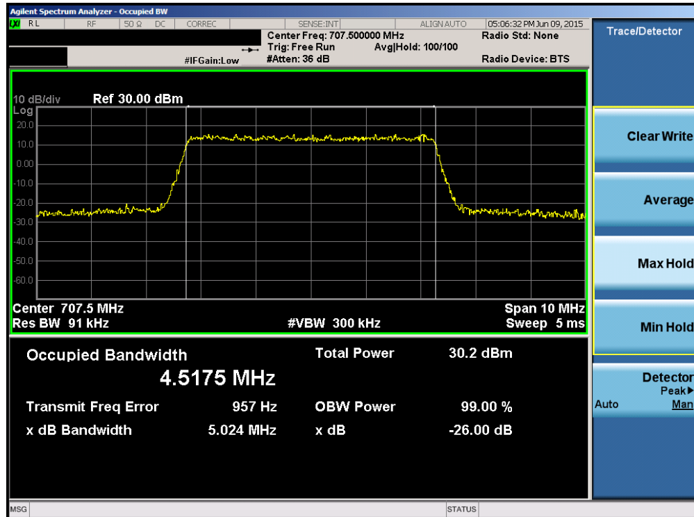
Plot 6-2. Occupied Bandwidth Plot (Band 12 – 5.0MHz 16-QAM – RB Size 25)
