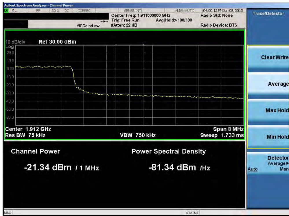
Plot 6-101. Upper Extended Band Edge Plot (Band 2 – 10.0MHz QPSK – RB Size 50)
