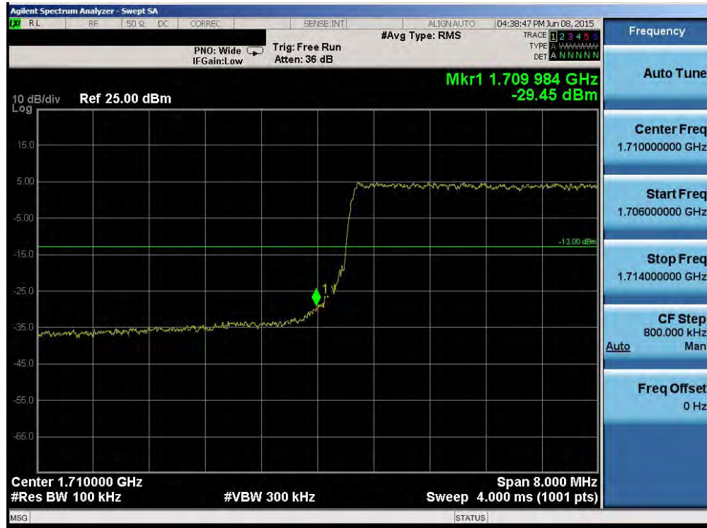
Plot 6-74. Lower Band Edge Plot (Band 4 – 10.0MHz QPSK – RB Size 50)
