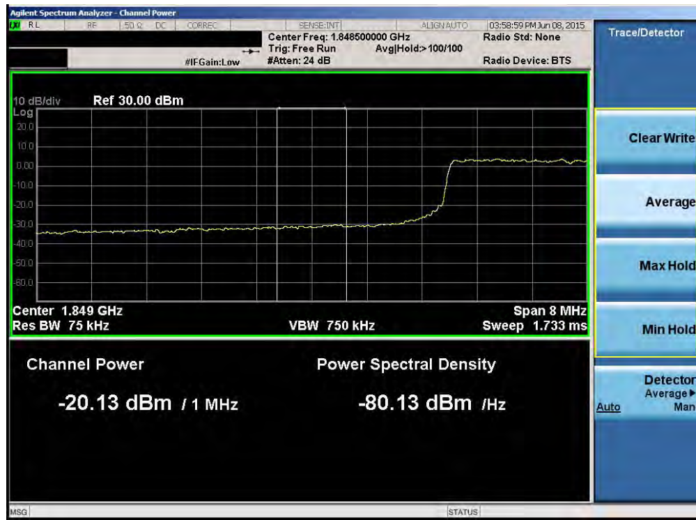
Plot 6-99. Lower Extended Band Edge Plot (Band 2 – 10.0MHz QPSK – RB Size 50)
