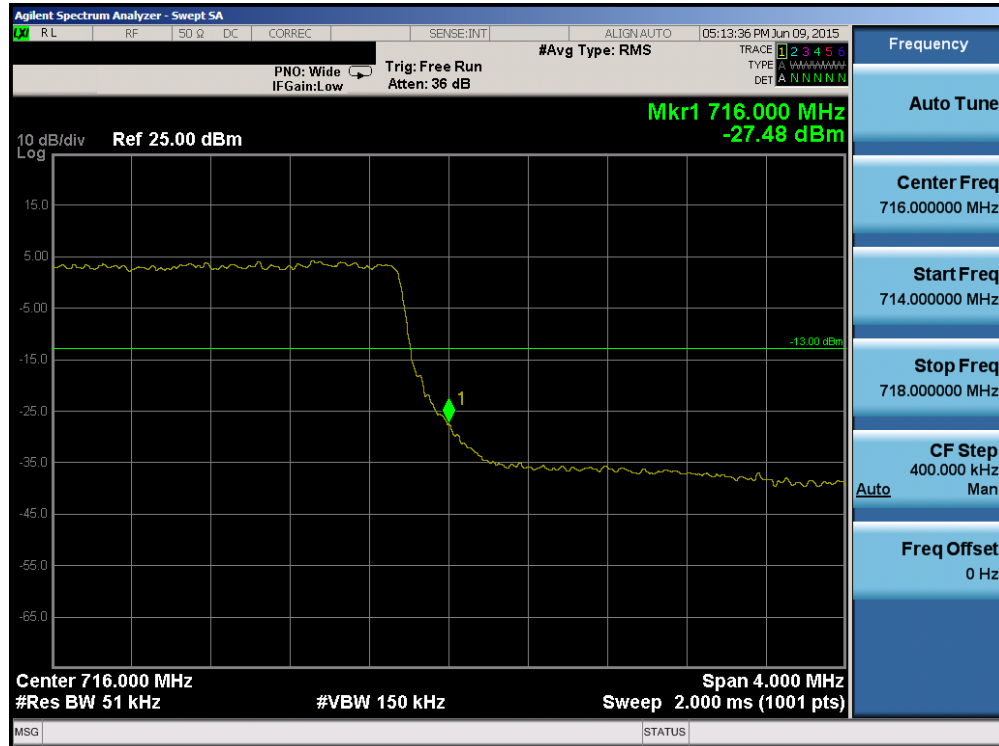
Plot 6-58. Upper Band Edge Plot (Band 12 – 5.0MHz QPSK – RB Size 25)
