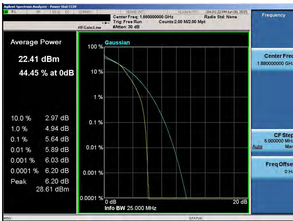
Plot 6-119. PAR Plot (Band 2 – 15.0MHz 16-QAM – RB Size 75)
