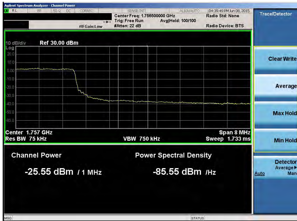
Plot 6-77. Upper Extended Band Edge Plot (Band 4 – 10.0MHz QPSK – RB Size 50)
