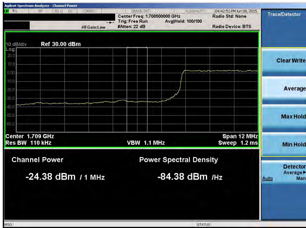
Plot 6-79. Lower Extended Band Edge Plot (Band 4 – 15.0MHz QPSK – RB Size 75)
