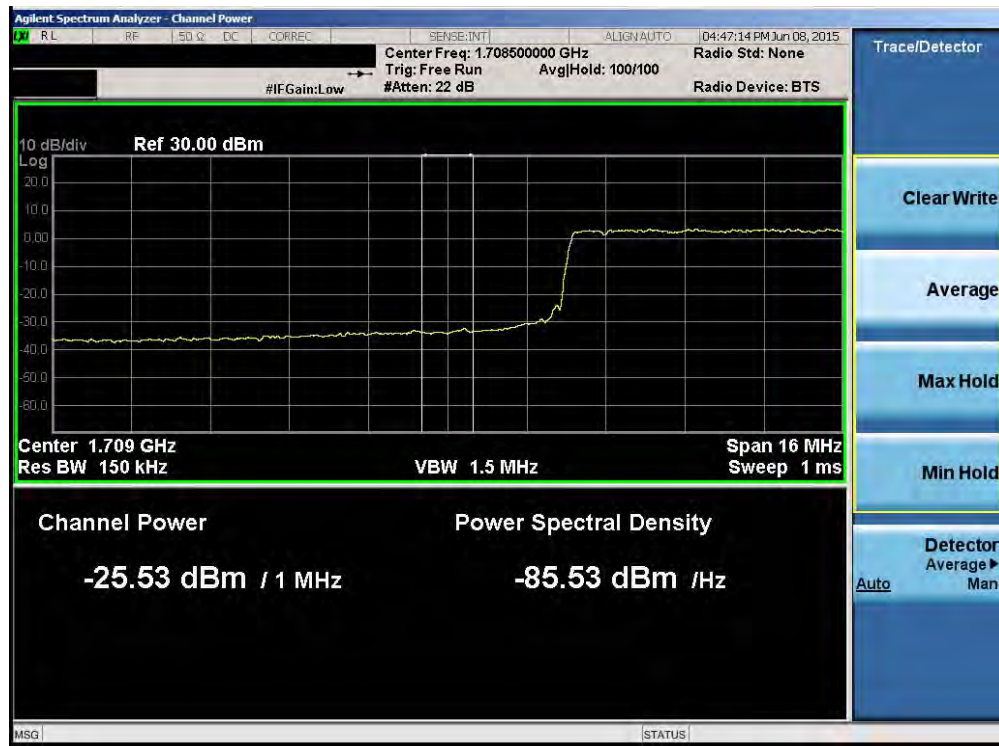
Plot 6-83. Lower Extended Band Edge Plot (Band 4 – 20.0MHz QPSK – RB Size 100)
