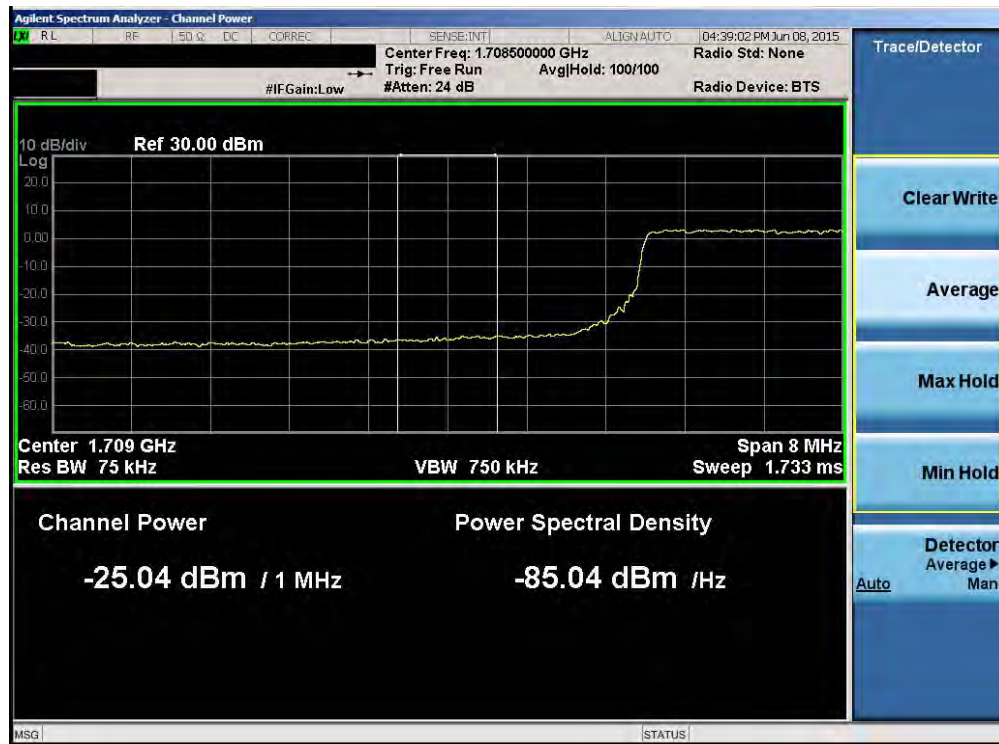
Plot 6-75. Lower Extended Band Edge Plot (Band 4 – 10.0MHz QPSK – RB Size 50)
