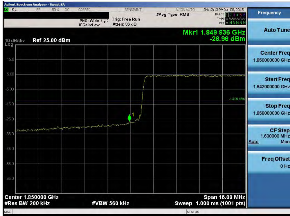
Plot 6-106. Lower Band Edge Plot (Band 2 – 20.0MHz QPSK – RB Size 100)
