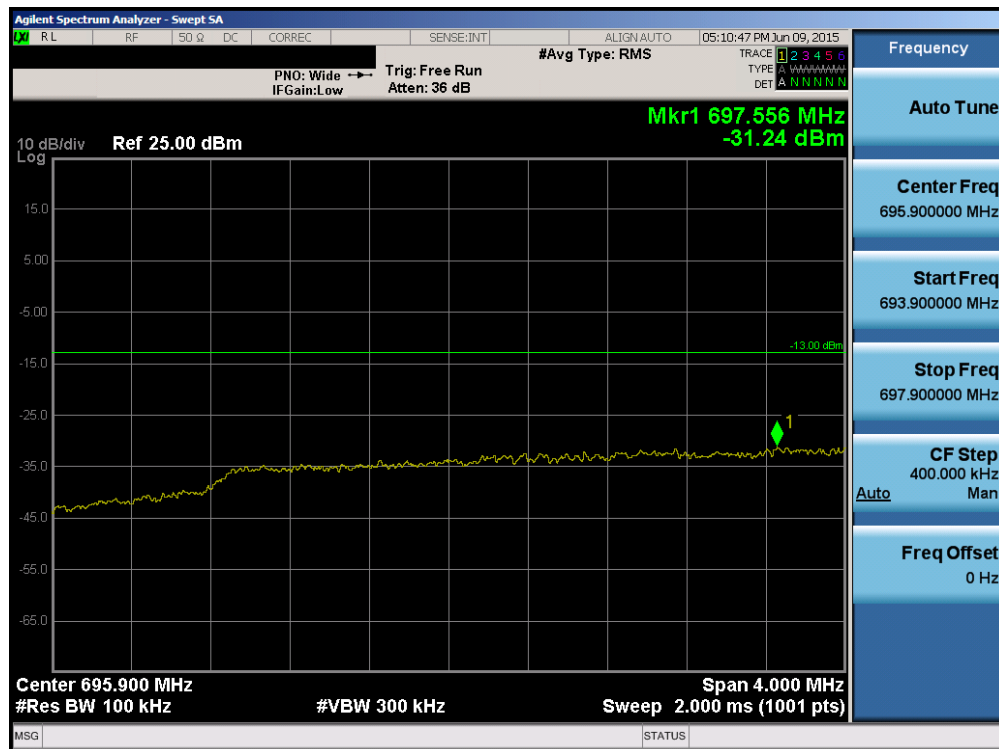
Plot 6-57. Lower Extended Band Edge Plot (Band 12 – 5.0MHz QPSK – RB Size 25)
