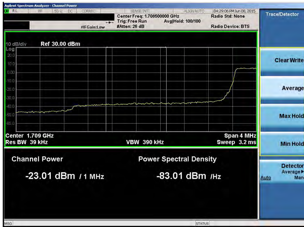
Plot 6-67. Lower Extended Band Edge Plot (Band 4 – 3.0MHz QPSK – RB Size 15)
