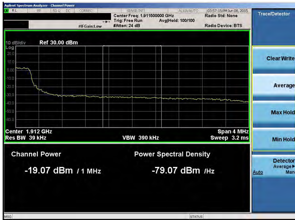
Plot 6-97. Upper Extended Band Edge Plot (Band 2 – 5.0MHz QPSK – RB Size 25)
