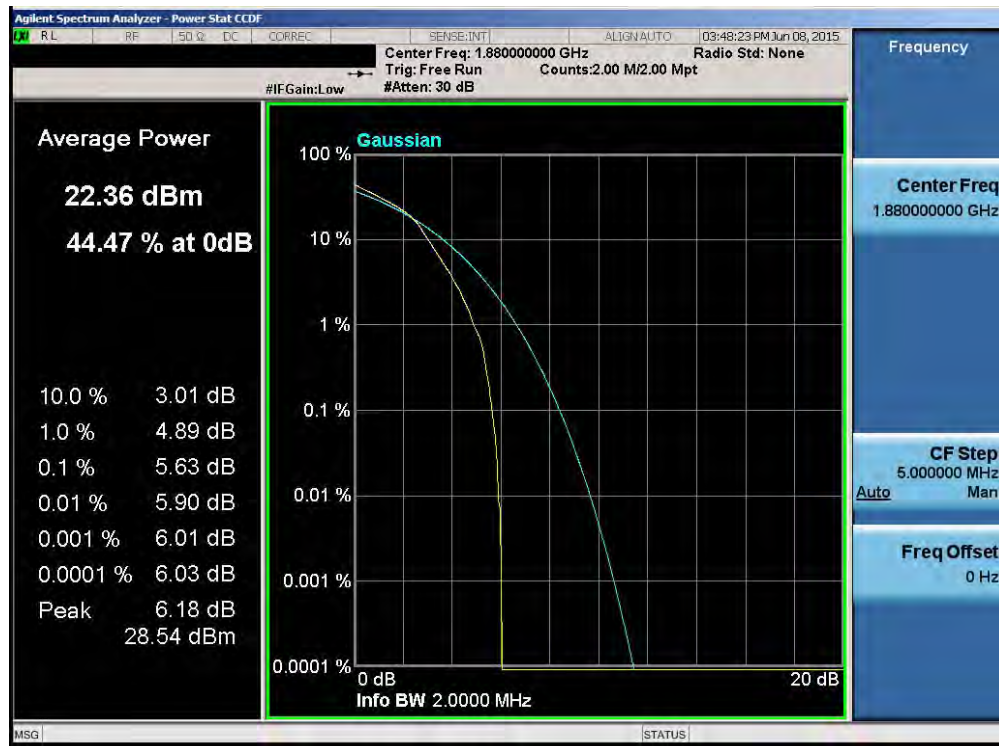
Plot 6-111. PAR Plot (Band 2 – 1.4MHz 16-QAM – RB Size 6)
