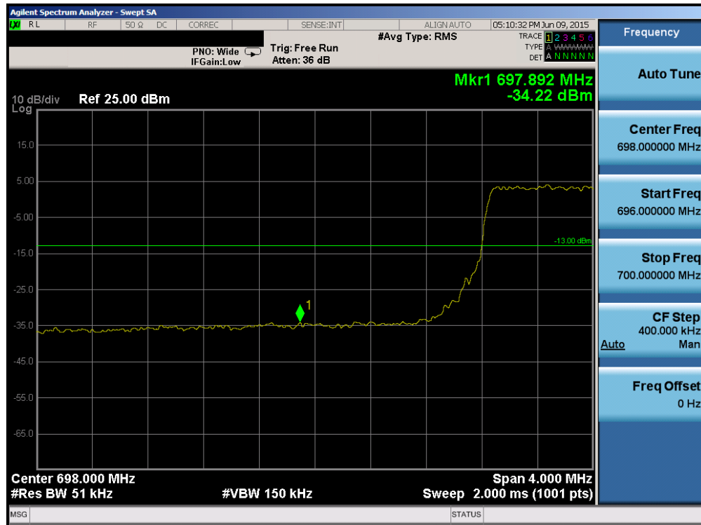
Plot 6-56. Lower Band Edge Plot (Band 12 – 5.0MHz QPSK – RB Size 25)
