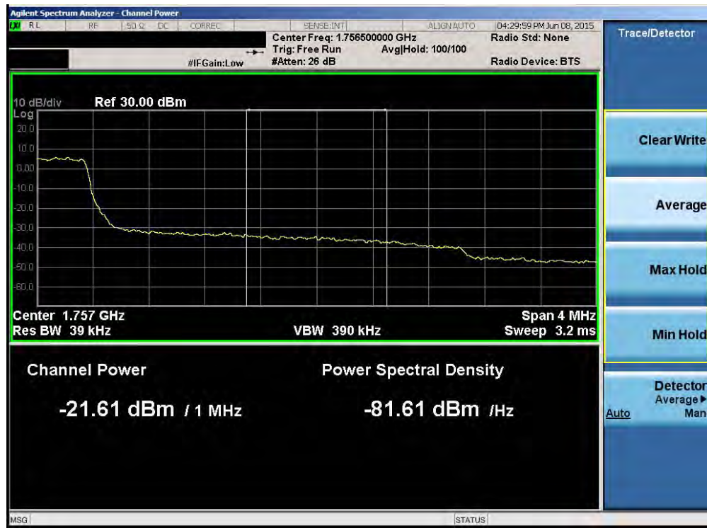
Plot 6-69. Upper Extended Band Edge Plot (Band 4 – 3.0MHz QPSK – RB Size 15)
