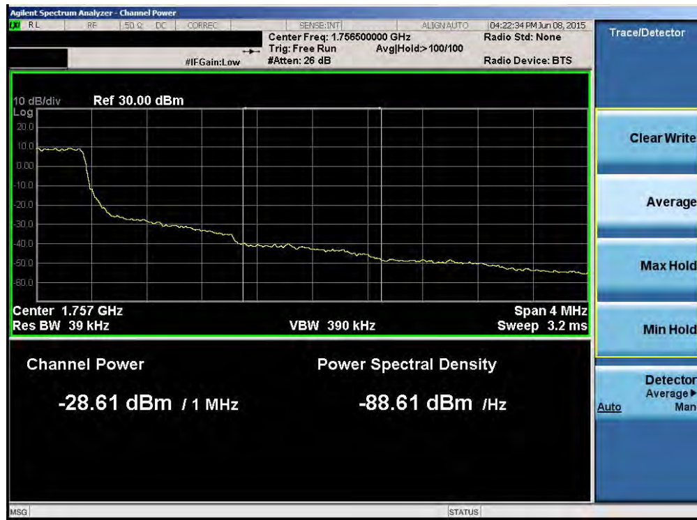
Plot 6-65. Upper Extended Band Edge Plot (Band 4 – 1.4MHz QPSK – RB Size 6)
