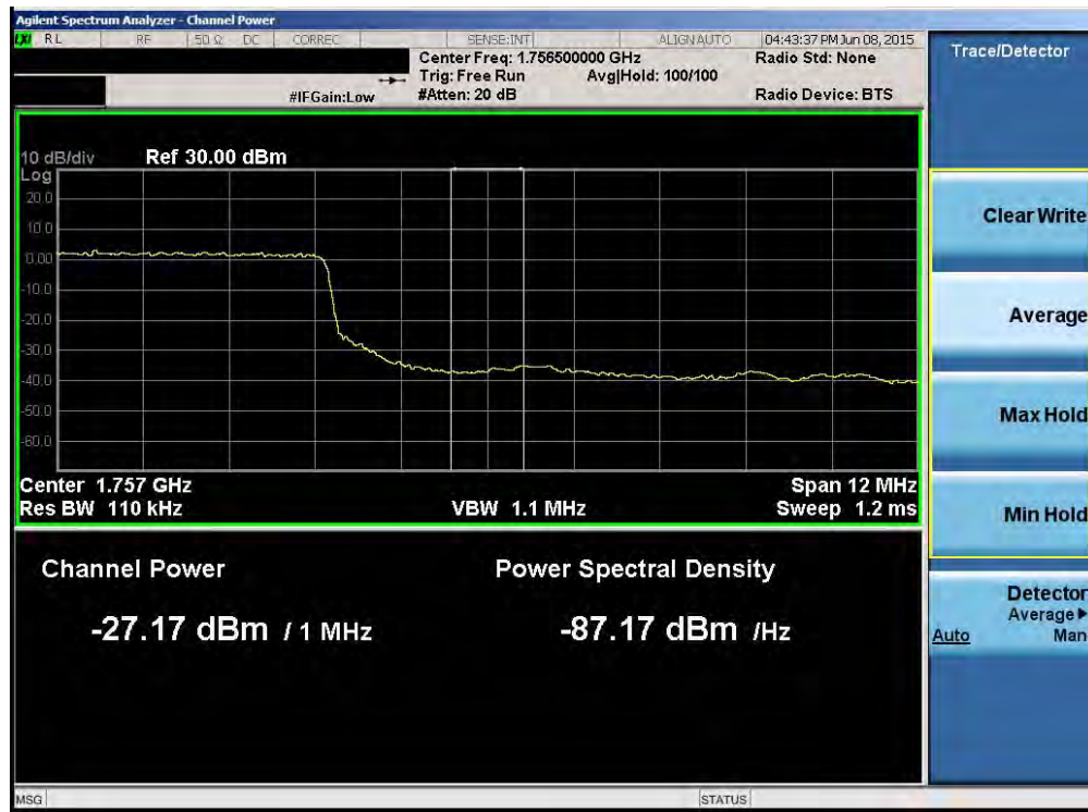
Plot 6-81. Upper Extended Band Edge Plot (Band 4 – 15.0MHz QPSK – RB Size 75)
