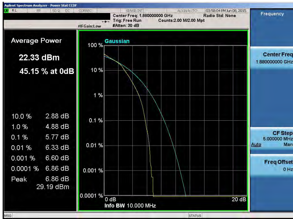
Plot 6-117. PAR Plot (Band 2 – 10.0MHz 16-QAM – RB Size 50)
