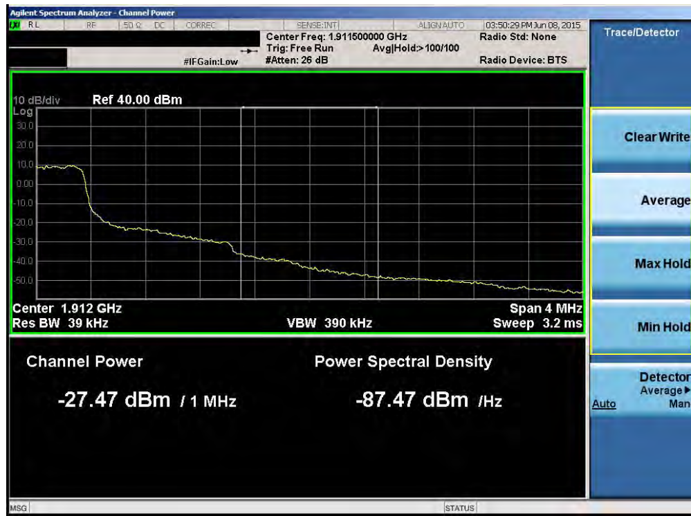
Plot 6-89. Upper Extended Band Edge Plot (Band 2 – 1.4MHz QPSK – RB Size 6)
