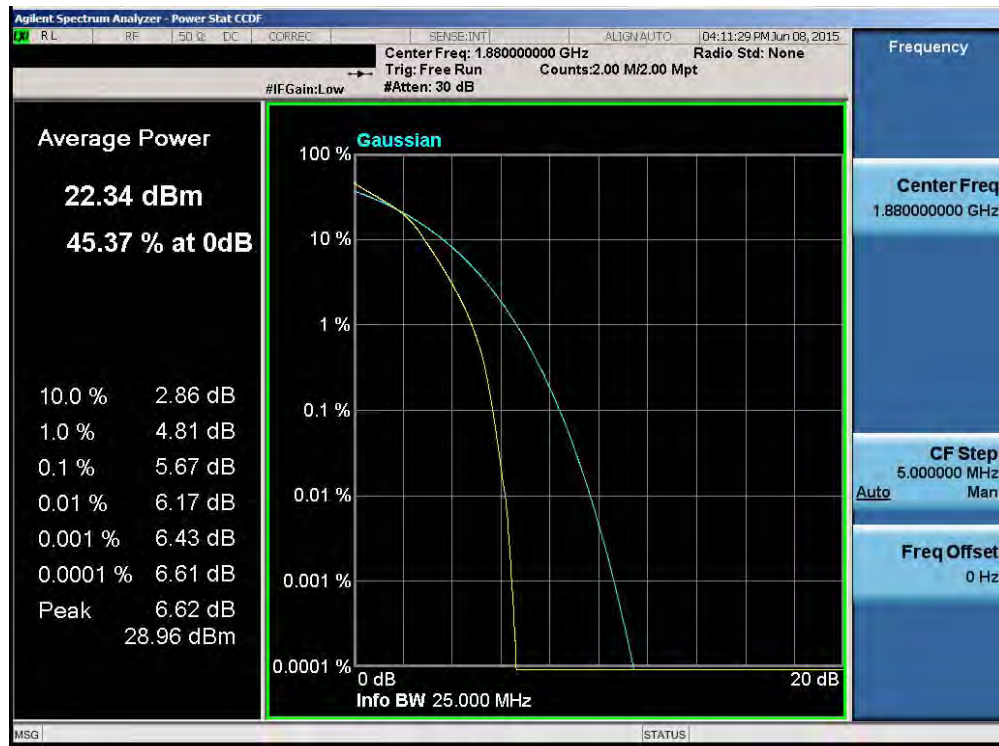
Plot 6-121. PAR Plot (Band 2 – 20.0MHz 16-QAM – RB Size 100)
