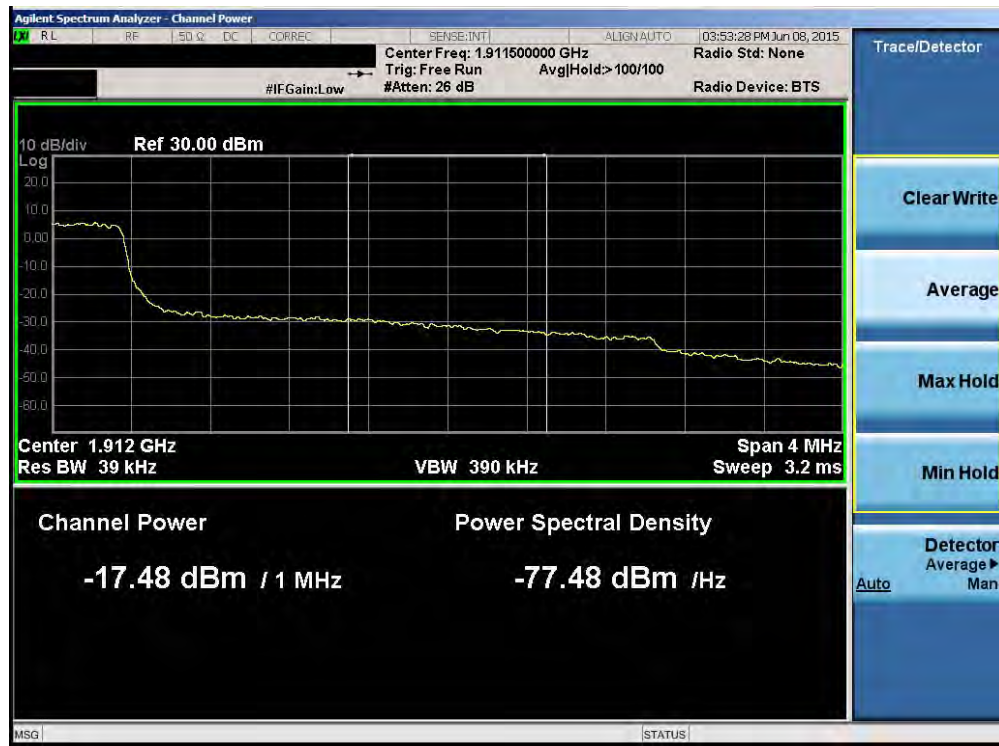
Plot 6-93. Upper Extended Band Edge Plot (Band 2 – 3.0MHz QPSK – RB Size 15)
