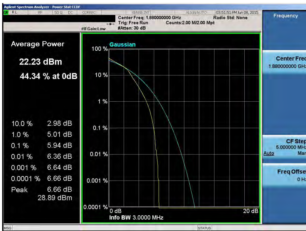
Plot 6-113. PAR Plot (Band 2 – 3.0MHz 16-QAM – RB Size 15)
