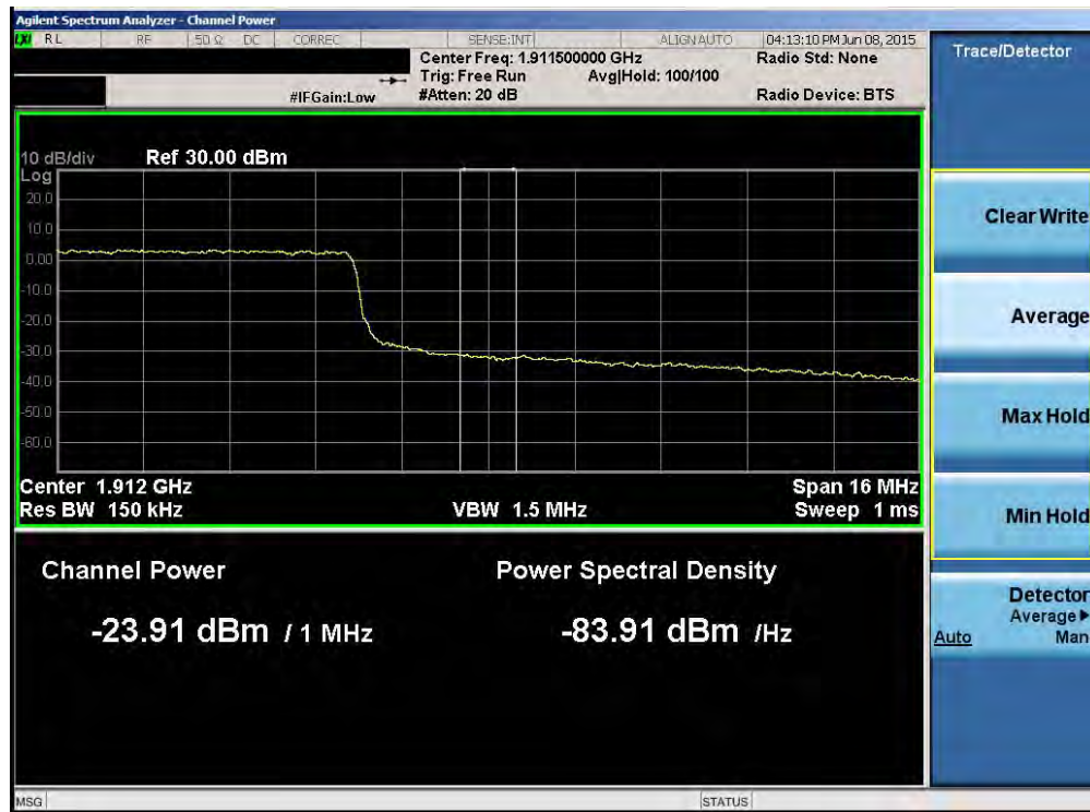
Plot 6-109. Upper Extended Band Edge Plot (Band 2 – 20.0MHz QPSK – RB Size 100)
