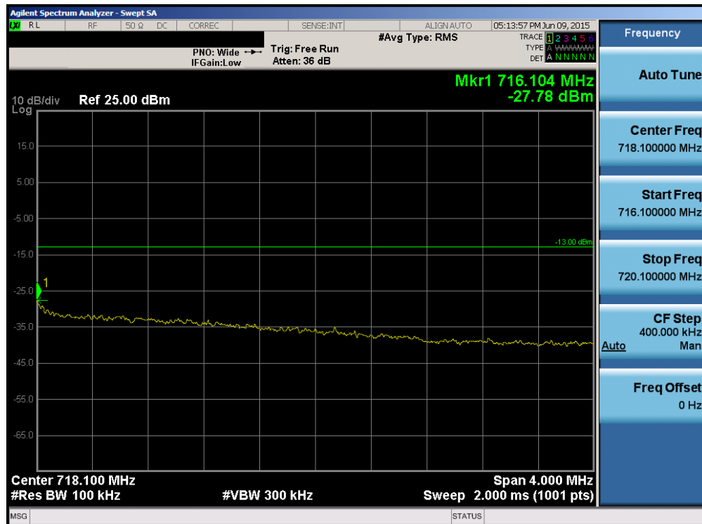
Plot 6-59. Upper Extended Band Edge Plot (Band 12 – 5.0MHz QPSK – RB Size 25)
