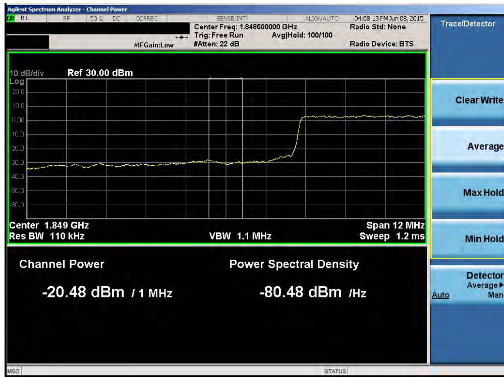
Plot 6-103. Lower Extended Band Edge Plot (Band 2 – 15.0MHz QPSK – RB Size 75)
