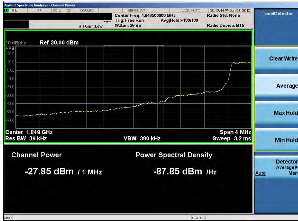
Plot 6-87. Lower Extended Band Edge Plot (Band 2 – 1.4MHz QPSK – RB Size 6)
