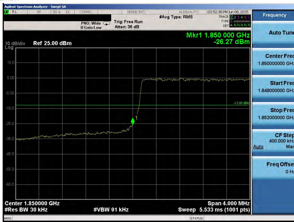
Plot 6-90. Lower Band Edge Plot (Band 2 – 3.0MHz QPSK – RB Size 15)
