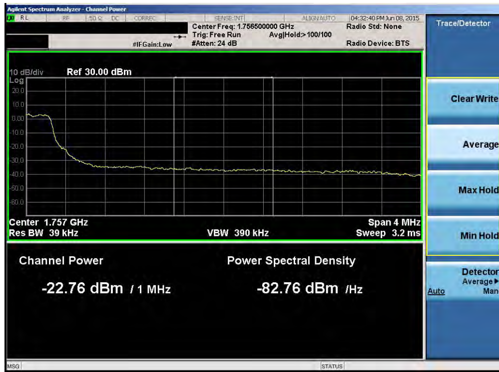
Plot 6-73. Upper Extended Band Edge Plot (Band 4 – 5.0MHz QPSK – RB Size 25)
