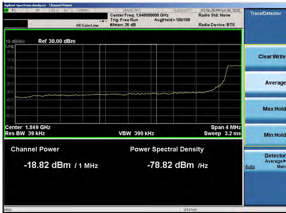
Plot 6-95. Lower Extended Band Edge Plot (Band 2 – 5.0MHz QPSK – RB Size 25)
