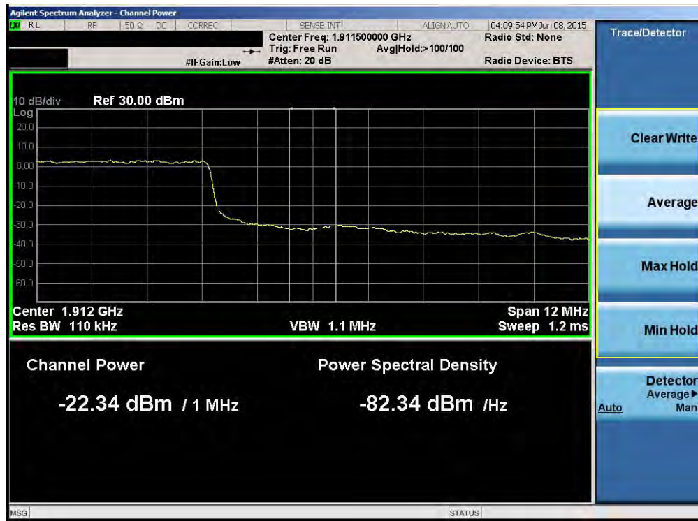
Plot 6-105. Upper Extended Band Edge Plot (Band 2 – 15.0MHz QPSK – RB Size 75)
