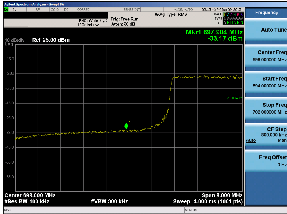
Plot 6-60. Lower Band Edge Plot (Band 12 – 10.0MHz QPSK – RB Size 50)
