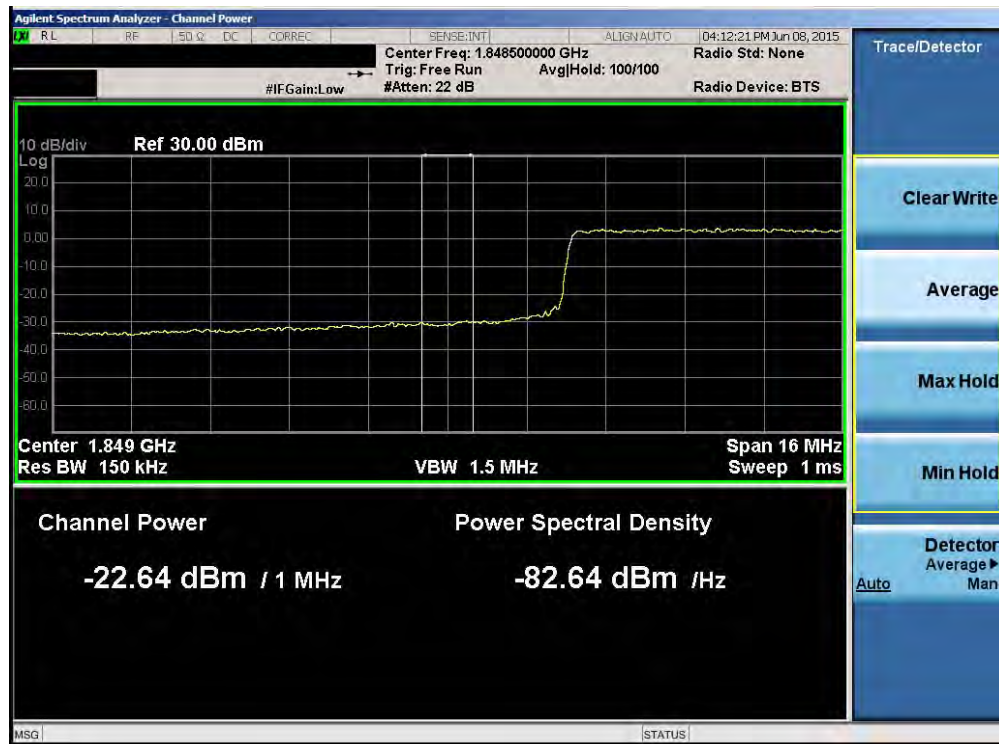
Plot 6-107. Lower Extended Band Edge Plot (Band 2 – 20.0MHz QPSK – RB Size 100)
