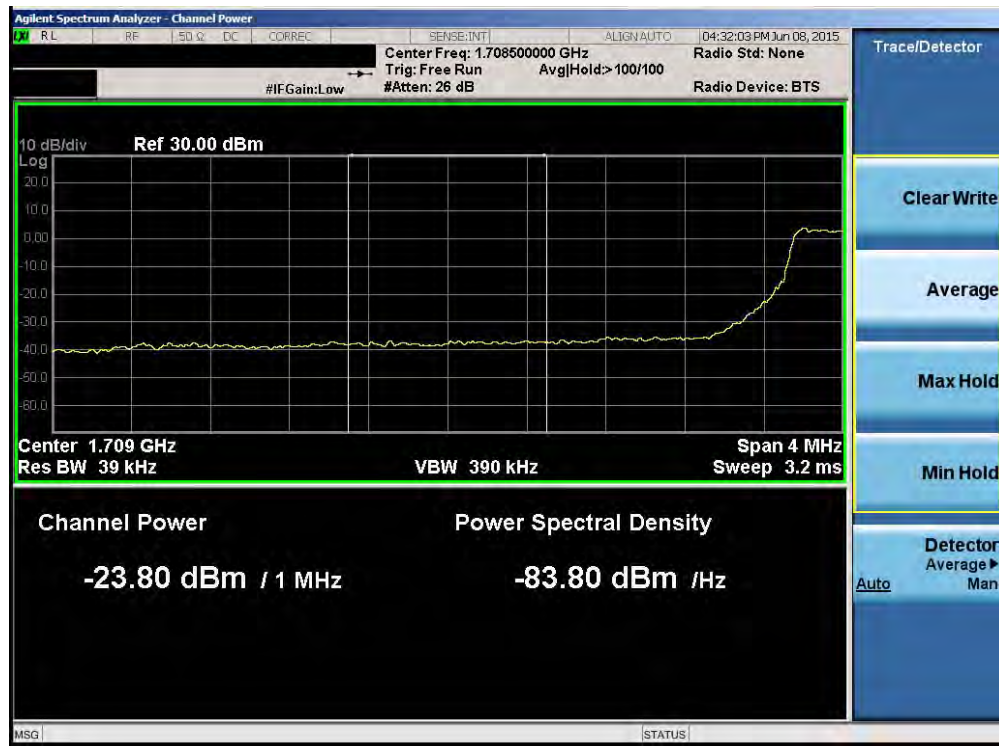
Plot 6-71. Lower Extended Band Edge Plot (Band 4 – 5.0MHz QPSK – RB Size 25)
