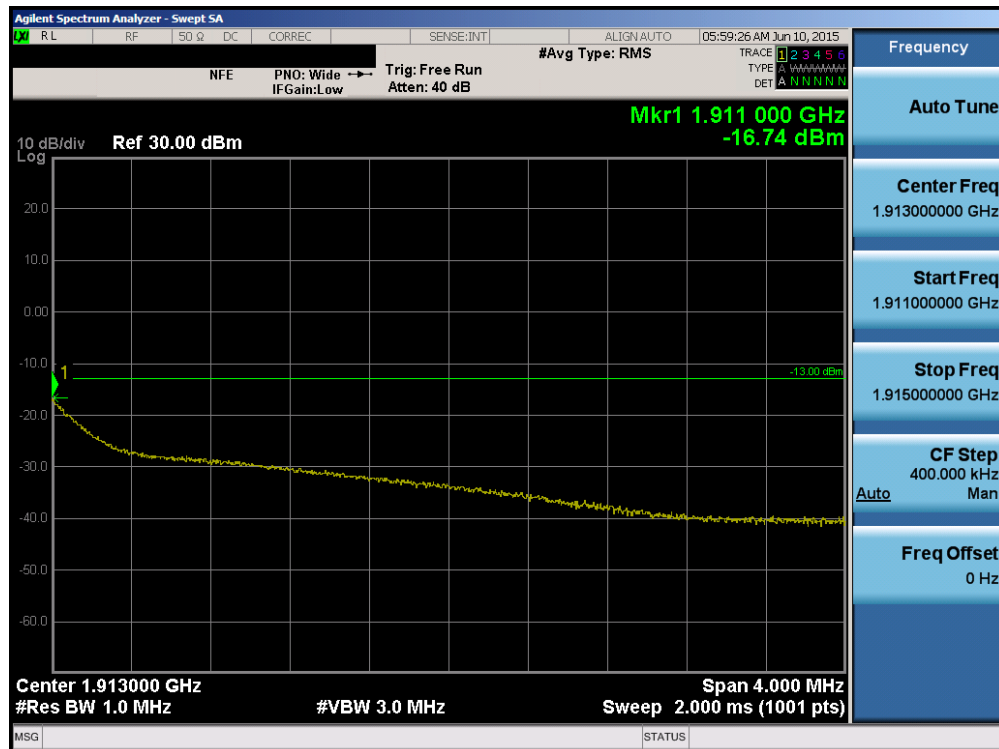
Plot 6-40. 4MHz Span Plot (PCS WCDMA Mode – Ch. 9538)
