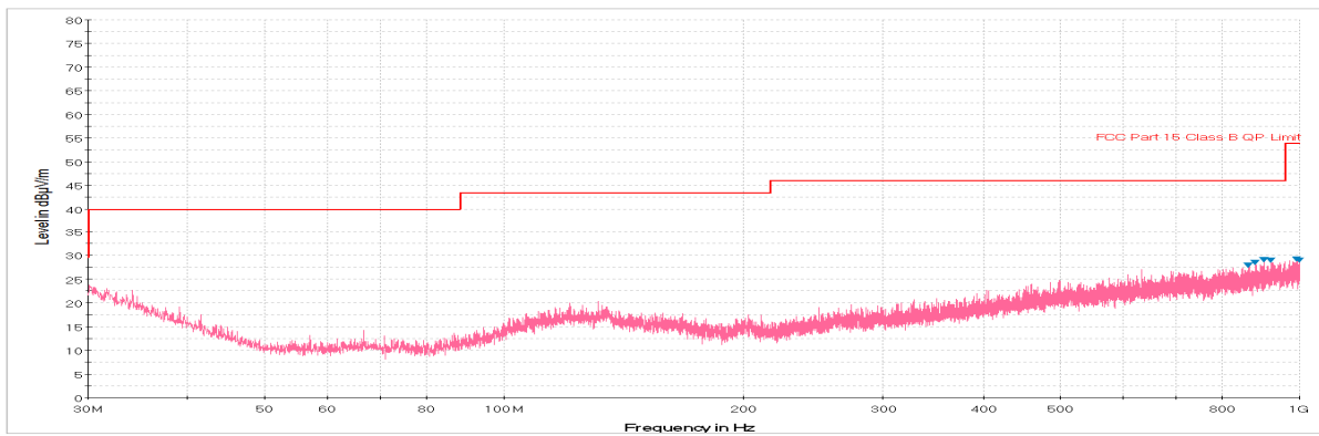
Plot 6-92. Radiated Spurious Plot below 1GHz (802.11a – U3 Ch. 157, Ant. Pol. V)
