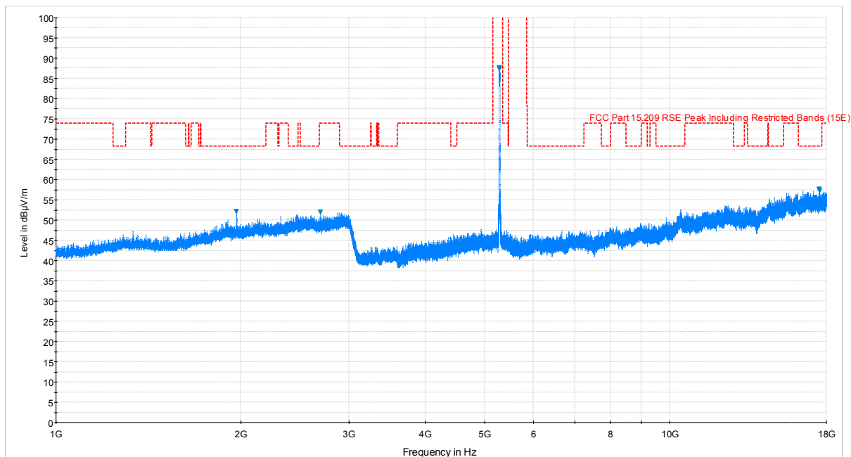
Plot 6-70. Radiated Spurious Plot above 1GHz (802.11a – U2A Ch. 56, Ant. Pol. V)
