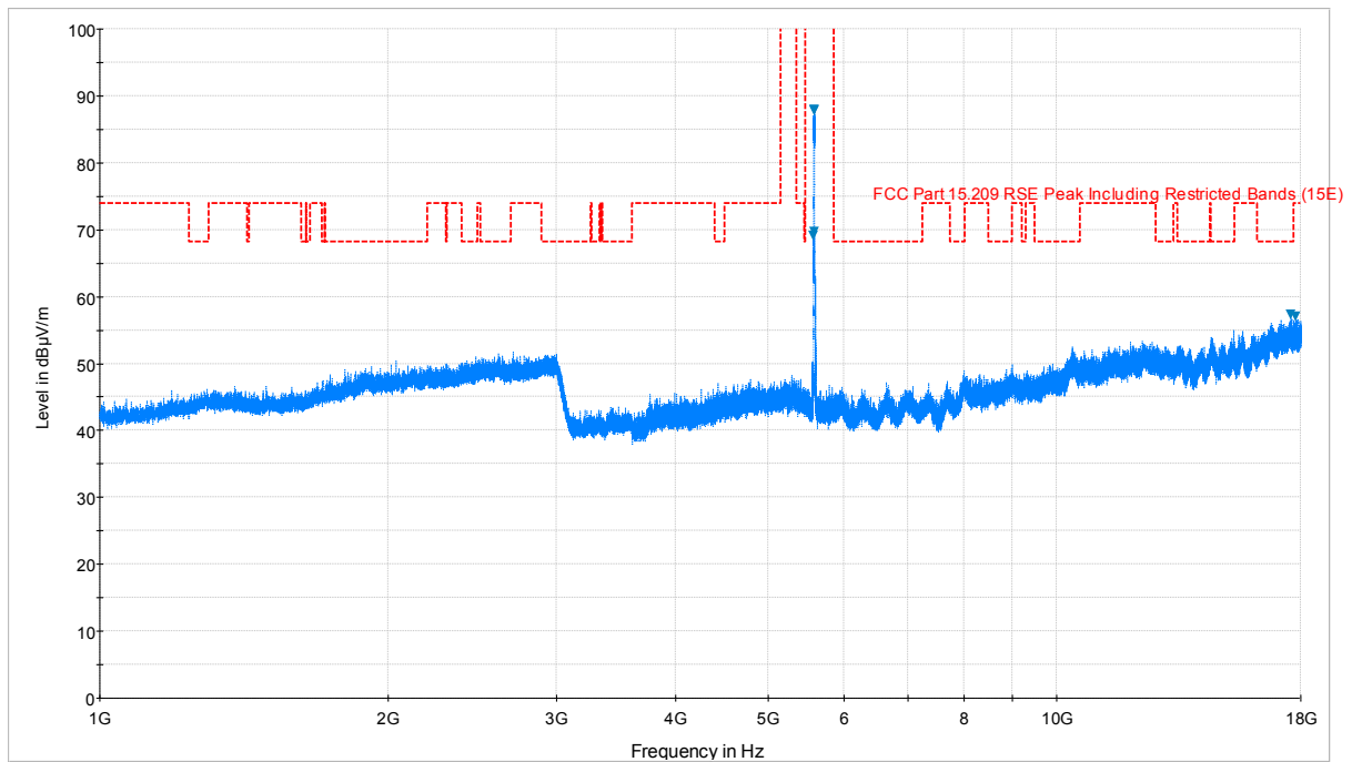
Plot 6-71. Radiated Spurious Plot above 1GHz (802.11a – U2C Ch. 116, Ant. Pol. H)
