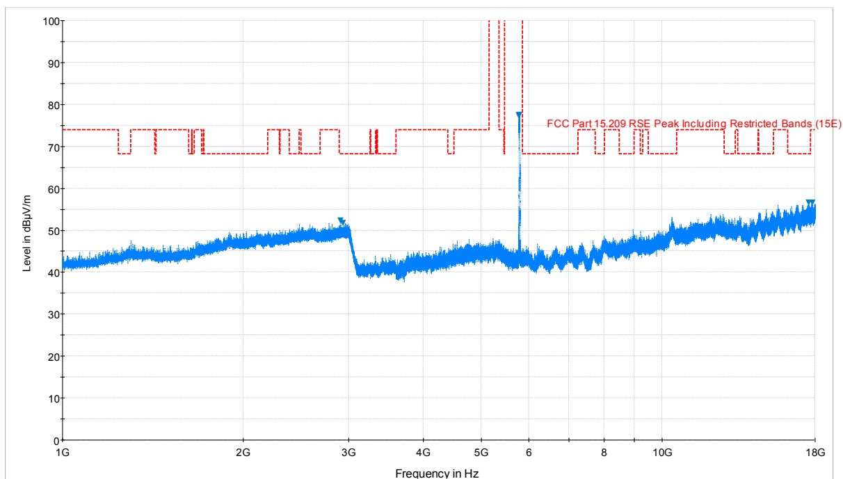
Plot 6-74. Radiated Spurious Plot above 1GHz (802.11a – U3 Ch. 157, Ant. Pol. V)
