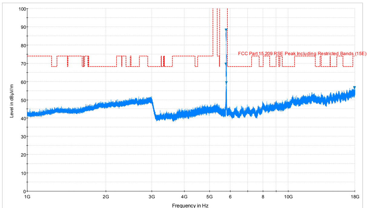
Plot 6-73. Radiated Spurious Plot above 1GHz (802.11a – U3 Ch. 157, Ant. Pol. H)
