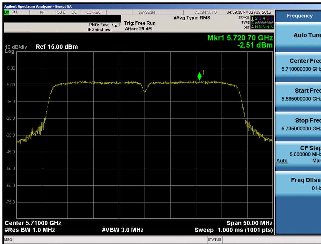
Plot 6-58. Power Spectral Density Plot (40MHz BW 802.11n (UNII Band 2C) – Ch. 142)
