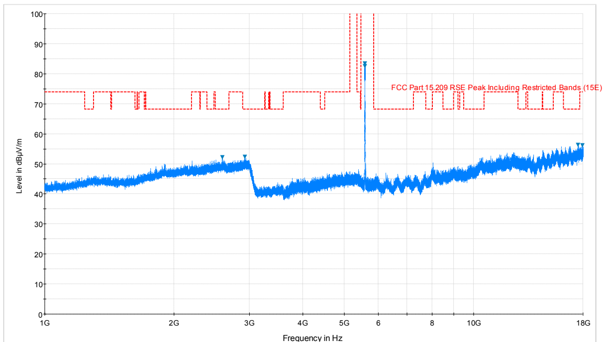
Plot 6-72. Radiated Spurious Plot above 1GHz (802.11a – U2C Ch. 116, Ant. Pol. V)
