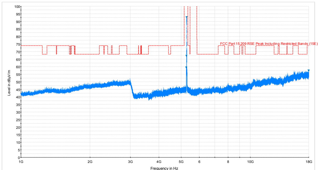
Plot 6-69. Radiated Spurious Plot above 1GHz (802.11a – U2A Ch. 56, Ant. Pol. H)
