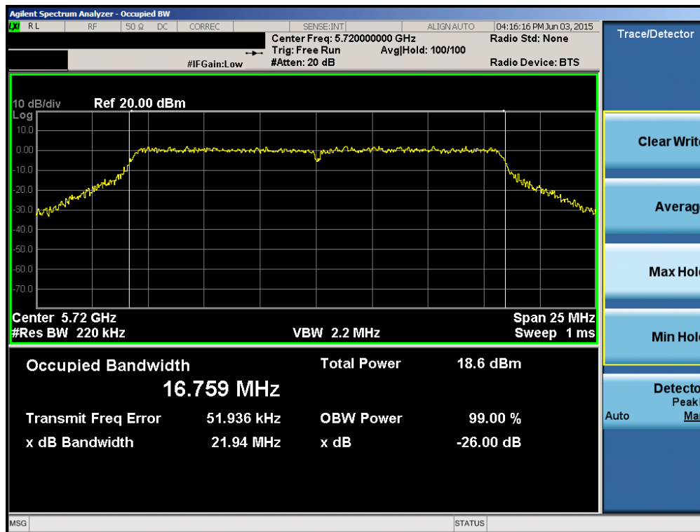
Plot 6-19. 26dB Bandwidth Plot (802.11a (UNII Band 2C) – Ch. 144)
