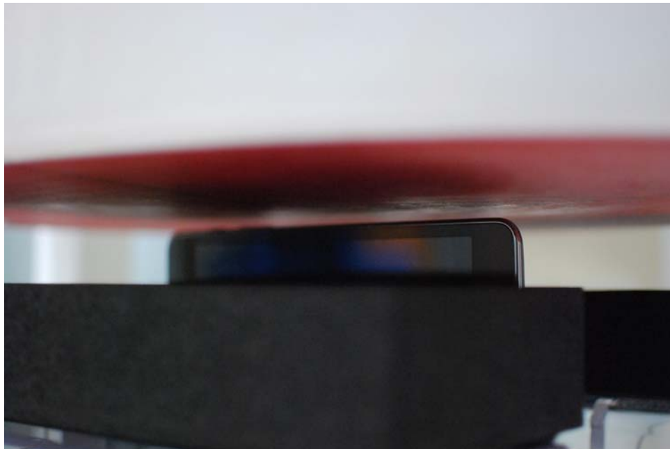
SAR Test Setup Photo 8: Right Edge at 0.6 cm
