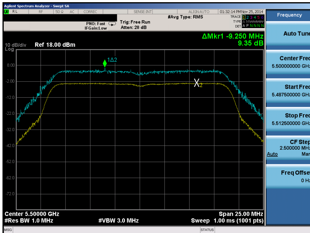
Plot 6-58. Peak Excursion Ratio Plot (20MHz BW 802.11n (UNII Band 2C) – Ch. 100)
