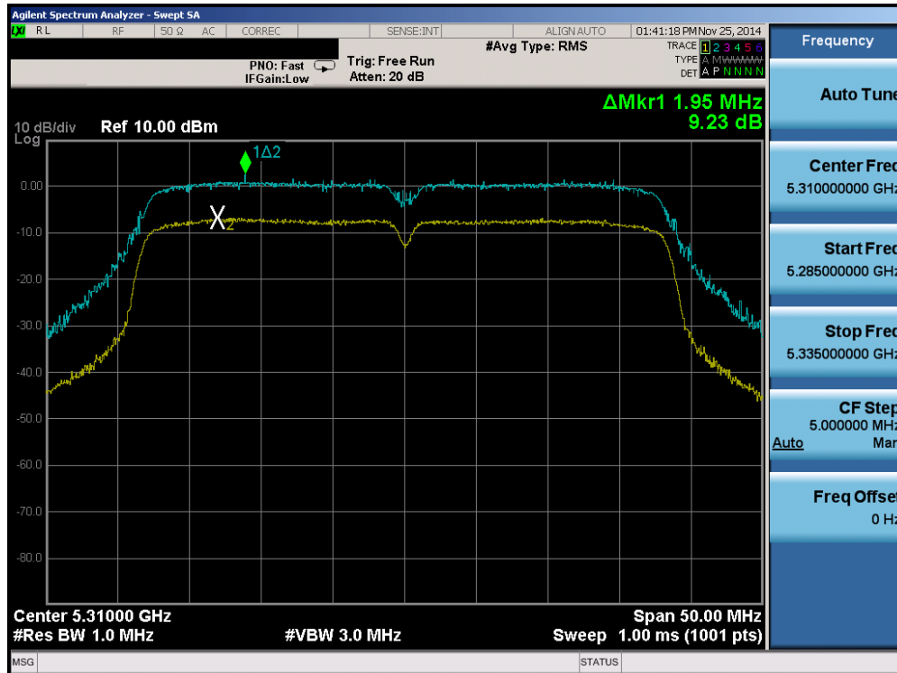
Plot 6-57. Peak Excursion Ratio Plot (40MHz BW 802.11n (UNII Band 2A) – Ch. 62)
