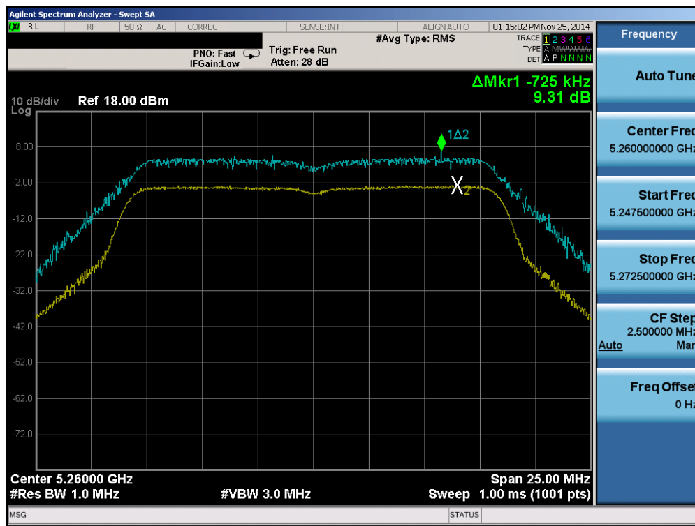
Plot 6-56. Peak Excursion Ratio Plot (802.11a (UNII Band 2A) – Ch. 52)
