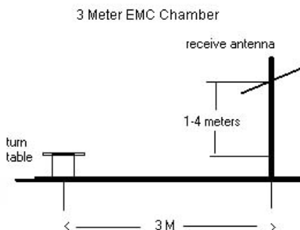
Figure 6-6. Test Instrument & Measurement Setup
