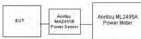
Figure 10-2 Power Measurement Setup
