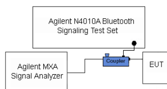
Figure 10-3 Power Measurement Setup
