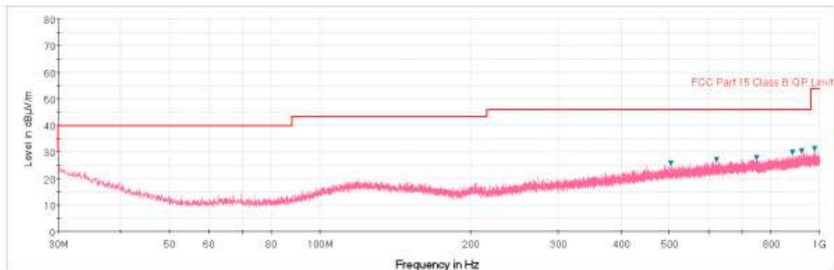
Plot 7-87. Radiated Spurious Plot below 1GHz (802.11a – U3 Ch. 157, Ant. Pol. H)
