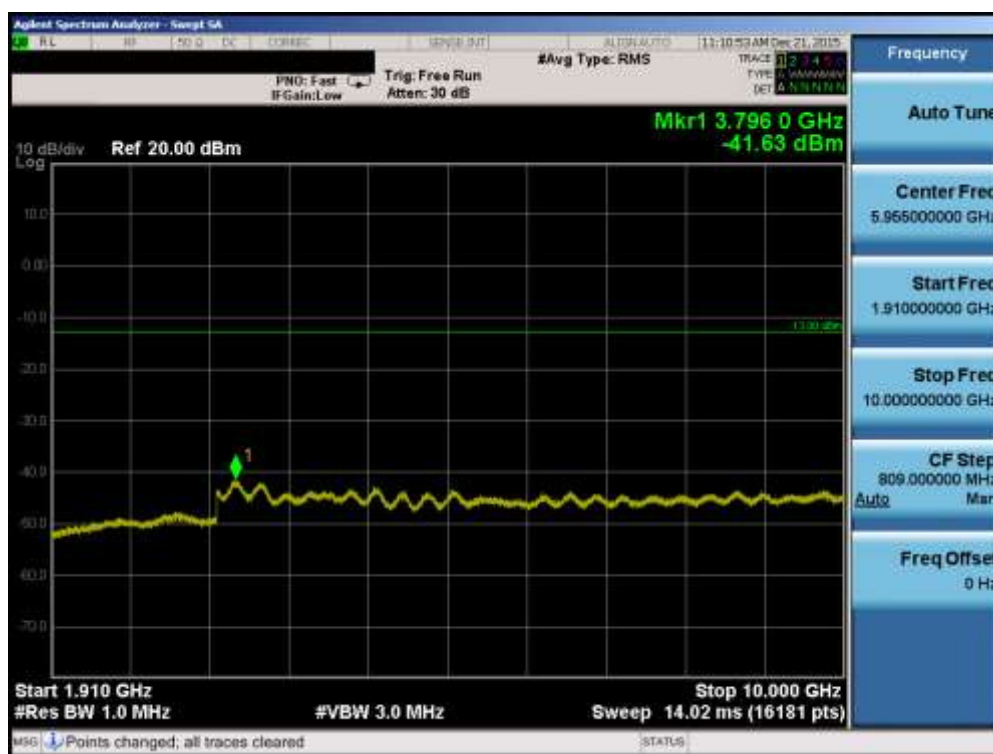
Plot 7-16. Conducted Spurious Plot (PCS WCDMA Mode – Ch. 9400)
