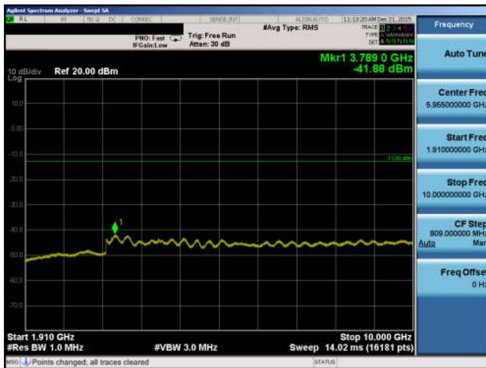
Plot 7-13. Conducted Spurious Plot (PCS WCDMA Mode – Ch. 9262)
