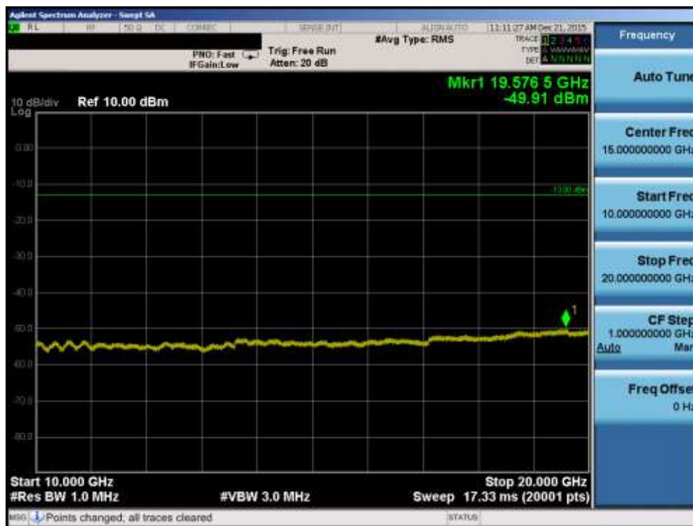
Plot 7-17. Conducted Spurious Plot (PCS WCDMA Mode – Ch. 9400)
