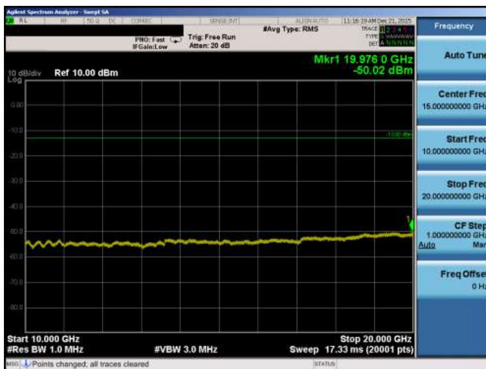
Plot 7-20. Conducted Spurious Plot (PCS WCDMA Mode – Ch. 9538)
