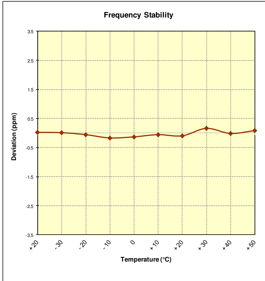
Figure 7-9. Frequency Stability Graph (PCS WCDMA Mode – Ch. 9400)
