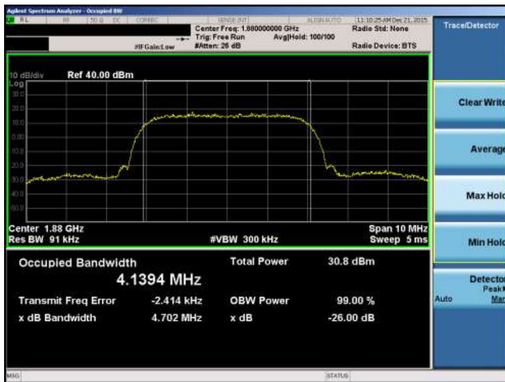
Plot 7-2. Occupied Bandwidth Plot (PCS WCDMA Mode – Ch. 9400)
