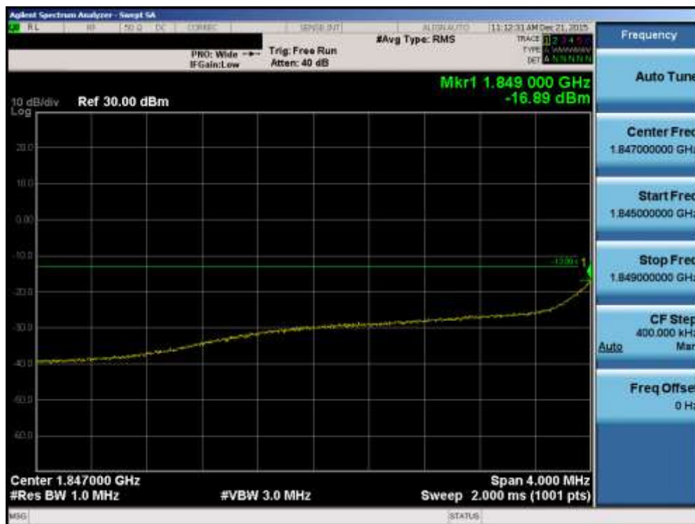
Plot 7-24. 4MHz Span Plot (PCS WCDMA Mode – Ch. 9262)
