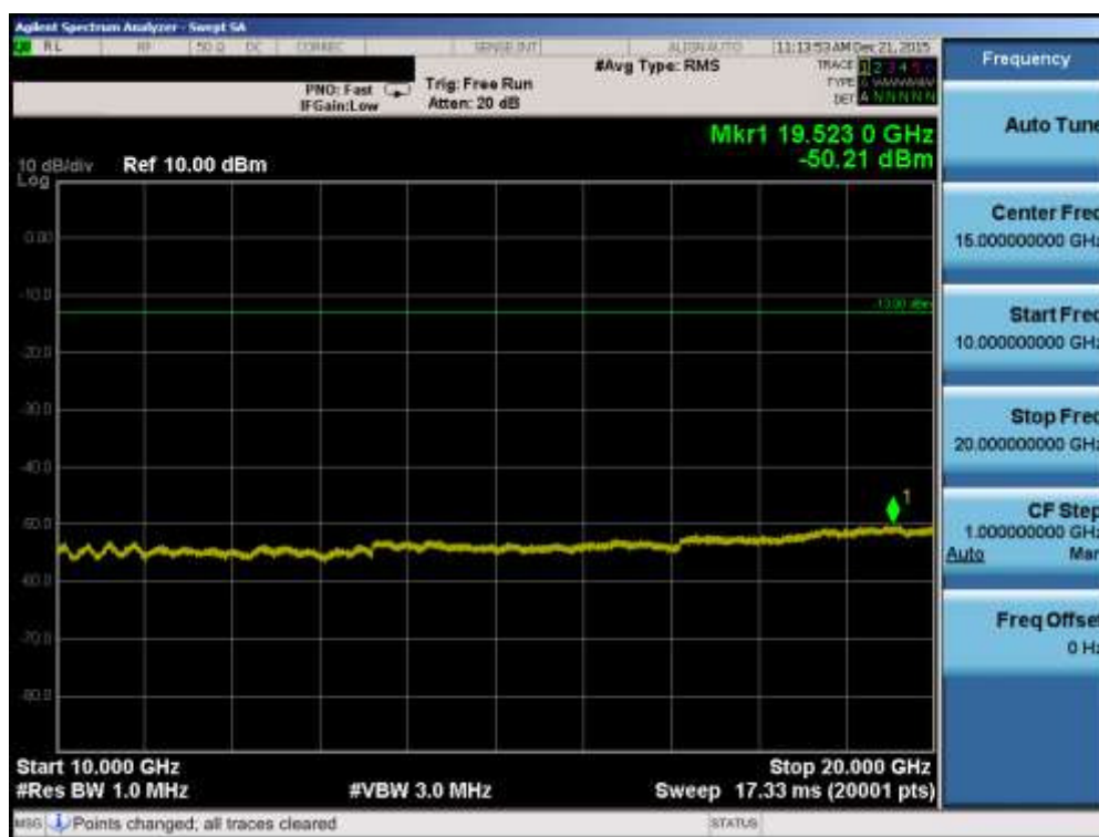
Plot 7-14. Conducted Spurious Plot (PCS WCDMA Mode – Ch. 9262)
