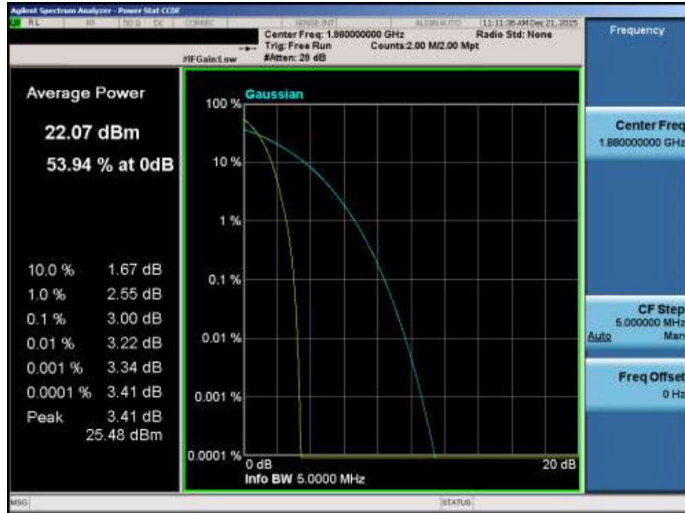
Plot 7-27. Peak-Average Ratio Plot (PCS WCDMA Mode – Ch. 9400)
