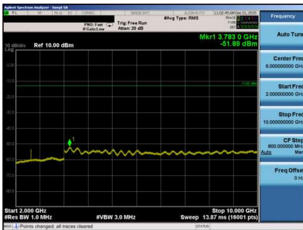
Plot 7-8. Conducted Spurious Plot (Cellular WCDMA Mode – Ch. 4183)
