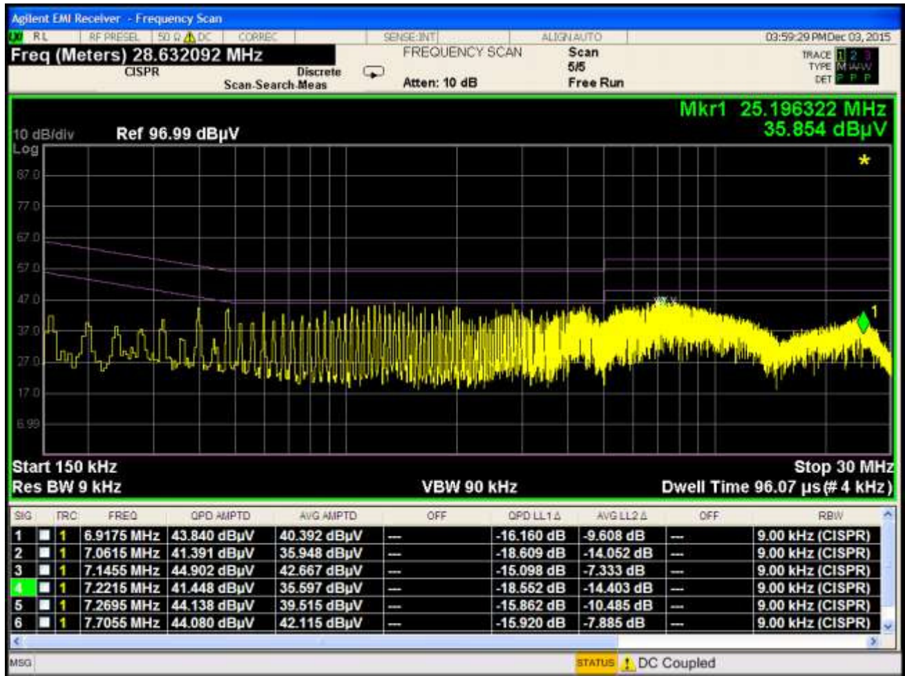
Plot 7-47. Line Conducted Plot with 802.11b (L1)
