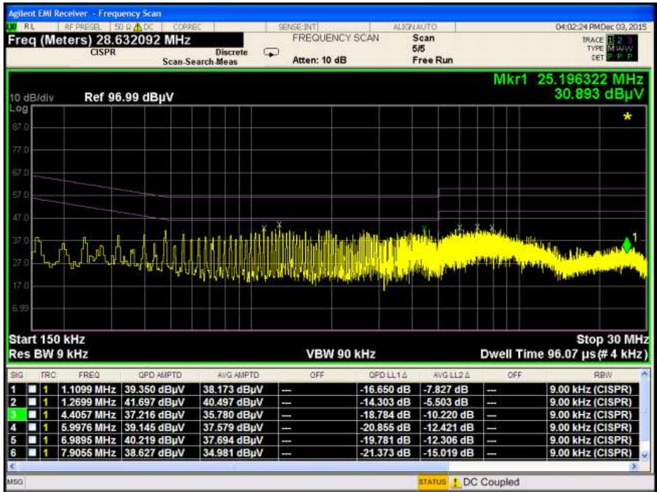
Plot 7-48. Line Conducted Plot with 802.11b (N)
