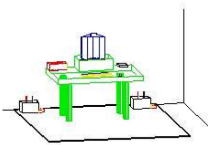
Figure 7-8. Test Instrument & Measurement Setup
