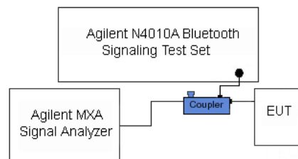
Figure 8-3 Power Measurement Setup
