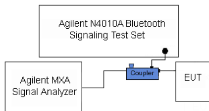
Figure 8-3 Power Measurement Setup
