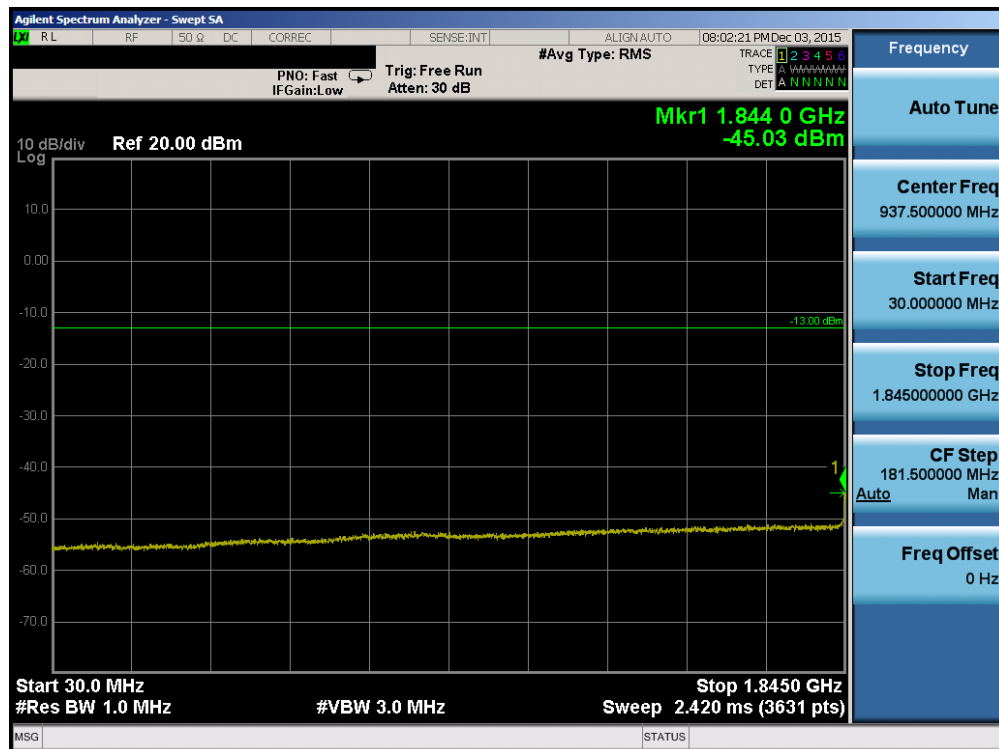
Plot 7-12. Conducted Spurious Plot (PCS WCDMA Mode – Ch. 9262)
