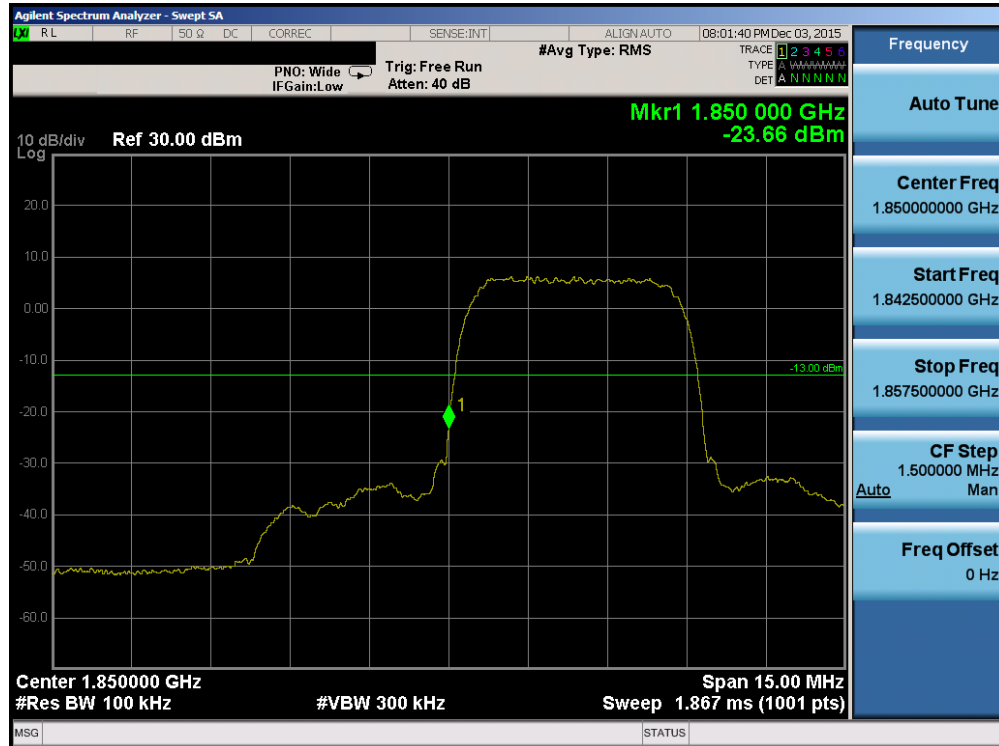
Plot 7-23. Band Edge Plot (PCS WCDMA Mode – Ch. 9262)
