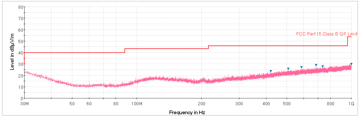
Plot 7-88. Radiated Spurious Plot below 1GHz (802.11a – U3 Ch. 157, Ant. Pol. V)
