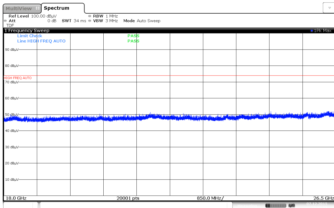
Plot 7-75. Radiated Spurious Plot from 18GHz – 26.5 GHz (802.11a – Ant. Pol. H)
