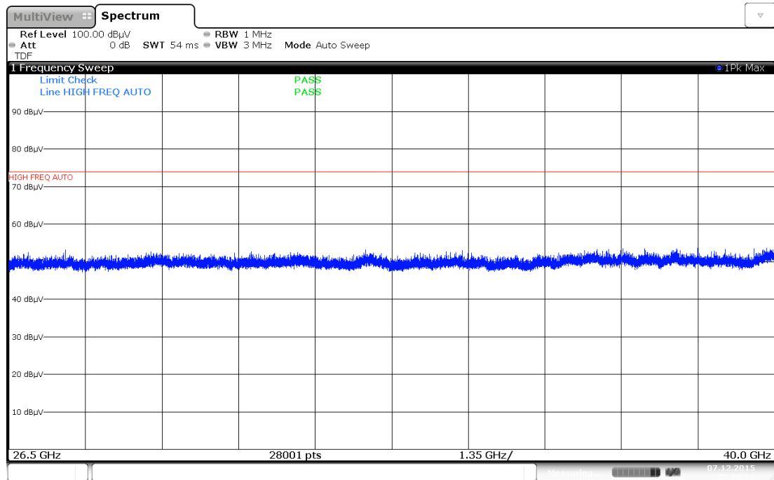
Plot 7-78. Radiated Spurious Plot above 26.5GHz (802.11a – Ant. Pol. V)
