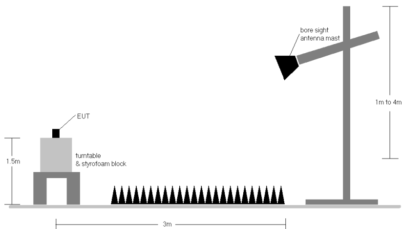
Figure 7-6. Test Instrument & Measurement Setup
