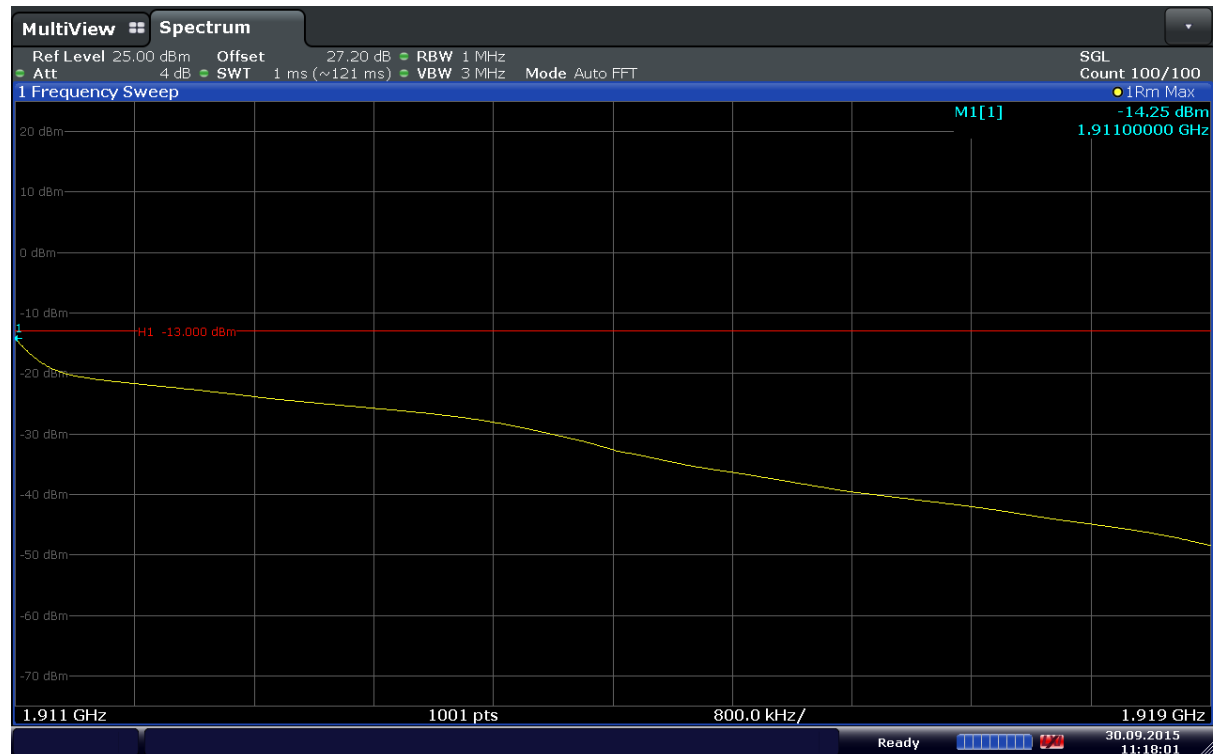
Plot 6-80. Extended Upper Band Edge Plot (Band2 – 5.0MHz – QPSK – RB Size 25)
