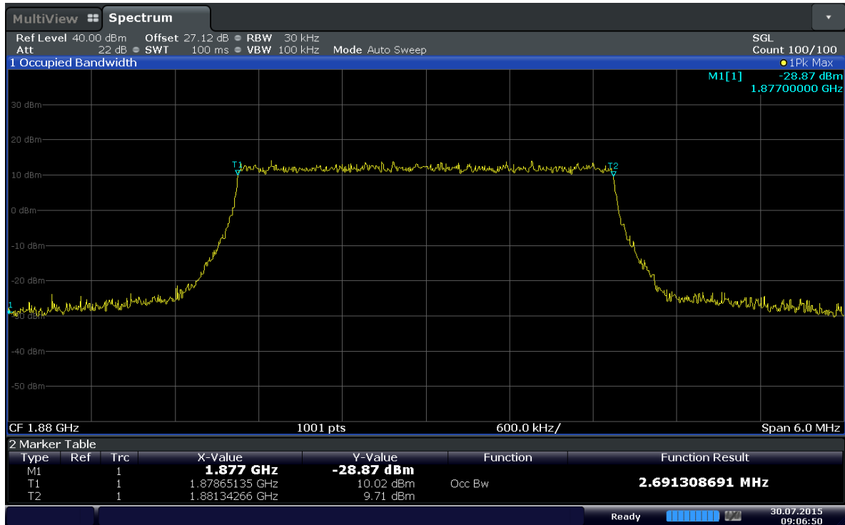
Plot 6-3. Occupied Bandwidth Plot (Band 2 – 3.0MHz – QPSK – RB Size 15)
