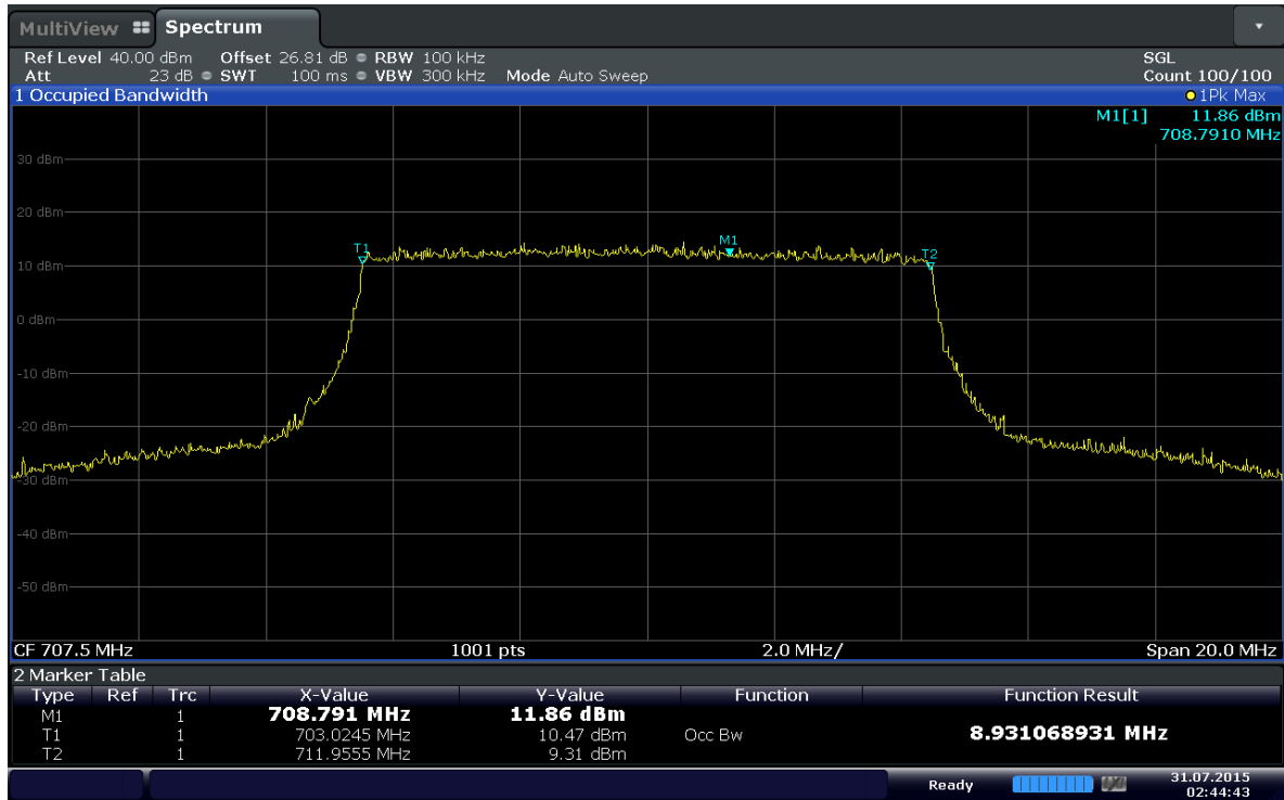
Plot 6-7. Occupied Bandwidth Plot (Band 12 – 10MHz QPSK - RB Size 50)
