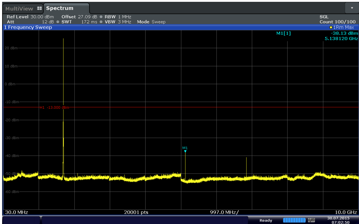
Plot 6-43. Conducted Spurious Plot (Band 4–3MHz–QPSK–RB Size 1–RB Offset 14–Ch.19965)
