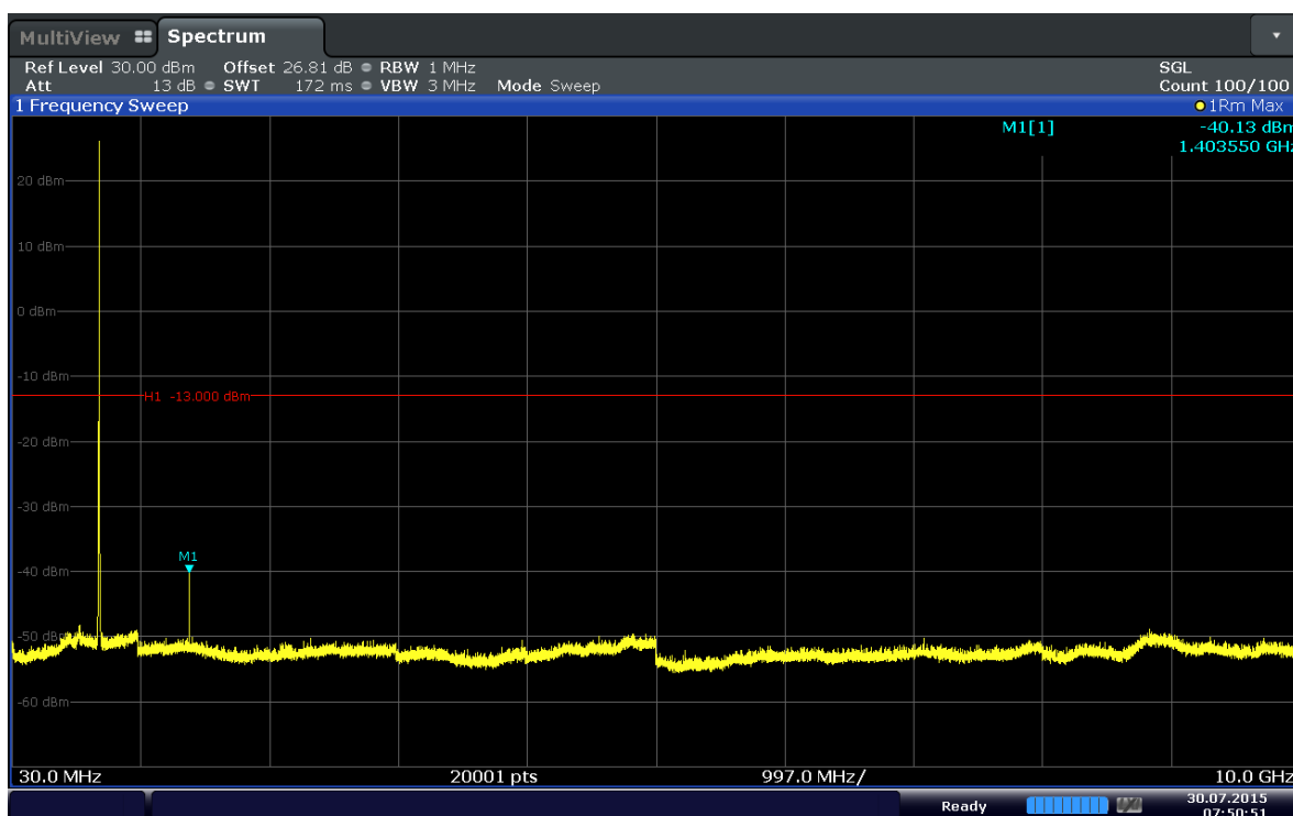
Plot 6-28. Conducted Spurious Plot (Band 12–3MHz–QPSK–RB Size 1–RB Offset 14–Ch.23025)
