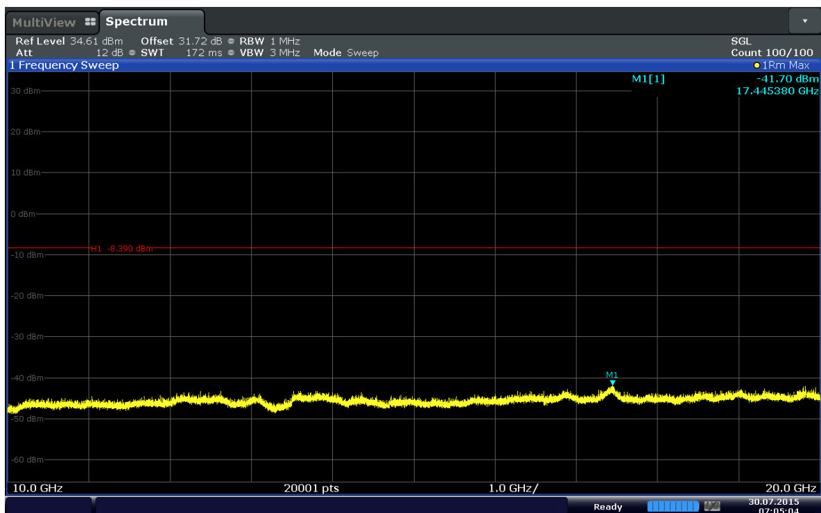
Plot 6-46. Conducted Spurious Plot (Band 4-3MHz-QPSK-RB Size 1-RB Offset 0-Ch.20175)
