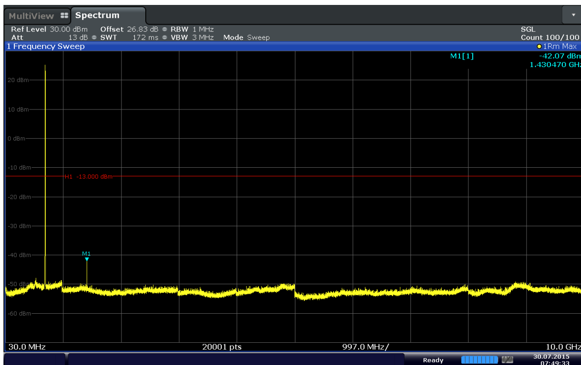
Plot 6-27. Conducted Spurious Plot (Band 12–1.4MHz–QPSK–RB Size 1–RB Offset 2–Ch.23173)
