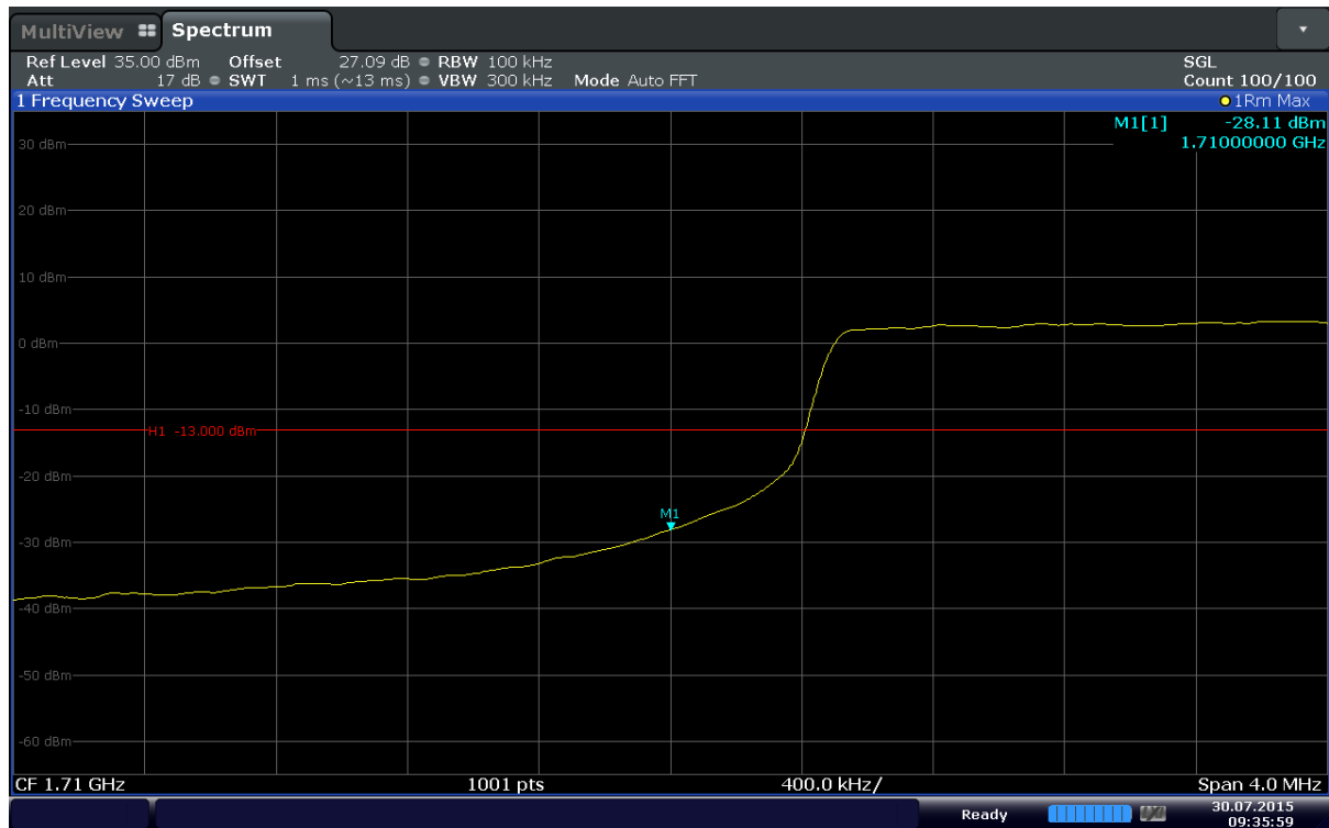
Plot 6-107. Lower Band Edge Plot (Band 4 – 10MHz – QPSK – RB Size 50)
