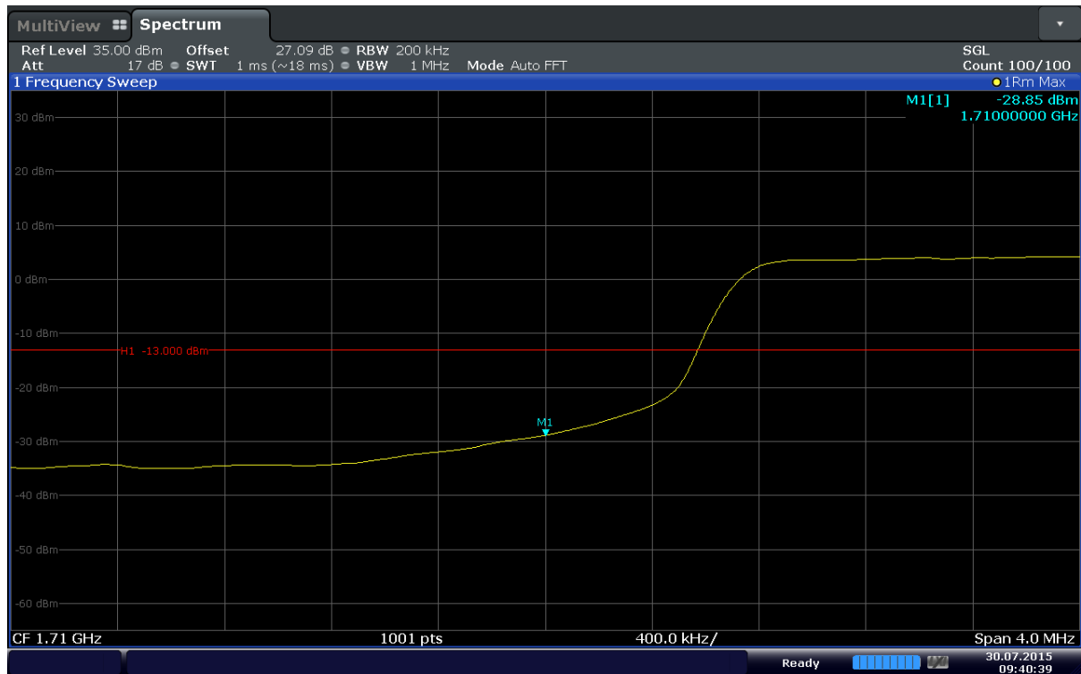
Plot 6-111. Lower Band Edge Plot (Band 4 – 15MHz – QPSK – RB Size 75)
