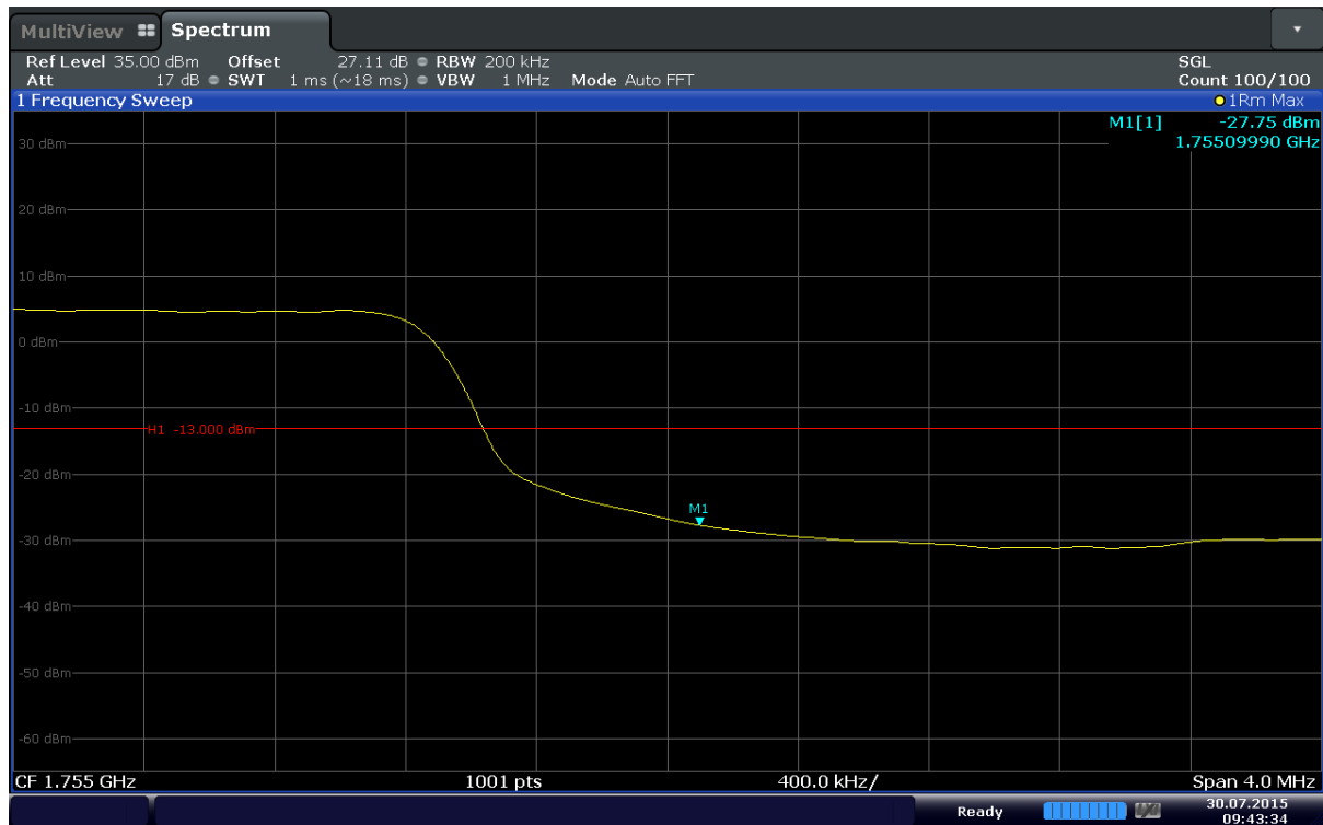
Plot 6-113. Upper Band Edge Plot (Band 4 – 15MHz – QPSK – RB Size 75)
