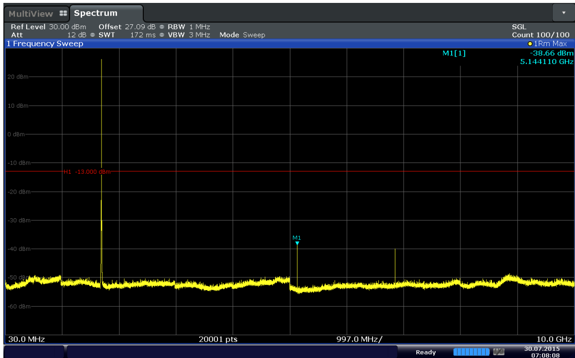
Plot 6-49. Conducted Spurious Plot (Band 4–5MHz–QPSK–RB Size 1–RB Offset 24–Ch.19975)
