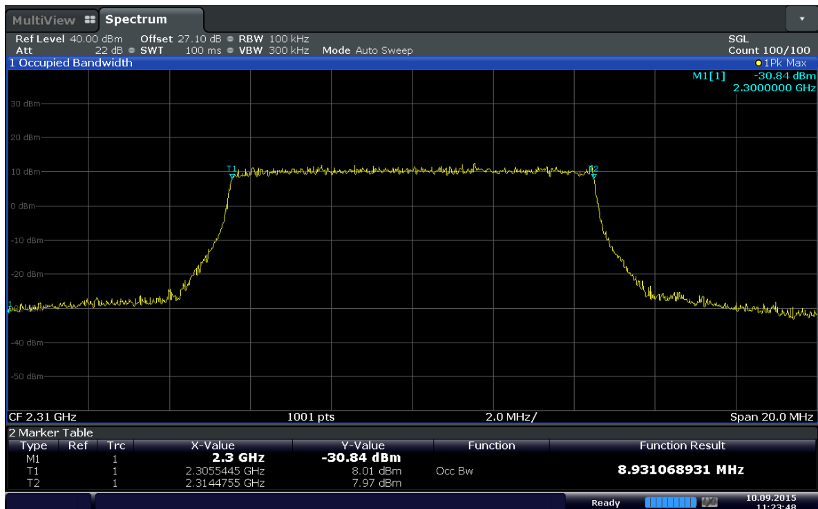
Plot 6-24. Occupied Bandwidth Plot (Band 30 – 10MHz 16QAM - RB Size 50)
