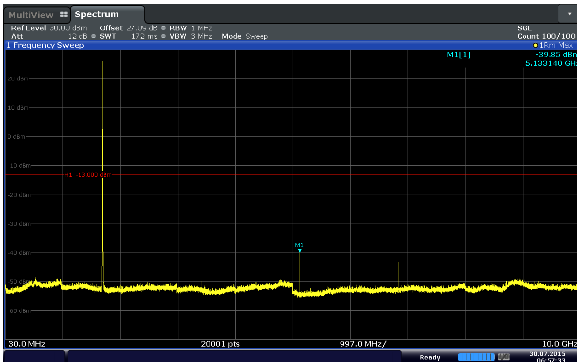
Plot 6-37. Conducted Spurious Plot (Band 4–1.4MHz–QPSK–RB Size 1–RB Offset 5–Ch.19957)
