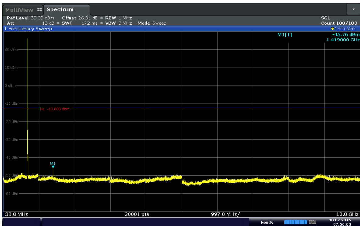
Plot 6-32. Conducted Spurious Plot (Band 12-5MHz-QPSK-RB Size 1-RB Offset 24-Ch.23095)
