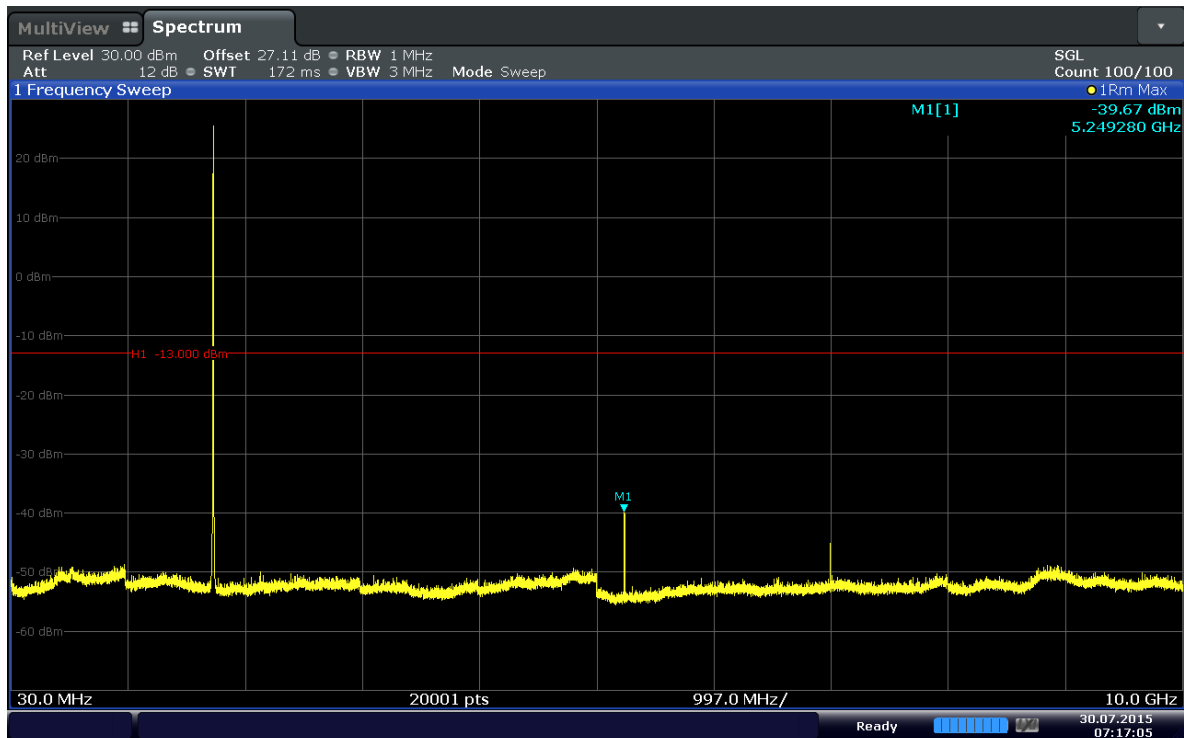
Plot 6-59. Conducted Spurious Plot (Band 4–10MHz–QPSK–RB Size 1–RB Offset 24–Ch.20350)
