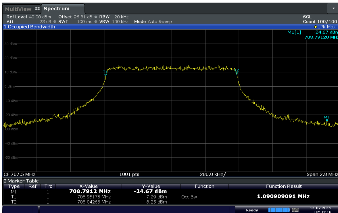
Plot 6-1. Occupied Bandwidth Plot (Band 12 – 1.4MHz QPSK - RB Size 6)
