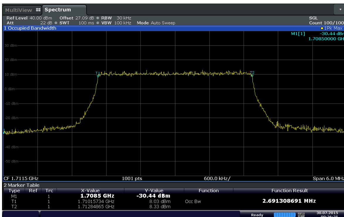
Plot 6-12. Occupied Bandwidth Plot (Band 4 – 3MHz 16QAM - RB Size 15)
