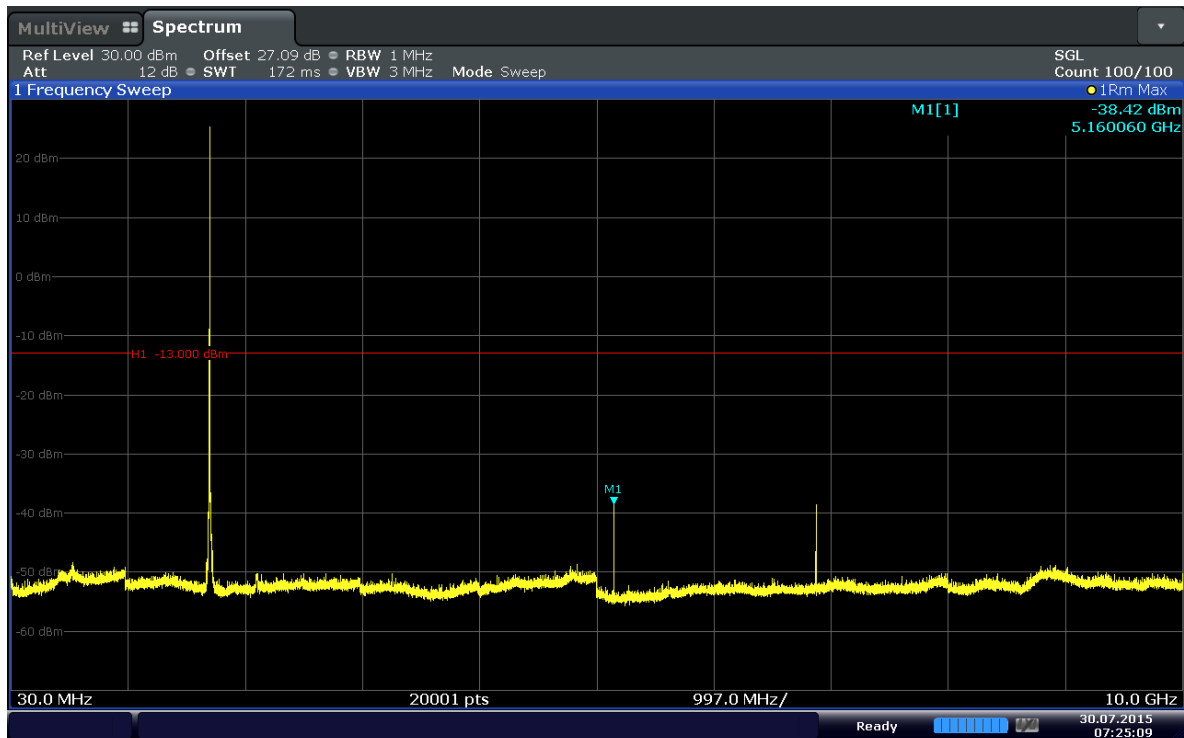
Plot 6-67. Conducted Spurious Plot (Band 4–20MHz–QPSK–RB Size 1–RB Offset 49–Ch.20050)
