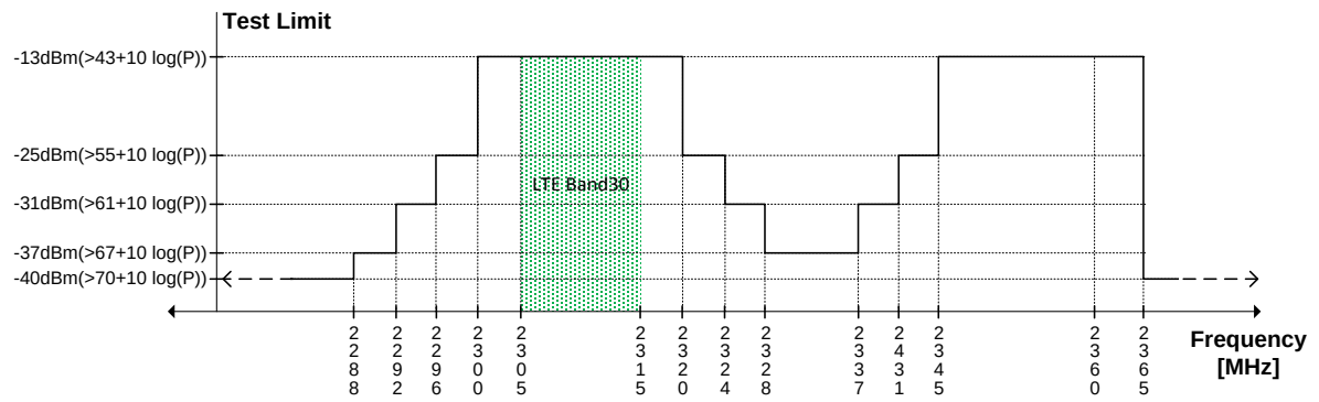
Figure 6-1. Emission limits (LTE Band 30)
