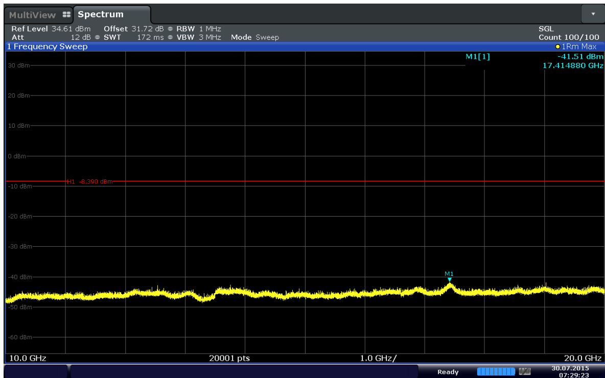
Plot 6-72. Conducted Spurious Plot (Band 4–20MHz–QPSK–RB Size 1–RB Offset 49–Ch.20300)
