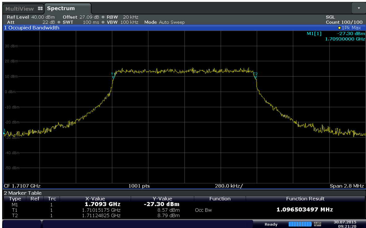
Plot 6-9. Occupied Bandwidth Plot (Band 4 – 1.4MHz QPSK - RB Size 6)
