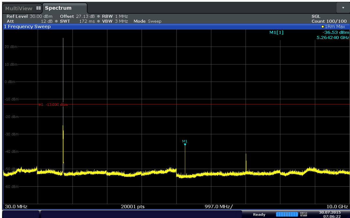
Plot 6-47. Conducted Spurious Plot (Band 4–3MHz–QPSK–RB Size 1–RB Offset 14–Ch.20385)
