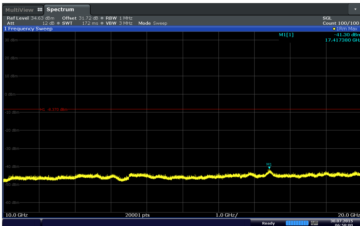
Plot 6-38. Conducted Spurious Plot (Band 4–1.4MHz–QPSK–RB Size 1–RB Offset 5–Ch.19957)
