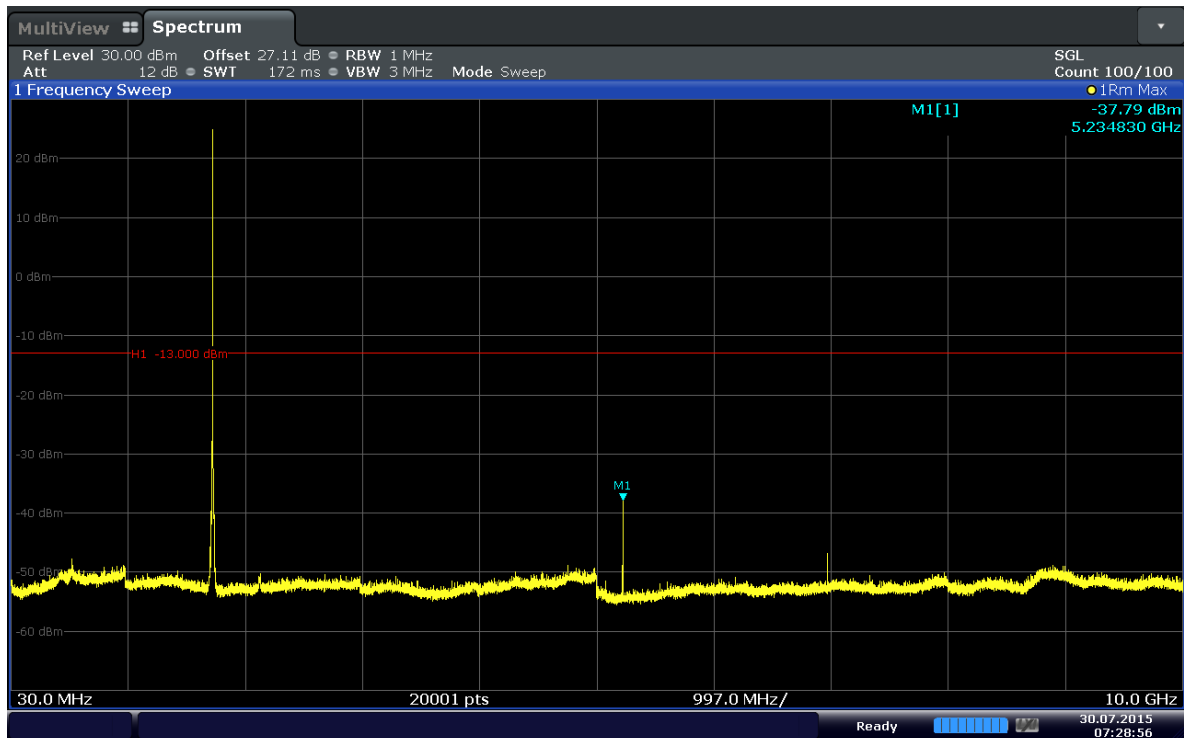
Plot 6-71. Conducted Spurious Plot (Band 4–20MHz–QPSK–RB Size 1–RB Offset 49–Ch.20300)
