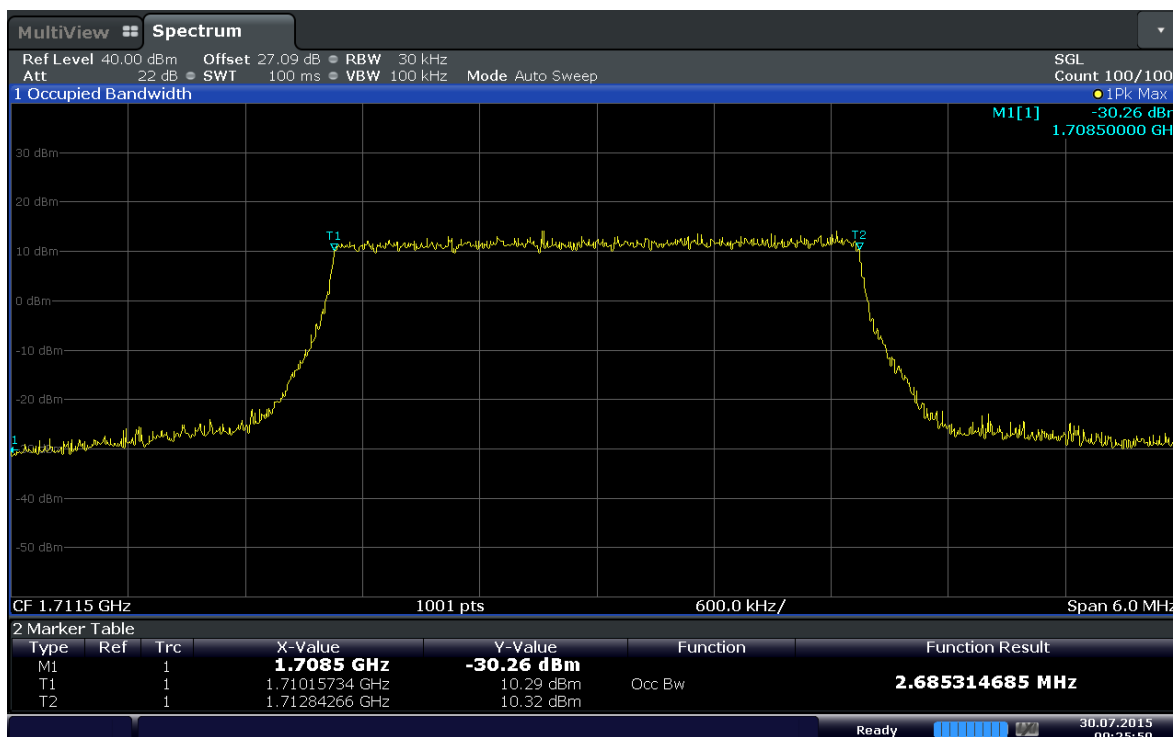
Plot 6-11. Occupied Bandwidth Plot (Band 4 – 3MHz QPSK - RB Size 15)
