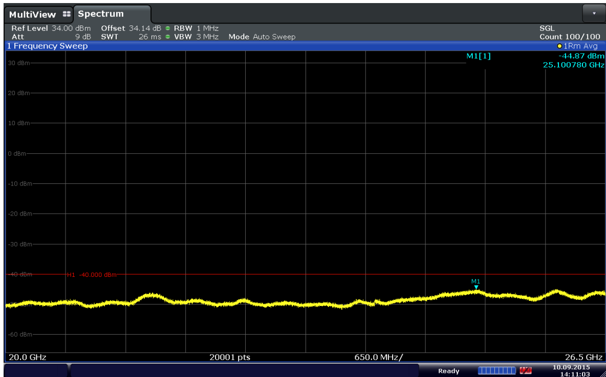
Plot 6-75. Conducted Spurious Plot (Band 30–5MHz–QPSK–RB Size 1–RB Offset 24– Ch.27685)
