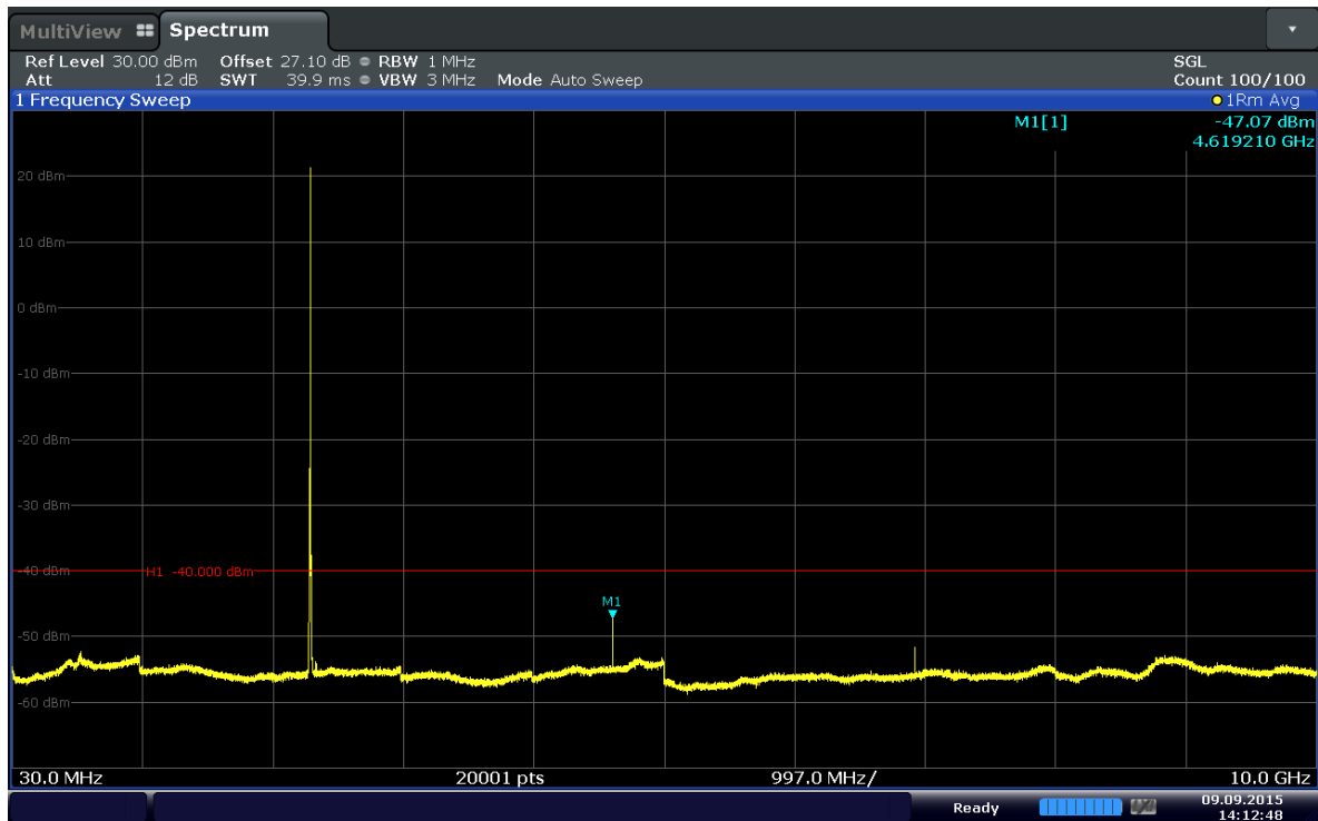
Plot 6-73. Conducted Spurious Plot (Band 30–5MHz–QPSK–RB Size 1–RB Offset 24– Ch.27685)
