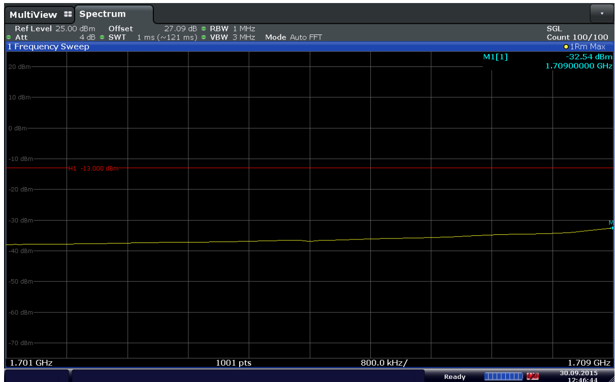
Plot 6-116. Extended Lower Band Edge Plot (Band 4 – 20MHz – QPSK – RB Size 100)
