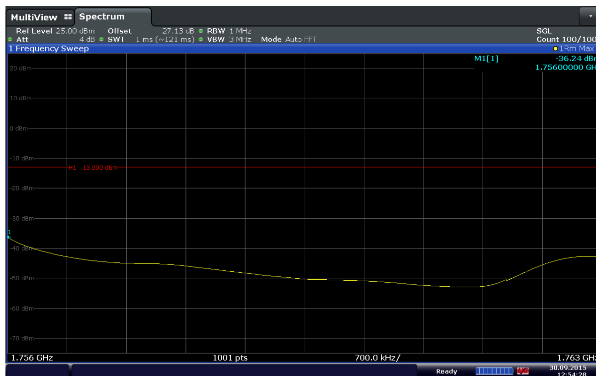
Plot 6-121. Upper Band Edge Plot (Band 4 – 20MHz – QPSK – RB Size 1 – RB Offset 99)
