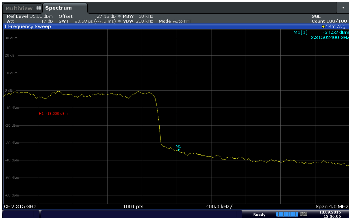
Plot 6-125. Upper Band Edge Plot (Band 30 – 5MHz – QPSK – RB Size 25)
