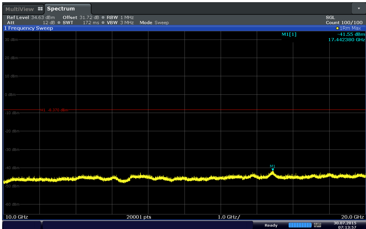
Plot 6-56. Conducted Spurious Plot (Band 4–10MHz–QPSK–RB Size 1–RB Offset 24–Ch.20000)
