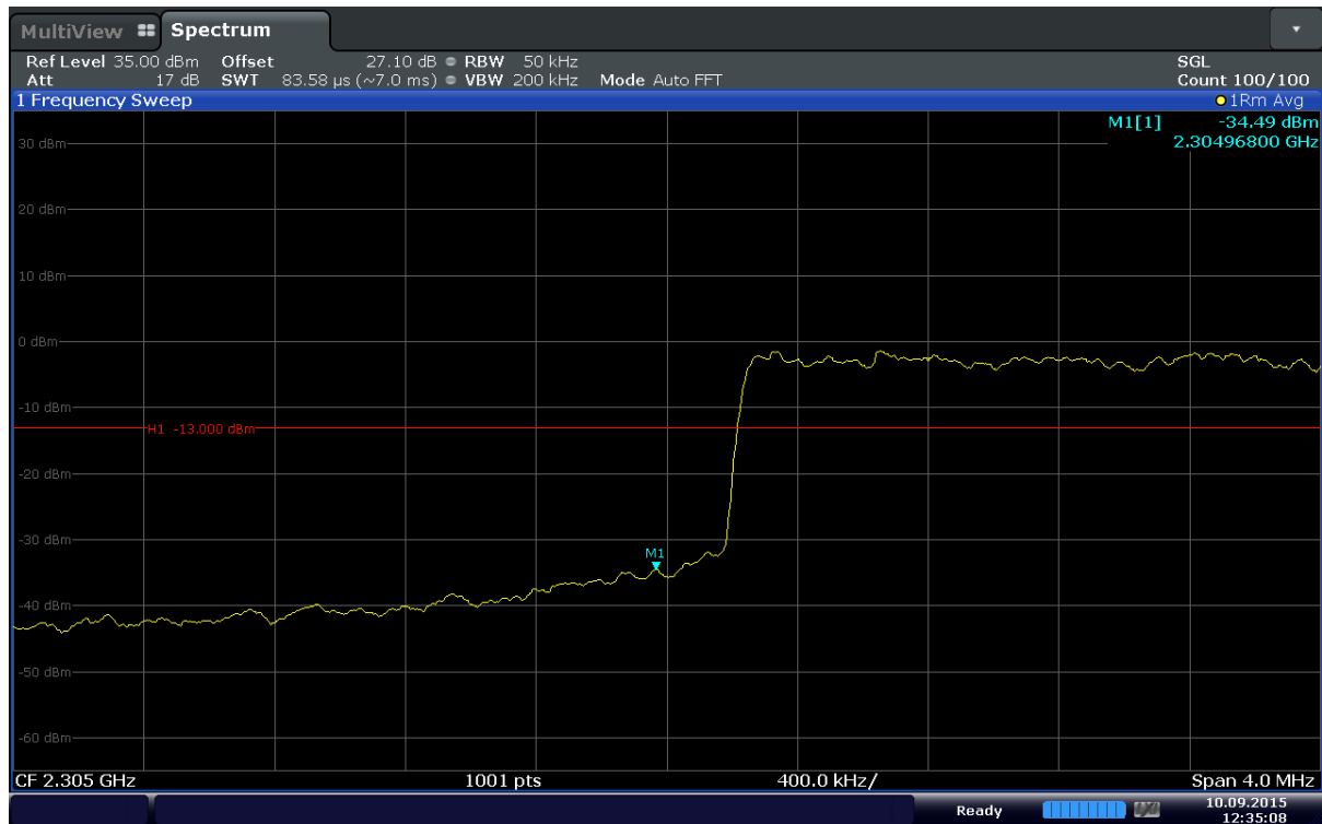
Plot 6-123. Lower Band Edge Plot (Band 30 – 5MHz – QPSK – RB Size 25)
