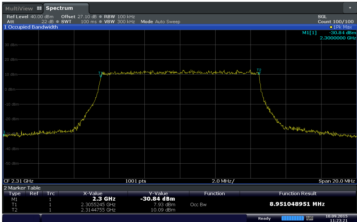
Plot 6-23. Occupied Bandwidth Plot (Band 30 – 10MHz QPSK - RB Size 50)
