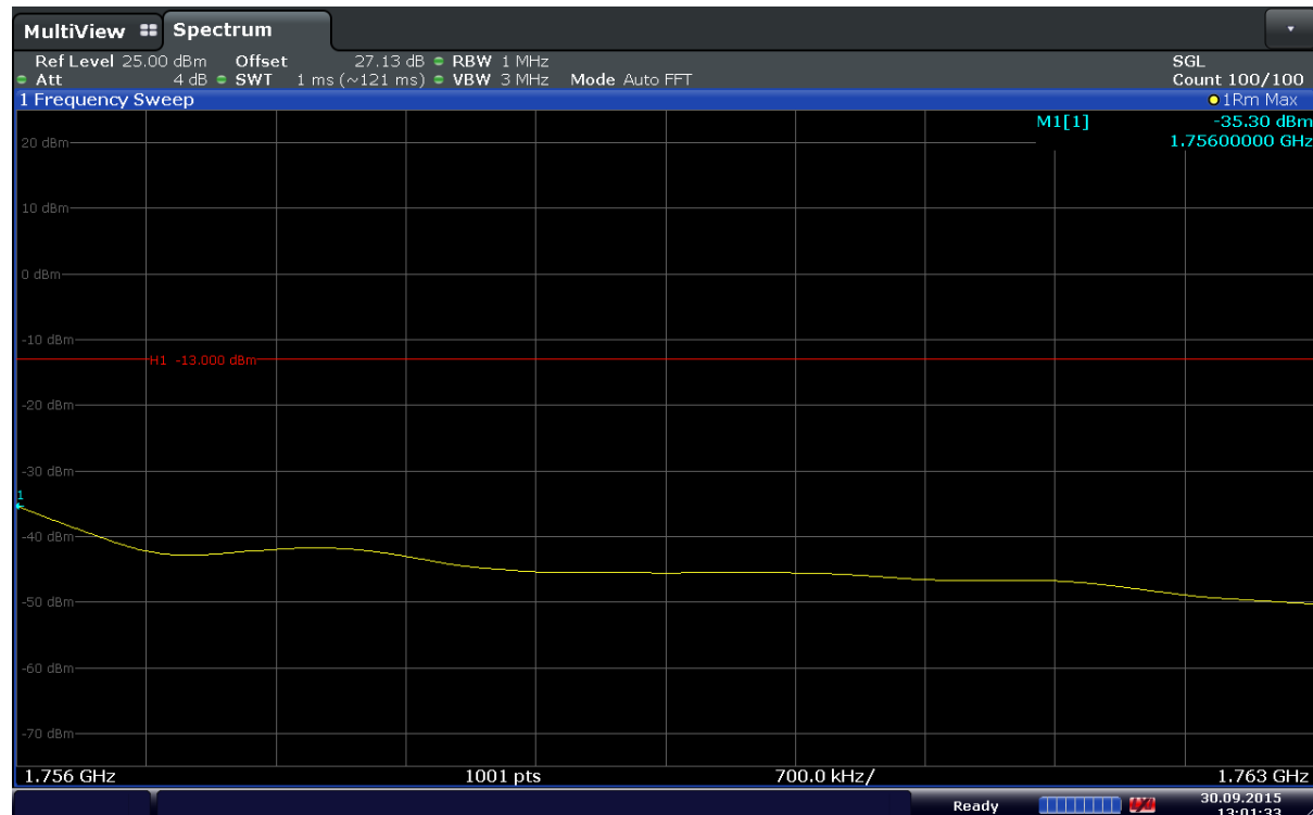
Plot 6-98. Extended Upper Band Edge Plot (Band 4 – 1.4MHz – QPSK – RB Size 6)
