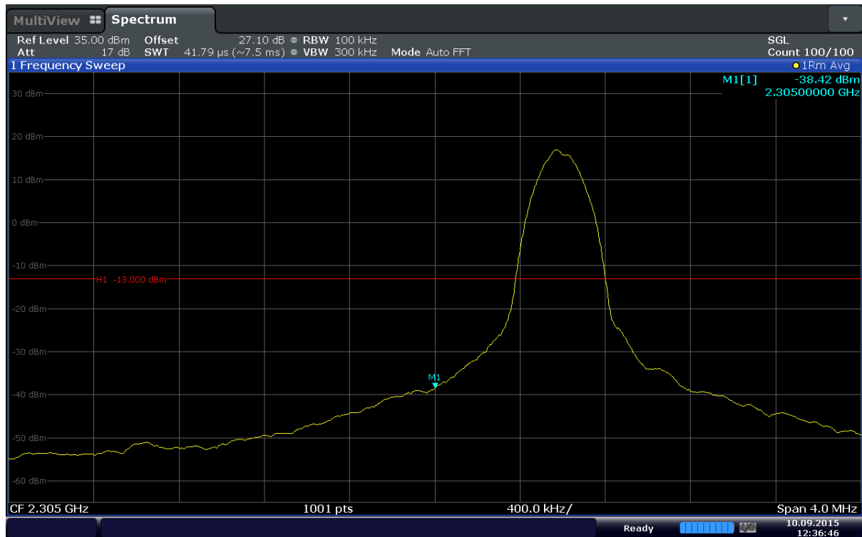
Plot 6-131. Lower Band Edge Plot (Band 30 – 10MHz – QPSK – RB Size1 – RB Offset 0)
