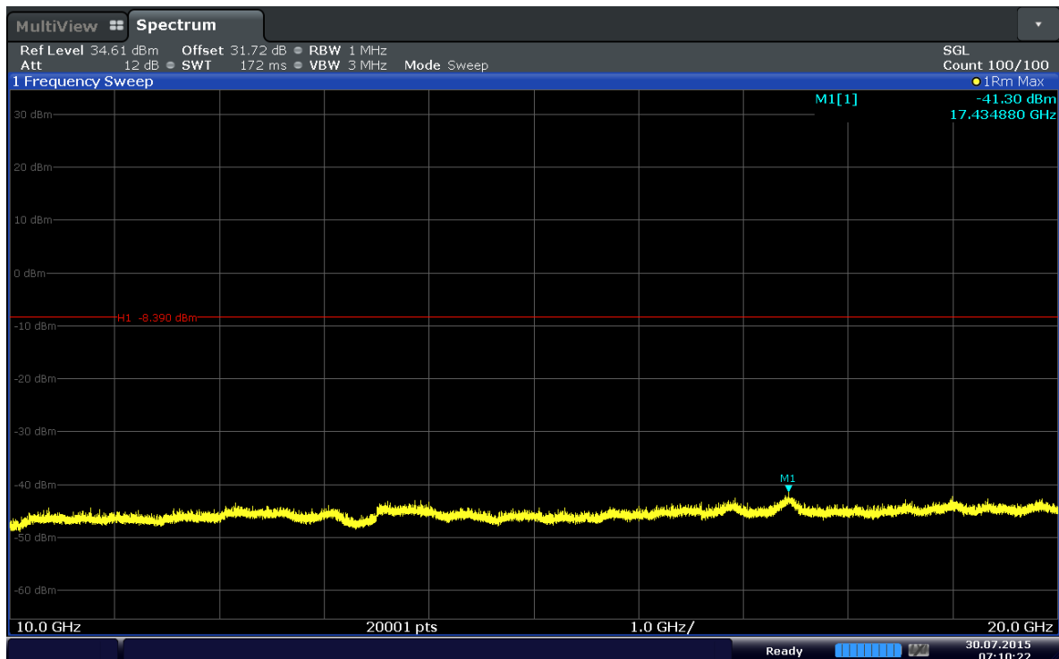
Plot 6-52. Conducted Spurious Plot (Band 4–5MHz–QPSK–RB Size 1–RB Offset 24–Ch.20175)
