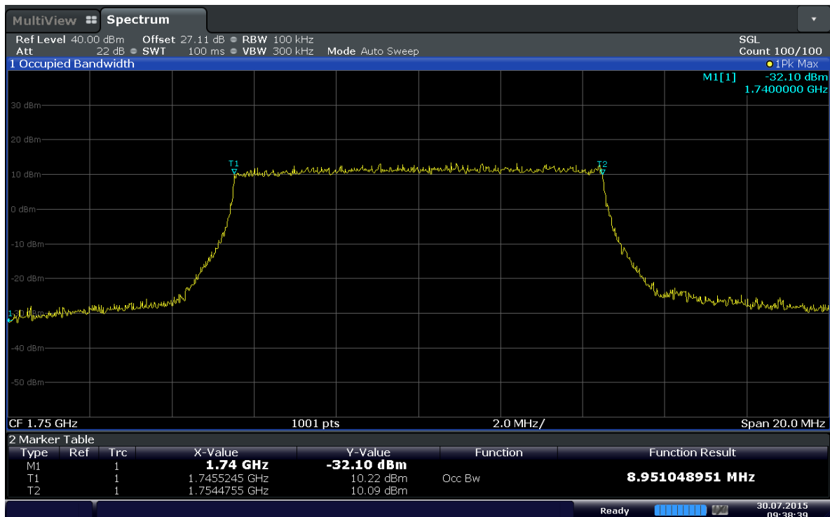
Plot 6-16. Occupied Bandwidth Plot (Band 4 – 10MHz 16QAM - RB Size 50)
