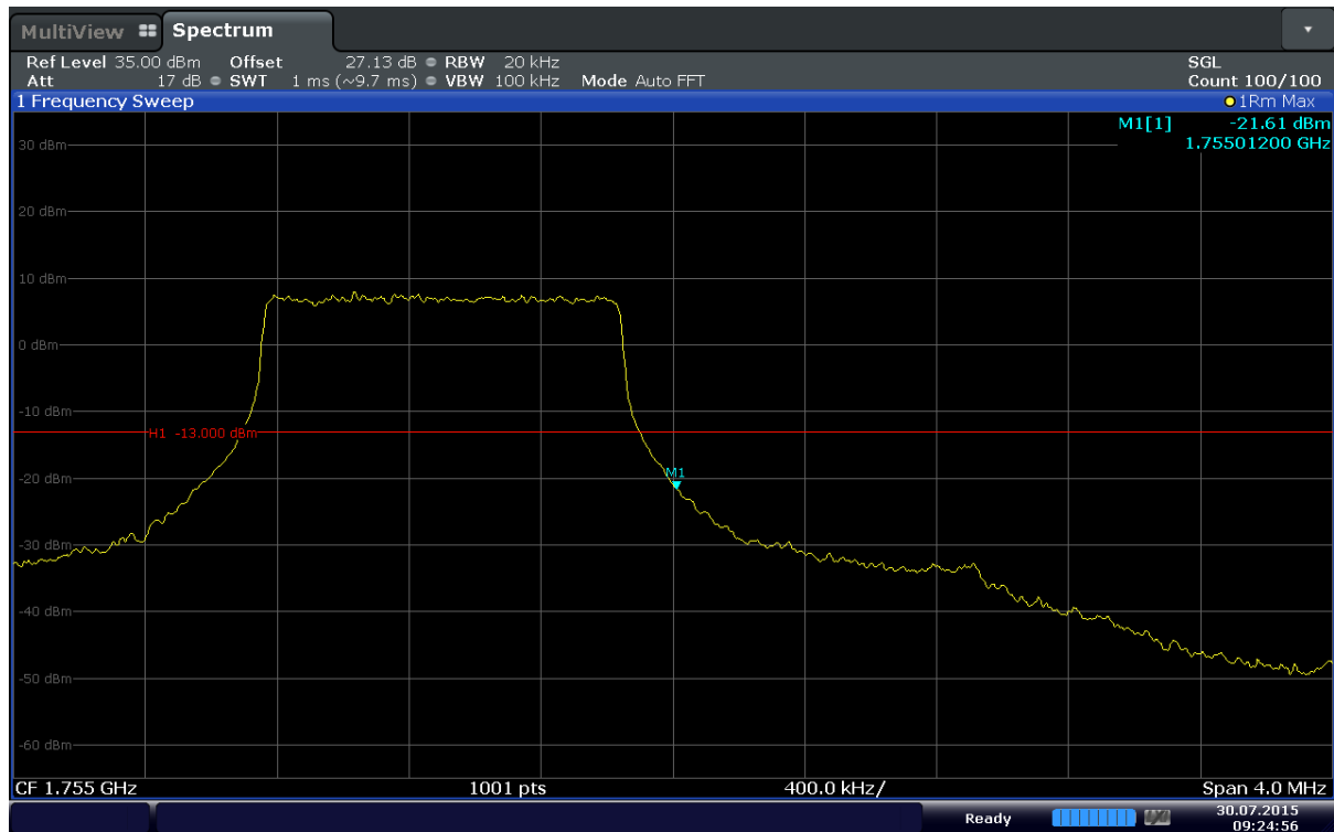
Plot 6-97. Upper Band Edge Plot (Band 4 – 1.4MHz – QPSK – RB Size 6)
