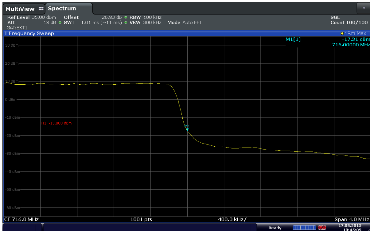
Plot 6-88. Upper Band Edge Plot (Band 12 – 3MHz – QPSK – RB Size 15)
