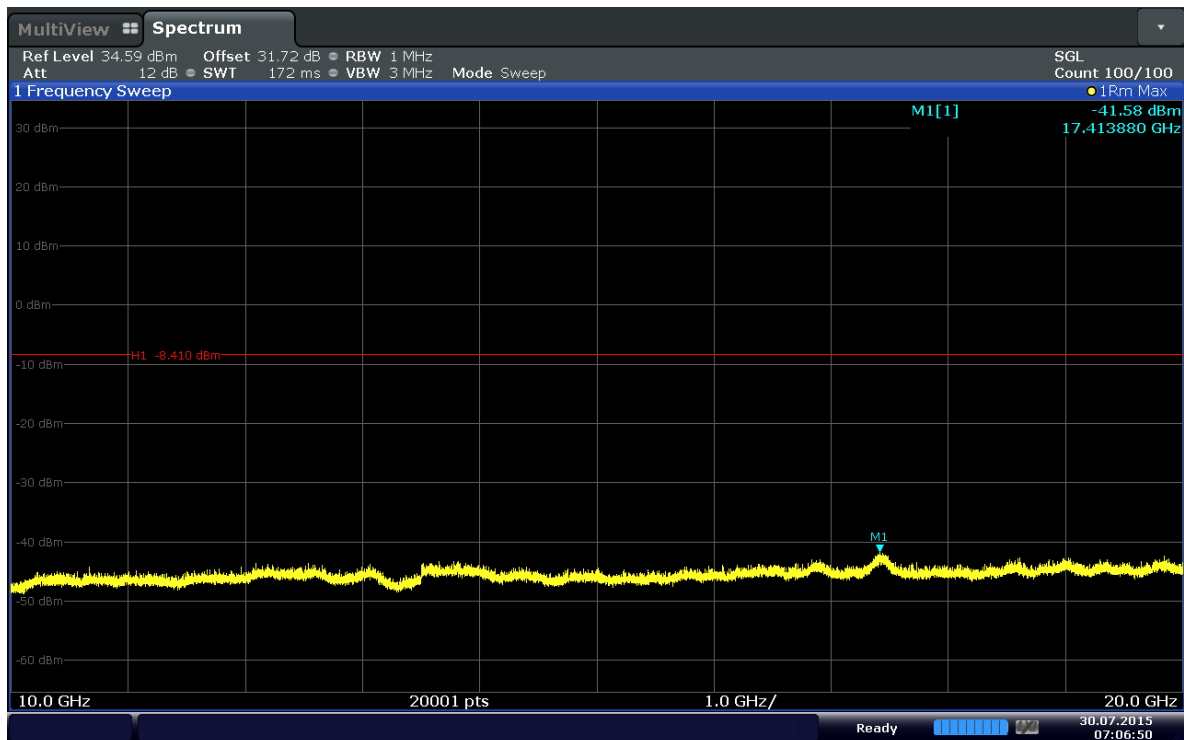
Plot 6-48. Conducted Spurious Plot (Band 4–3MHz–QPSK–RB Size 1–RB Offset 14–Ch.20385)
