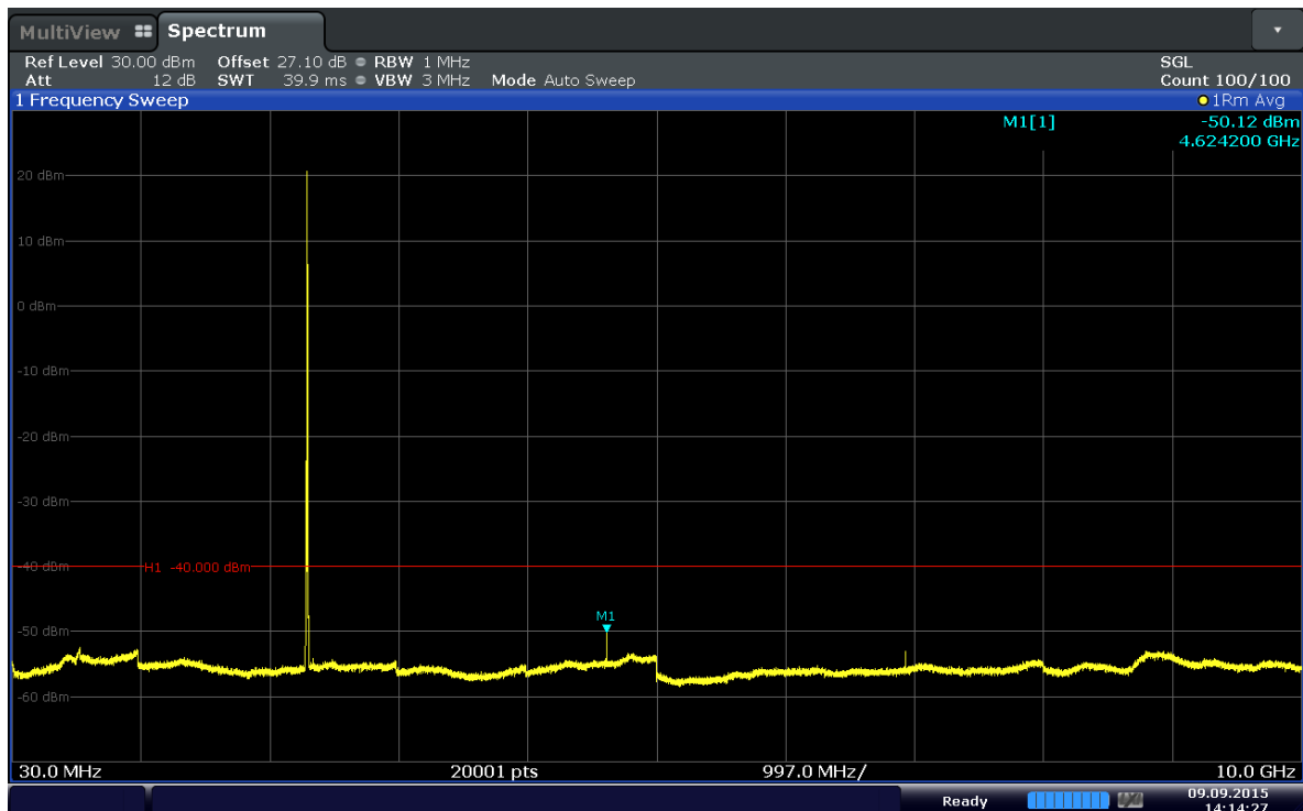
Plot 6-76. Conducted Spurious Plot (Band 30–5MHz–QPSK–RB Size 1–RB Offset 24– Ch.27710)
