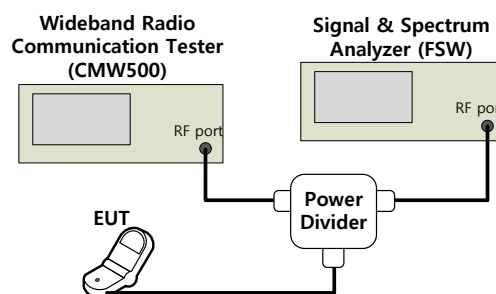
Figure 6-2. Test Instruments & Measurement Setup
