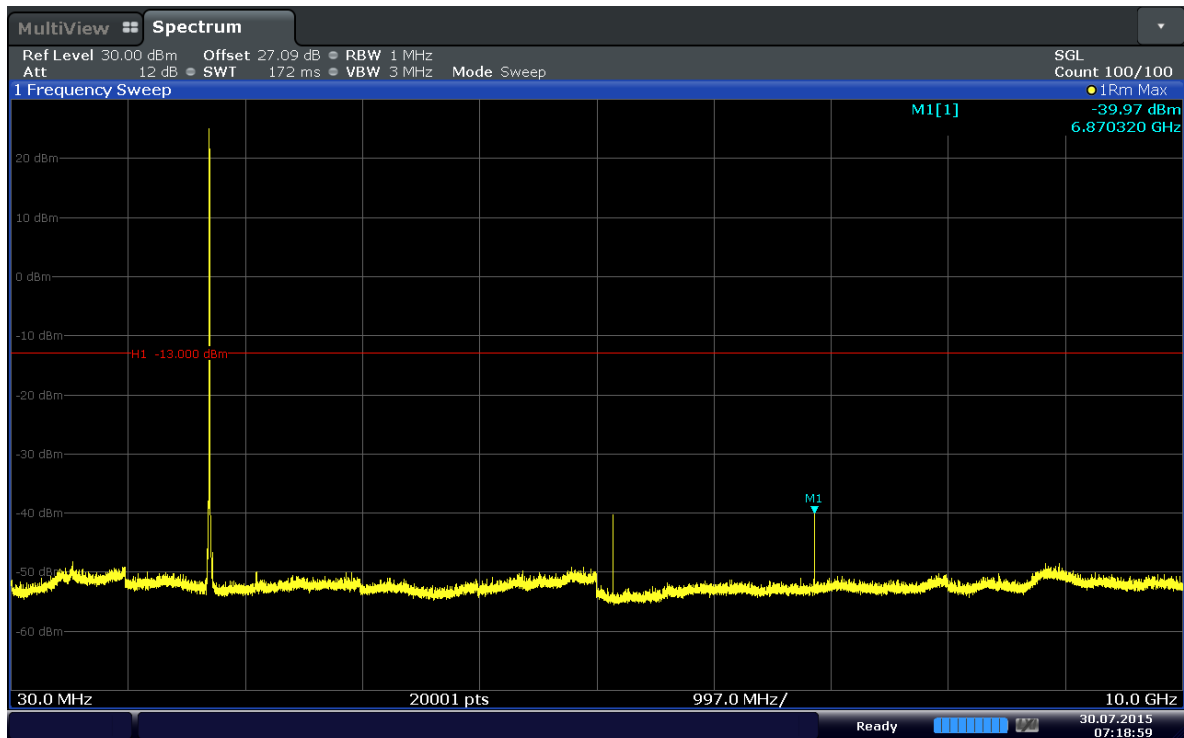
Plot 6-61. Conducted Spurious Plot (Band 4–15MHz–QPSK–RB Size 1–RB Offset 37–Ch.20025)
