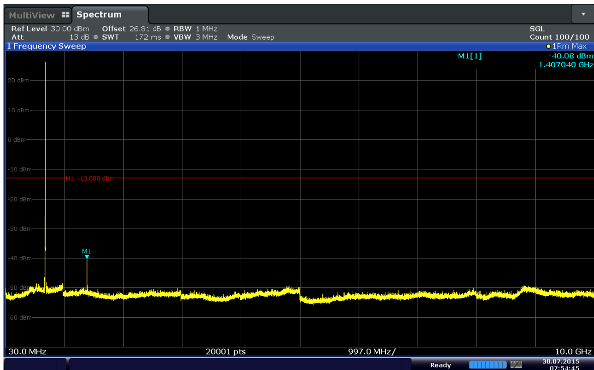
Plot 6-31. Conducted Spurious Plot (Band 12-5MHz-QPSK-RB Size 1-RB Offset 24-Ch.23035)
