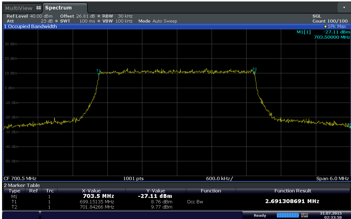
Plot 6-4. Occupied Bandwidth Plot (Band 12 – 3MHz 16QAM - RB Size 15)
