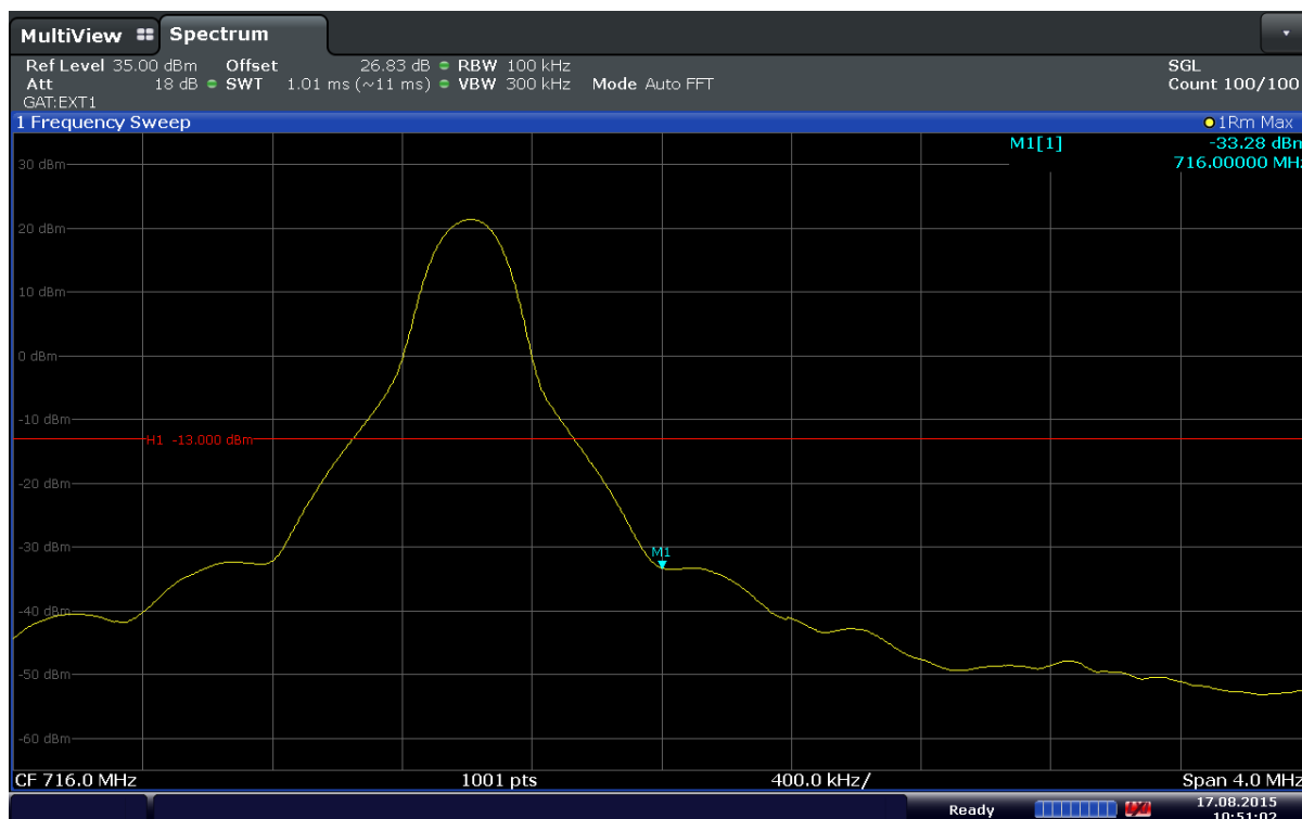
Plot 6-94. Upper Band Edge Plot (Band 12 – 10MHz – QPSK – RB Size 1 – RB Offset 49)
