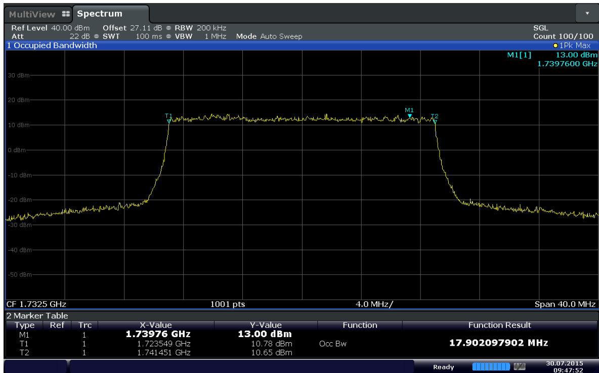
Plot 6-19. Occupied Bandwidth Plot (Band 4 - 20MHz QPSK - RB Size 100)
