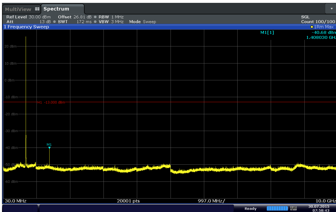
Plot 6-34. Conducted Spurious Plot (Band 12–10MHz–QPSK–RB Size 1–RB Offset 24–Ch.23060)
