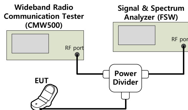
Figure 6-5. Test Instruments & Measurement Setup
