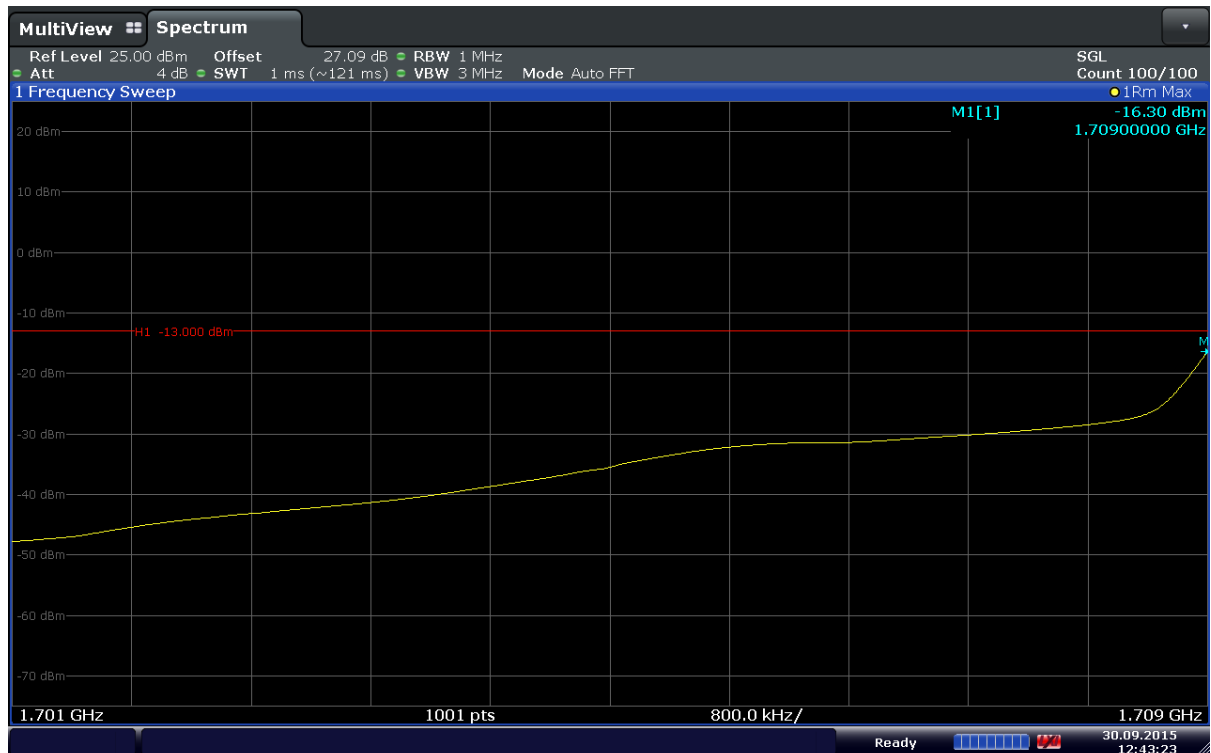
Plot 6-104. Extended Lower Band Edge Plot (Band 4 – 5MHz – QPSK – RB Size 25)
