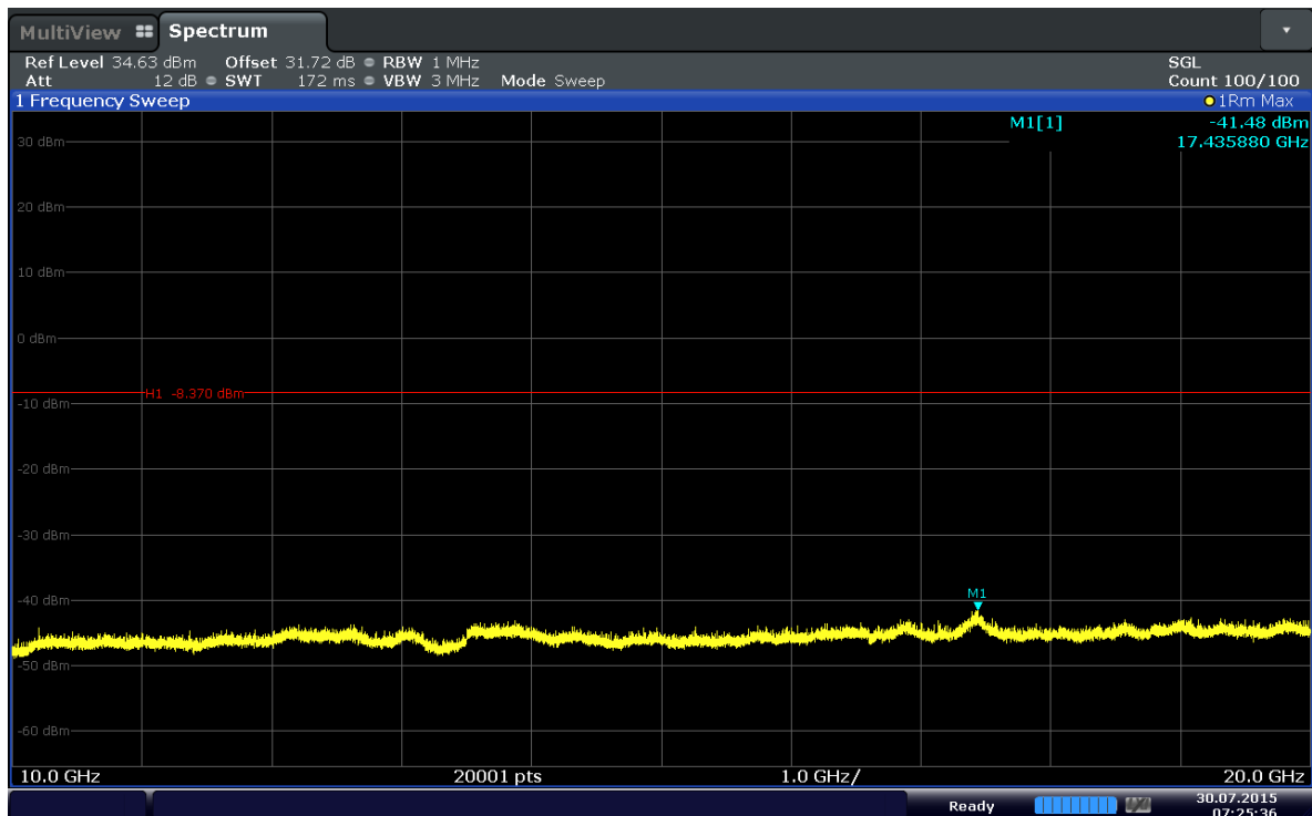
Plot 6-68. Conducted Spurious Plot (Band 4–20MHz–QPSK–RB Size 1–RB Offset 49–Ch.20050)
