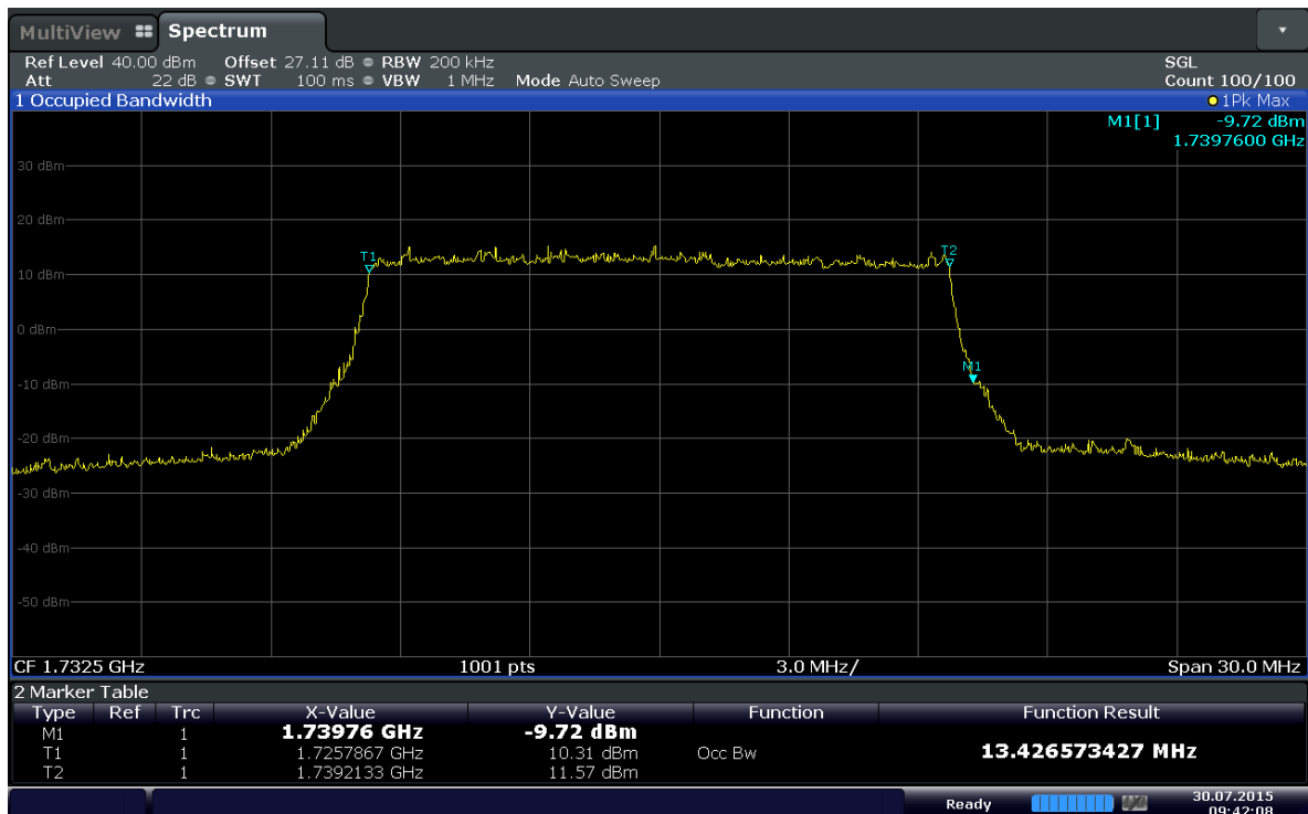
Plot 6-18. Occupied Bandwidth Plot (Band 4 - 15MHz 16QAM - RB Size 75)
