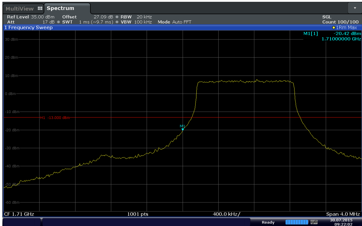
Plot 6-95. Lower Band Edge Plot (Band 4 – 1.4MHz – QPSK – RB Size 6)
