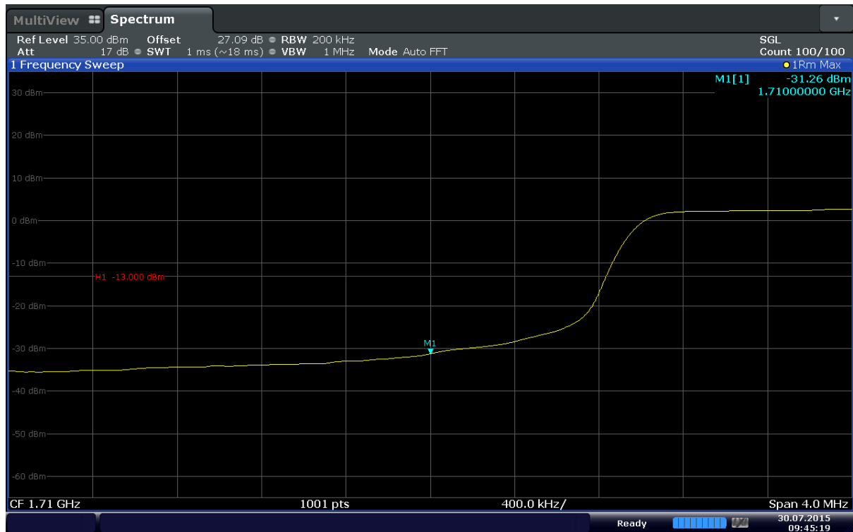
Plot 6-115. Lower Band Edge Plot (Band 4 – 20MHz – QPSK – RB Size 100)
