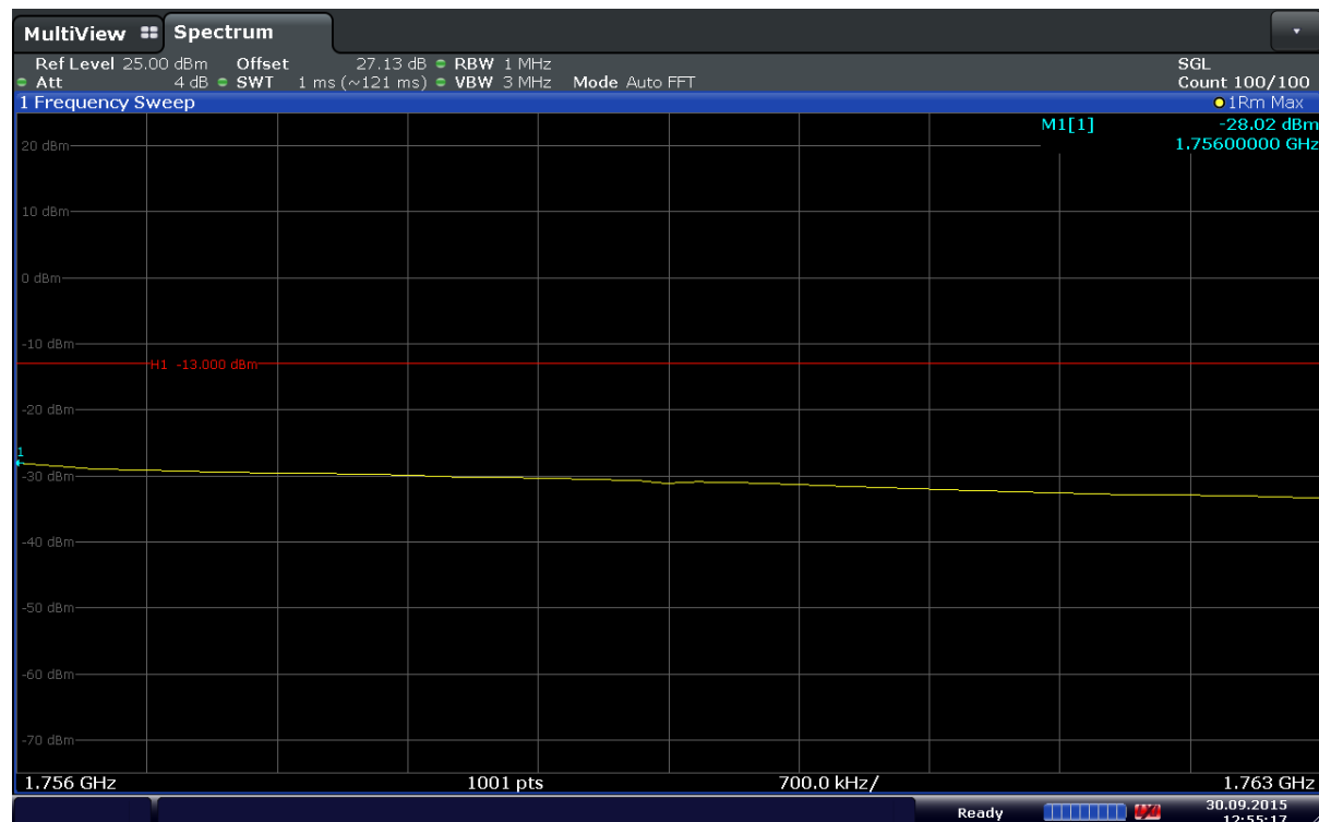
Plot 6-118. Extended Upper Band Edge Plot (Band 4 – 20MHz – QPSK – RB Size 100)
