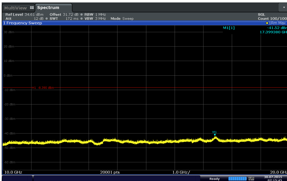
Plot 6-58. Conducted Spurious Plot (Band 4–10MHz–QPSK–RB Size 1–RB Offset 24–Ch.20175)
