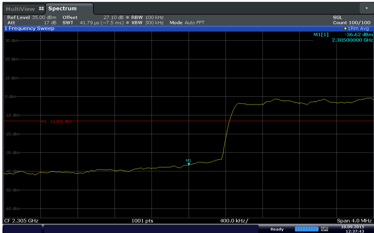
Plot 6-127. Lower Band Edge Plot (Band 30 – 10MHz – QPSK – RB Size 50)
