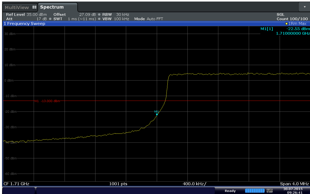
Plot 6-99. Lower Band Edge Plot (Band 4 – 3MHz – QPSK – RB Size 15)
