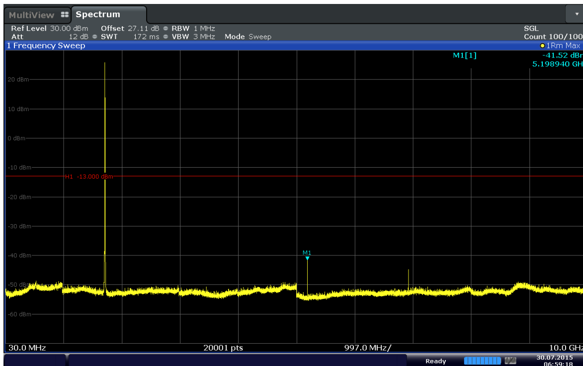
Plot 6-39. Conducted Spurious Plot (Band 4–1.4MHz–QPSK–RB Size 1–RB Offset 5–Ch.20175)
