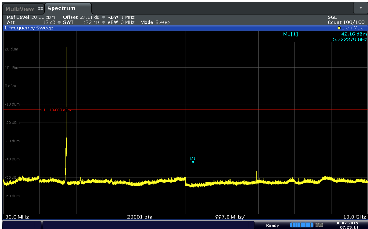
Plot 6-65. Conducted Spurious Plot (Band 4–15MHz–QPSK–RB Size 1–RB Offset 0–Ch.20325)
