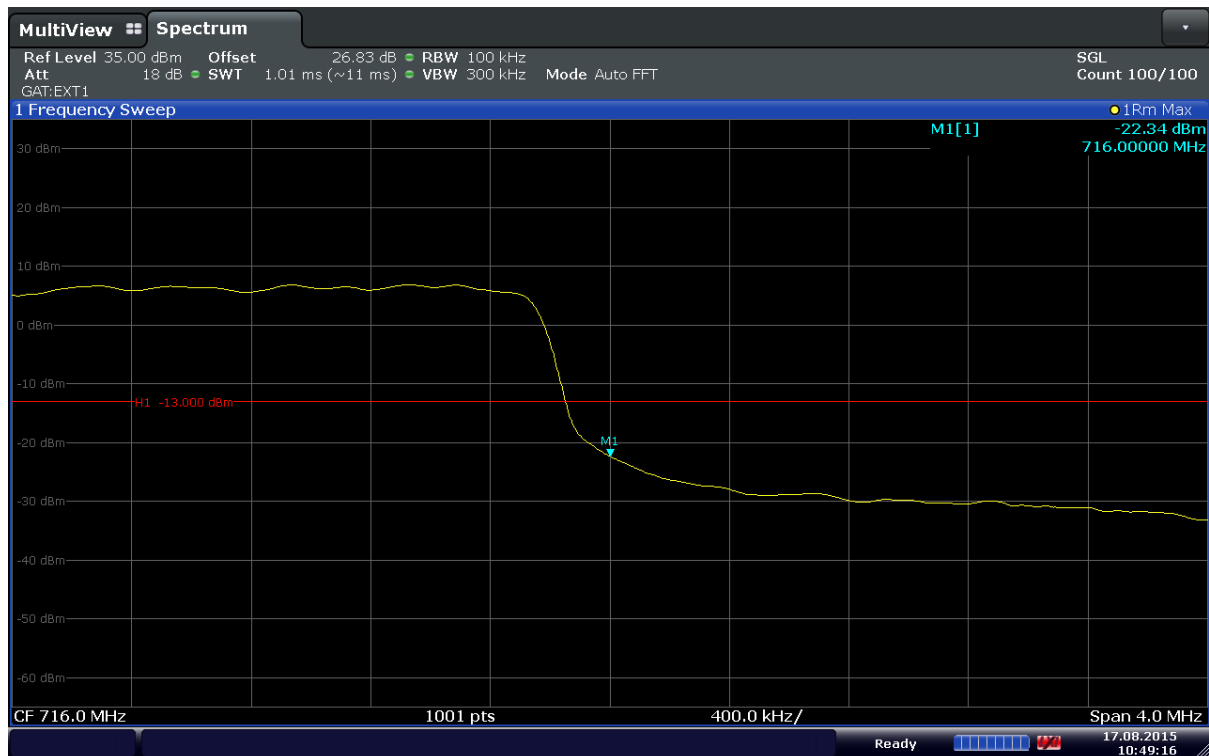
Plot 6-90. Upper Band Edge Plot (Band 12 – 5MHz – QPSK – RB Size 25)
