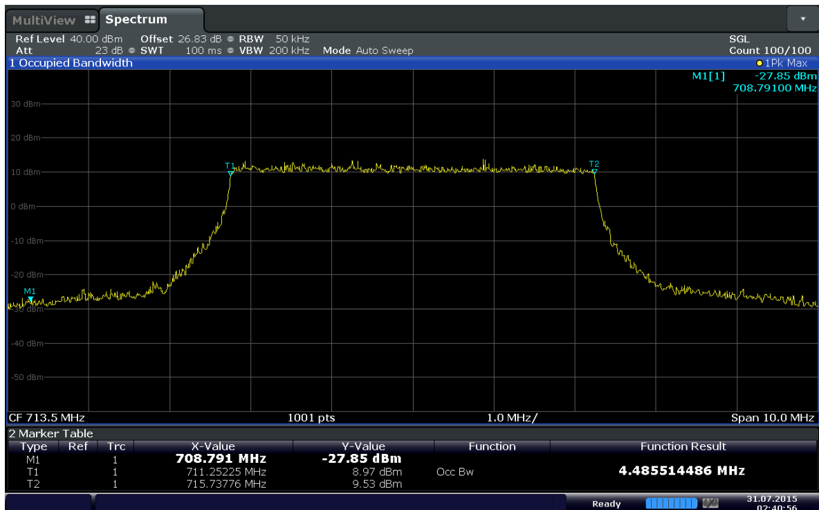
Plot 6-6. Occupied Bandwidth Plot (Band 12 – 5MHz 16QAM - RB Size 25)
