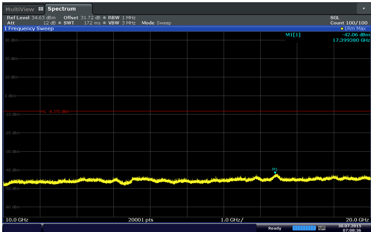
Plot 6-50. Conducted Spurious Plot (Band 4–5MHz–QPSK–RB Size 1–RB Offset 24–Ch.19975)
