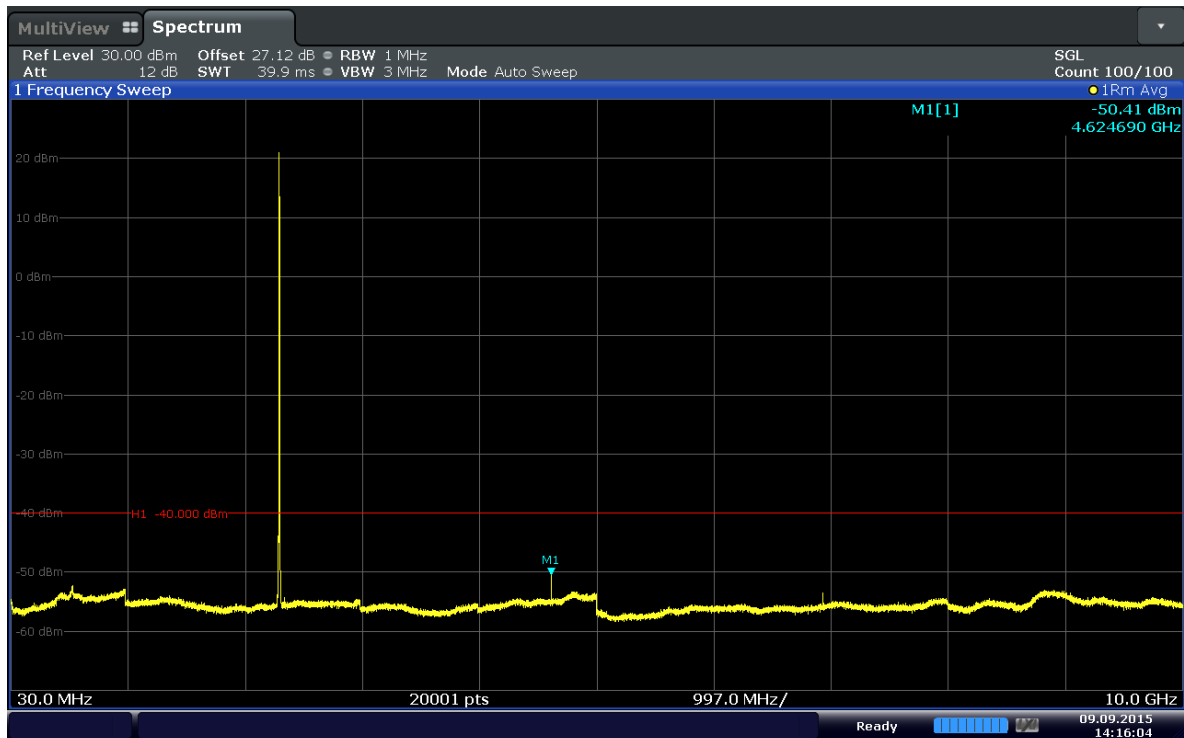
Plot 6-79. Conducted Spurious Plot (Band 30–5MHz–QPSK–RB Size 1–RB Offset 12– Ch.27735)
