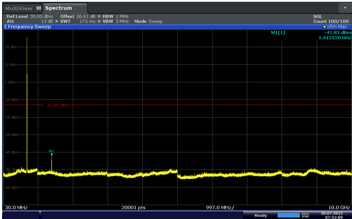
Plot 6-29. Conducted Spurious Plot (Band 12-3MHz-QPSK-RB Size 1-RB Offset 0-Ch.23095)
