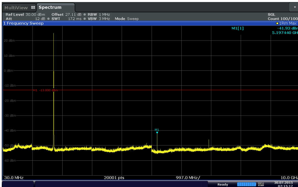
Plot 6-57. Conducted Spurious Plot (Band 4–10MHz–QPSK–RB Size 1–RB Offset 24–Ch.20175)
