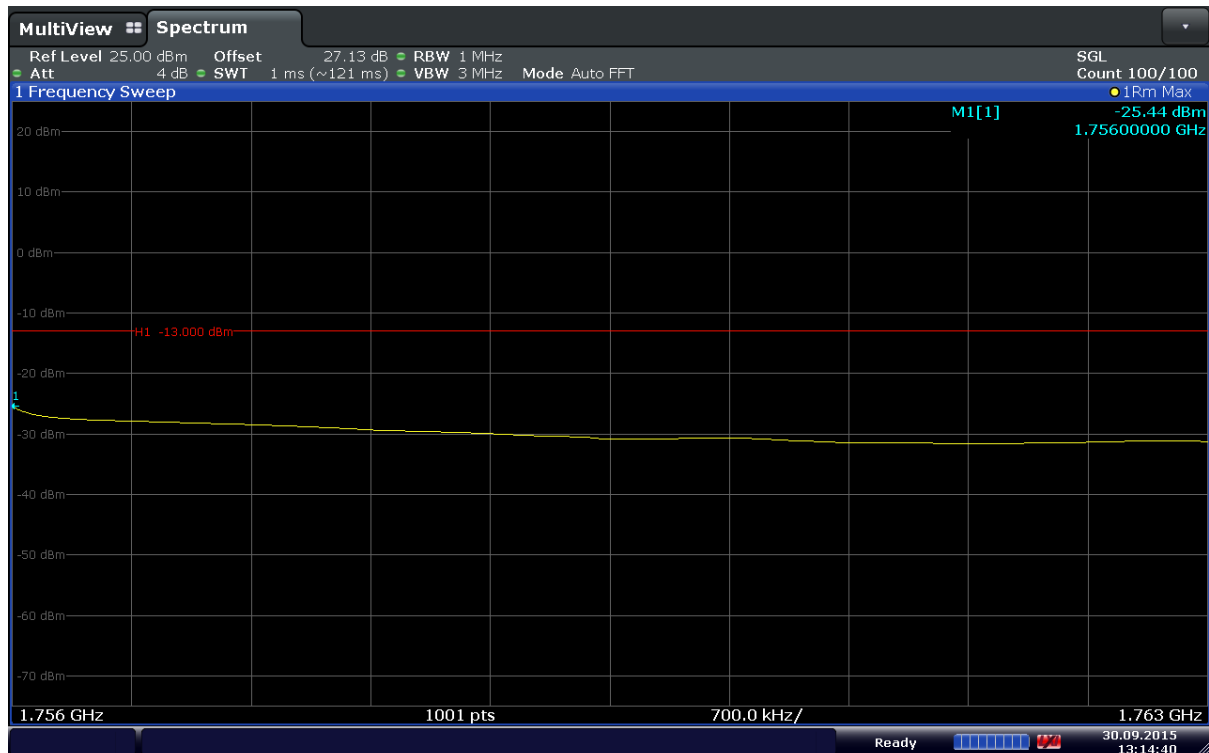
Plot 6-110. Extended Upper Band Edge Plot (Band 4 – 10MHz – QPSK – RB Size 50)
