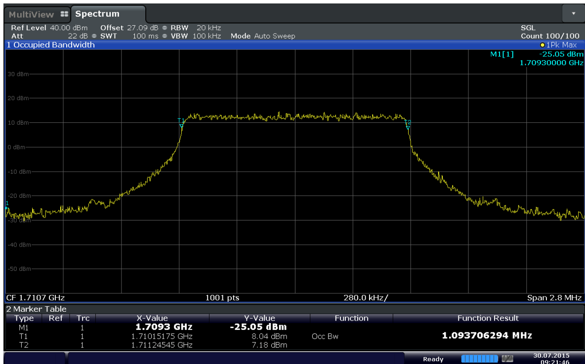
Plot 6-10. Occupied Bandwidth Plot (Band 4 – 1.4MHz 16QAM - RB Size 6)
