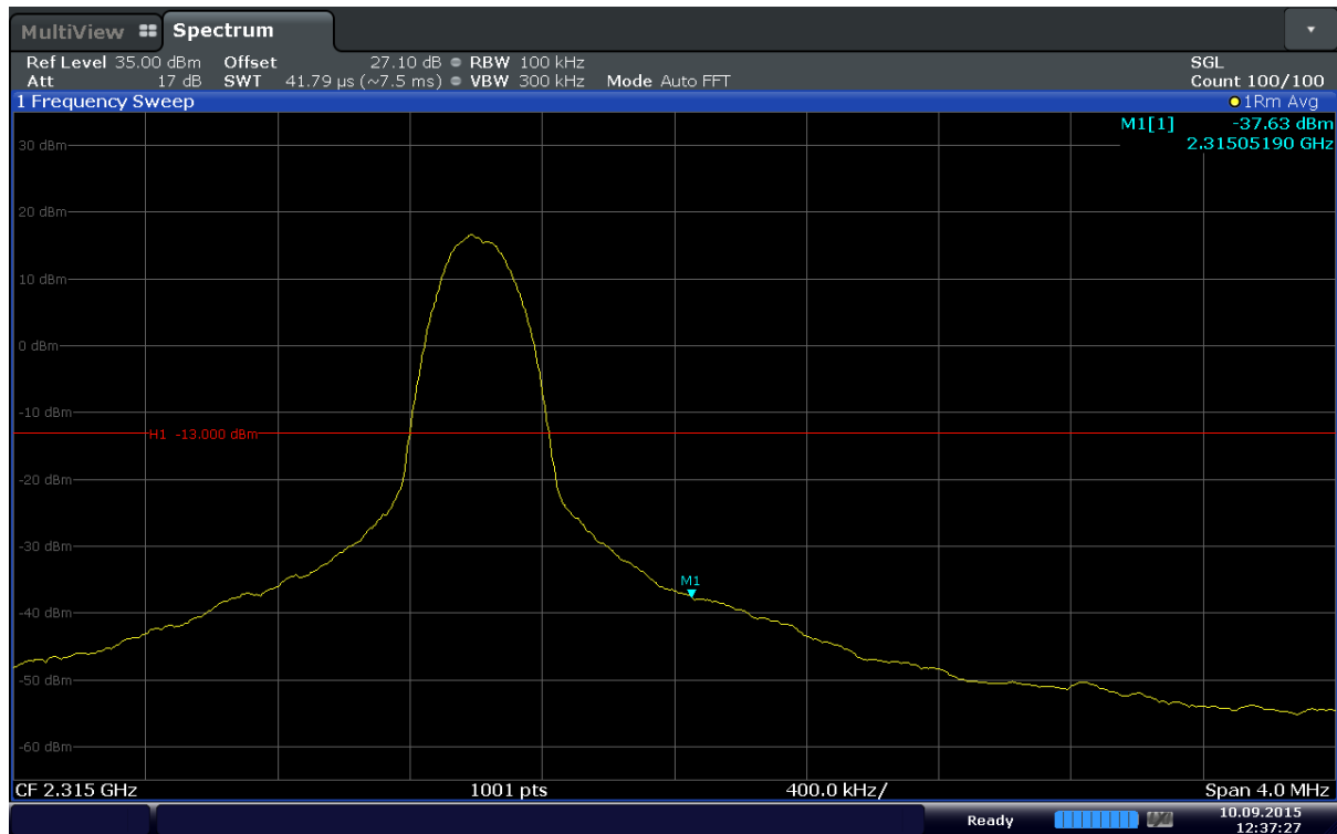
Plot 6-133. Upper Band Edge Plot (Band 30 – 10MHz – QPSK – RB Size 1 – RB Offset 49)
