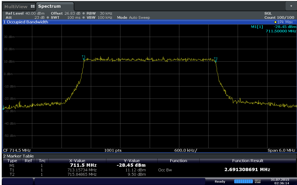
Plot 6-3. Occupied Bandwidth Plot (Band 12 – 3MHz QPSK - RB Size 15)
