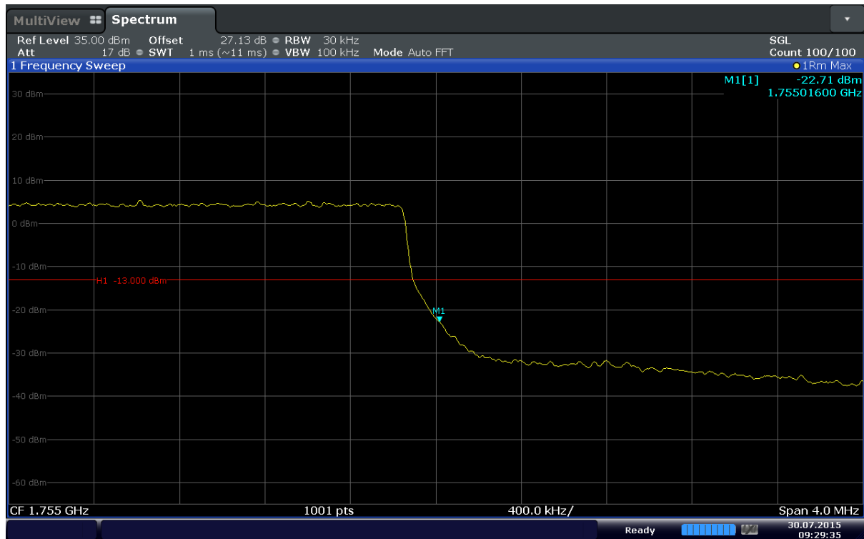
Plot 6-101. Upper Band Edge Plot (Band 4 – 3MHz – QPSK – RB Size 15)
