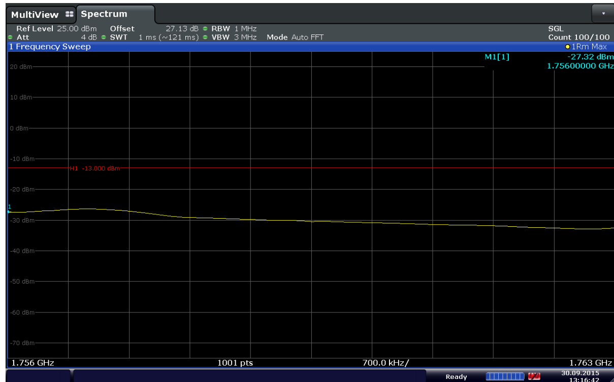
Plot 6-114. Extended Upper Band Edge Plot (Band 4 – 15MHz – QPSK – RB Size 75)
