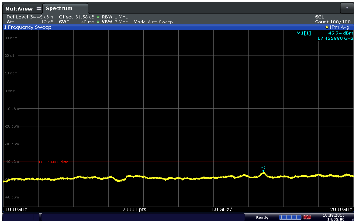
Plot 6-74. Conducted Spurious Plot (Band 30–5MHz–QPSK–RB Size 1–RB Offset 24– Ch.27685)
