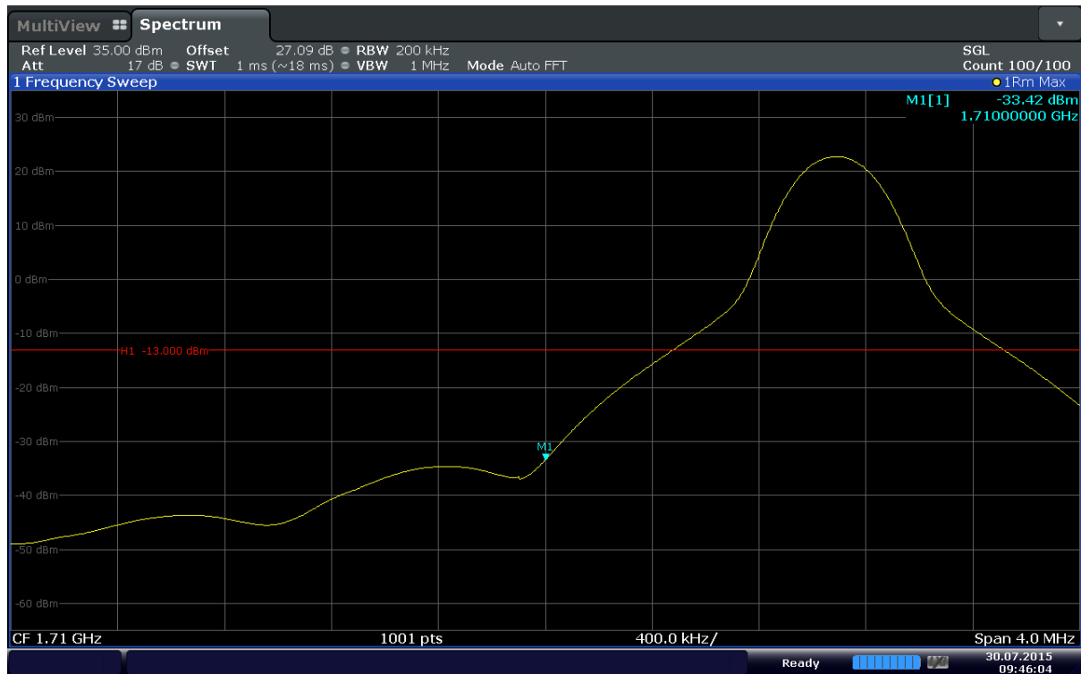
Plot 6-119. Lower Band Edge Plot (Band 4 – 20MHz – QPSK – RB Size 1 – RB Offset 0)
