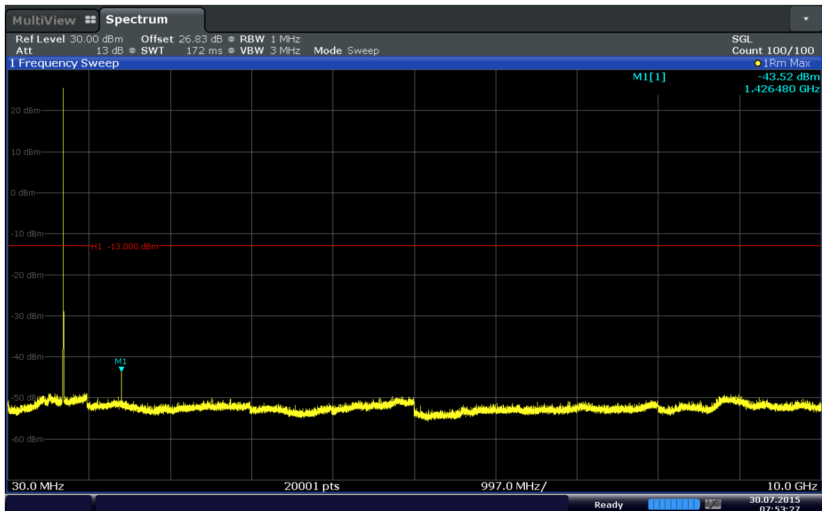
Plot 6-30. Conducted Spurious Plot (Band 12-3MHz-QPSK-RB Size 1-RB Offset 0-Ch.23165)
