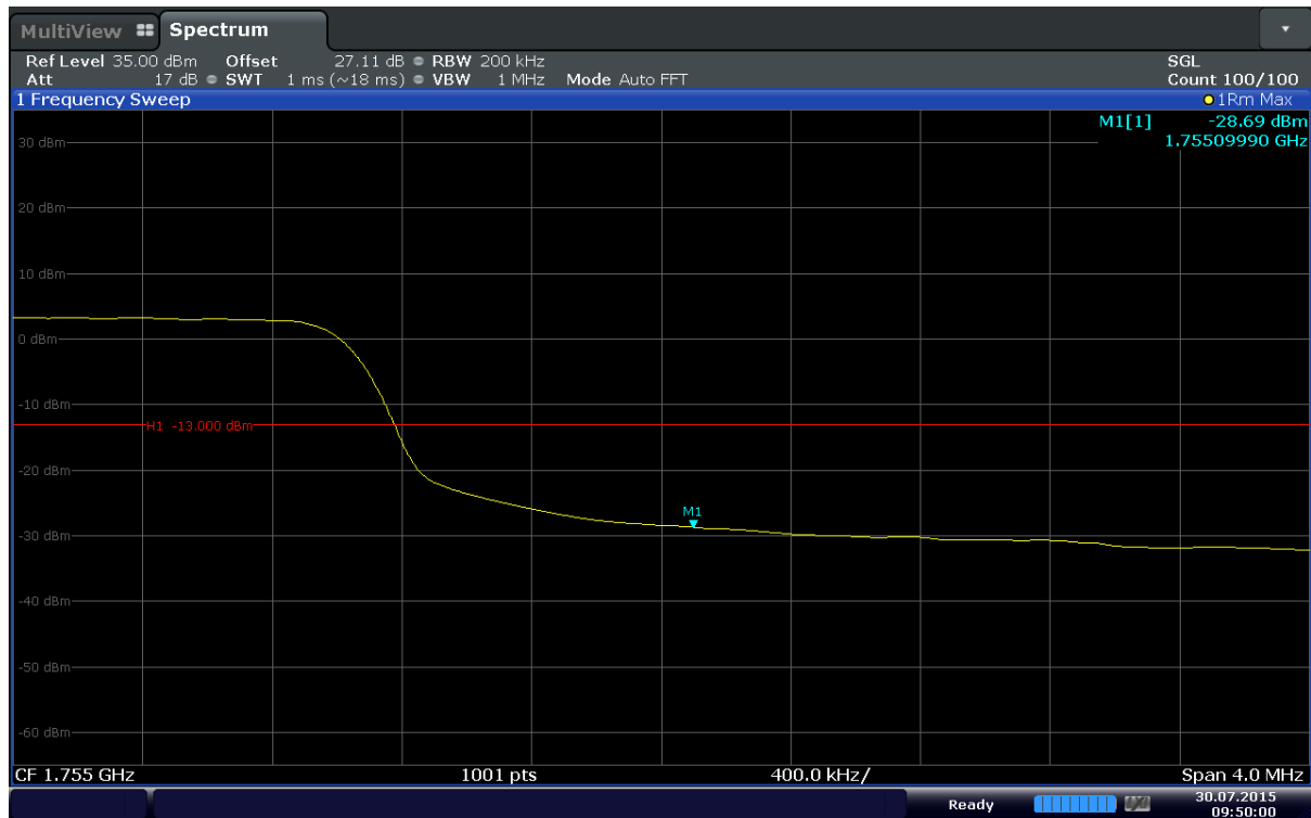
Plot 6-117. Upper Band Edge Plot (Band 4 – 20MHz – QPSK – RB Size 100)
