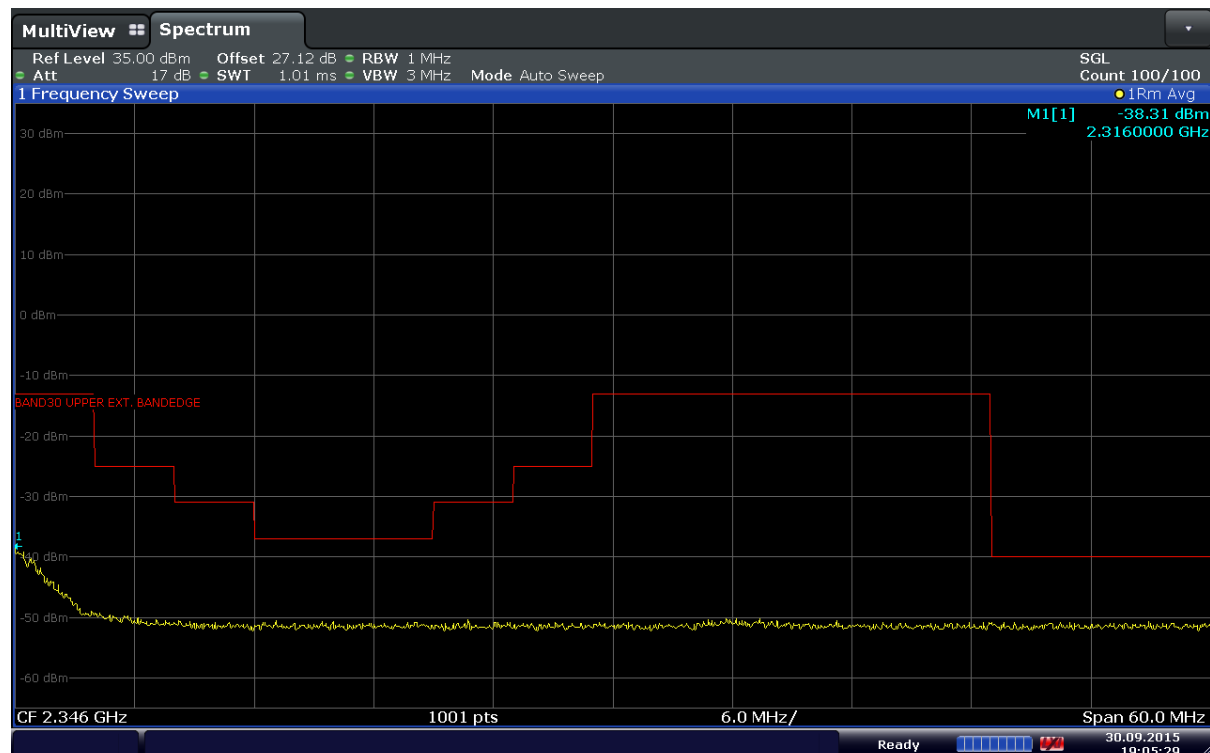
Plot 6-126. Extended Upper Band Edge Plot (Band 30 – 5MHz – QPSK – RB Size 25)
