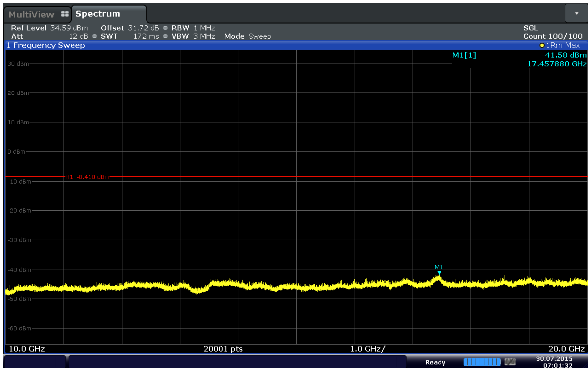
Plot 6-42. Conducted Spurious Plot (Band 4–1.4MHz–QPSK–RB Size 1–RB Offset 5–Ch.20393)
