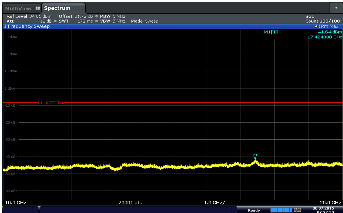
Plot 6-70. Conducted Spurious Plot (Band 4–20MHz–QPSK–RB Size 1–RB Offset 49–Ch.20175)
