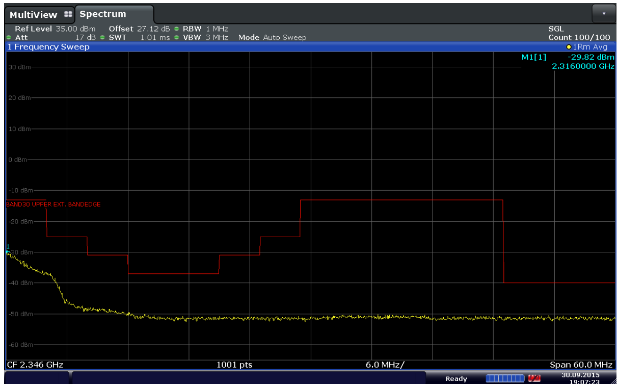
Plot 6-130. Extended Upper Band Edge Plot (Band 30 – 10MHz – QPSK – RB Size 50)
