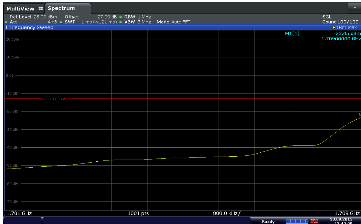
Plot 6-96. Extended Lower Band Edge Plot (Band 4 – 1.4MHz – QPSK – RB Size 6)
