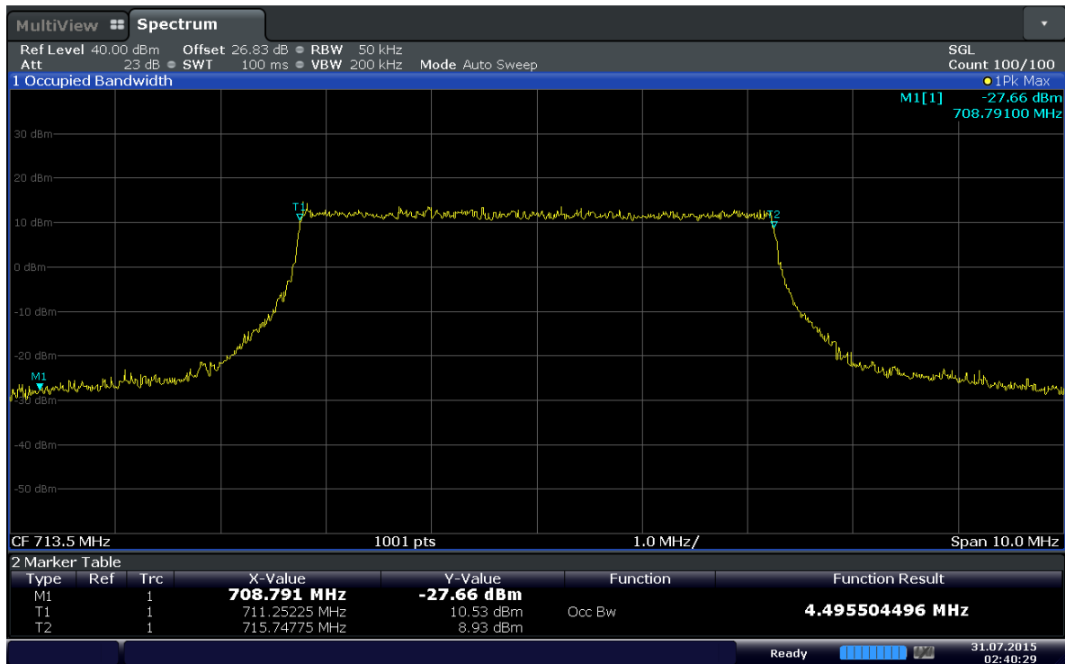
Plot 6-5. Occupied Bandwidth Plot (Band 12 – 5MHz QPSK - RB Size 25)
