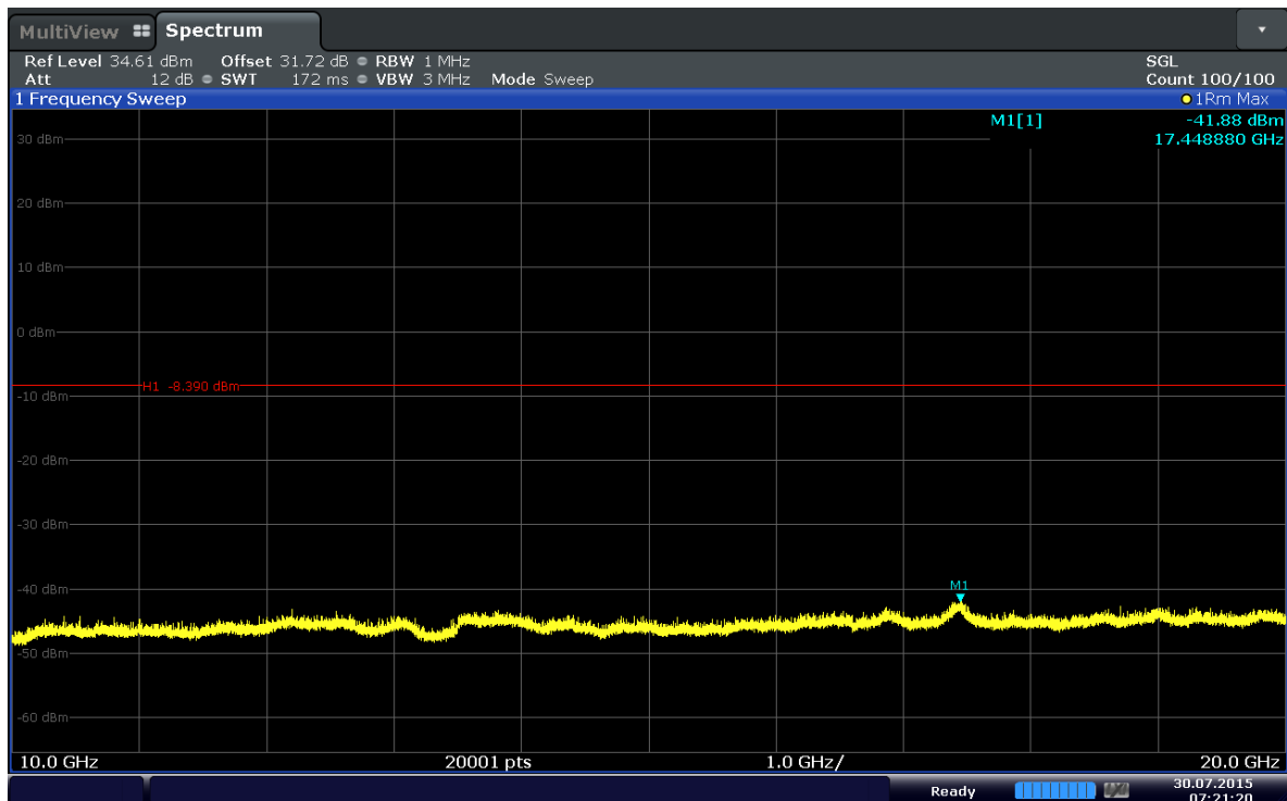
Plot 6-64. Conducted Spurious Plot (Band 4–15MHz–QPSK–RB Size 1–RB Offset 37–Ch.20175)
