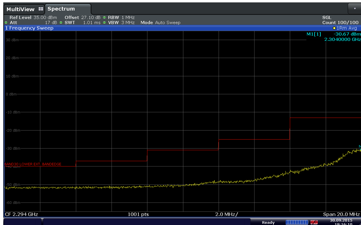
Plot 6-124. Extended Lower Band Edge Plot (Band 30 – 5MHz – QPSK – RB Size 25)
