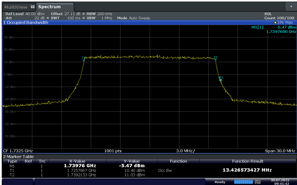
Plot 6-17. Occupied Bandwidth Plot (Band 4 - 15MHz QPSK - RB Size 75)
