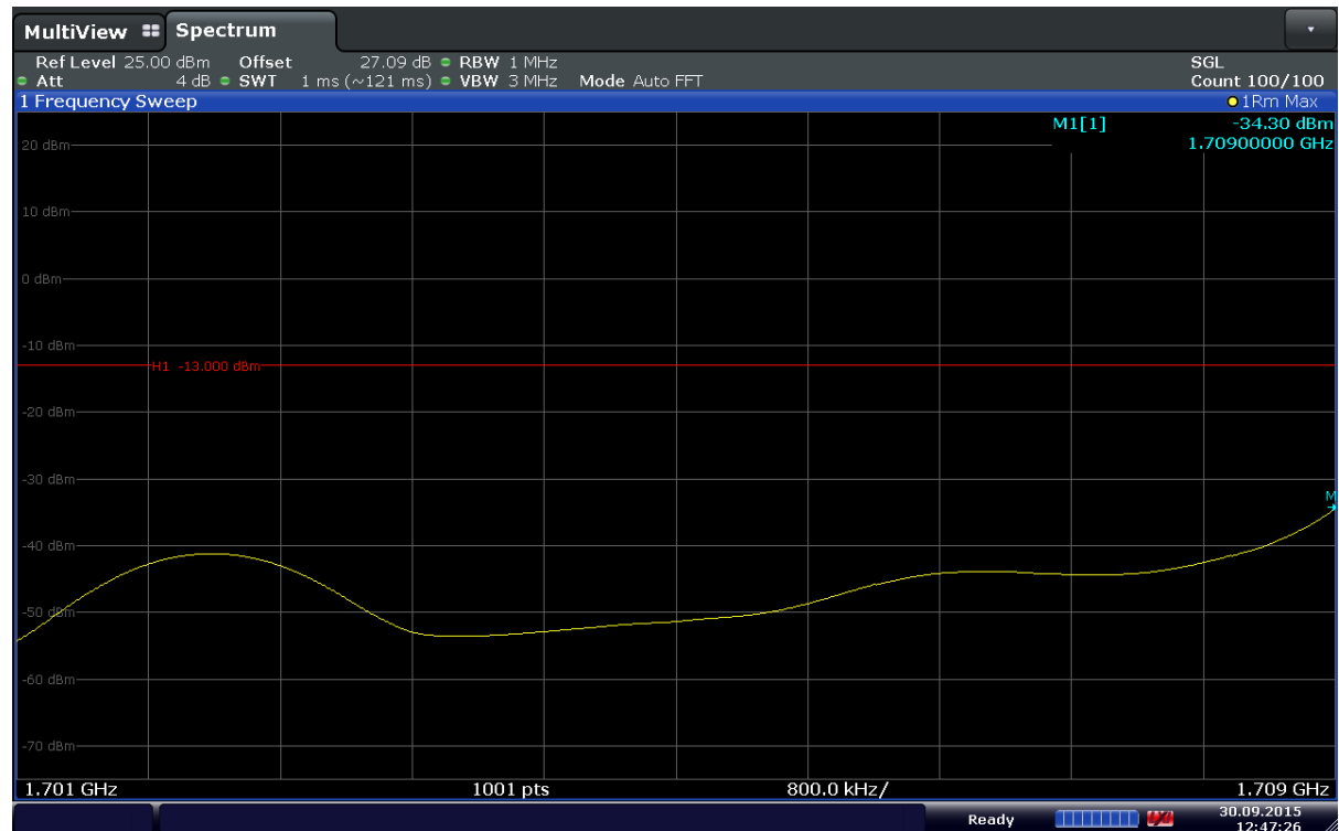
Plot 6-120. Extended Lower Band Edge Plot (Band 4 – 20MHz – QPSK – RB Size 1 – RB Offset 0)
