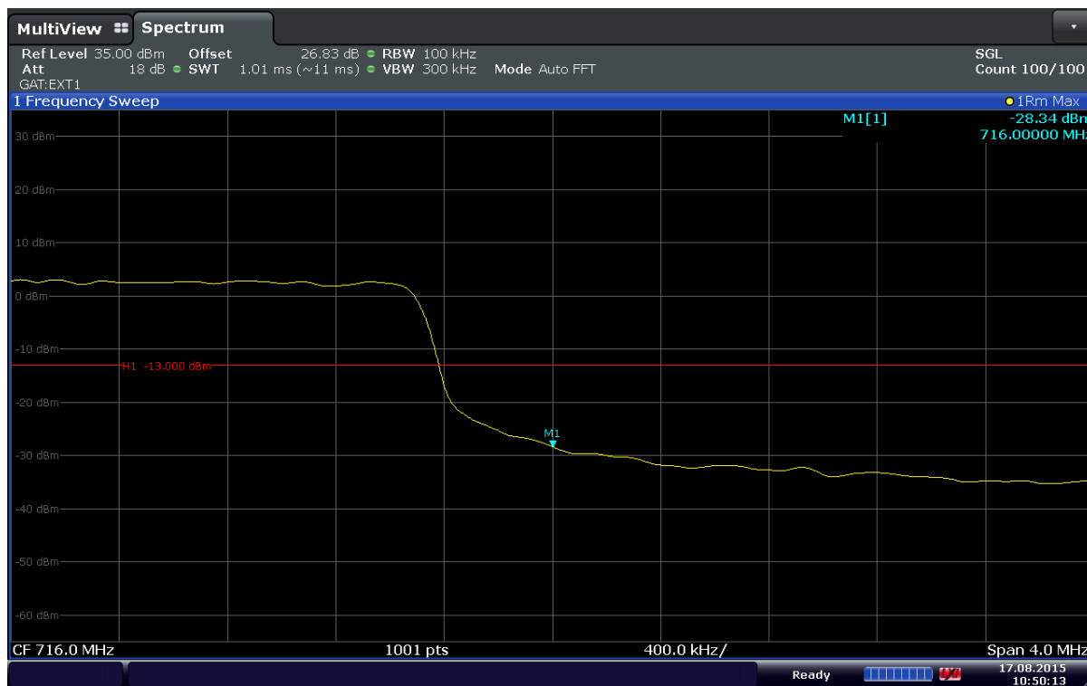
Plot 6-92. Upper Band Edge Plot (Band 12 – 10MHz – QPSK – RB Size 50)
