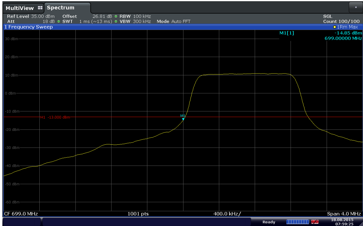
Plot 6-85. Lower Band Edge Plot (Band 12 – 1.4MHz – QPSK – RB Size 6)
