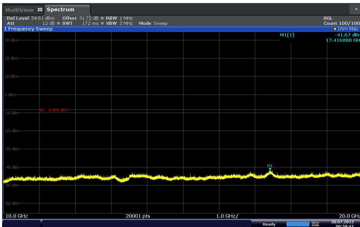
Plot 6-40. Conducted Spurious Plot (Band 4–1.4MHz–QPSK–RB Size 1–RB Offset 5–Ch.20175)
