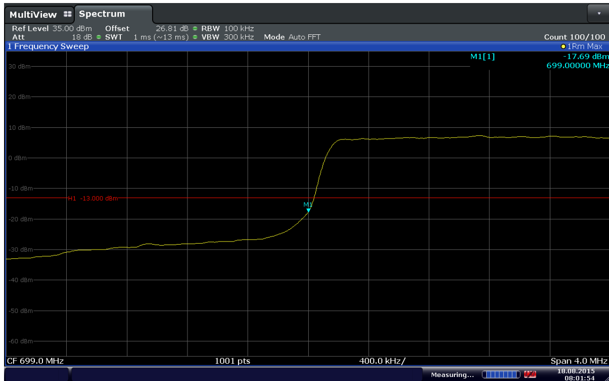
Plot 6-87. Lower Band Edge Plot (Band 12 – 3MHz – QPSK – RB Size 15)
