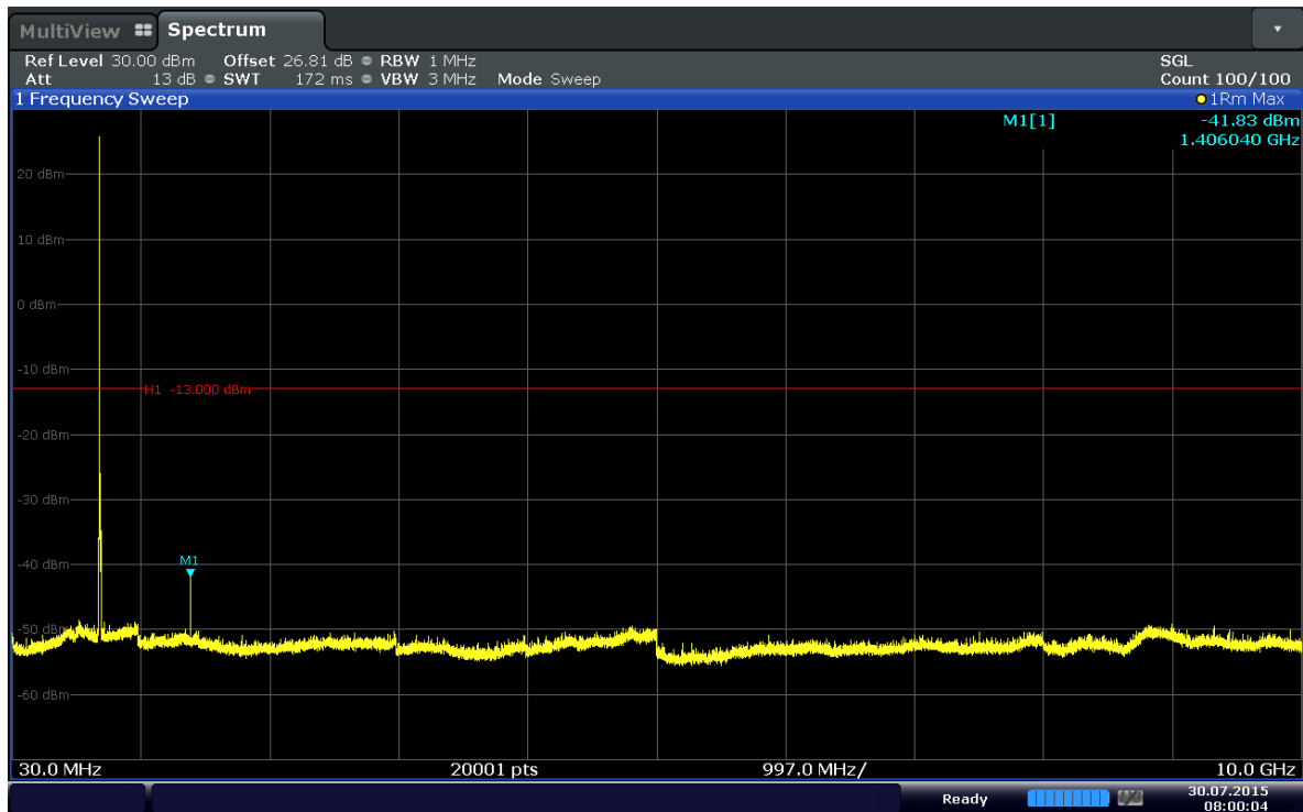
Plot 6-35. Conducted Spurious Plot (Band 12–10MHz–QPSK–RB Size 1–RB Offset 0–Ch.23095)
