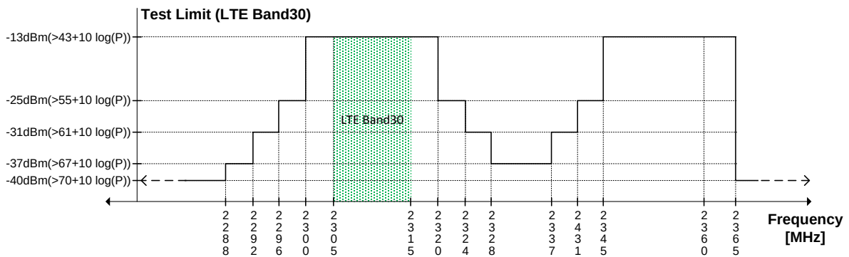
Figure 6-4. Emission limits (LTE Band 30)
