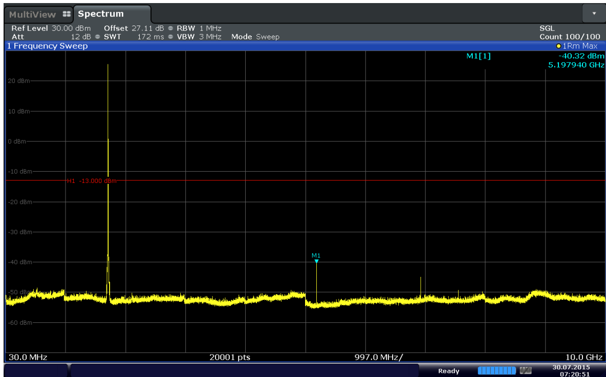
Plot 6-63. Conducted Spurious Plot (Band 4–15MHz–QPSK–RB Size 1–RB Offset 37–Ch.20175)
