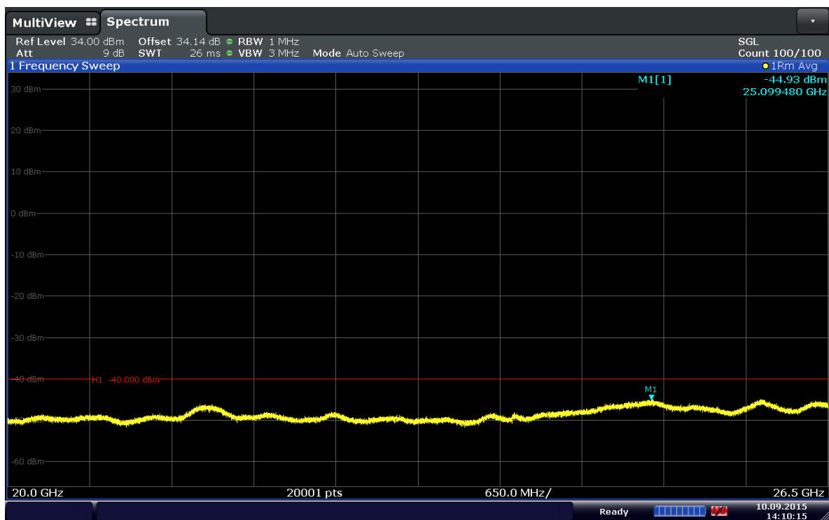
Plot 6-78. Conducted Spurious Plot (Band 30–5MHz–QPSK–RB Size 1–RB Offset 24– Ch.27710)
