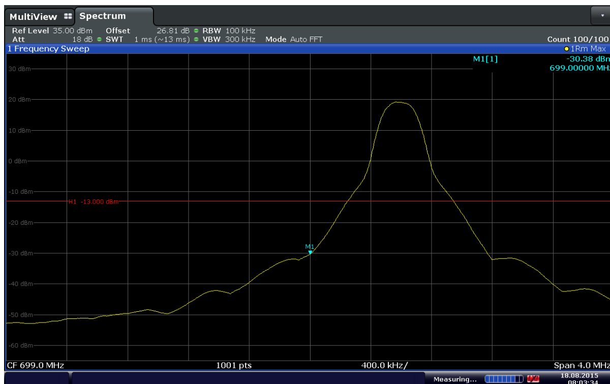
Plot 6-93. Lower Band Edge Plot (Band 12 – 10MHz – QPSK – RB Size 1 – RB Offset 0)
