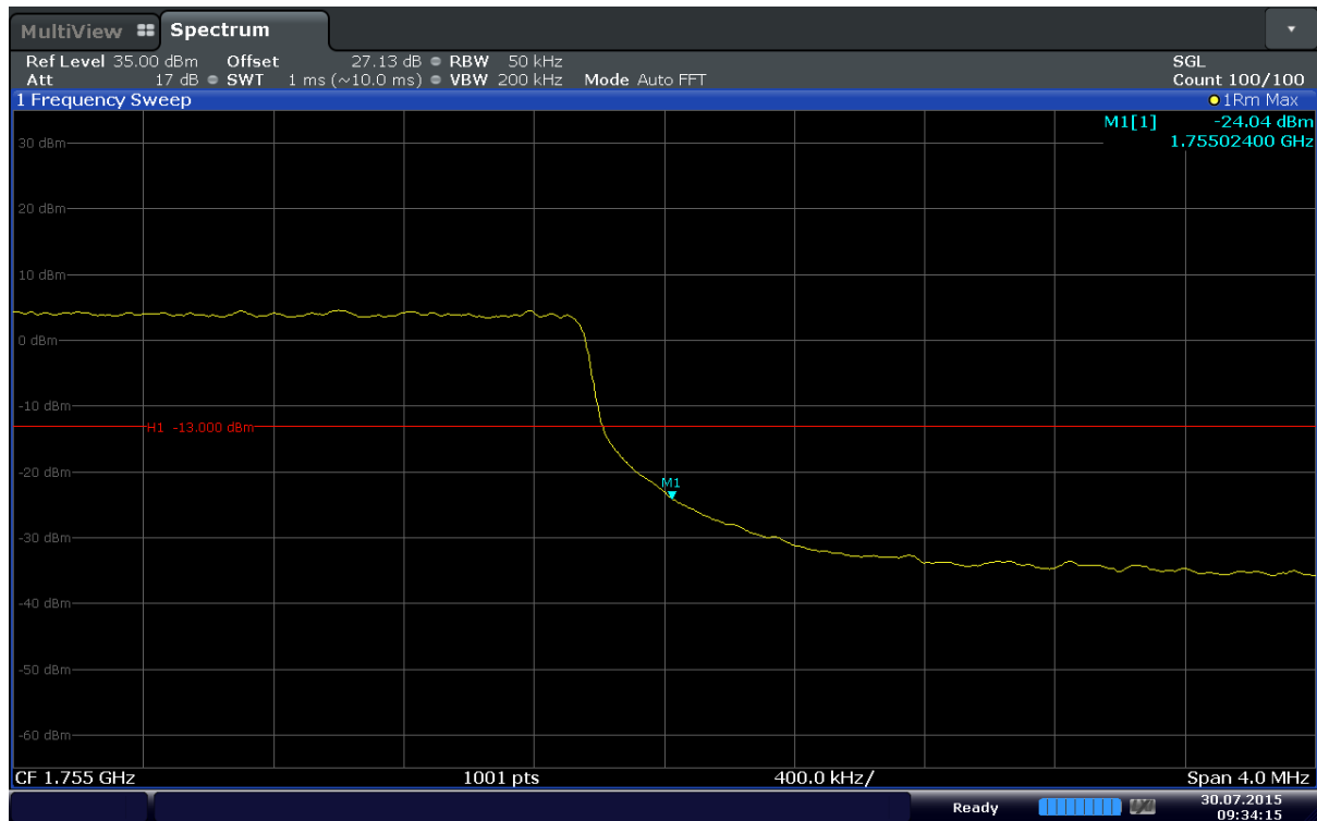
Plot 6-105. Upper Band Edge Plot (Band 4 – 5MHz – QPSK – RB Size 25)
