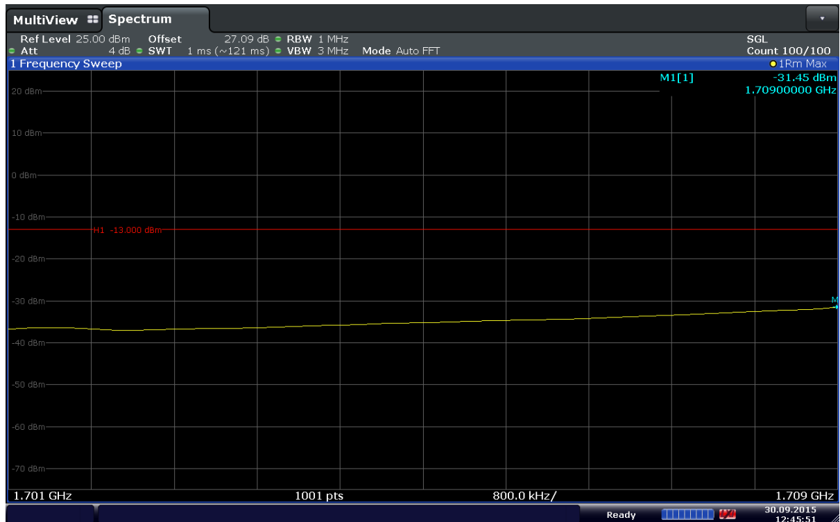
Plot 6-112. Extended Lower Band Edge Plot (Band 4 – 15MHz – QPSK – RB Size 75)
