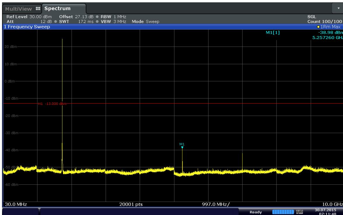
Plot 6-53. Conducted Spurious Plot (Band 4–5MHz–QPSK–RB Size 1–RB Offset 12–Ch.20375)
