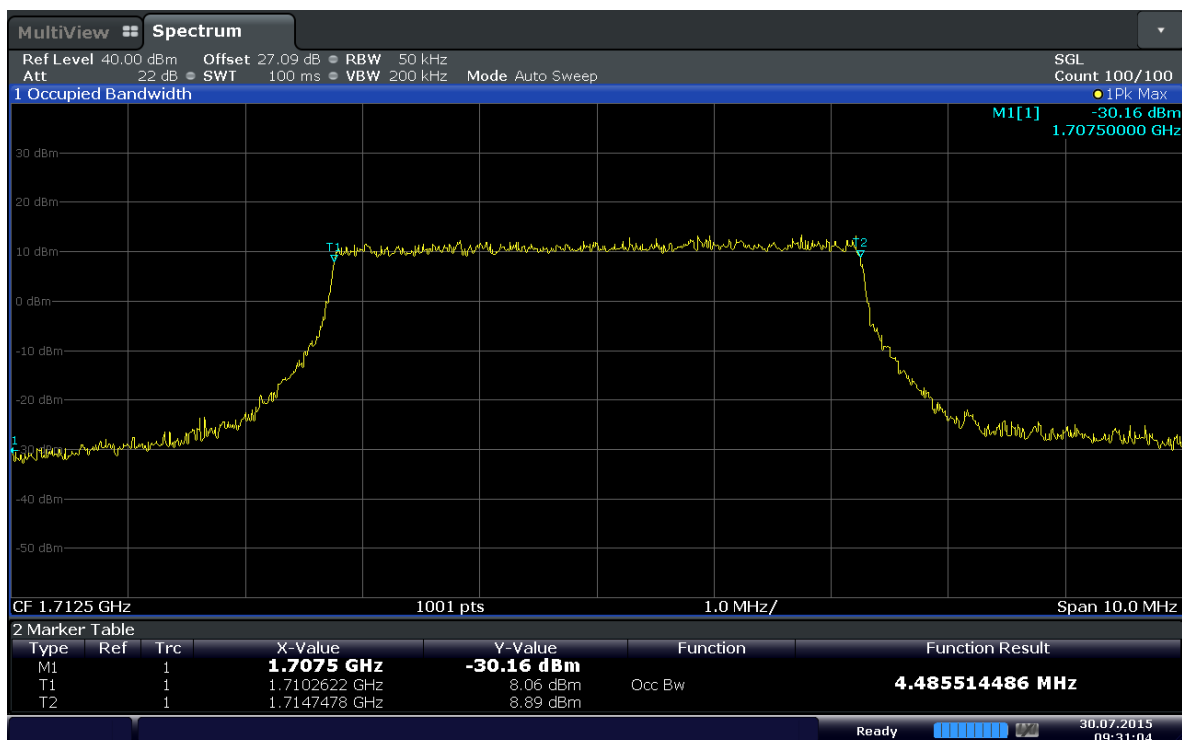
Plot 6-14. Occupied Bandwidth Plot (Band 4 – 5MHz 16QAM - RB Size 25)
