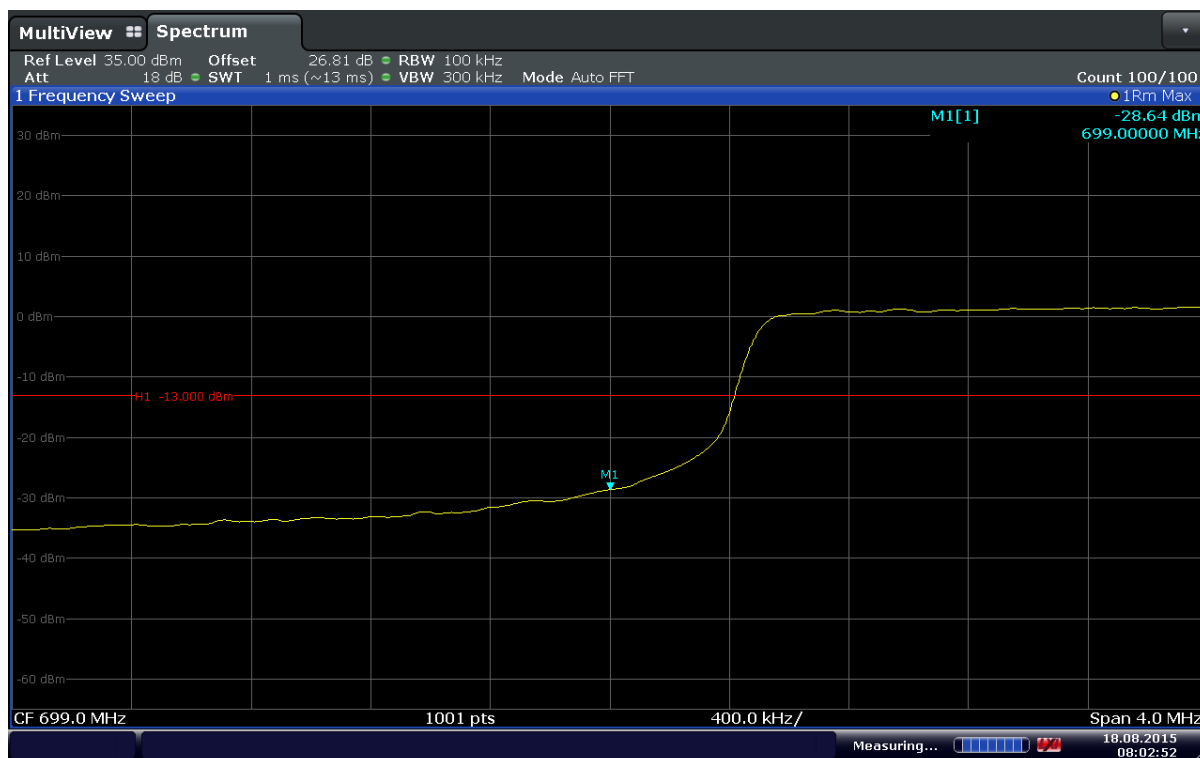
Plot 6-91. Lower Band Edge Plot (Band 12 – 10MHz – QPSK – RB Size 50)
