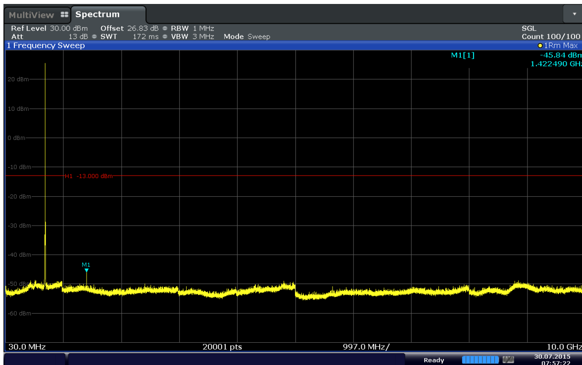
Plot 6-33. Conducted Spurious Plot (Band 12–5MHz–QPSK–RB Size 1–RB Offset 0–Ch.23155)
