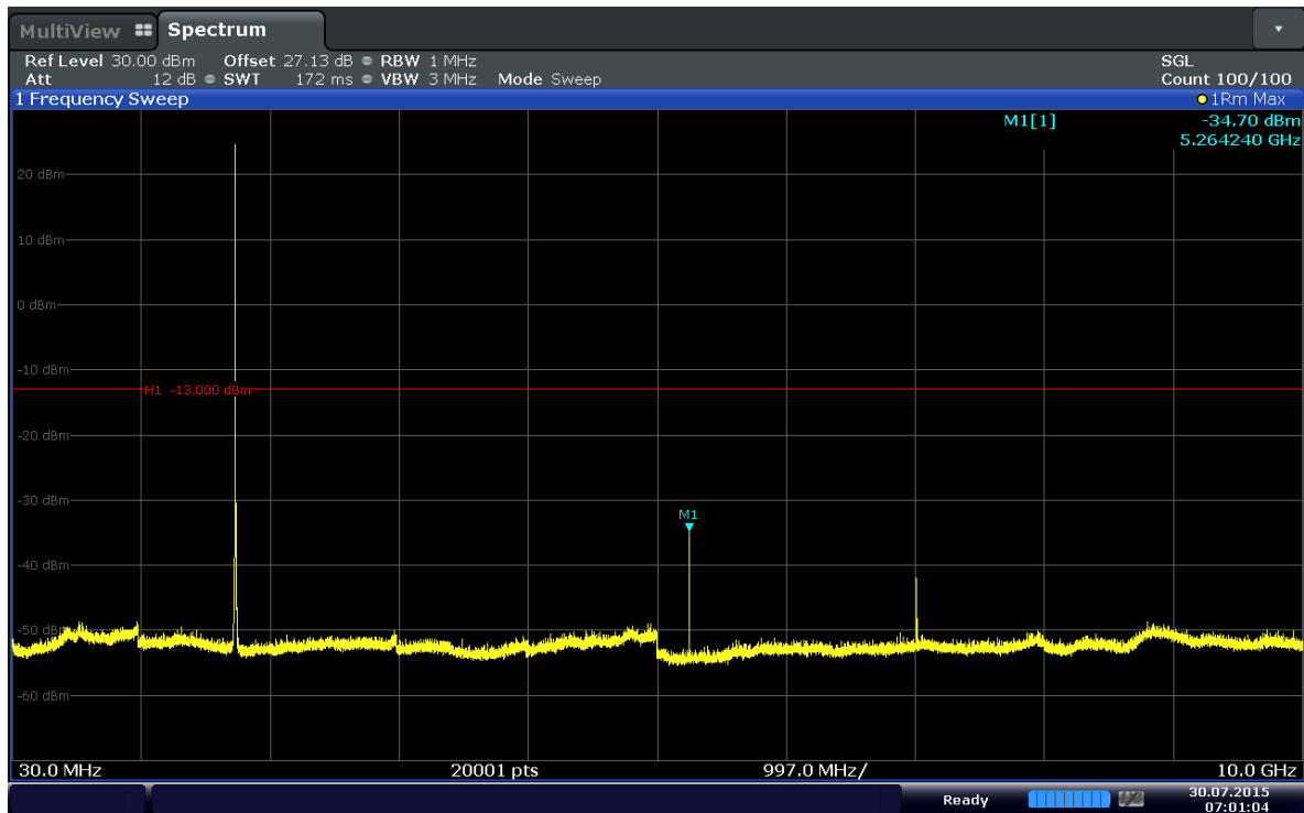
Plot 6-41. Conducted Spurious Plot (Band 4–1.4MHz–QPSK–RB Size 1–RB Offset 5–Ch.20393)
