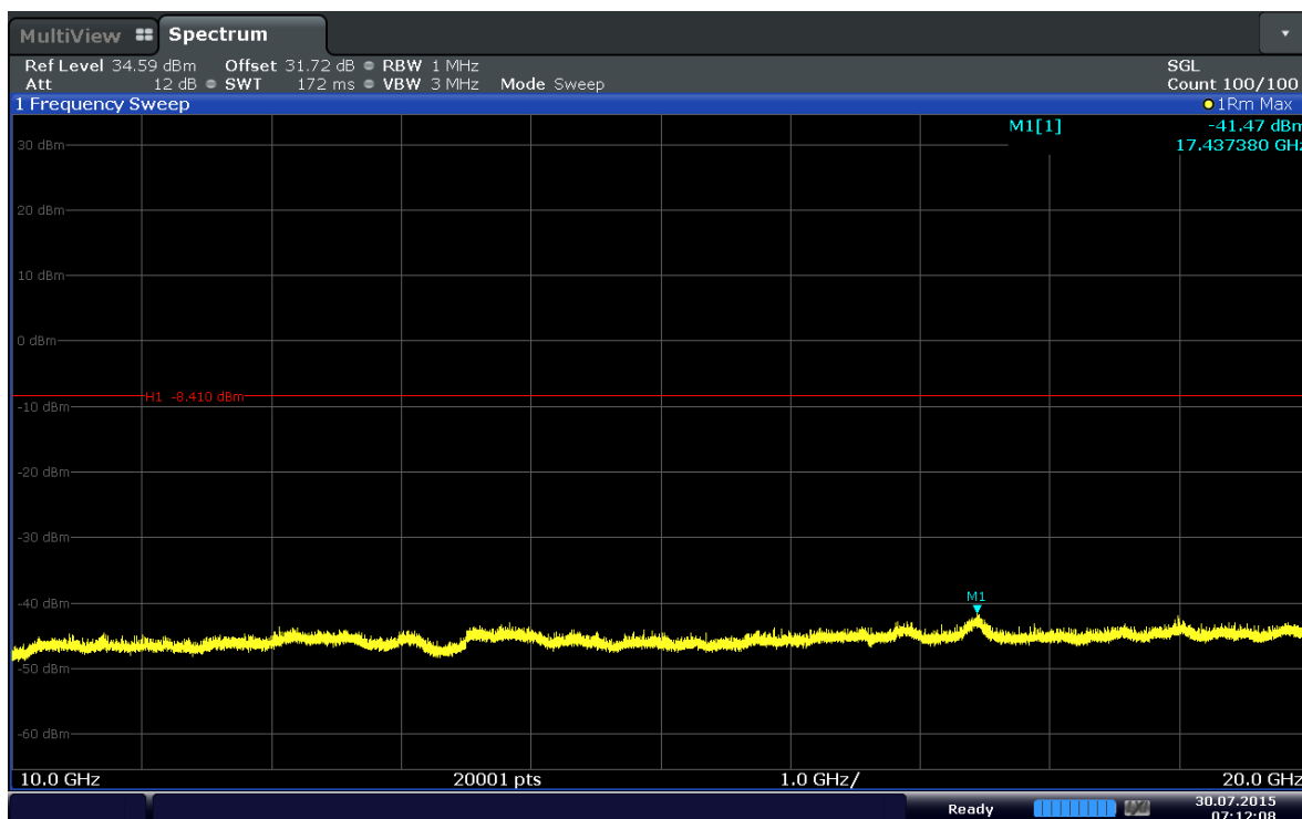
Plot 6-54. Conducted Spurious Plot (Band 4–5MHz–QPSK–RB Size 1–RB Offset 12–Ch.20375)
