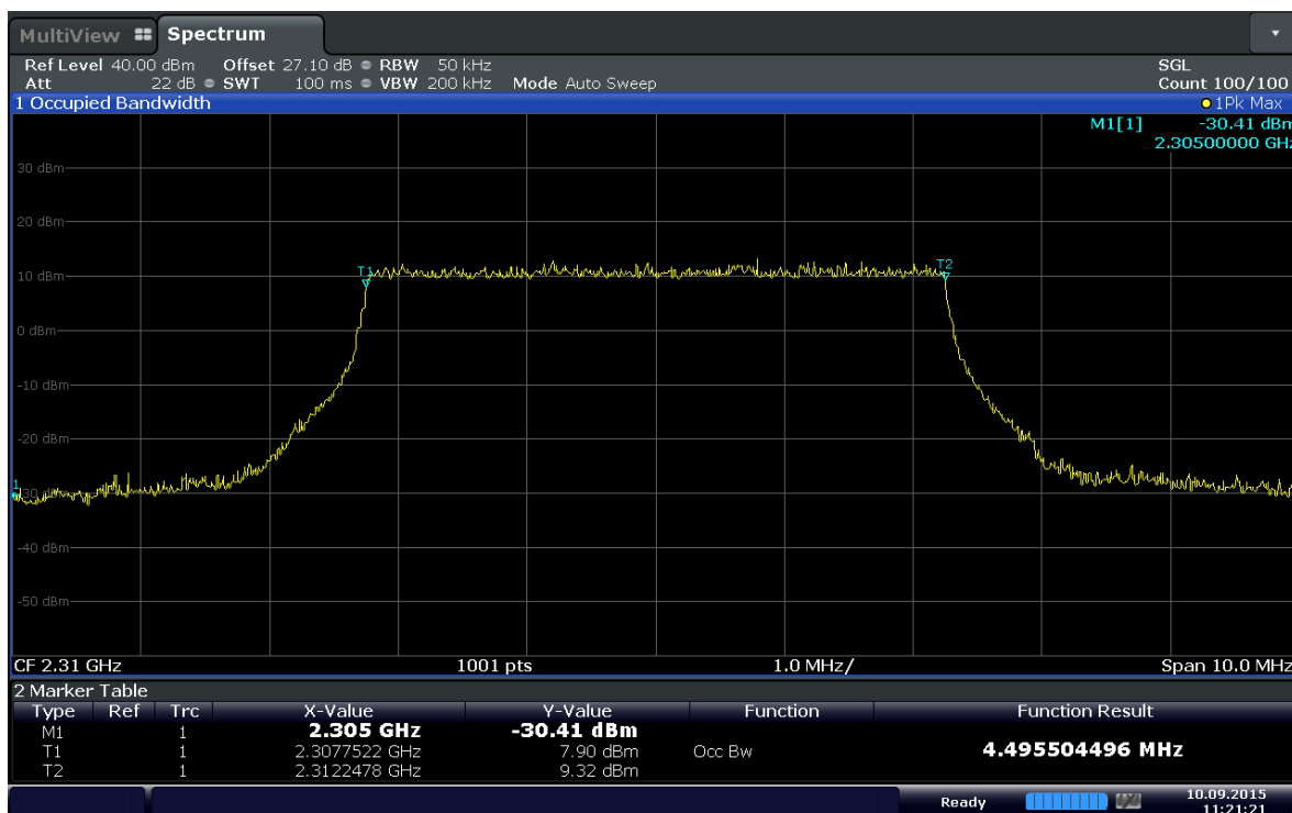
Plot 6-21. Occupied Bandwidth Plot (Band 30 – 5MHz QPSK - RB Size 25)
