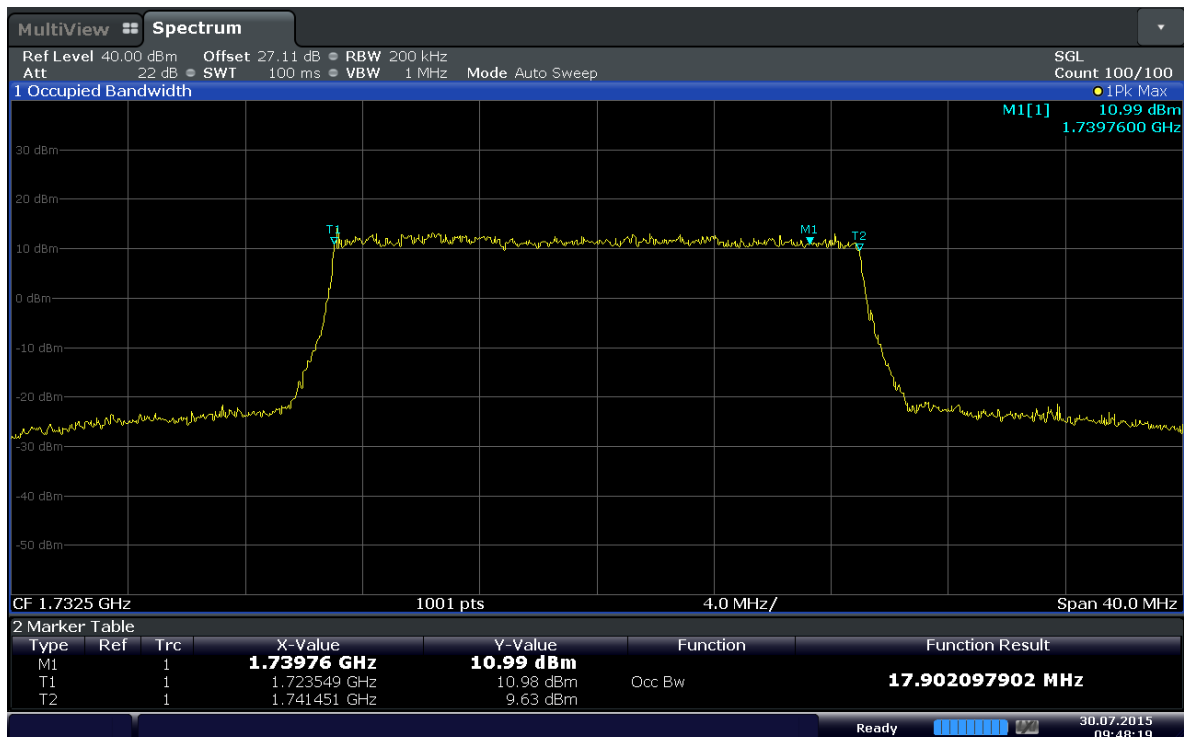
Plot 6-20. Occupied Bandwidth Plot (Band 4 - 20MHz 16QAM - RB Size 100)
