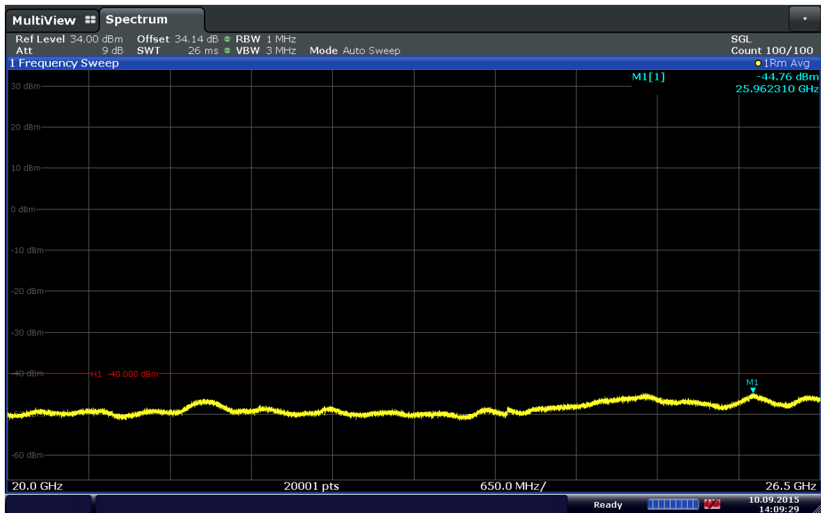
Plot 6-84. Conducted Spurious Plot (Band 30–10MHz–QPSK–RB Size 1–RB Offset 24–Ch.27710)
