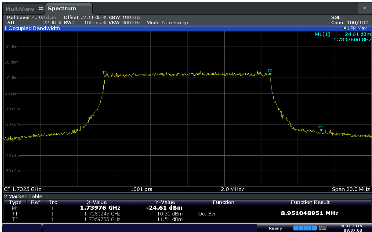
Plot 6-15. Occupied Bandwidth Plot (Band 4 – 10MHz QPSK - RB Size 50)
