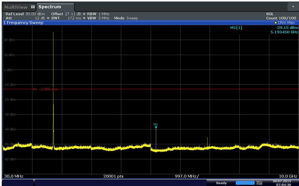
Plot 6-45. Conducted Spurious Plot (Band 4-3MHz-QPSK-RB Size 1-RB Offset 0-Ch.20175)
