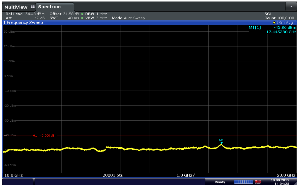
Plot 6-77. Conducted Spurious Plot (Band 30–5MHz–QPSK–RB Size 1–RB Offset 24– Ch.27710)
