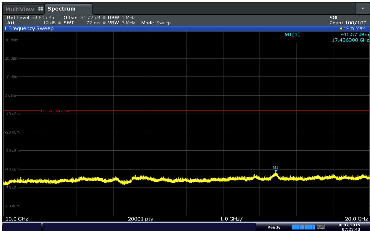
Plot 6-66. Conducted Spurious Plot (Band 4–15MHz–QPSK–RB Size 1–RB Offset 0–Ch.20325)
