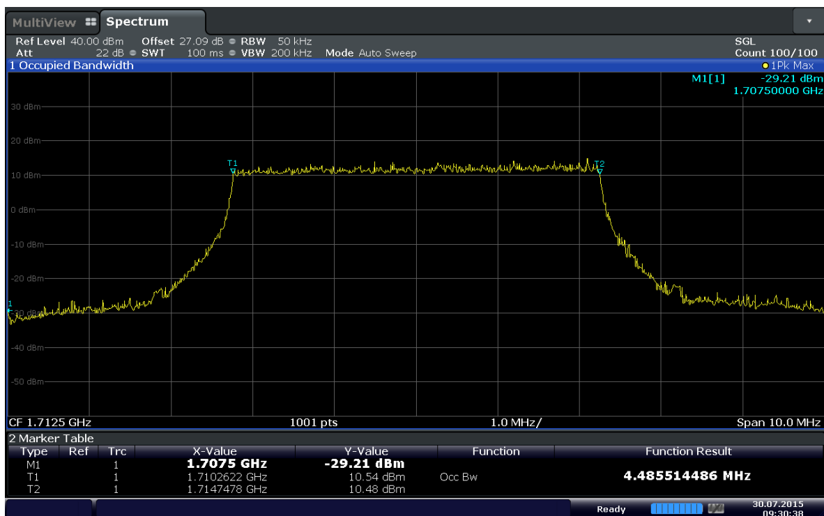
Plot 6-13. Occupied Bandwidth Plot (Band 4 – 5MHz QPSK - RB Size 25)
