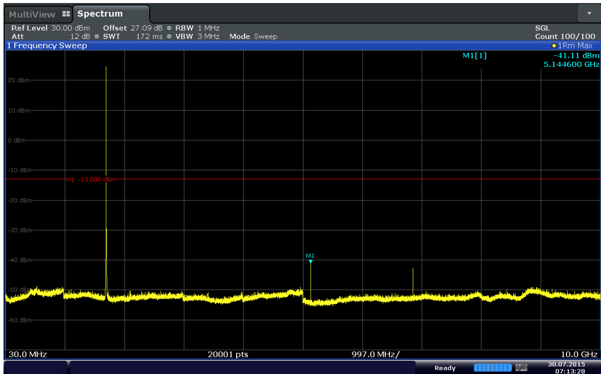
Plot 6-55. Conducted Spurious Plot (Band 4–10MHz–QPSK–RB Size 1–RB Offset 24–Ch.20000)
