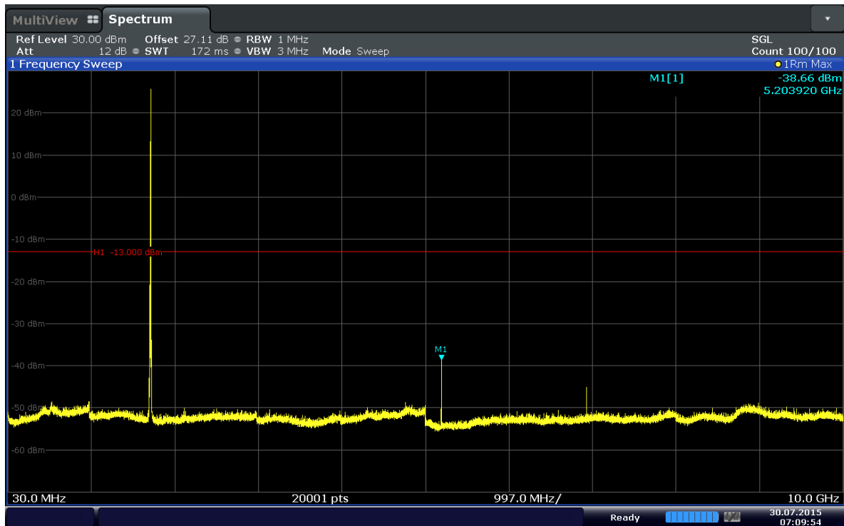
Plot 6-51. Conducted Spurious Plot (Band 4–5MHz–QPSK–RB Size 1–RB Offset 24–Ch.20175)
