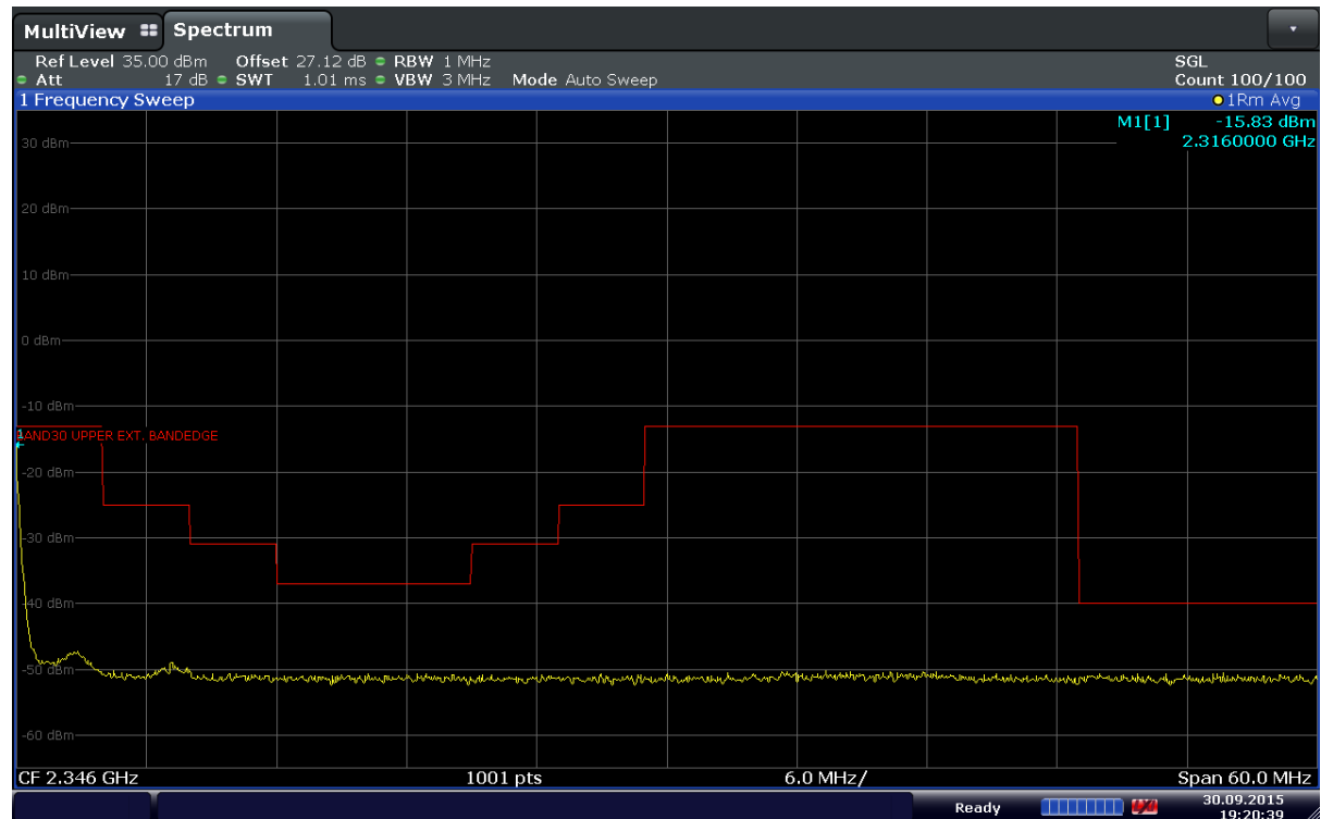
Plot 6-134. Extended Upper Band Edge Plot (Band 30 – 10MHz – QPSK – RB Size 1 – RB Offset 49)
