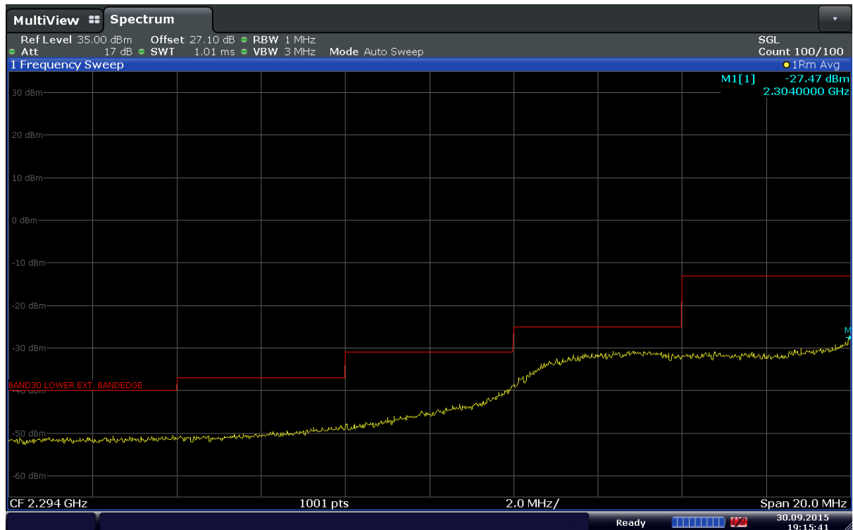
Plot 6-128. Extended Lower Band Edge Plot (Band 30 – 10MHz – QPSK – RB Size 50)
