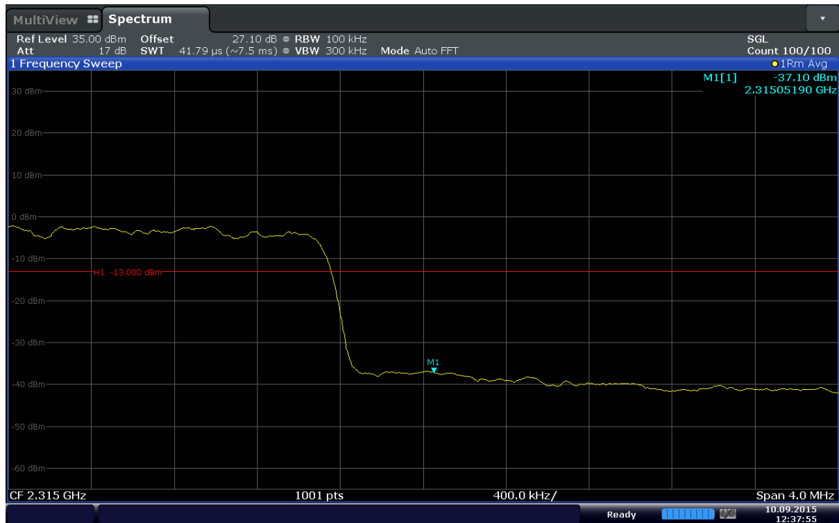
Plot 6-129. Upper Band Edge Plot (Band 30 – 10MHz – QPSK – RB Size 50)
