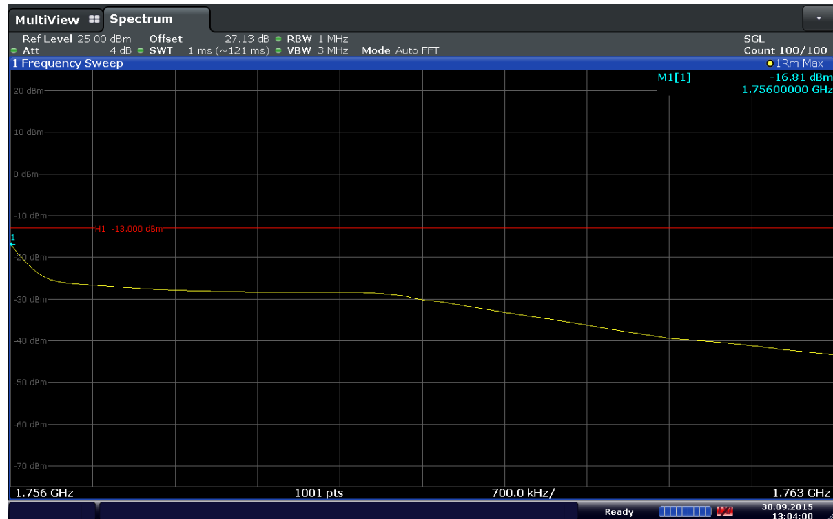
Plot 6-106. Extended Upper Band Edge Plot (Band 4 – 5MHz – QPSK – RB Size 25)
