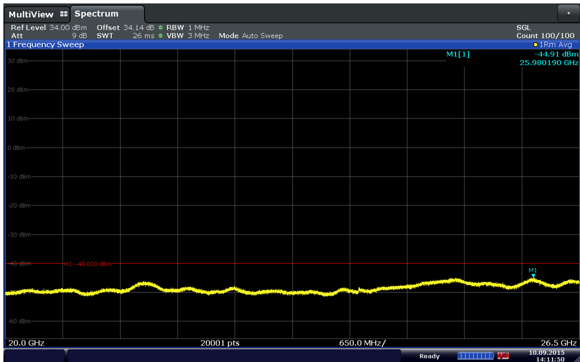
Plot 6-80. Conducted Spurious Plot (Band 30–5MHz–QPSK–RB Size 1–RB Offset 12– Ch.27735)
