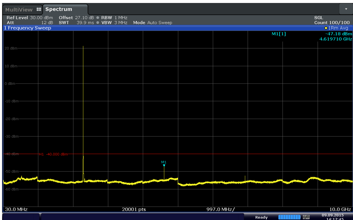
Plot 6-82. Conducted Spurious Plot (Band 30–10MHz–QPSK–RB Size 1–RB Offset 24–Ch.27710)
