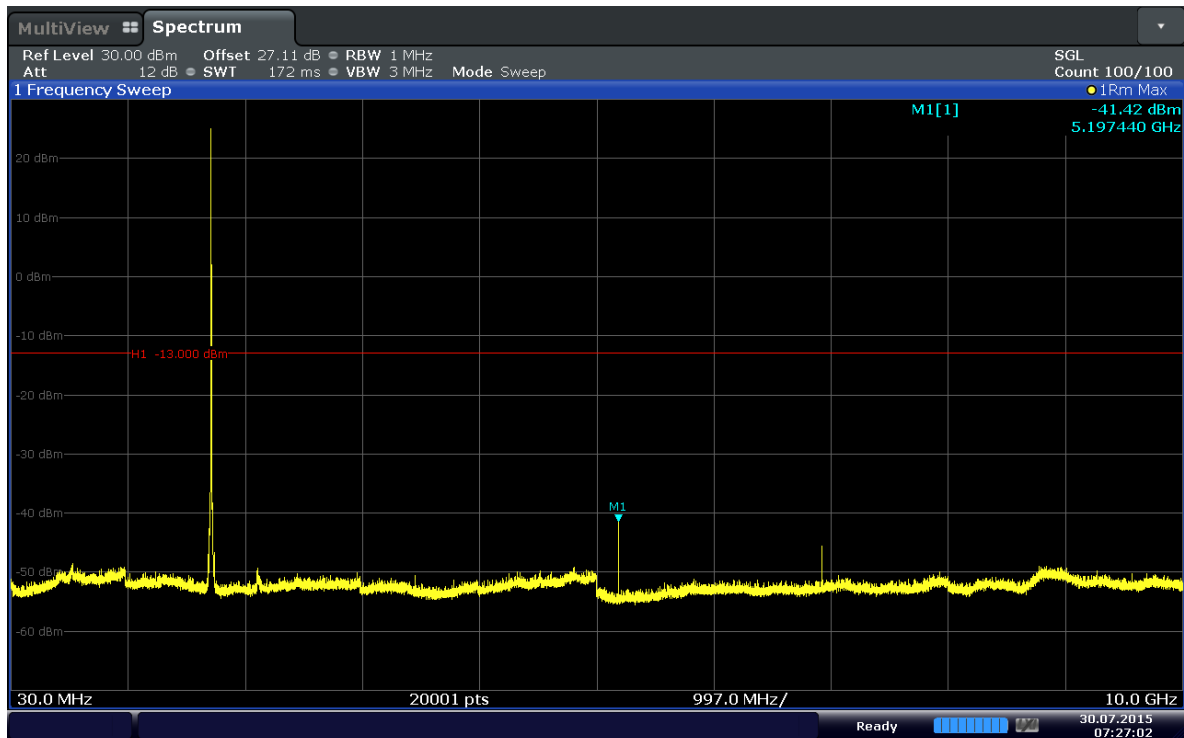
Plot 6-69. Conducted Spurious Plot (Band 4–20MHz–QPSK–RB Size 1–RB Offset 49–Ch.20175)
