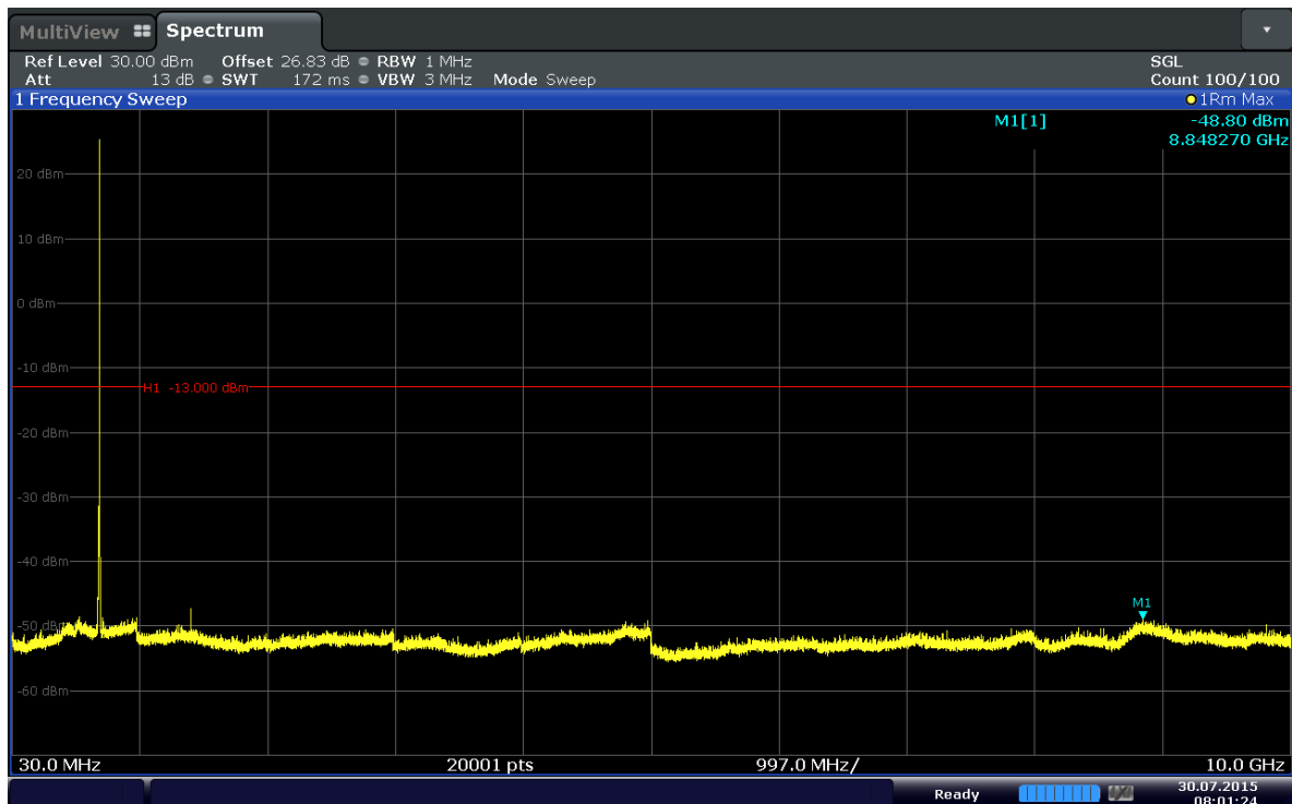
Plot 6-36. Conducted Spurious Plot (Band 12–10MHz–QPSK–RB Size 1–RB Offset 24–Ch.23130)
