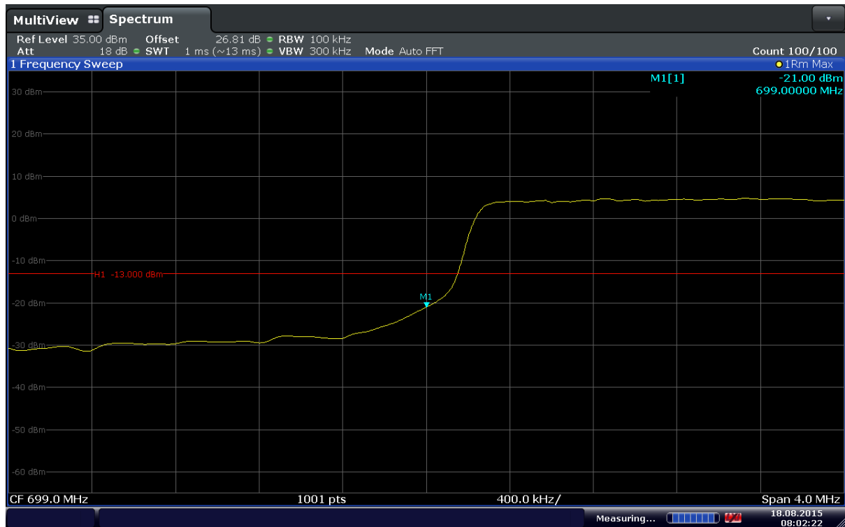
Plot 6-89. Lower Band Edge Plot (Band 12 – 5MHz – QPSK – RB Size 25)
