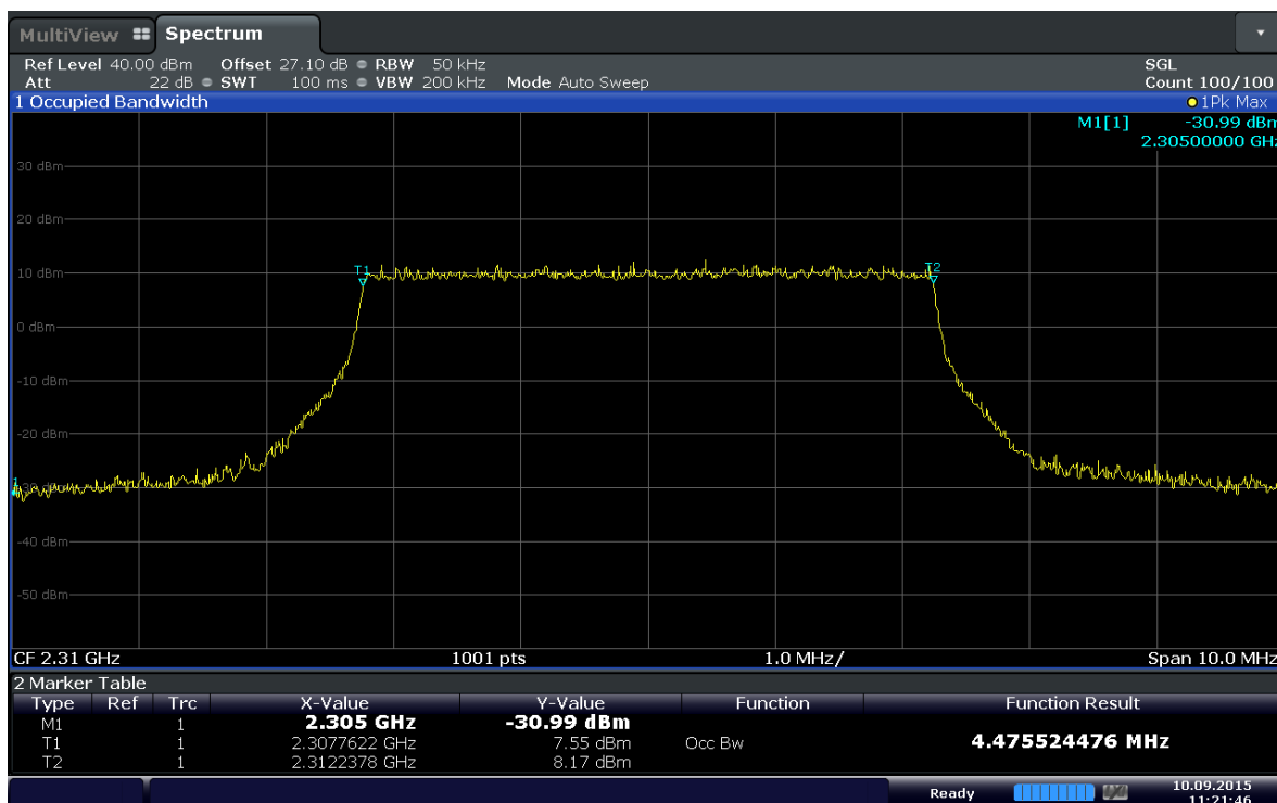
Plot 6-22. Occupied Bandwidth Plot (Band 30 – 5MHz 16QAM - RB Size 25)
