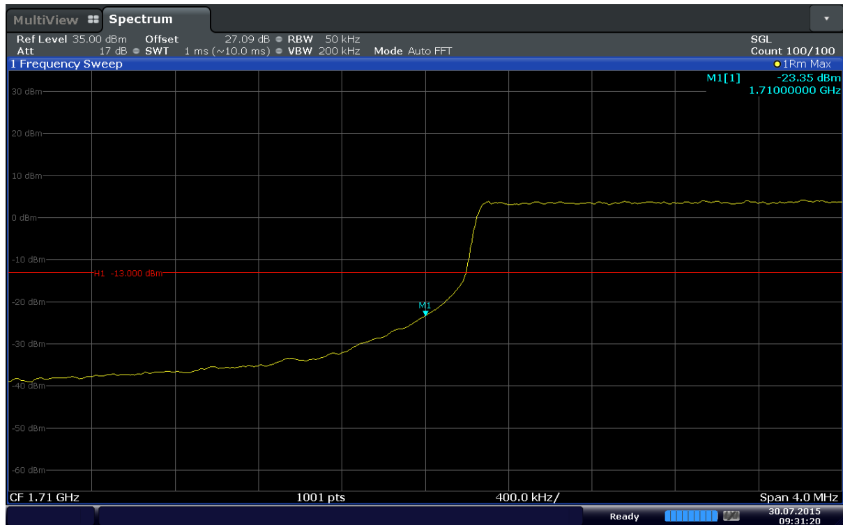
Plot 6-103. Lower Band Edge Plot (Band 4 – 5MHz – QPSK – RB Size 25)
