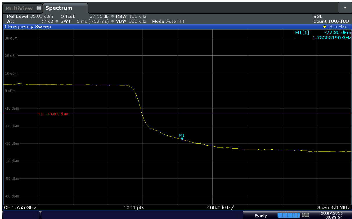
Plot 6-109. Upper Band Edge Plot (Band 4 – 10MHz – QPSK – RB Size 50)
