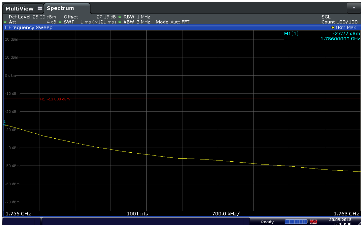
Plot 6-102. Extended Upper Band Edge Plot (Band 4 – 3MHz – QPSK – RB Size 15)
