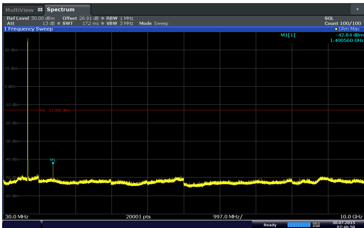
Plot 6-25. Conducted Spurious Plot (Band 12-1.4MHz-QPSK-RB Size 1-RB Offset 5-Ch.23017)
