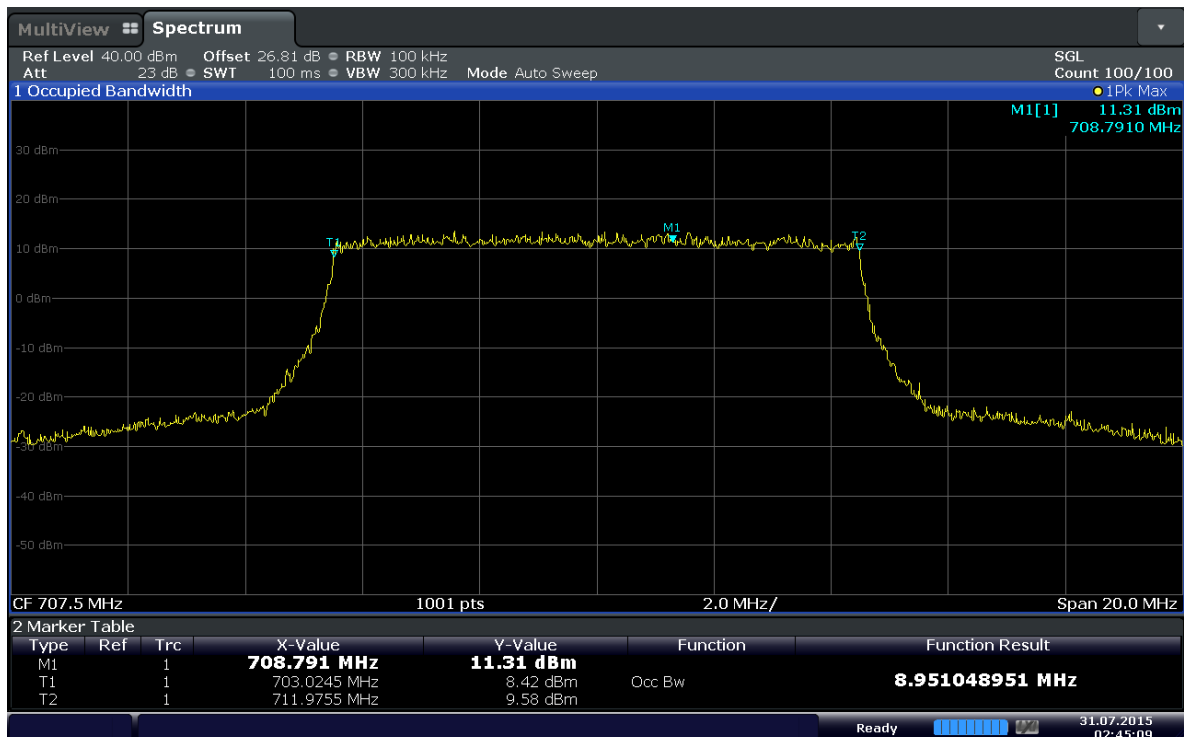
Plot 6-8. Occupied Bandwidth Plot (Band 12 – 10MHz 16QAM - RB Size 50)
