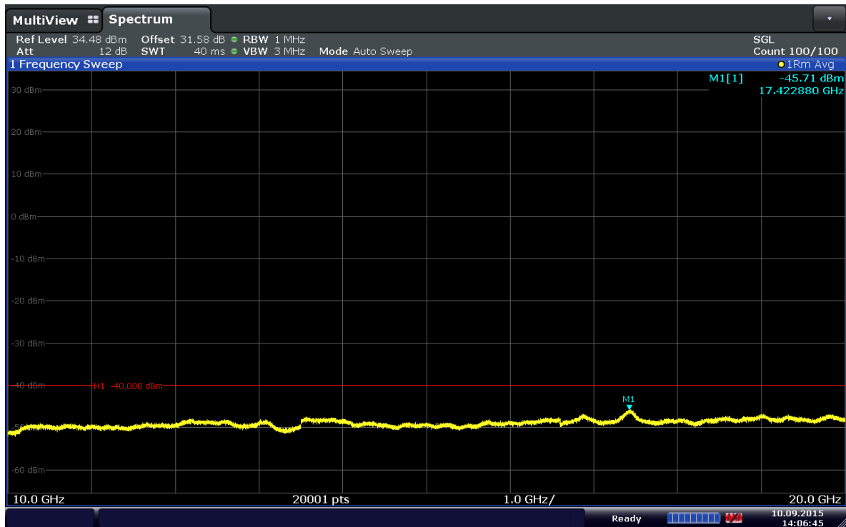
Plot 6-83. Conducted Spurious Plot (Band 30–10MHz–QPSK–RB Size 1–RB Offset 24–Ch.27710)
