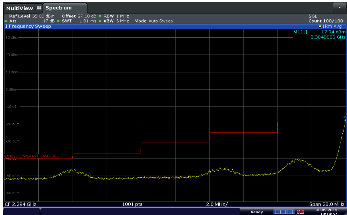
Plot 6-132. Extended Lower Band Edge Plot (Band 30 – 10MHz – QPSK – RB Size1 – RB Offset 0)
