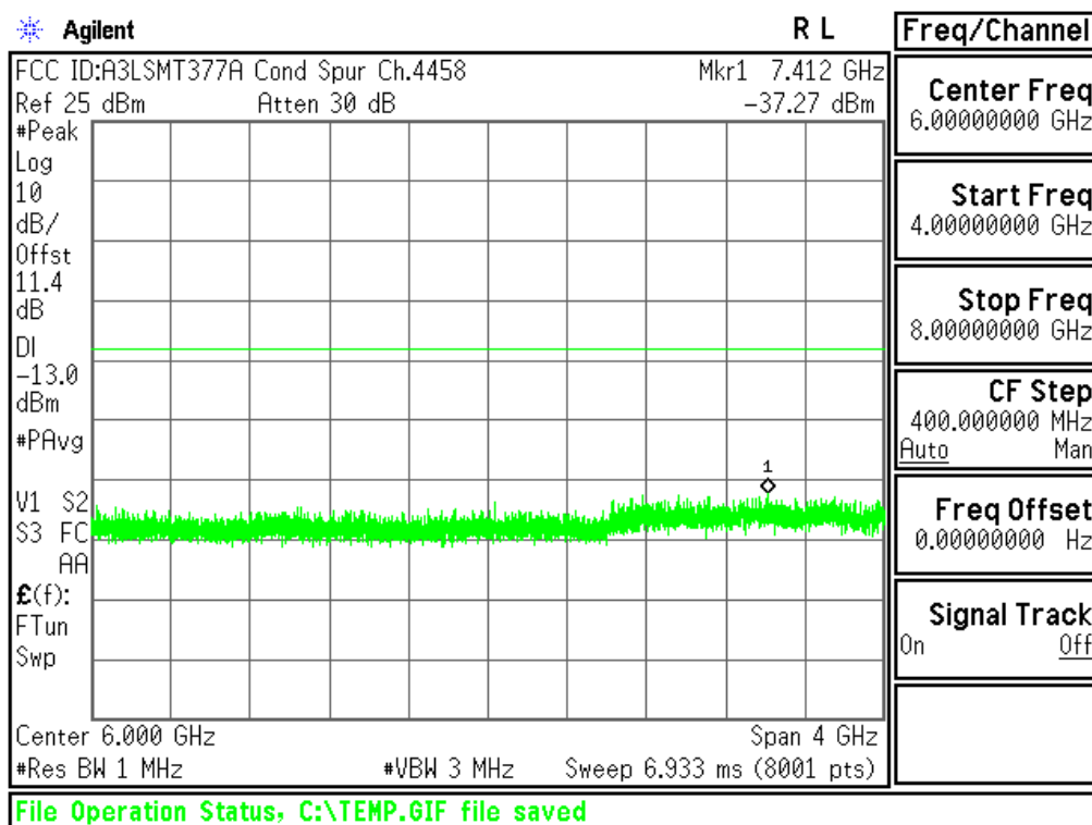
Plot 6-10. Conducted Spurious Plot (Cellular WCDMA Mode - Ch.4233(DL4458))
