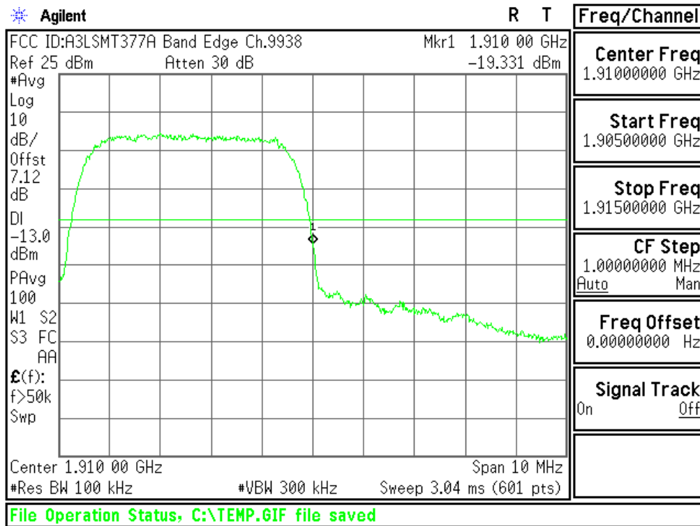
Plot 6-31. Upper Band Edge Plot (PCS WCDMA Mode - Ch.9538(DL9938))
