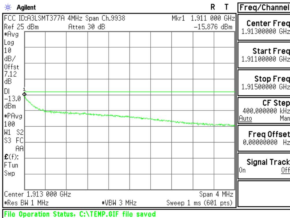
Plot 6-32. Extended Upper Band Edge Plot (PCS WCDMA Mode - Ch.9538(DL9938))
