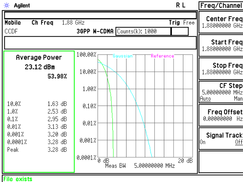
Plot 6-33. Peak-Average Ratio Plot (PCS WCDMA Mode - Ch.9400(DL9800))
