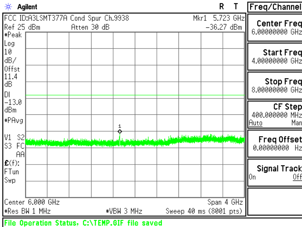
Plot 6-23. Conducted Spurious Plot (PCS WCDMA Mode - Ch.9538(DL9938))
