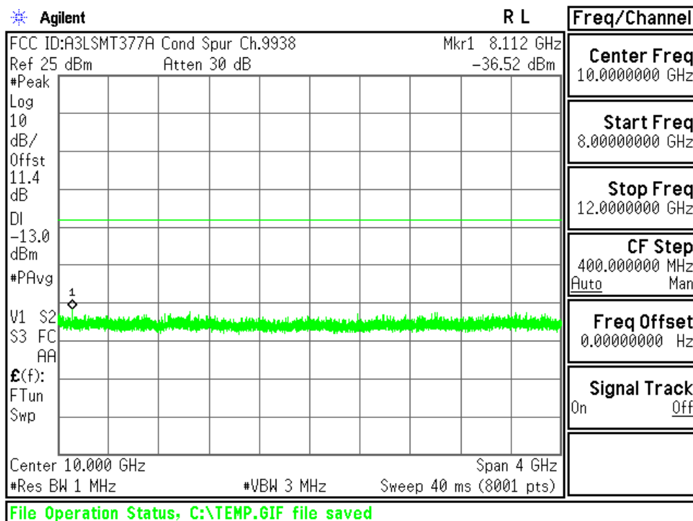
Plot 6-24. Conducted Spurious Plot (PCS WCDMA Mode - Ch.9538(DL9938))
