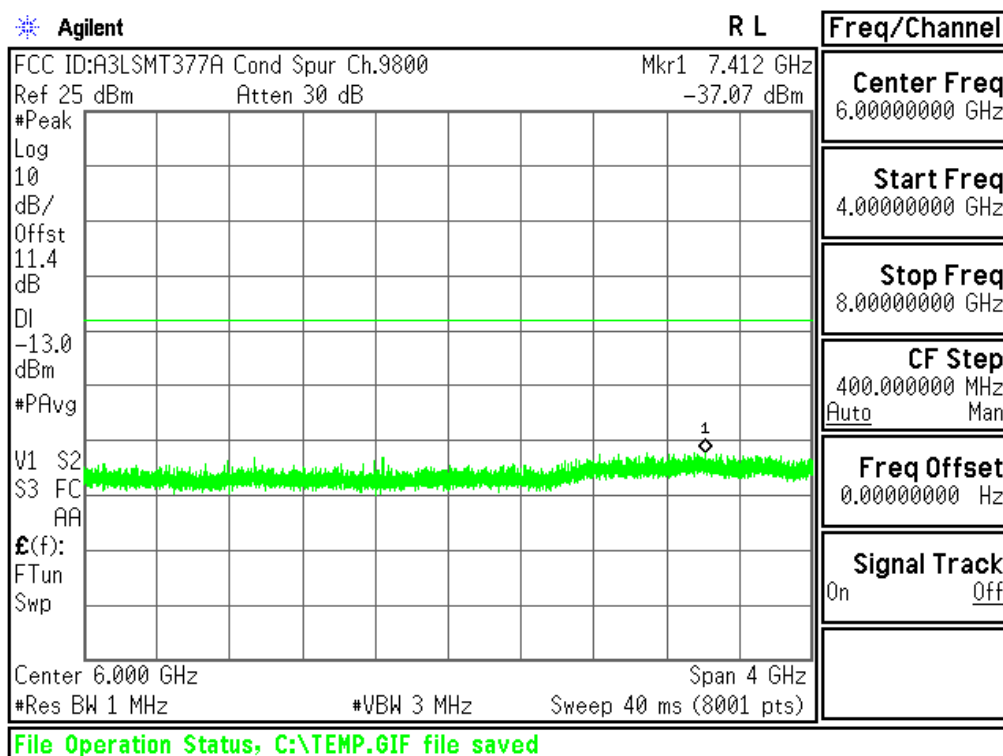
Plot 6-18. Conducted Spurious Plot (PCS WCDMA Mode - Ch.9400(DL9800))
