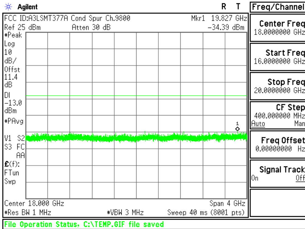
Plot 6-21. Conducted Spurious Plot (PCS WCDMA Mode - Ch.9400(DL9800))
