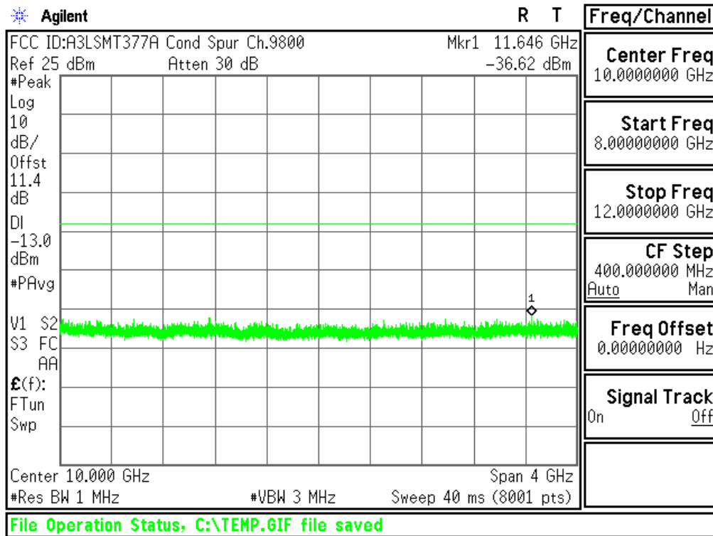
Plot 6-19. Conducted Spurious Plot (PCS WCDMA Mode - Ch.9400(DL9800))
