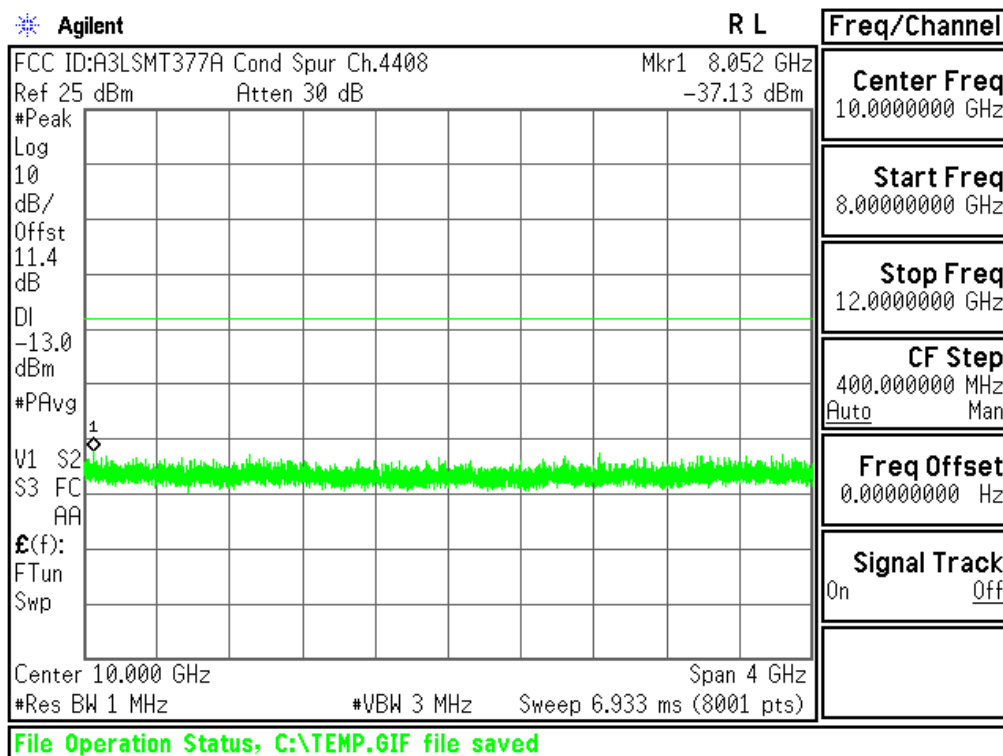
Plot 6-8. Conducted Spurious Plot (Cellular WCDMA Mode - Ch.4183(DL4408))
