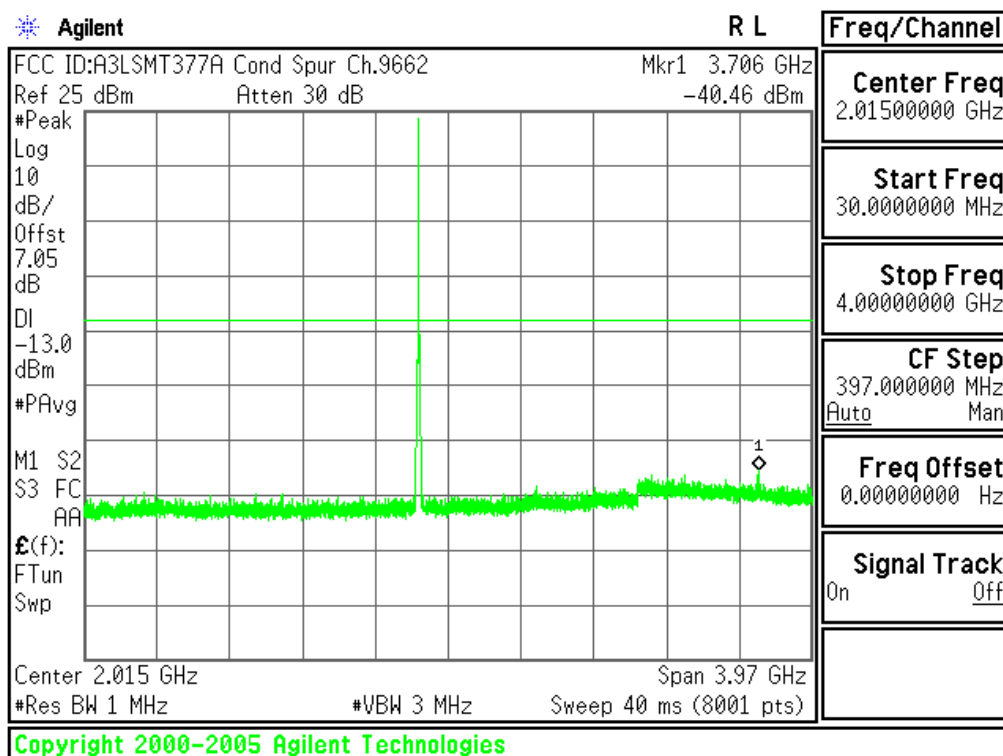
Plot 6-12. Conducted Spurious Plot (PCS WCDMA Mode - Ch.9262(DL9662))
