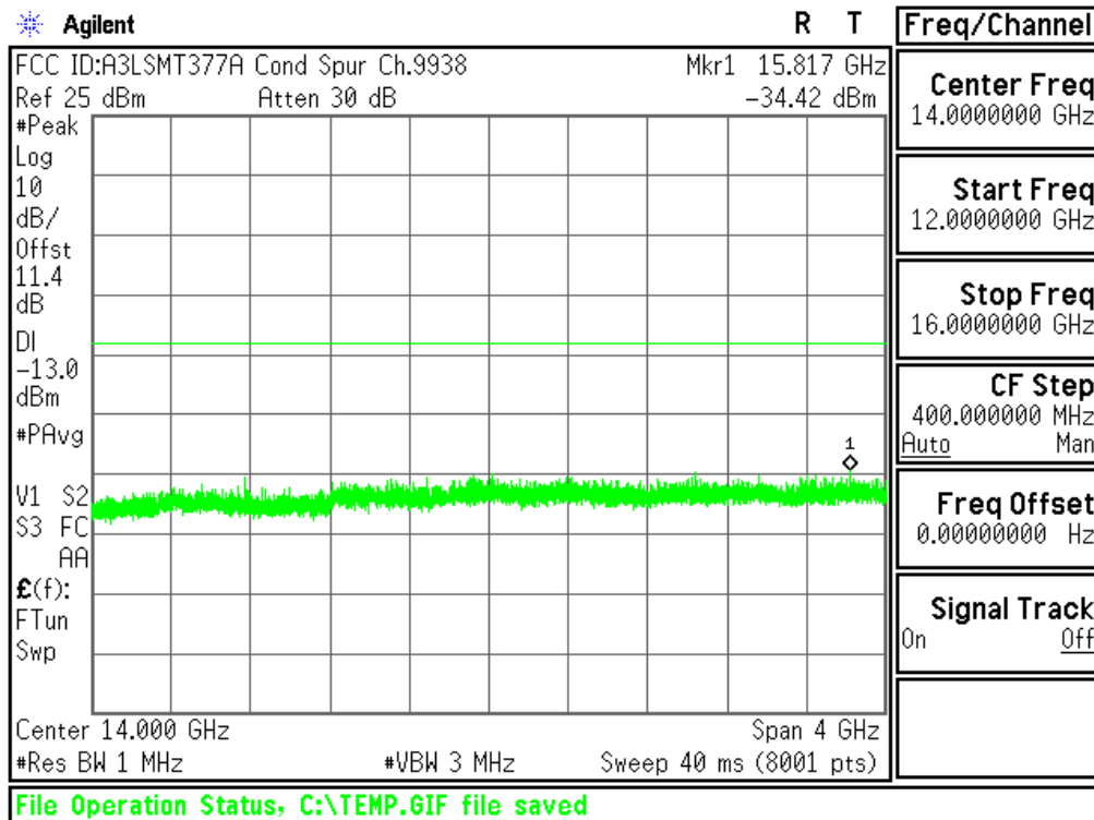
Plot 6-25. Conducted Spurious Plot (PCS WCDMA Mode - Ch.9538(DL9938))
