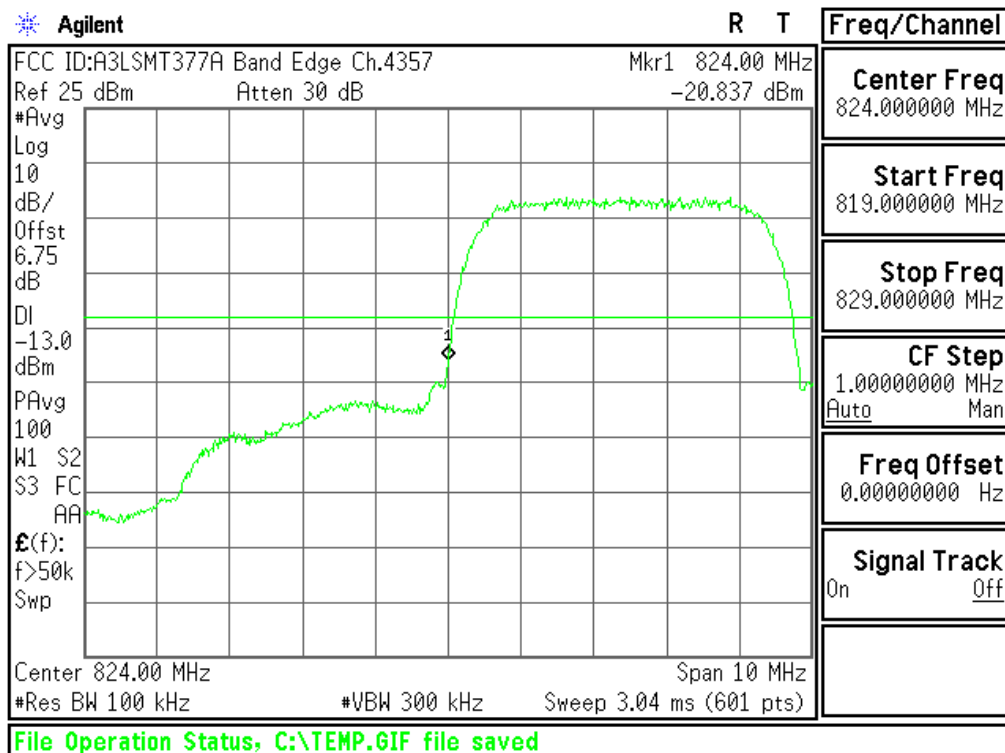
Plot 6-27. Lower Band Edge Plot (Cellular WCDMA Mode - Ch.4132(DL4357))
