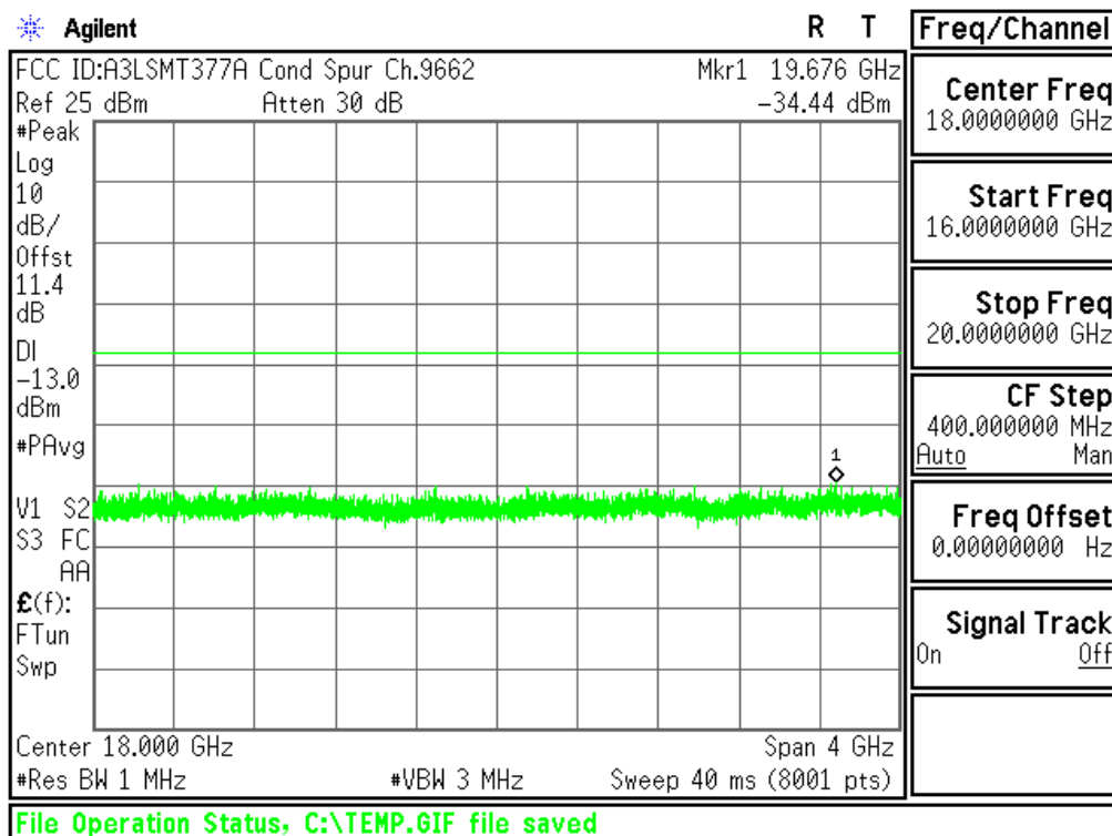
Plot 6-16. Conducted Spurious Plot (PCS WCDMA Mode - Ch.9262(DL9662))
