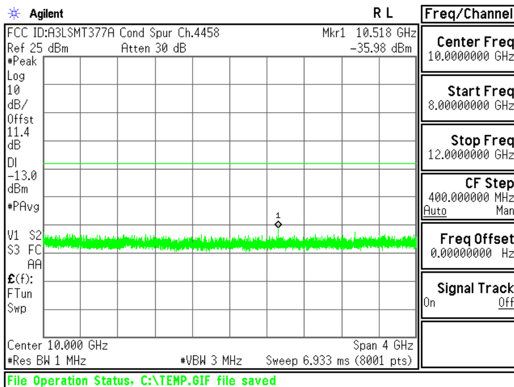
Plot 6-11. Conducted Spurious Plot (Cellular WCDMA Mode - Ch.4233(DL4458))
