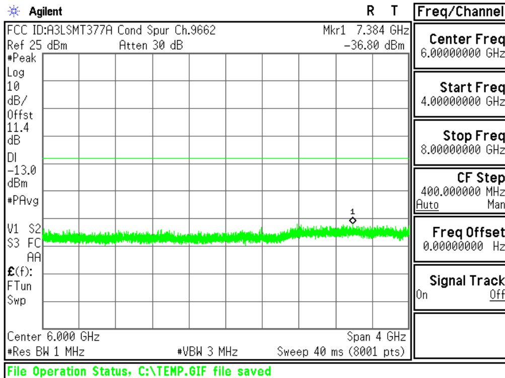
Plot 6-13. Conducted Spurious Plot (PCS WCDMA Mode - Ch.9262(DL9662))
