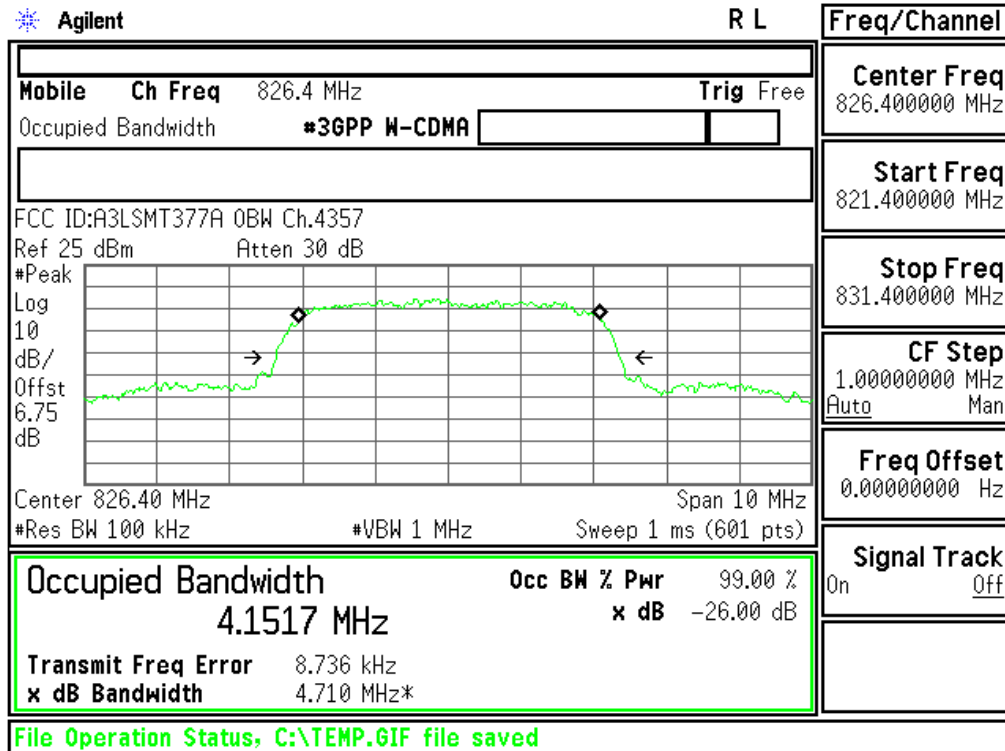
Plot 6-1. Occupied Bandwidth Plot (Cellular WCDMA Mode - Ch.4132(DL4357))
