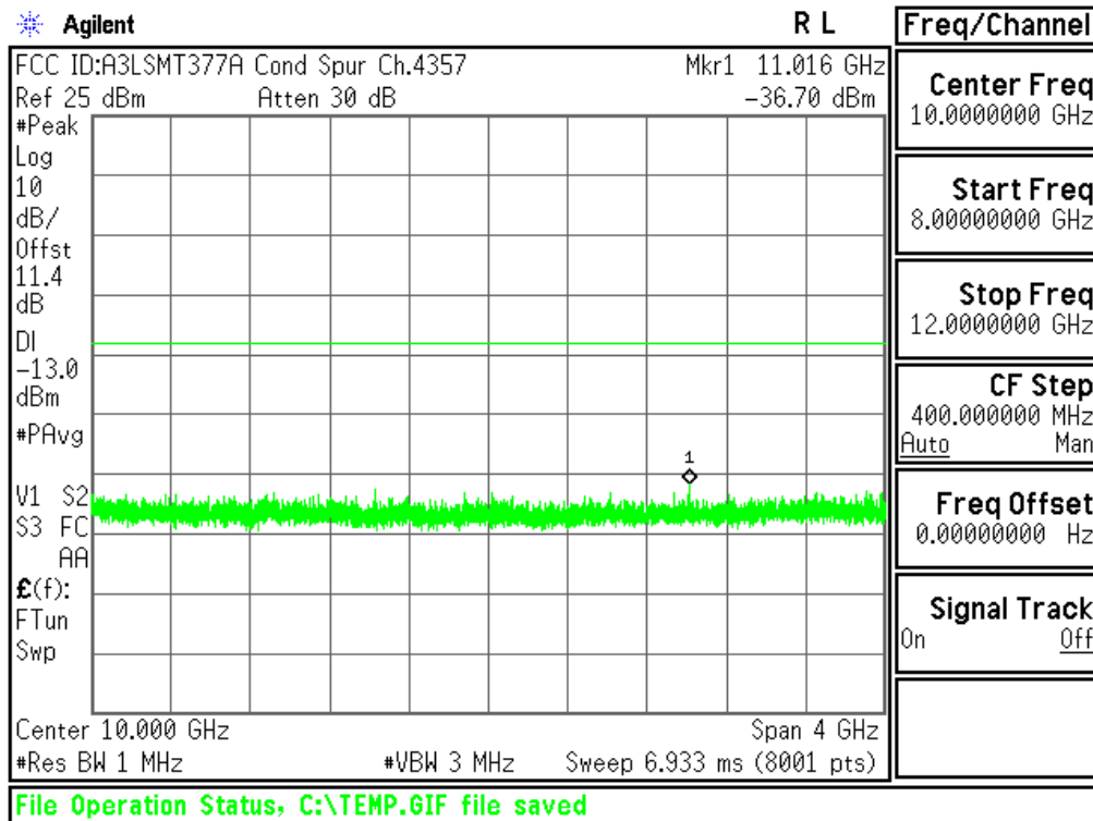
Plot 6-5. Conducted Spurious Plot (Cellular WCDMA Mode - Ch.4132(DL4357))
