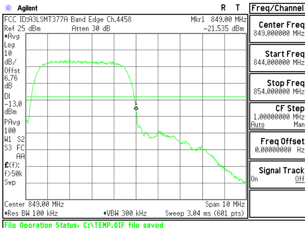
Plot 6-28. Upper Band Edge Plot (Cellular WCDMA Mode - Ch.4233(DL4458))
