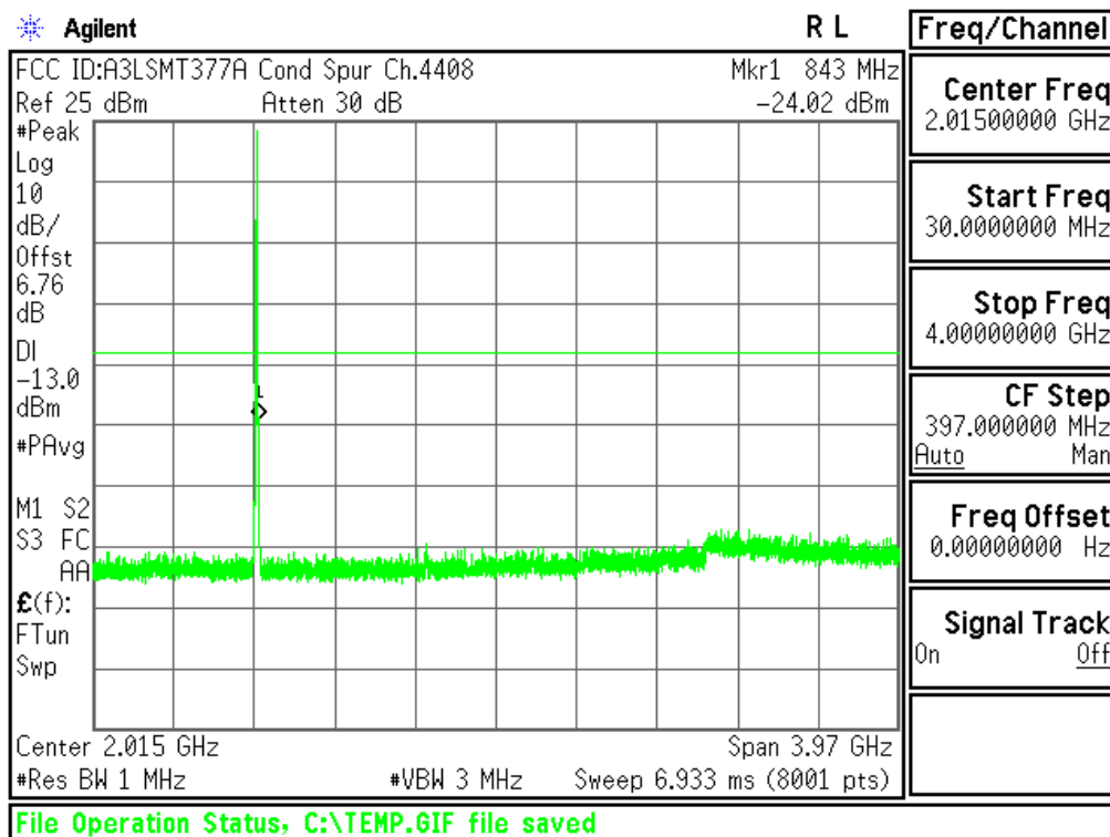
Plot 6-6. Conducted Spurious Plot (Cellular WCDMA Mode - Ch.4183(DL4408))
