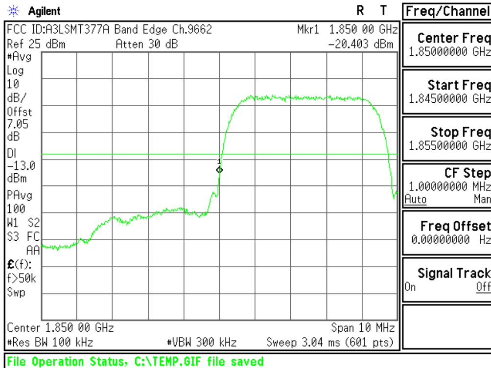
Plot 6-29. Lower Band Edge Plot (PCS WCDMA Mode - Ch.9262(DL9662))
