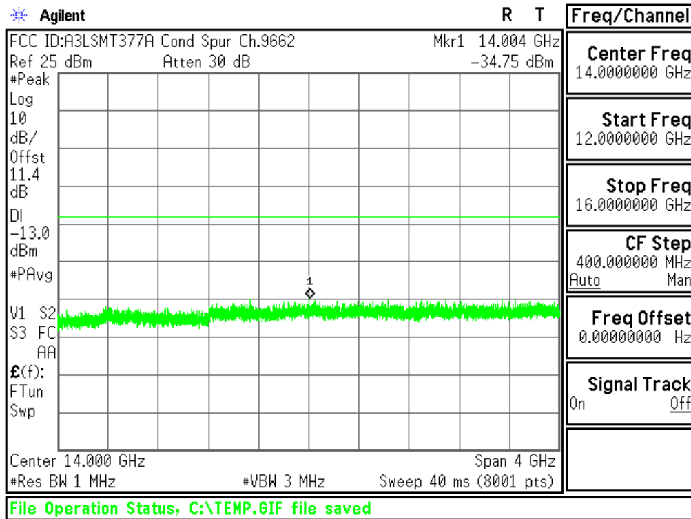
Plot 6-15. Conducted Spurious Plot (PCS WCDMA Mode - Ch.9262(DL9662))
