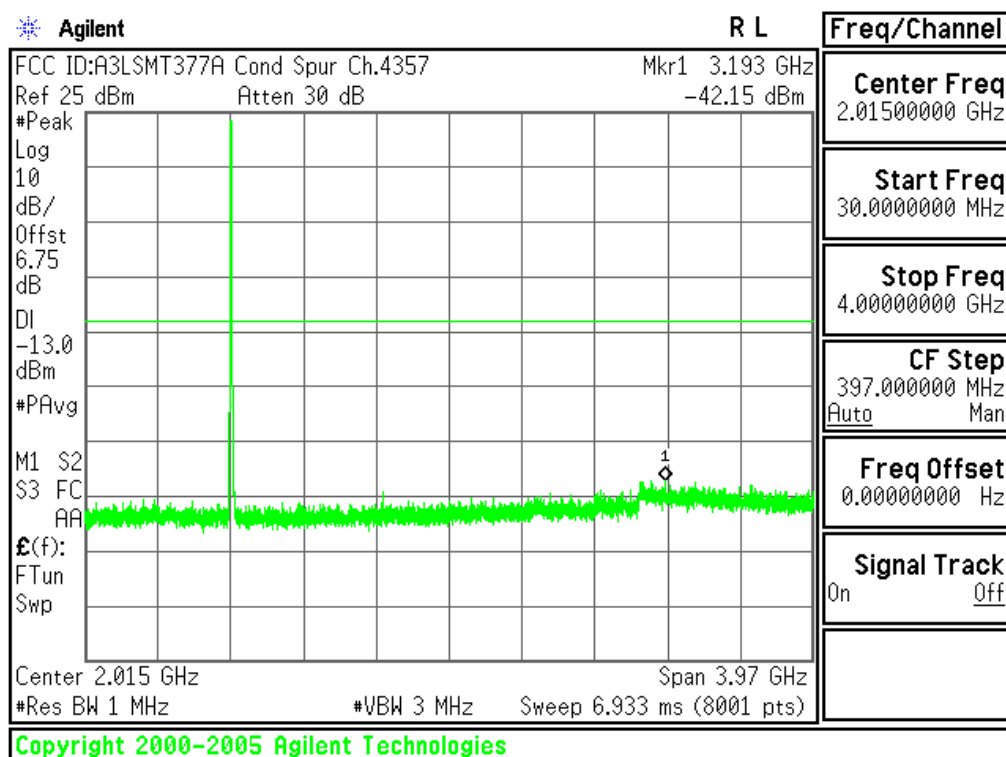
Plot 6-3. Conducted Spurious Plot (Cellular WCDMA Mode - Ch.4132(DL4357))
