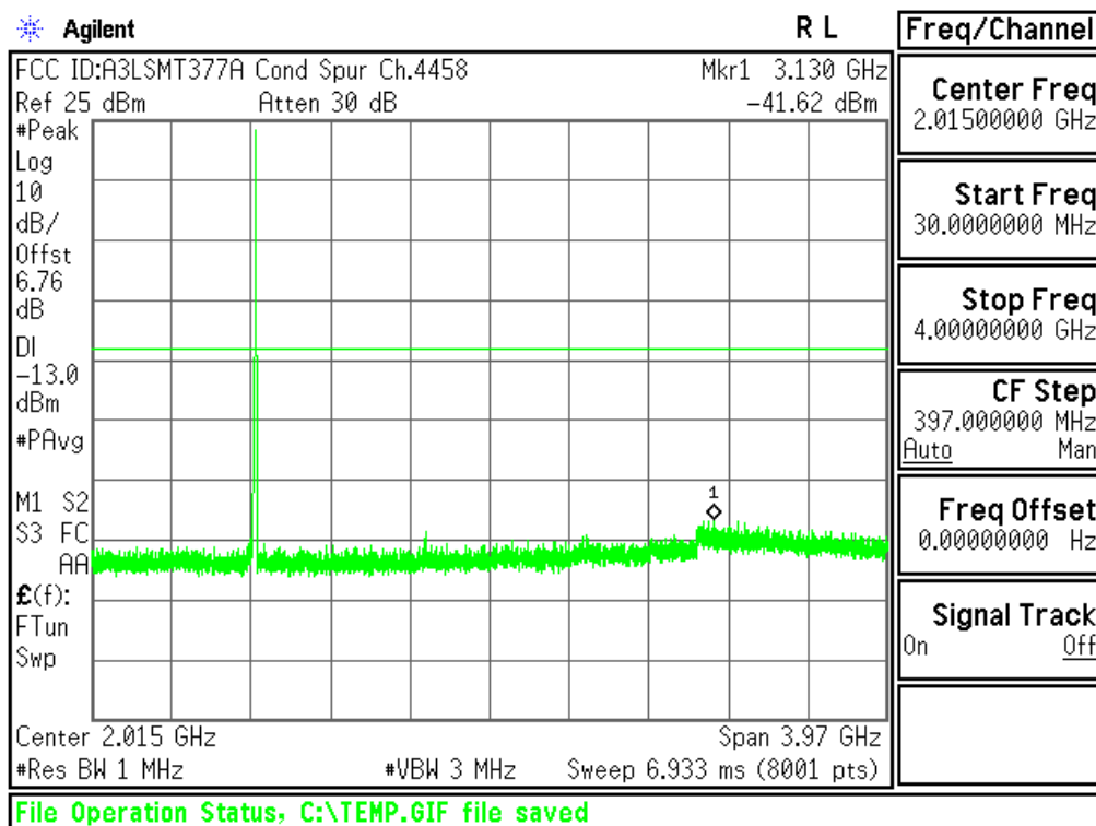
Plot 6-9. Conducted Spurious Plot (Cellular WCDMA Mode - Ch.4233(DL4458))
