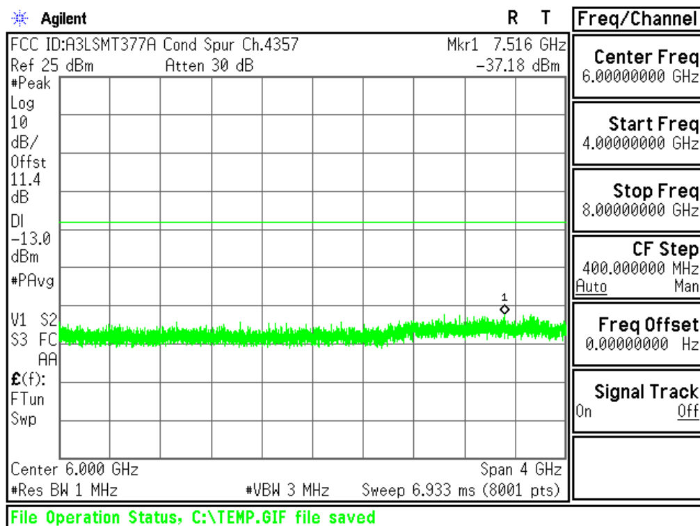
Plot 6-4. Conducted Spurious Plot (Cellular WCDMA Mode - Ch.4132(DL4357))
