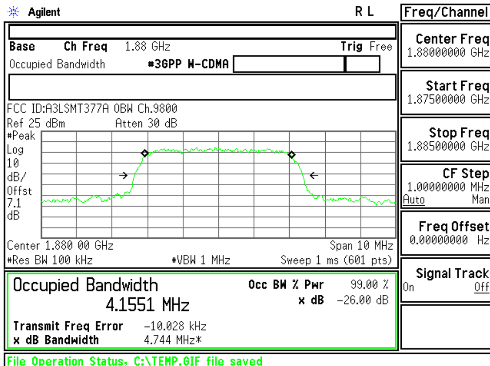
Plot 6-2. Occupied Bandwidth Plot (PCS WCDMA Mode - Ch.9400(DL9800))
