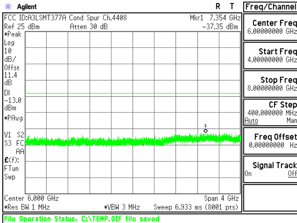
Plot 6-7. Conducted Spurious Plot (Cellular WCDMA Mode - Ch.4183(DL4408))
