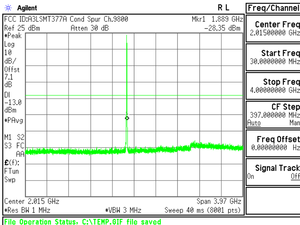
Plot 6-17. Conducted Spurious Plot (PCS WCDMA Mode - Ch.9400(DL9800))
