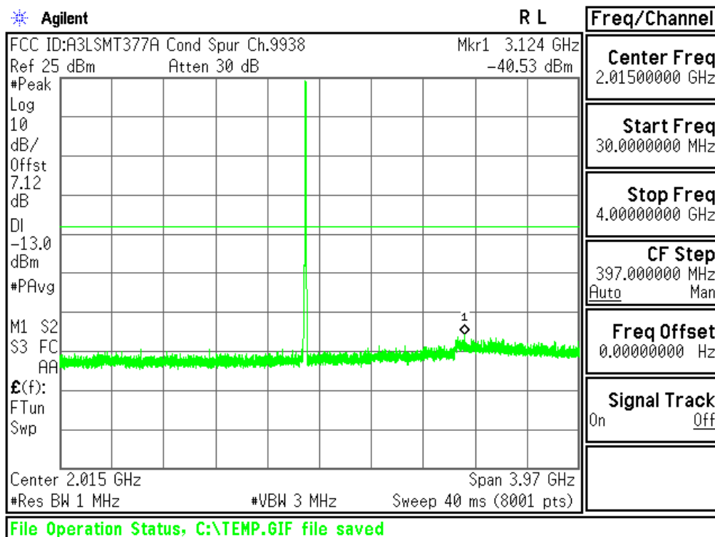
Plot 6-22. Conducted Spurious Plot (PCS WCDMA Mode - Ch.9538(DL9938))
