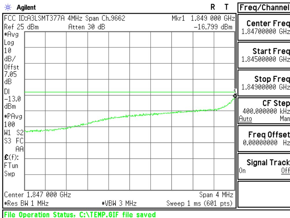
Plot 6-30. Extended Lower Band Edge Plot (PCS WCDMA Mode - Ch.9262(DL9662))
