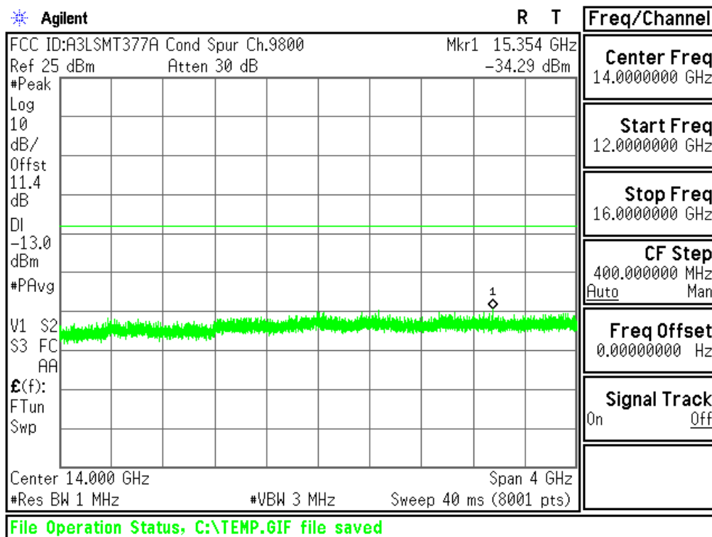
Plot 6-20. Conducted Spurious Plot (PCS WCDMA Mode - Ch.9400(DL9800))
