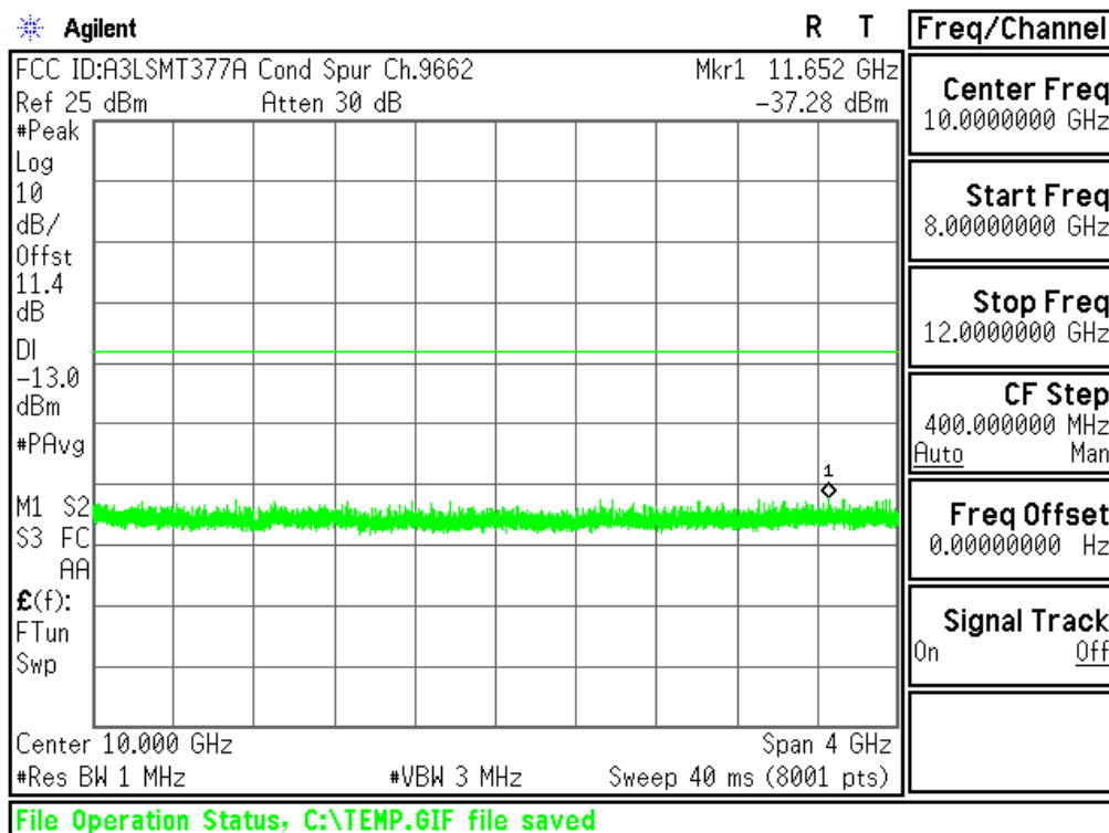
Plot 6-14. Conducted Spurious Plot (PCS WCDMA Mode - Ch.9262(DL9662))
