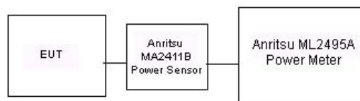
Figure 8-2 Power Measurement Setup
