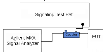
Figure 6-2. Test Instrument & Measurement Setup
