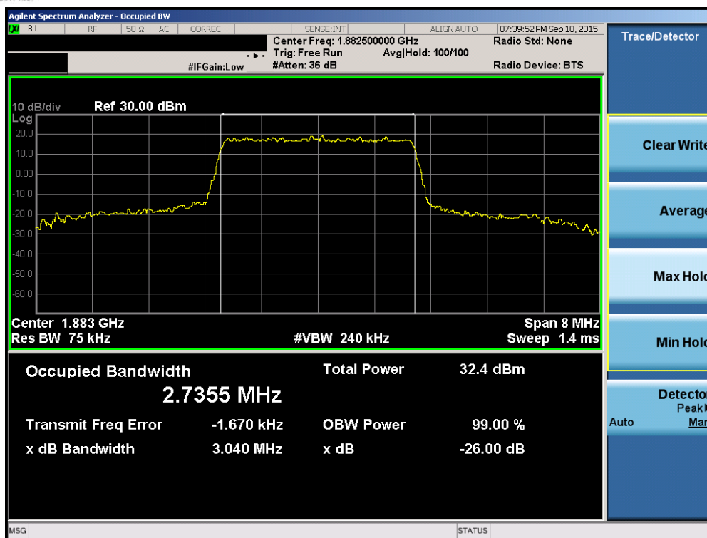
Plot 6-33. Occupied Bandwidth Plot (Band 2/25 – 3.0MHz QPSK – RB Size 15)
