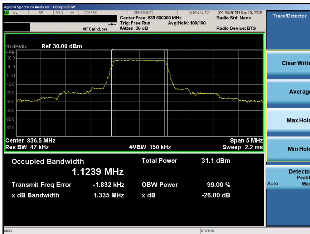
Plot 6-9. Occupied Bandwidth Plot (Band 5/26 – 1.4MHz QPSK – RB Size 6)
