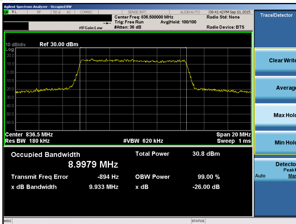
Plot 6-15. Occupied Bandwidth Plot (Band 5/26 – 10.0MHz QPSK – RB Size 50)
