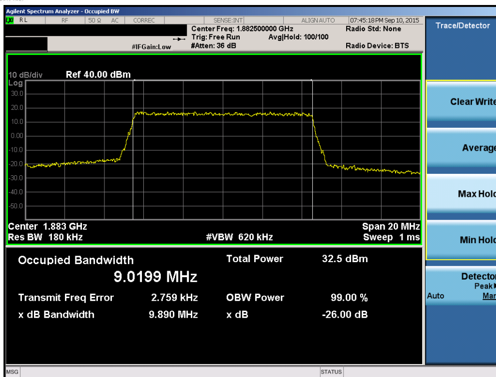
Plot 6-37. Occupied Bandwidth Plot (Band 2/25 – 10.0MHz QPSK – RB Size 50)
