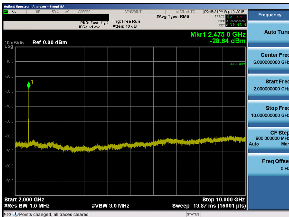
Plot 6-62. Conducted Spurious Plot (Band 5/26 – 10.0MHz QPSK – RB Size 1, RB Offset 0 – Low Channel)
