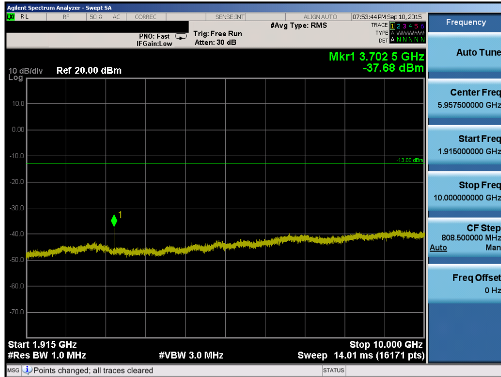
Plot 6-79. Conducted Spurious Plot (Band 2/25 – 20.0MHz QPSK – RB Size 1, RB Offset 0 – Low Channel)
