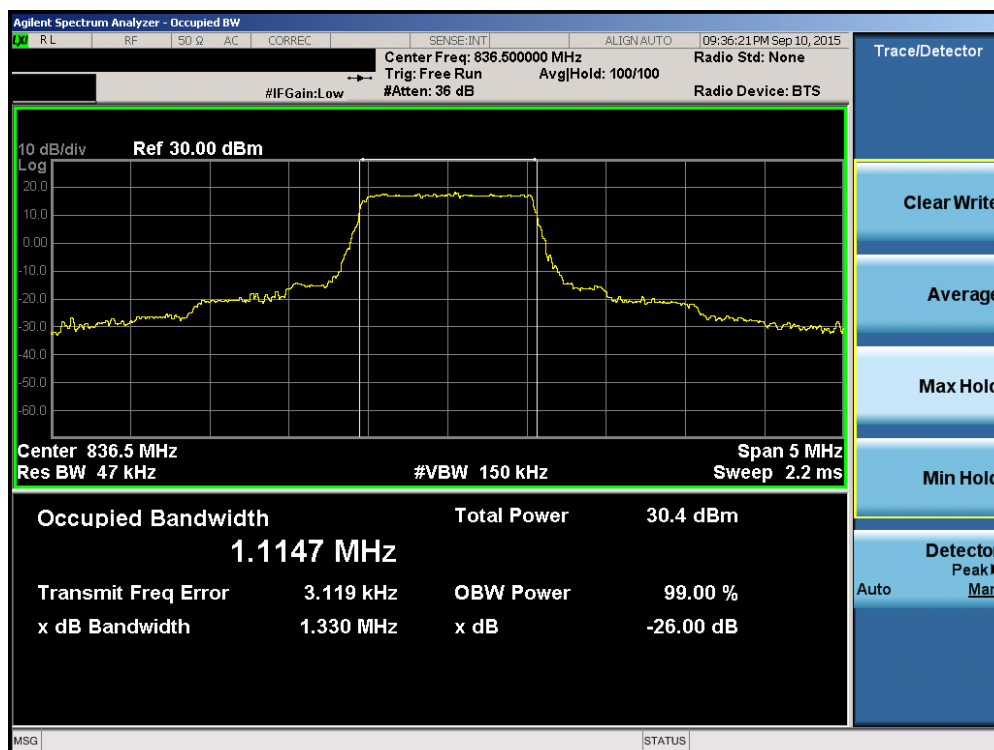
Plot 6-10. Occupied Bandwidth Plot (Band 5/26 – 1.4MHz 16-QAM – RB Size 6)
