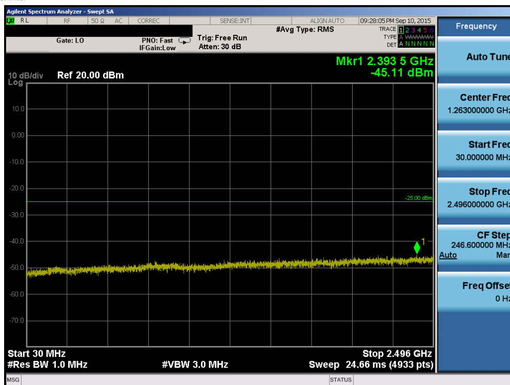
Plot 6-93. Conducted Spurious Plot (Band 41 – 20.0MHz QPSK – RB Size 1, RB Offset 0 – High Channel)
