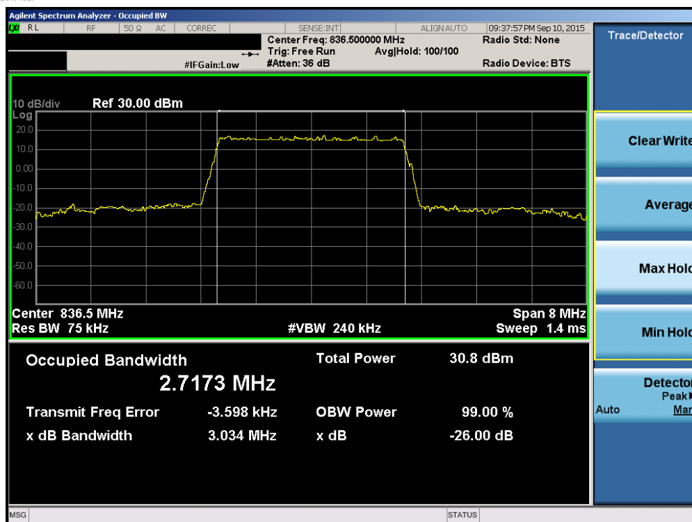
Plot 6-11. Occupied Bandwidth Plot (Band 5/26 – 3.0MHz QPSK – RB Size 15)
