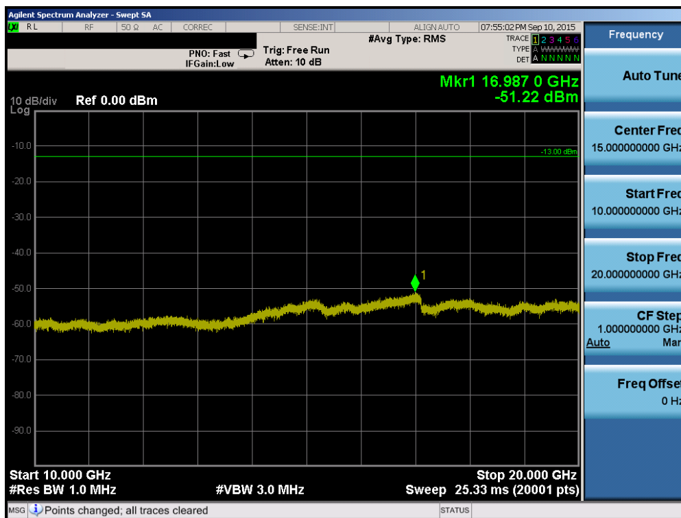
Plot 6-86. Conducted Spurious Plot (Band 2/25 – 20.0MHz QPSK – RB Size 1, RB Offset 0 – High Channel)
