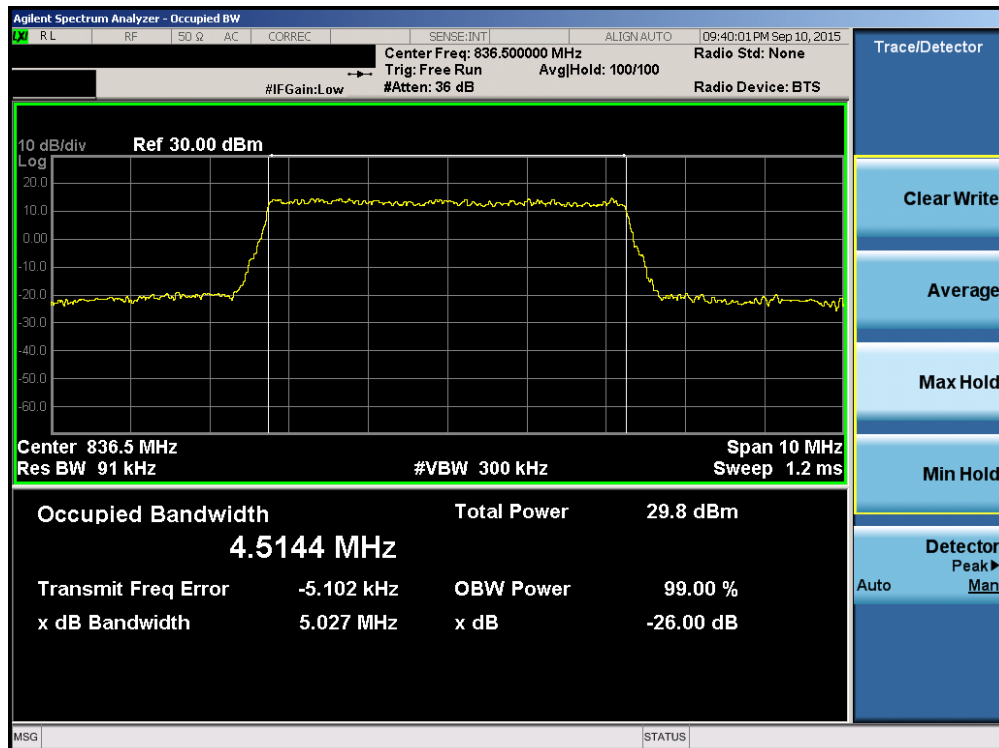
Plot 6-14. Occupied Bandwidth Plot (Band 5/26 – 5.0MHz 16-QAM – RB Size 25)
