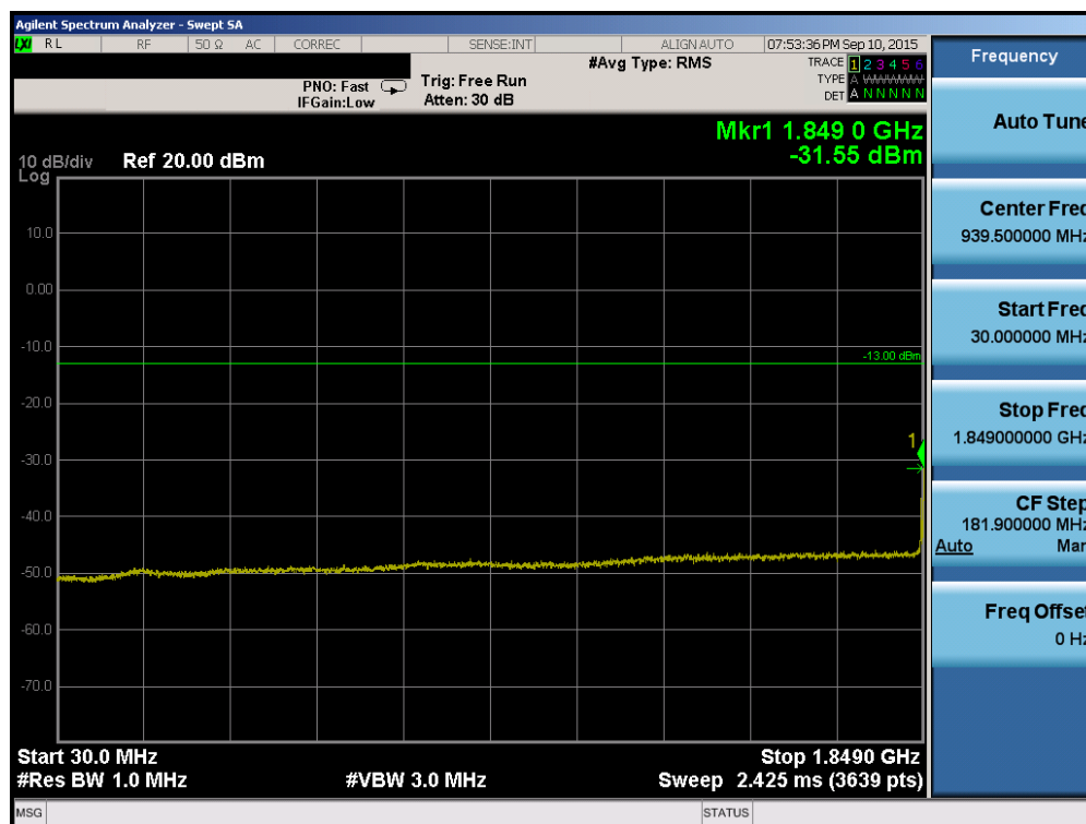
Plot 6-78. Conducted Spurious Plot (Band 2/25 – 20.0MHz QPSK – RB Size 1, RB Offset 0– Low Channel)
