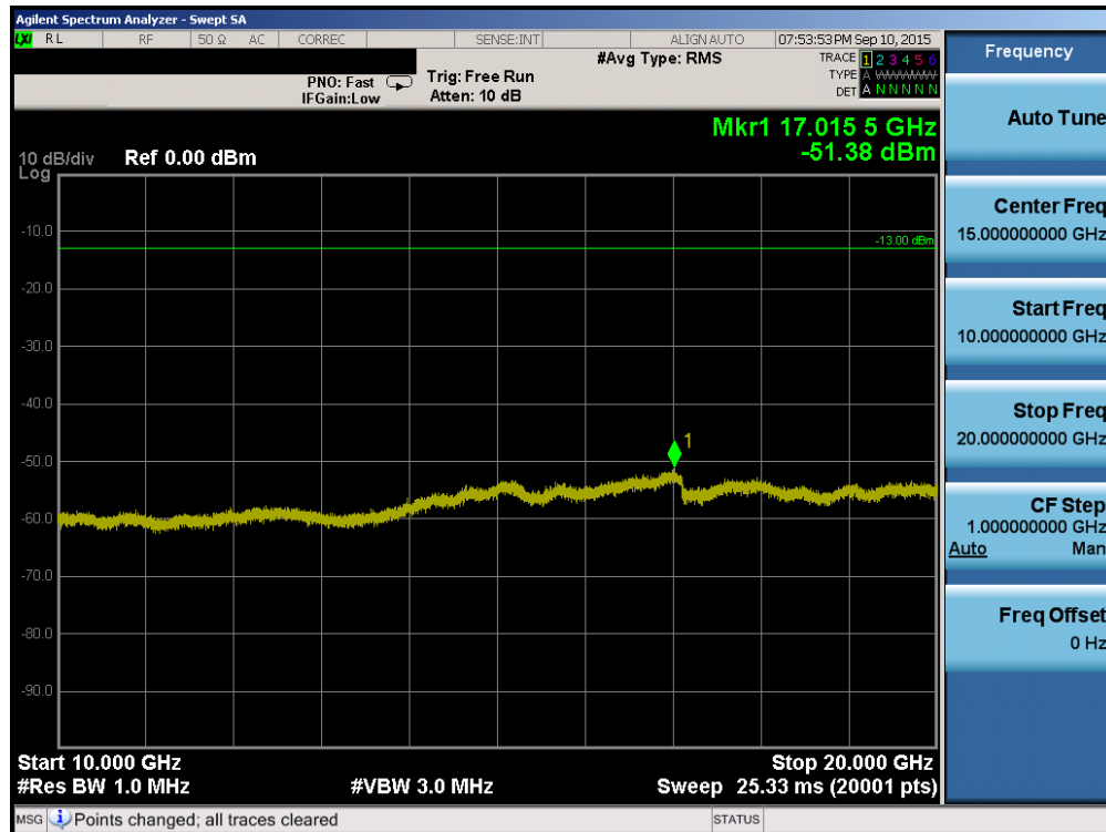
Plot 6-80. Conducted Spurious Plot (Band 2/25 – 20.0MHz QPSK – RB Size 1, RB Offset 0 – Low Channel)
