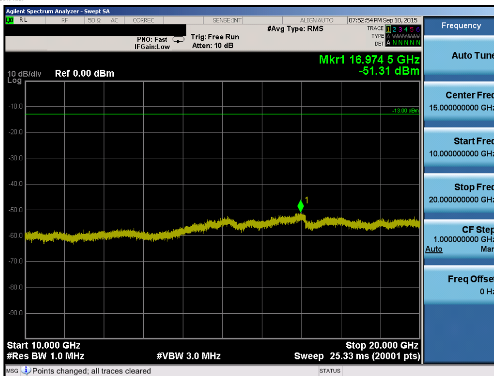
Plot 6-83. Conducted Spurious Plot (Band 2/25 – 20.0MHz QPSK – RB Size 1, RB Offset 0 – Mid Channel)
