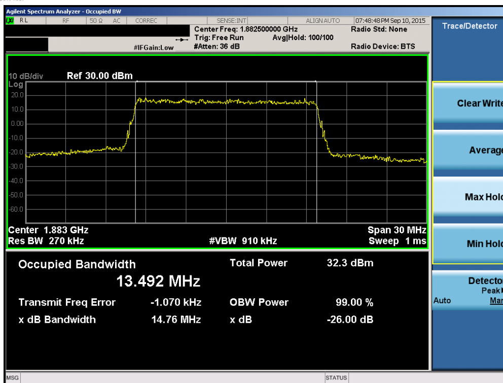
Plot 6-39. Occupied Bandwidth Plot (Band 2/25 – 15.0MHz QPSK – RB Size 75)
