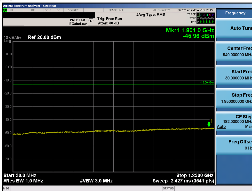
Plot 6-81. Conducted Spurious Plot (Band 2/25 – 20.0MHz QPSK – RB Size 1, RB Offset 0 – Mid Channel)
