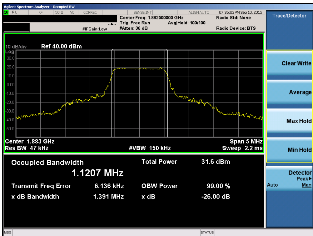
Plot 6-32. Occupied Bandwidth Plot (Band 2/25 – 1.4MHz 16-QAM – RB Size 6)
