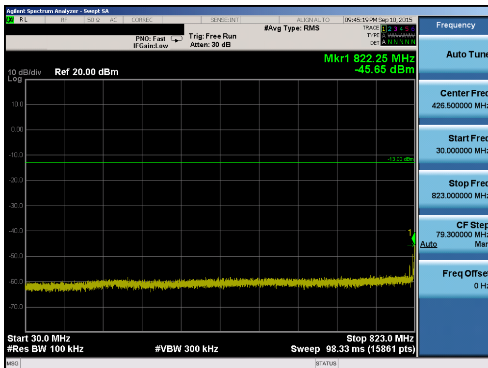
Plot 6-60. Conducted Spurious Plot (Band 5/26 – 10.0MHz QPSK – RB Size 1, RB Offset 0 – Low Channel)
