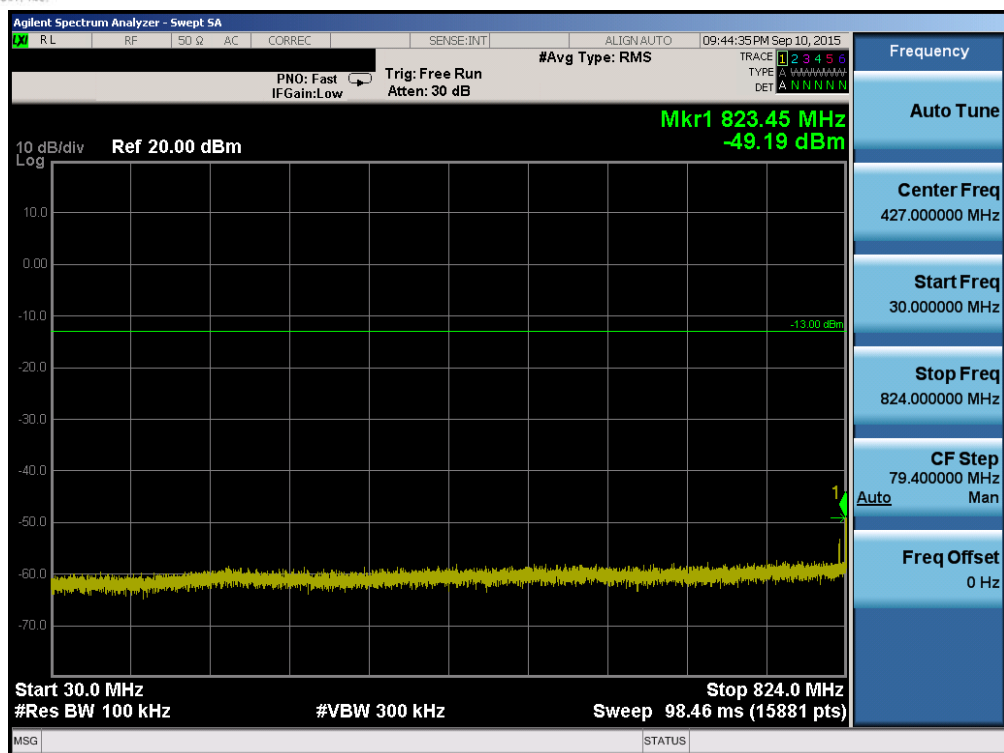
Plot 6-63. Conducted Spurious Plot (Band 5/26 – 10.0MHz QPSK – RB Size 1, RB Offset 0 – Mid Channel)
