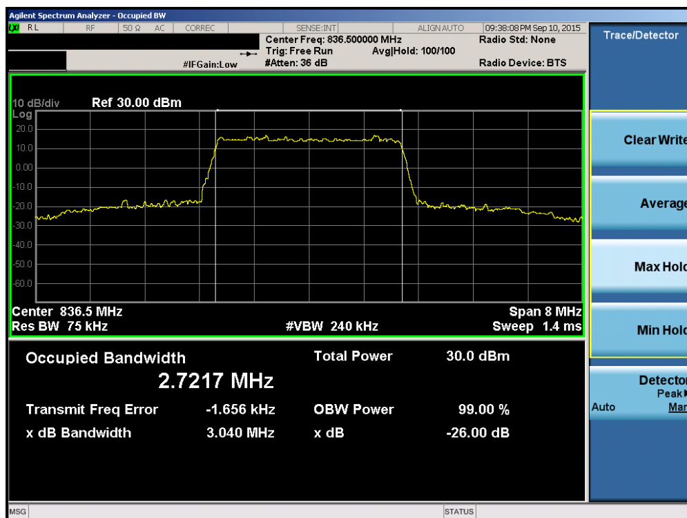
Plot 6-12. Occupied Bandwidth Plot (Band 5/26 – 3.0MHz 16-QAM – RB Size 15)
