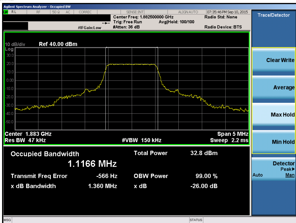
Plot 6-31. Occupied Bandwidth Plot (Band 2/25 – 1.4MHz QPSK – RB Size 6)
