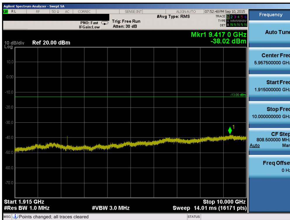
Plot 6-82. Conducted Spurious Plot (Band 2/25 – 20.0MHz QPSK – RB Size 1, RB Offset 0 – Mid Channel)
