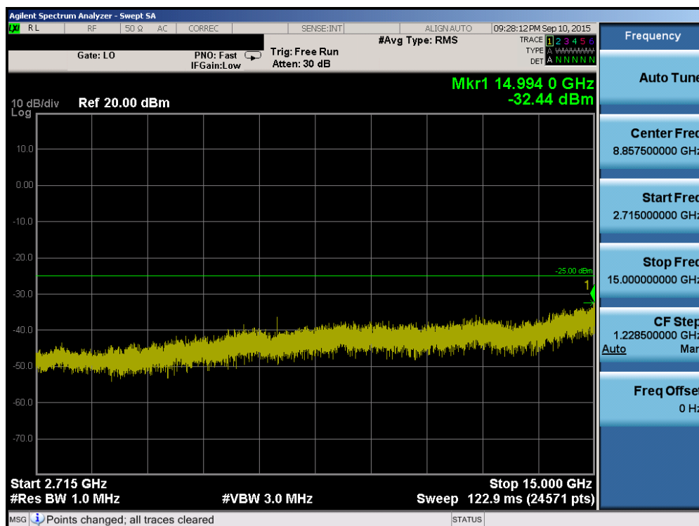
Plot 6-94. Conducted Spurious Plot (Band 41 – 20.0MHz QPSK – RB Size 1, RB Offset 0 – High Channel)
