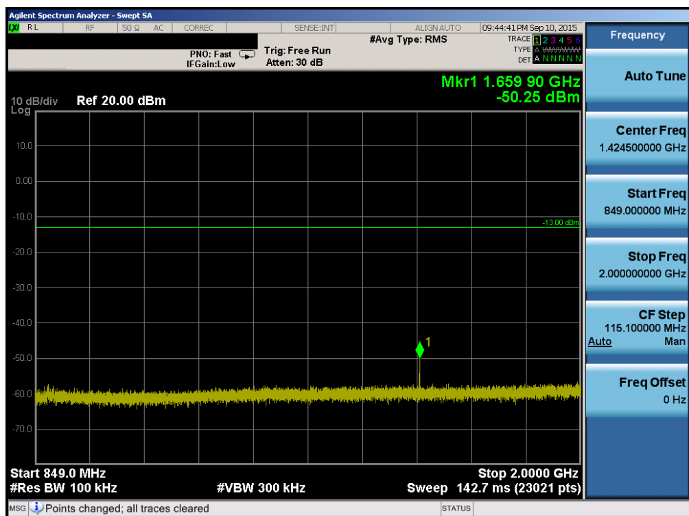
Plot 6-64. Conducted Spurious Plot (Band 5/26 – 10.0MHz QPSK – RB Size 1, RB Offset 0 – Mid Channel)
