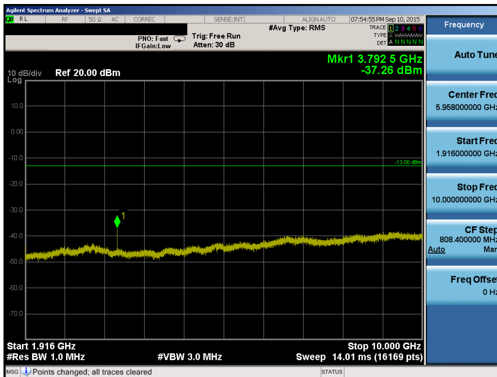
Plot 6-85. Conducted Spurious Plot (Band 2/25 – 20.0MHz QPSK – RB Size 1, RB Offset 0 – High Channel)
