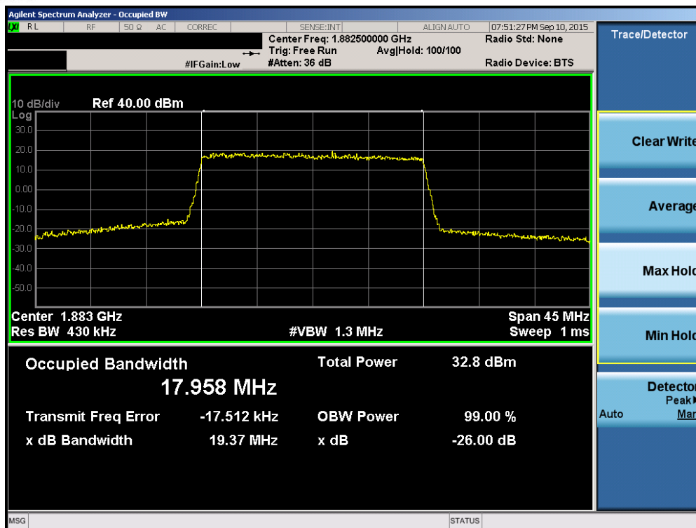
Plot 6-41. Occupied Bandwidth Plot (Band 2/25 – 20.0MHz QPSK – RB Size 100)
