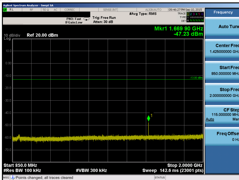
Plot 6-67. Conducted Spurious Plot (Band 5/26 – 10.0MHz QPSK – RB Size 1, RB Offset 0 – High Channel)
