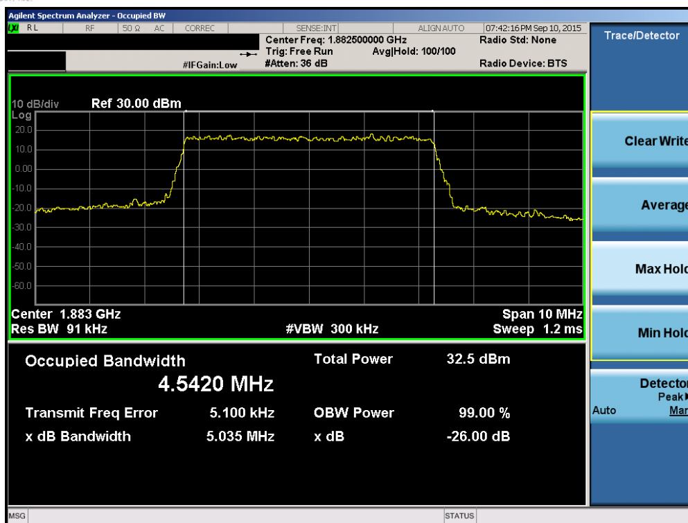
Plot 6-35. Occupied Bandwidth Plot (Band 2/25 – 5.0MHz QPSK – RB Size 25)
