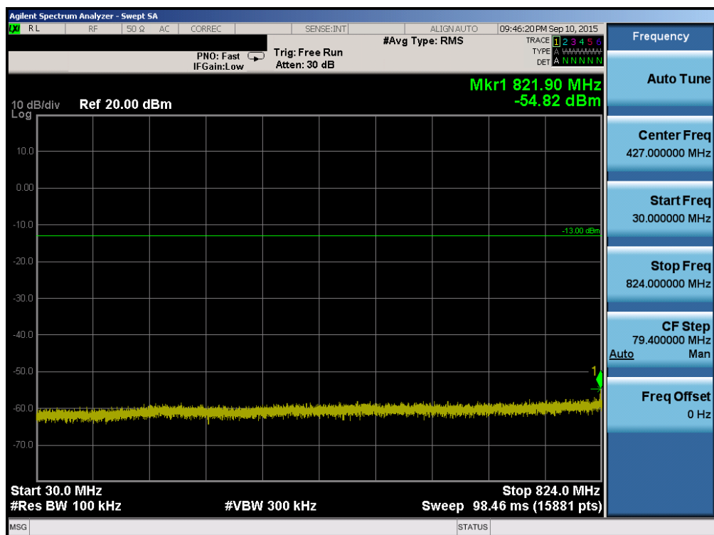
Plot 6-66. Conducted Spurious Plot (Band 5/26 – 10.0MHz QPSK – RB Size 1, RB Offset 0 – High Channel)
