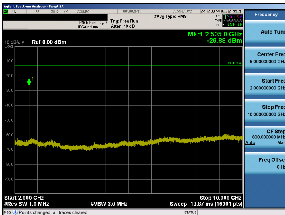
Plot 6-68. Conducted Spurious Plot (Band 5/26 – 10.0MHz QPSK – RB Size 1, RB Offset 0 – High Channel)
