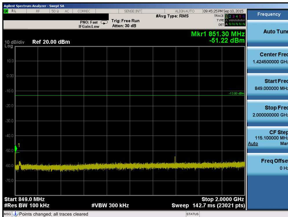
Plot 6-61. Conducted Spurious Plot (Band 5/26 – 10.0MHz QPSK – RB Size 1, RB Offset 0 – Low Channel)
