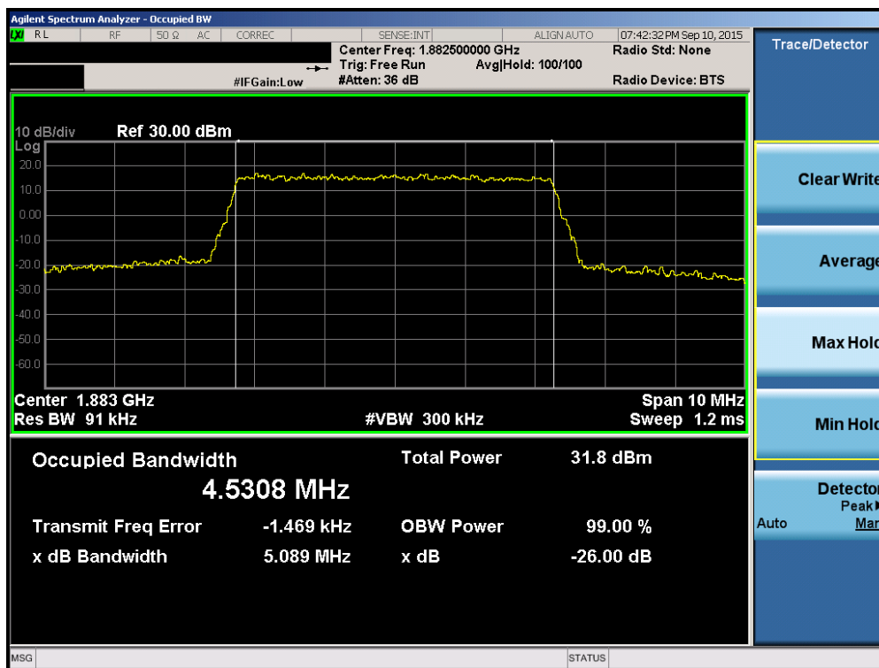
Plot 6-36. Occupied Bandwidth Plot (Band 2/25 – 5.0MHz 16-QAM – RB Size 25)
