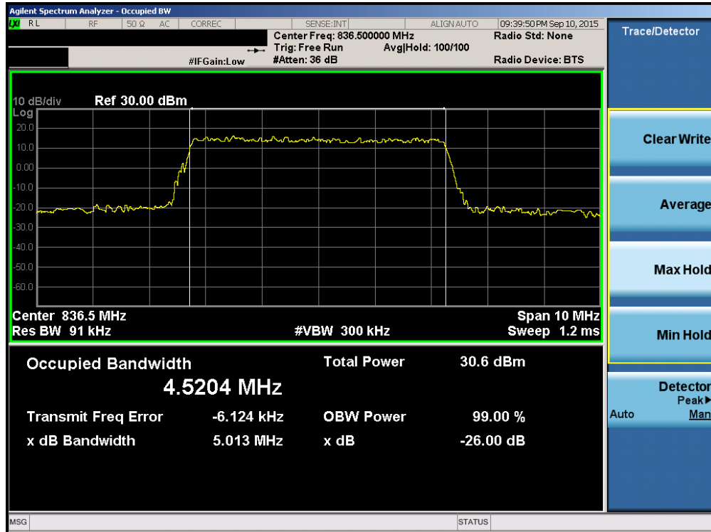
Plot 6-13. Occupied Bandwidth Plot (Band 5/26 – 5.0MHz QPSK – RB Size 25)
