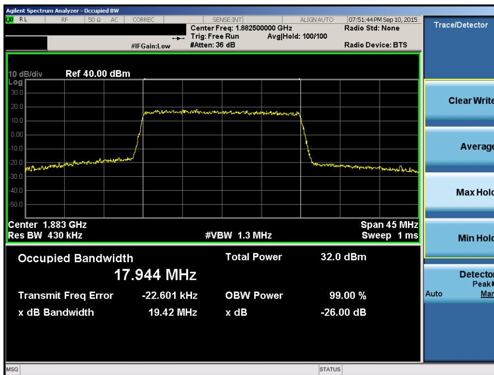
Plot 6-42. Occupied Bandwidth Plot (Band 2/25 – 20.0MHz 16-QAM – RB Size 100)
