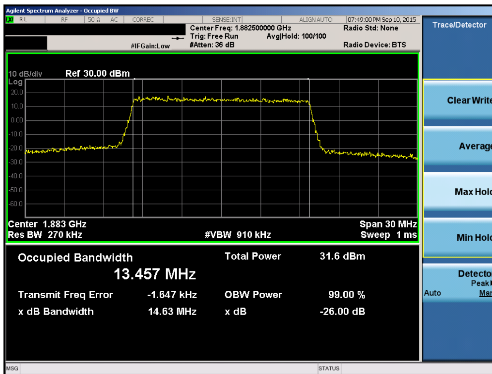
Plot 6-40. Occupied Bandwidth Plot (Band 2/25 – 15.0MHz 16-QAM – RB Size 75)
