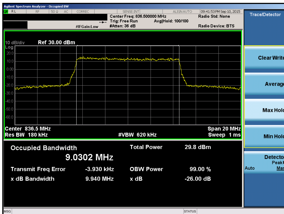
Plot 6-16. Occupied Bandwidth Plot (Band 5/26 – 10.0MHz 16-QAM – RB Size 50)
