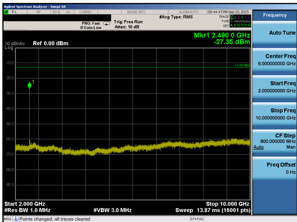
Plot 6-65. Conducted Spurious Plot (Band 5/26 – 10.0MHz QPSK – RB Size 1, RB Offset 0 – Mid Channel)
