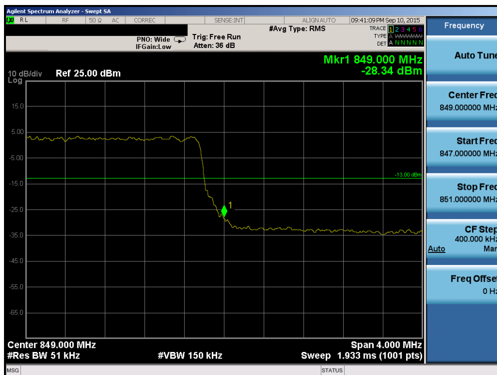
Plot 6-122. Upper Band Edge Plot (Band 5/26 – 5.0MHz QPSK – RB Size 25)
