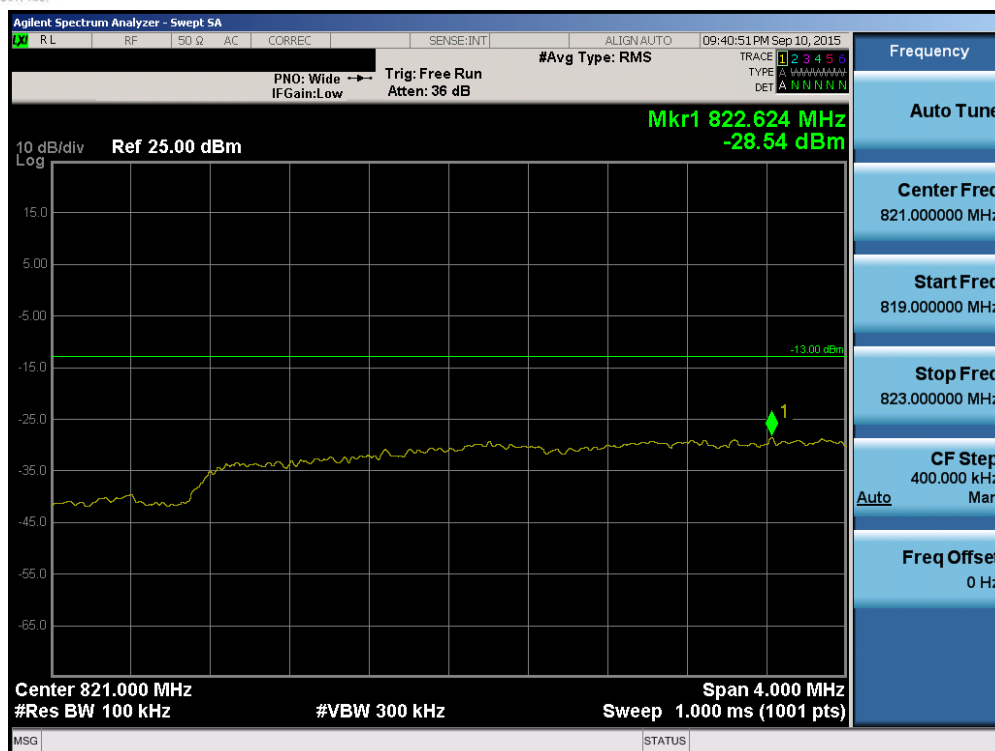
Plot 6-121. Lower Extended Band Edge Plot (Band 5/26 – 5.0MHz QPSK – RB Size 25)
