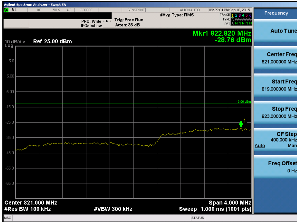
Plot 6-117. Lower Extended Band Edge Plot (Band 5/26 – 3.0MHz QPSK – RB Size 15)
