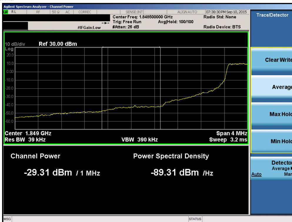
Plot 6-153. Lower Extended Band Edge Plot (Band 2/25 – 1.4MHz QPSK – RB Size 6)
