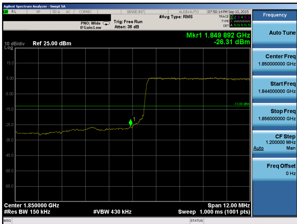
Plot 6-168. Lower Band Edge Plot (Band 2/25 – 15.0MHz QPSK – RB Size 75)
