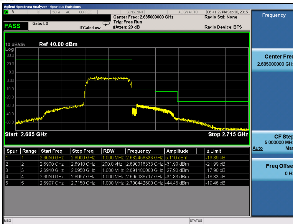
Plot 6-179. Upper ACP Plot (Band 41 – 10.0MHz QPSK – RB Size 50)
