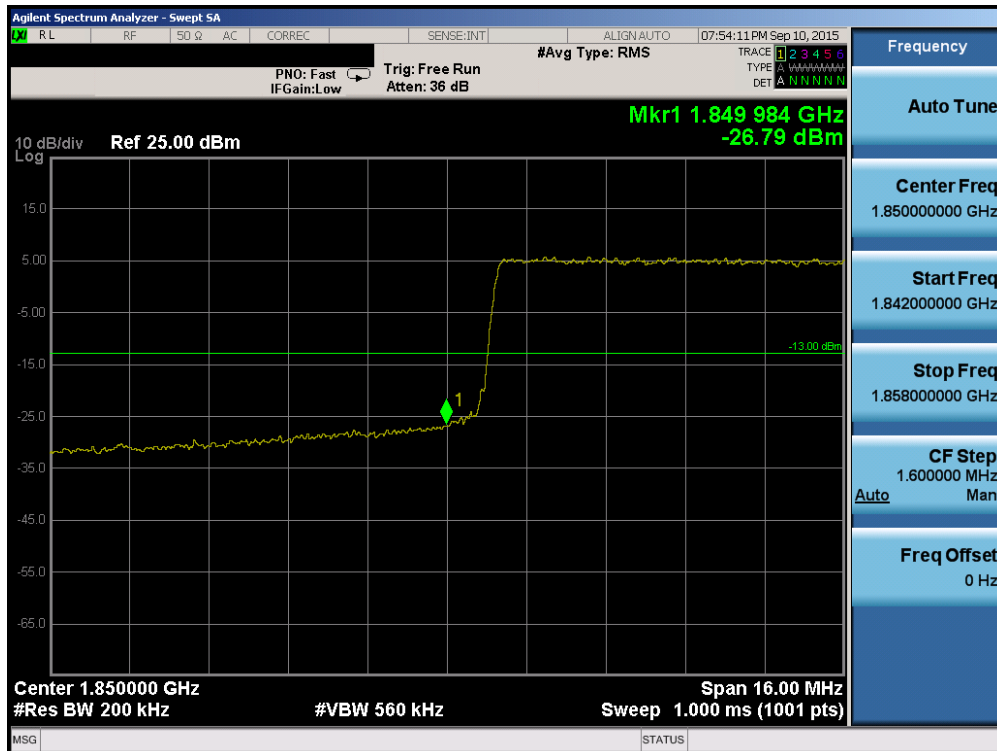
Plot 6-172. Lower Band Edge Plot (Band 2/25 – 20.0MHz QPSK – RB Size 100)
