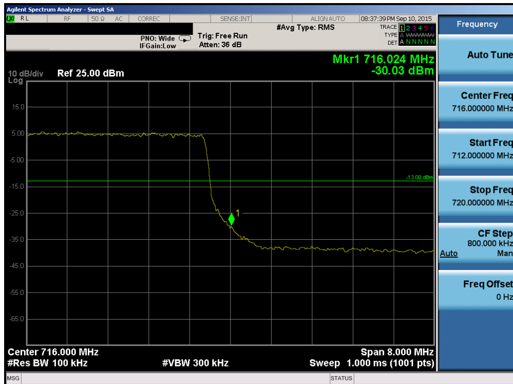
Plot 6-110. Upper Band Edge Plot (Band 12 – 10.0MHz QPSK – RB Size 50)
