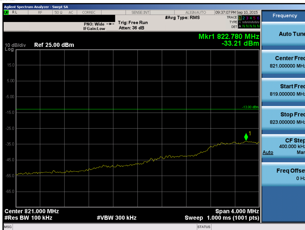
Plot 6-113. Lower Extended Band Edge Plot (Band 5/26 – 1.4MHz QPSK – RB Size 6)
