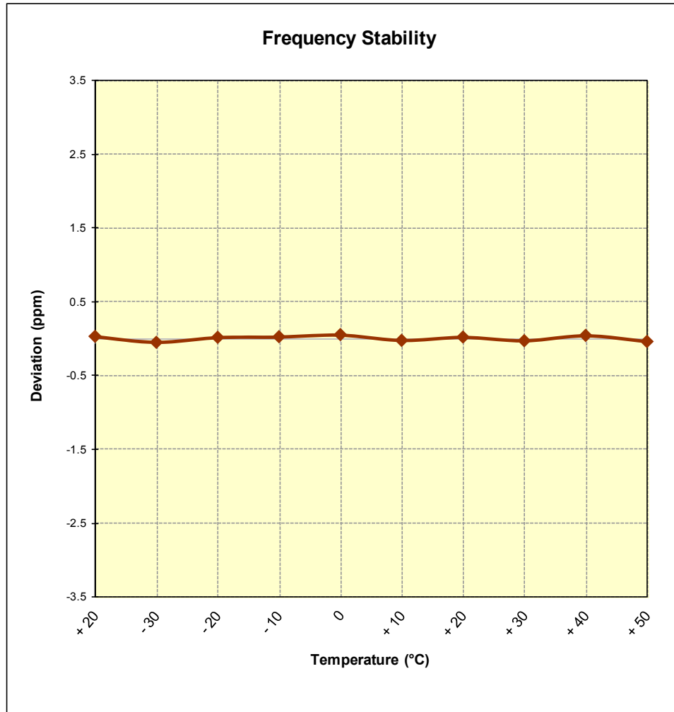
Figure 6-11. Frequency Stability Graph (Band 41)
