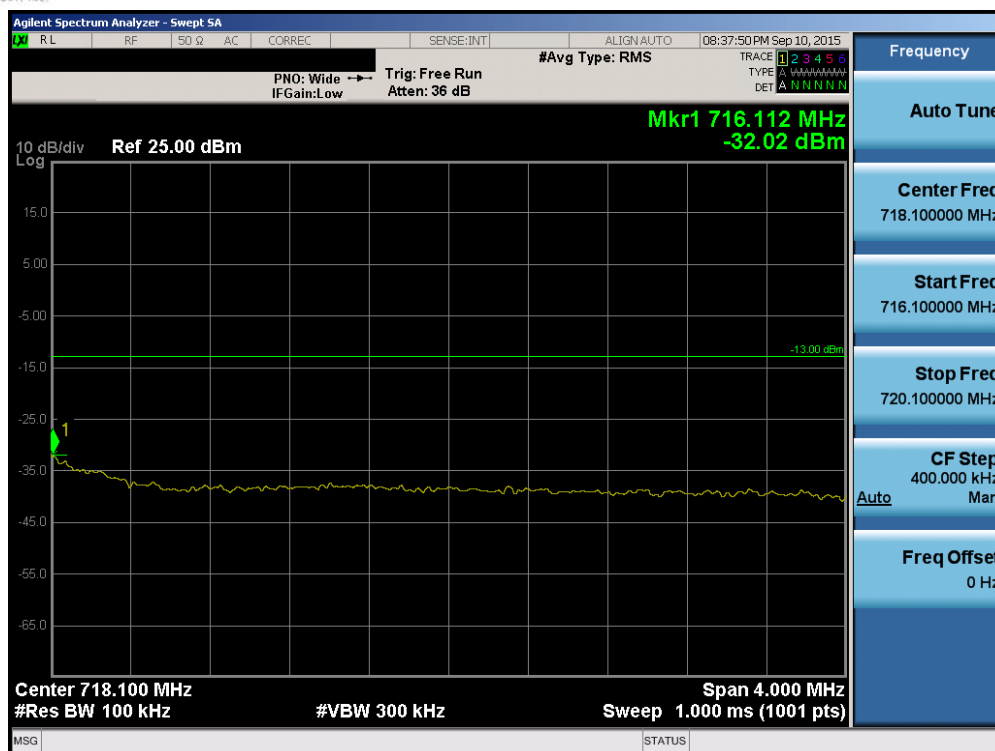
Plot 6-111. Upper Extended Band Edge Plot (Band 12 – 10.0MHz QPSK – RB Size 50)
