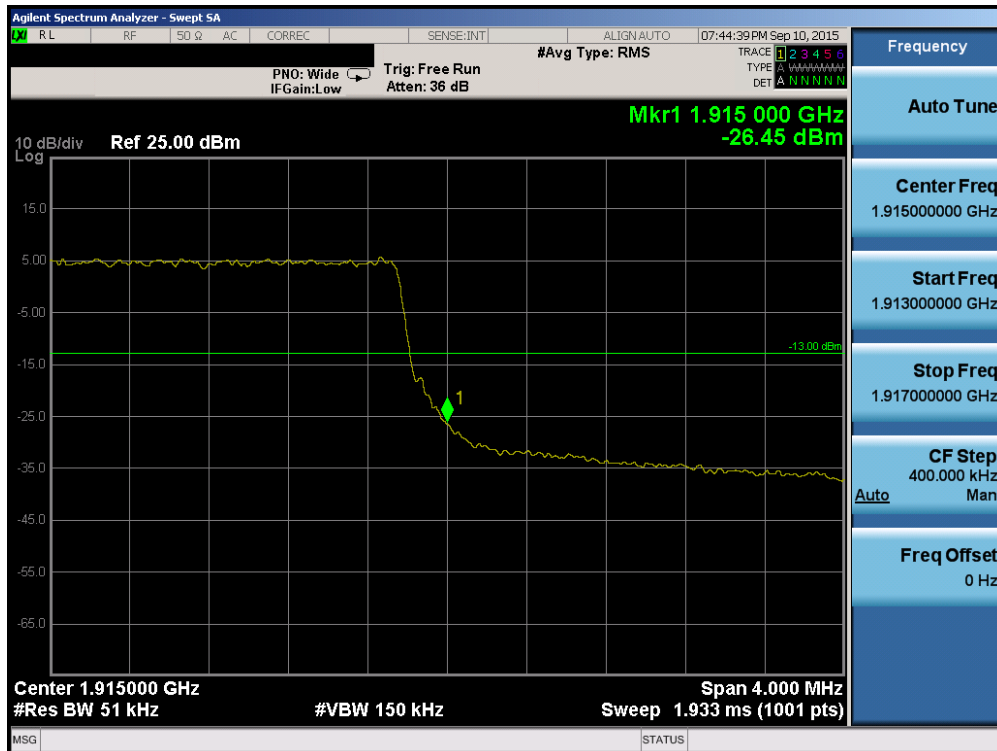
Plot 6-162. Upper Band Edge Plot (Band 2/25 – 5.0MHz QPSK – RB Size 25)
