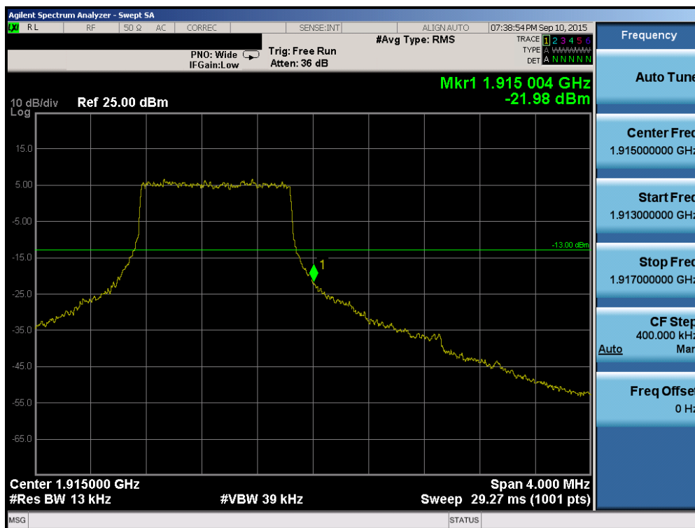
Plot 6-154. Upper Band Edge Plot (Band 2/25 – 1.4MHz QPSK – RB Size 6)
