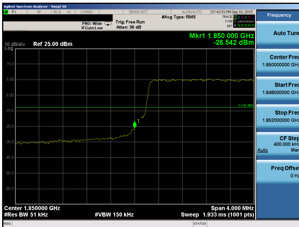
Plot 6-160. Lower Band Edge Plot (Band 2/25 – 5.0MHz QPSK – RB Size 25)
