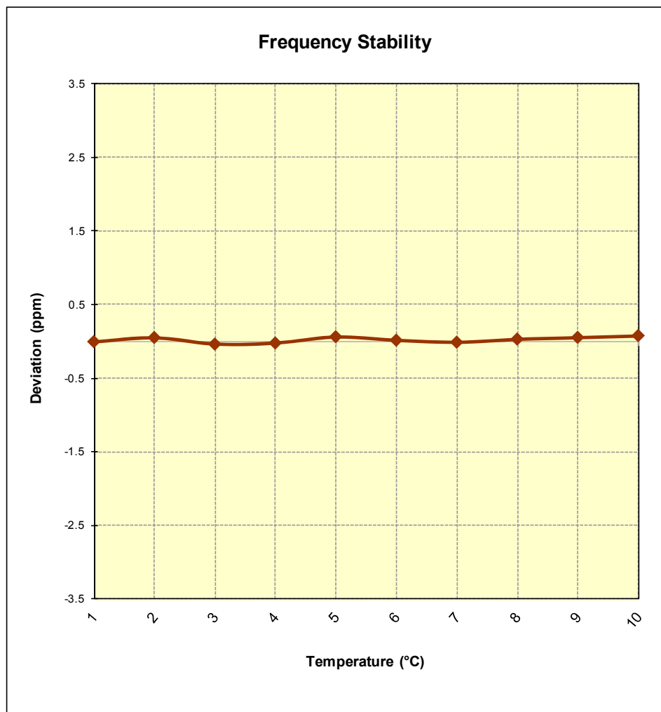
Figure 6-10. Frequency Stability Graph (Band 2/25)
