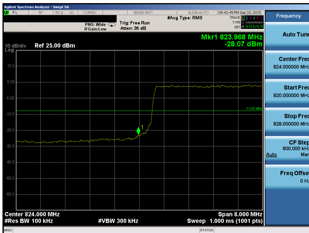
Plot 6-124. Lower Band Edge Plot (Band 5/26 - 10.0MHz QPSK - RB Size 50)
