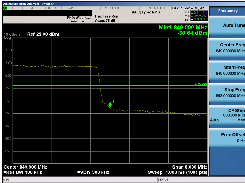
Plot 6-125. Upper Band Edge Plot (Band 5/26 – 10.0MHz QPSK – RB Size 50)
