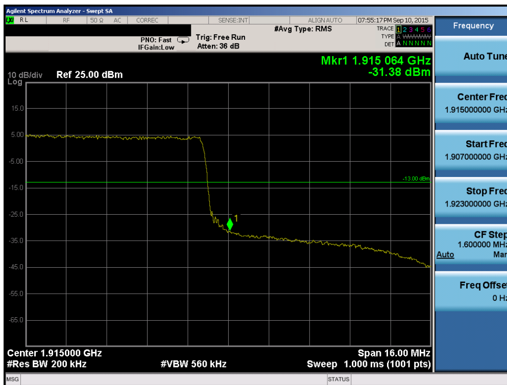
Plot 6-174. Upper Band Edge Plot (Band 2/25 – 20.0MHz QPSK – RB Size 100)
