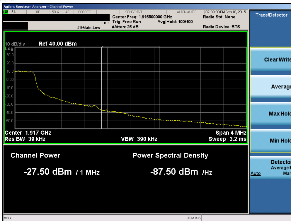
Plot 6-155. Upper Extended Band Edge Plot (Band 2/25 – 1.4MHz QPSK – RB Size 6)
