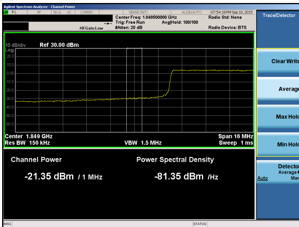
Plot 6-173. Lower Extended Band Edge Plot (Band 2/25 – 20.0MHz QPSK – RB Size 100)
