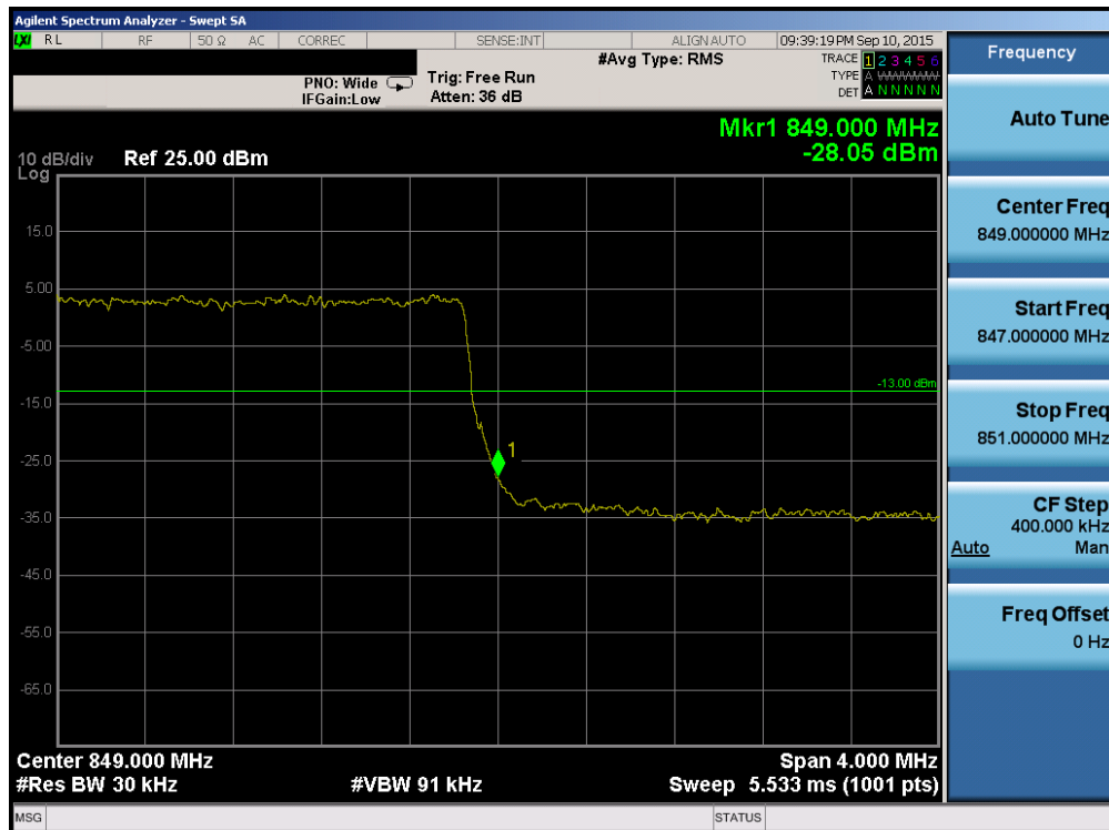
Plot 6-118. Upper Band Edge Plot (Band 5/26 – 3.0MHz QPSK – RB Size 15)
