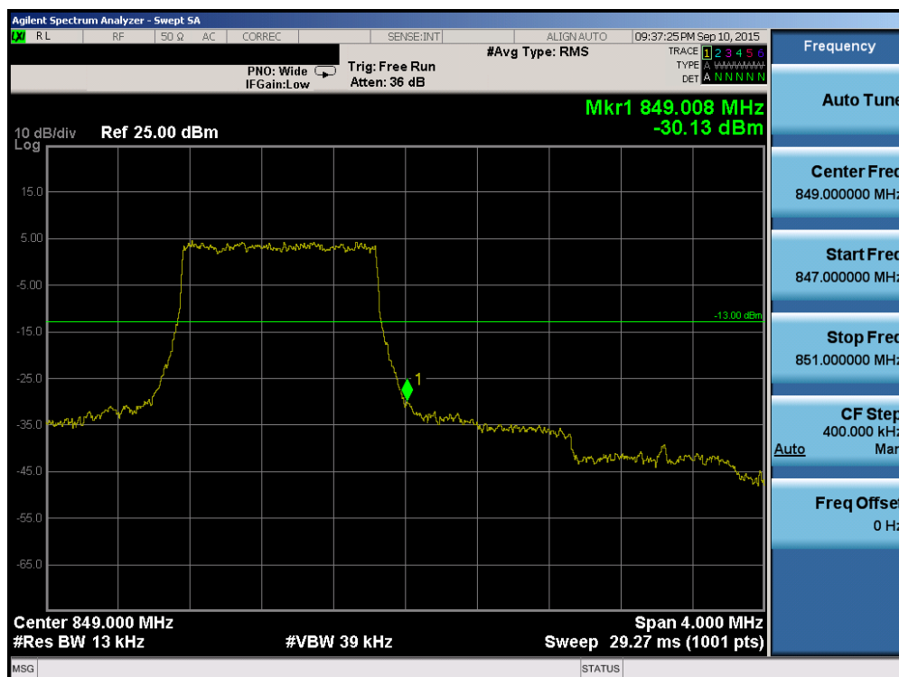
Plot 6-114. Upper Band Edge Plot (Band 5/26 – 1.4MHz QPSK – RB Size 6)
