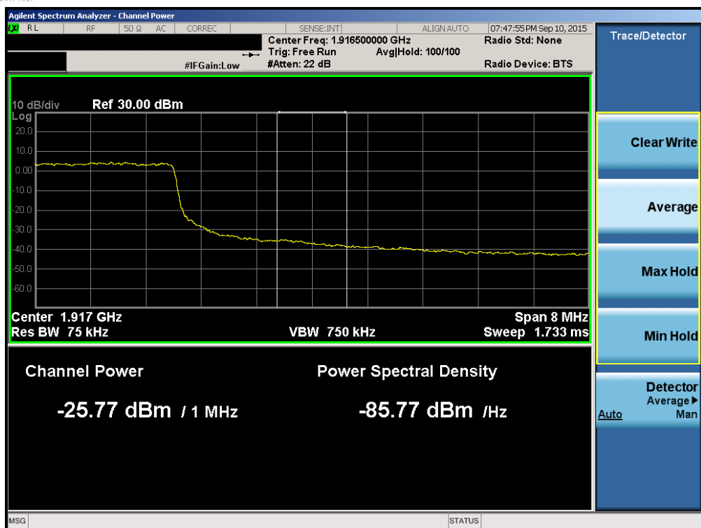
Plot 6-167. Upper Extended Band Edge Plot (Band 2/25 – 10.0MHz QPSK – RB Size 50)
