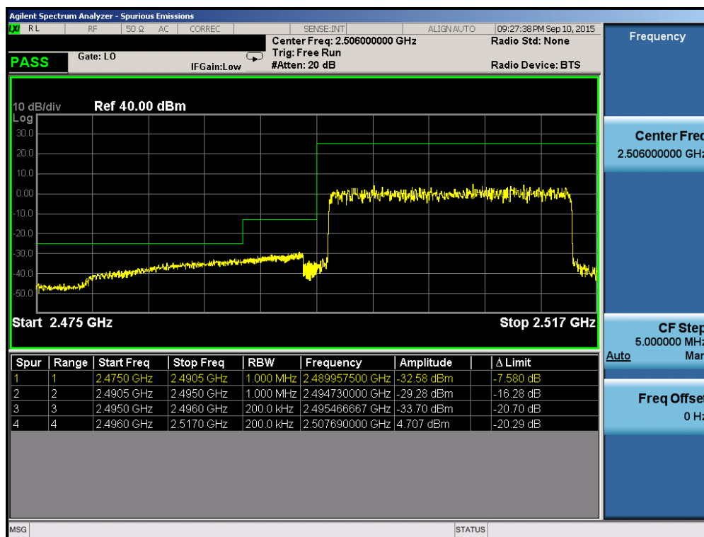
Plot 6-182. Lower ACP Plot (Band 41 – 20.0MHz QPSK – RB Size 100)
