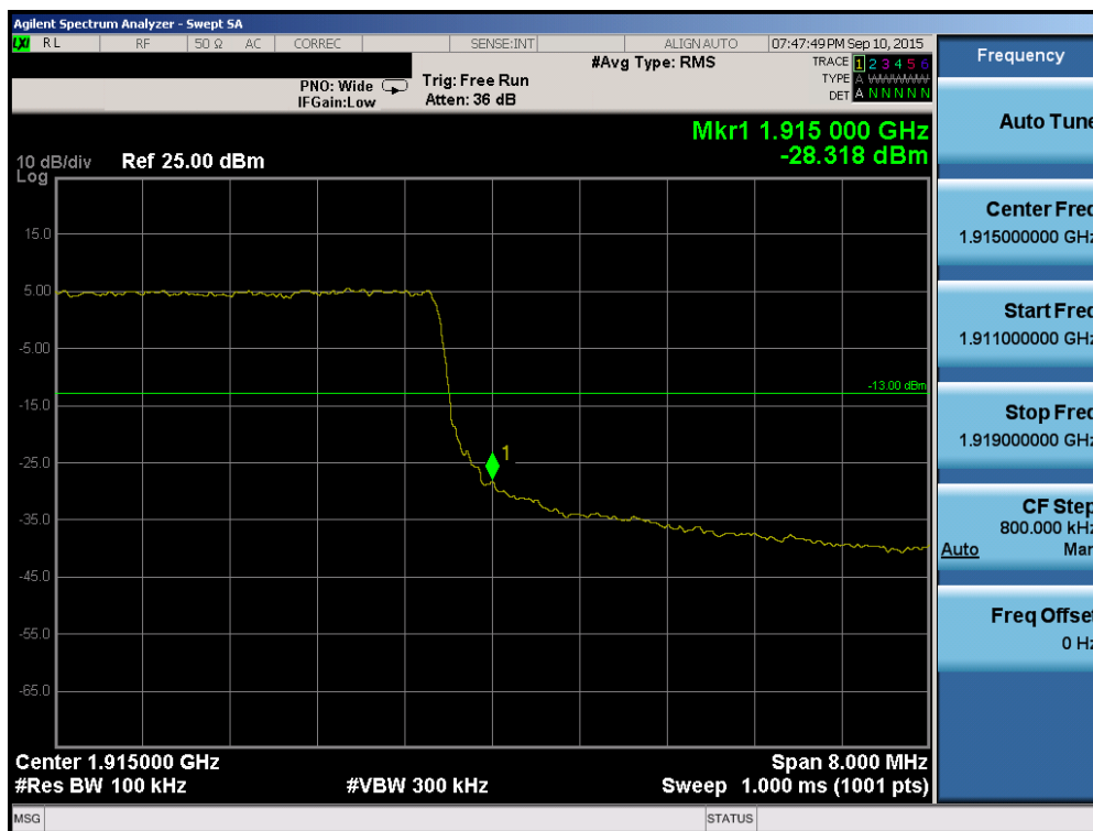
Plot 6-166. Upper Band Edge Plot (Band 2/25 – 10.0MHz QPSK – RB Size 50)
