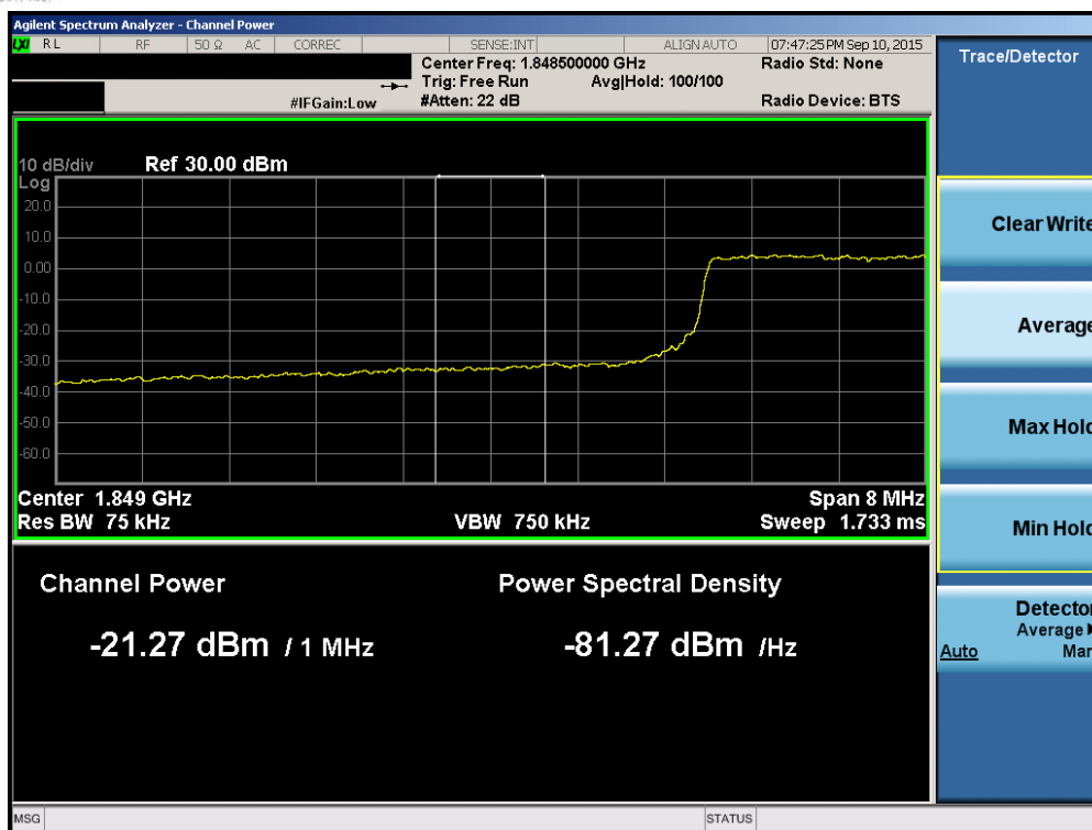
Plot 6-165. Lower Extended Band Edge Plot (Band 2/25 – 10.0MHz QPSK – RB Size 50)
