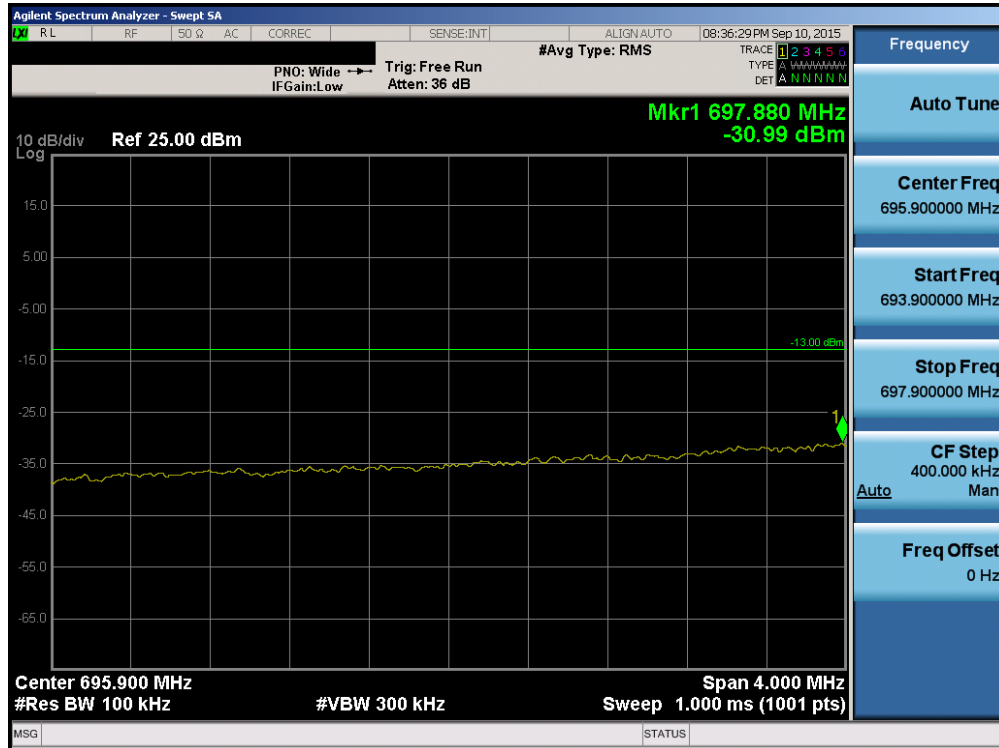
Plot 6-109. Lower Extended Band Edge Plot (Band 12 – 10.0MHz QPSK – RB Size 50)
