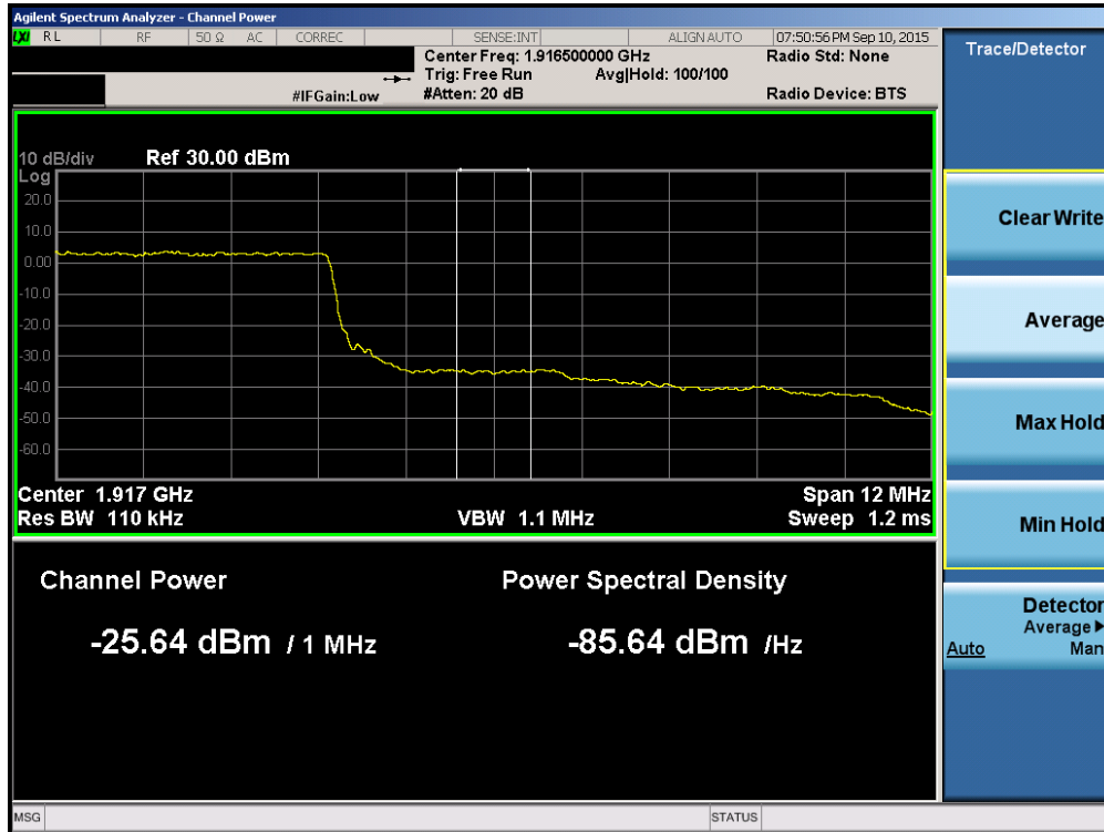
Plot 6-171. Upper Extended Band Edge Plot (Band 2/25 – 15.0MHz QPSK – RB Size 75)
