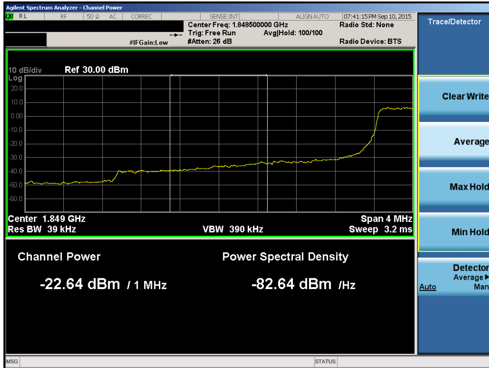
Plot 6-157. Lower Extended Band Edge Plot (Band 2/25 – 3.0MHz QPSK – RB Size 15)
