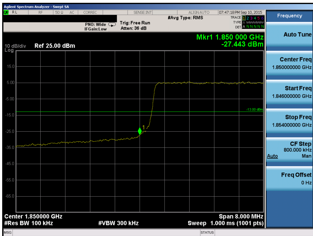
Plot 6-164. Lower Band Edge Plot (Band 2/25 – 10.0MHz QPSK – RB Size 50)
