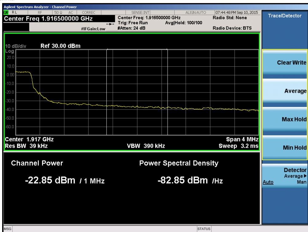
Plot 6-163. Upper Extended Band Edge Plot (Band 2/25 – 5.0MHz QPSK – RB Size 25)
