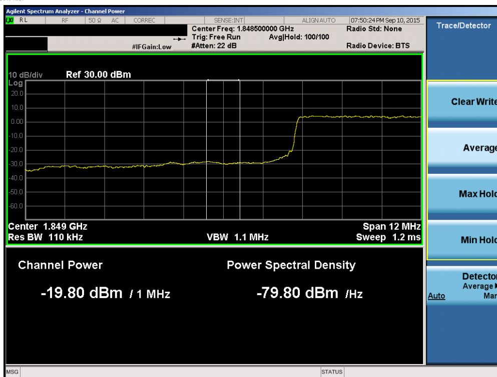
Plot 6-169. Lower Extended Band Edge Plot (Band 2/25 – 15.0MHz QPSK – RB Size 75)
