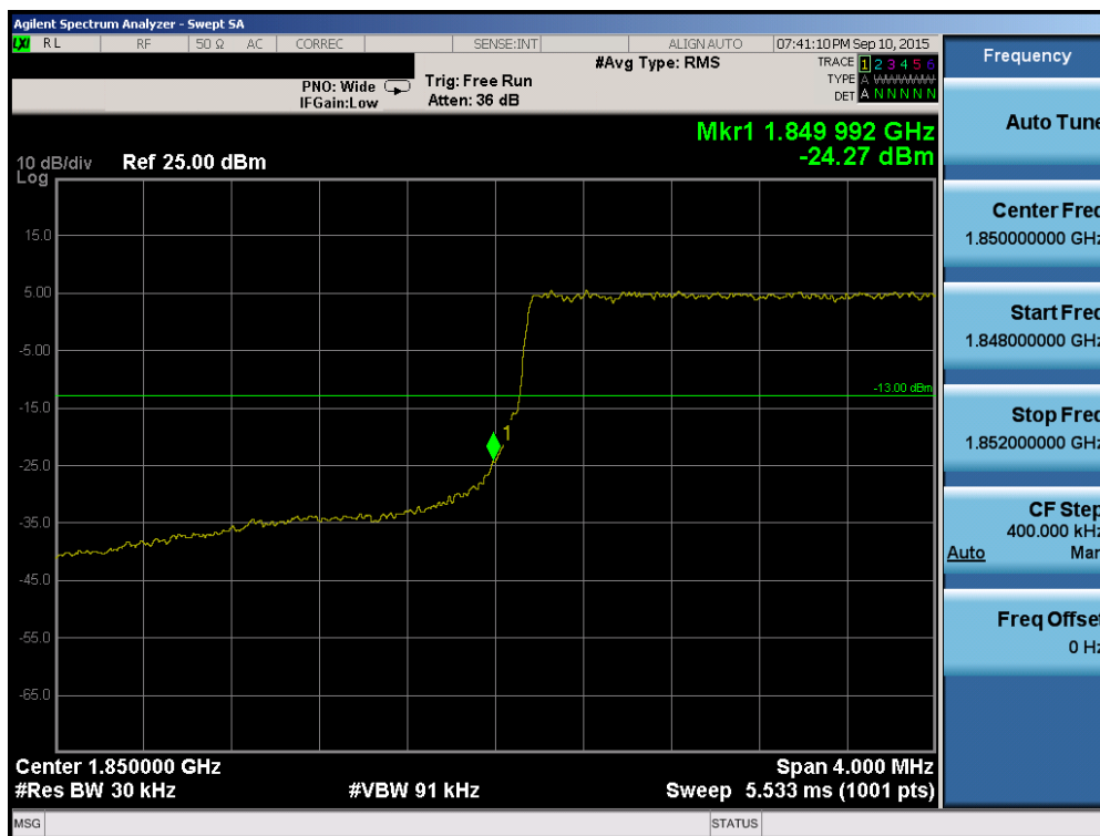
Plot 6-156. Lower Band Edge Plot (Band 2/25 – 3.0MHz QPSK – RB Size 15)
