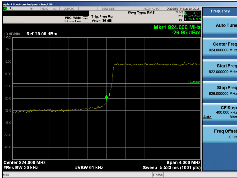
Plot 6-116. Lower Band Edge Plot (Band 5/26 – 3.0MHz QPSK – RB Size 15)
