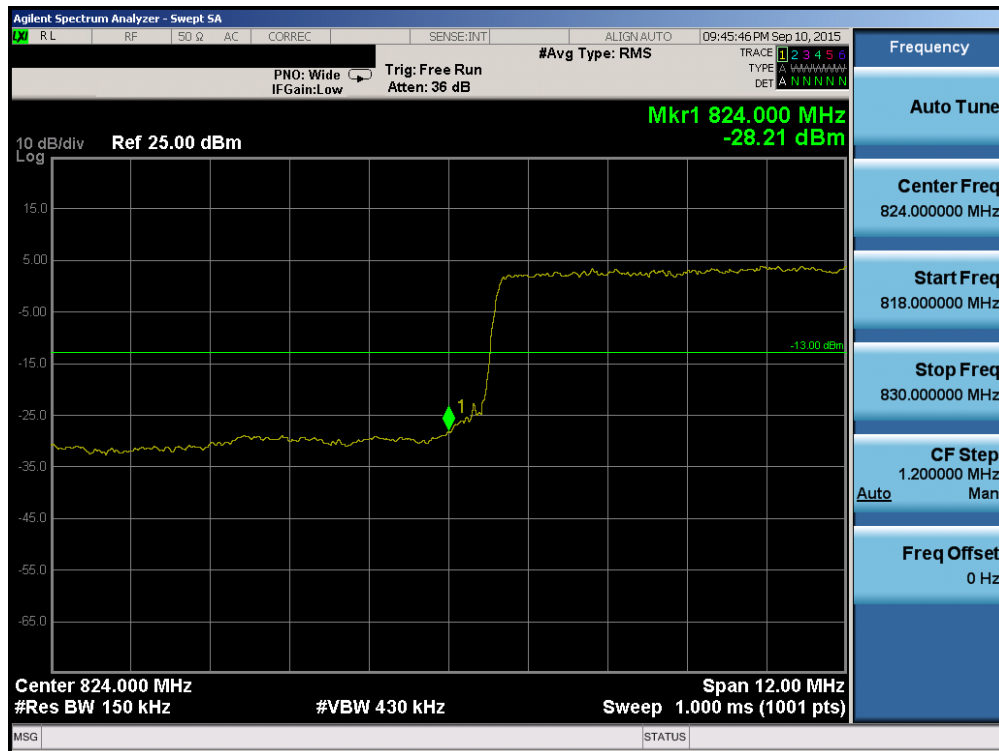
Plot 6-126. Lower Band Edge Plot (Band 26 – 15.0MHz QPSK – RB Size 75)
