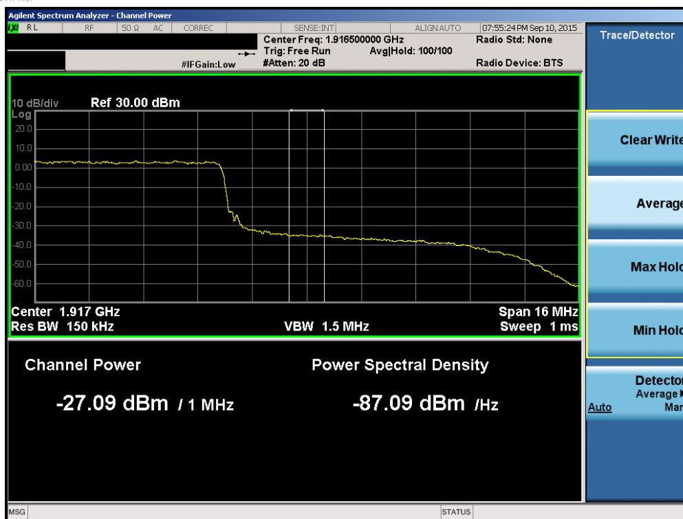
Plot 6-175. Upper Extended Band Edge Plot (Band 2/25 – 20.0MHz QPSK – RB Size 100)
