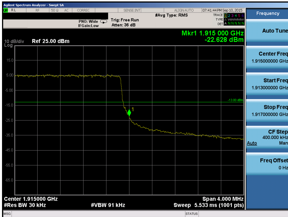
Plot 6-158. Upper Band Edge Plot (Band 2/25 – 3.0MHz QPSK – RB Size 15)
