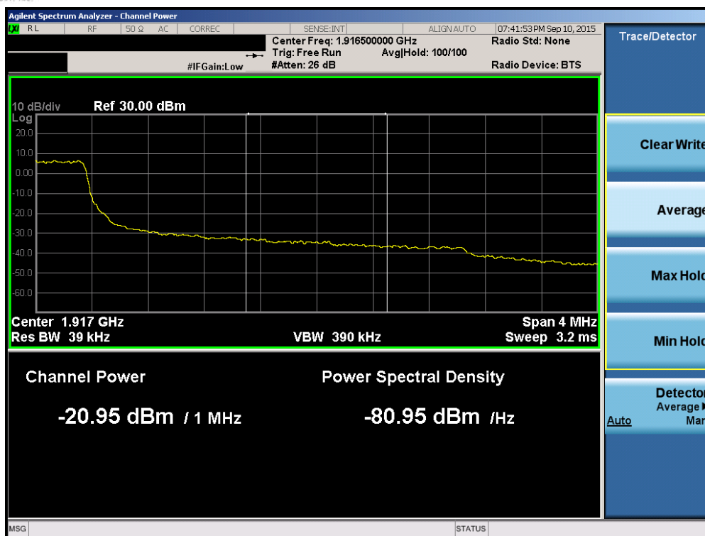
Plot 6-159. Upper Extended Band Edge Plot (Band 2/25 – 3.0MHz QPSK – RB Size 15)
