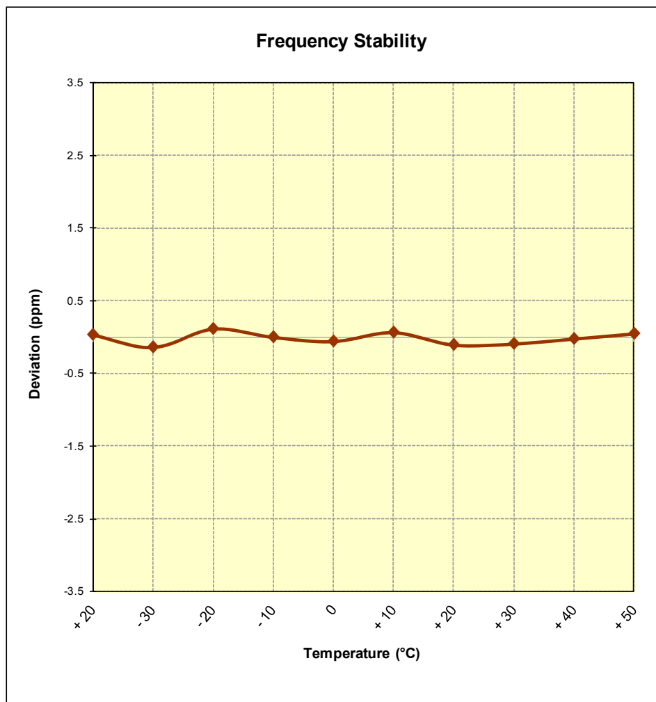
Figure 6-8. Frequency Stability Graph (Band 5/26)
