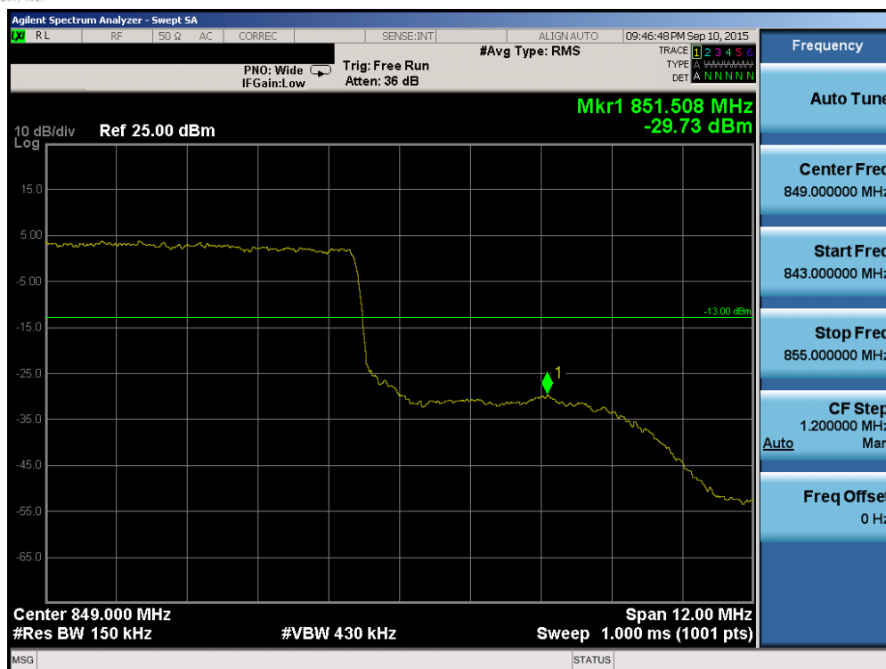
Plot 6-127. Upper Band Edge Plot (Band 26 – 15.0MHz QPSK – RB Size 75)
