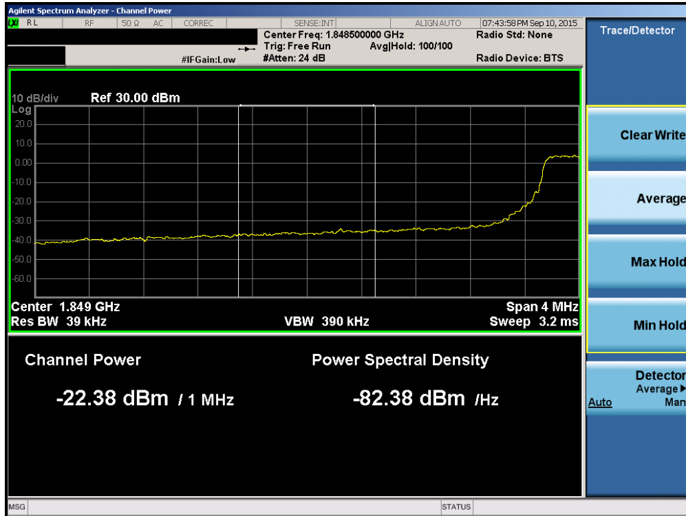
Plot 6-161. Lower Extended Band Edge Plot (Band 2/25 – 5.0MHz QPSK – RB Size 25)
