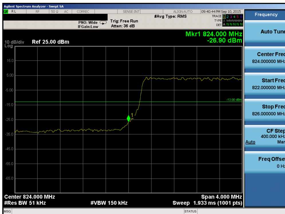
Plot 6-120. Lower Band Edge Plot (Band 5/26 – 5.0MHz QPSK – RB Size 25)
