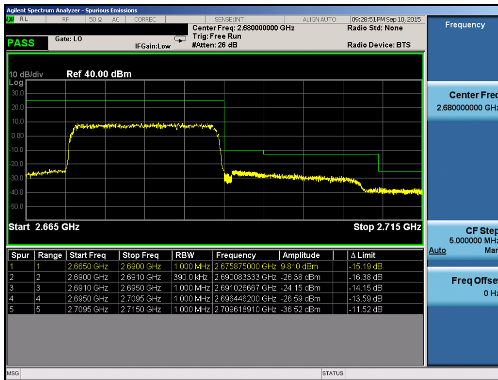
Plot 6-183. Upper ACP Plot (Band 41 – 20.0MHz QPSK – RB Size 100)
