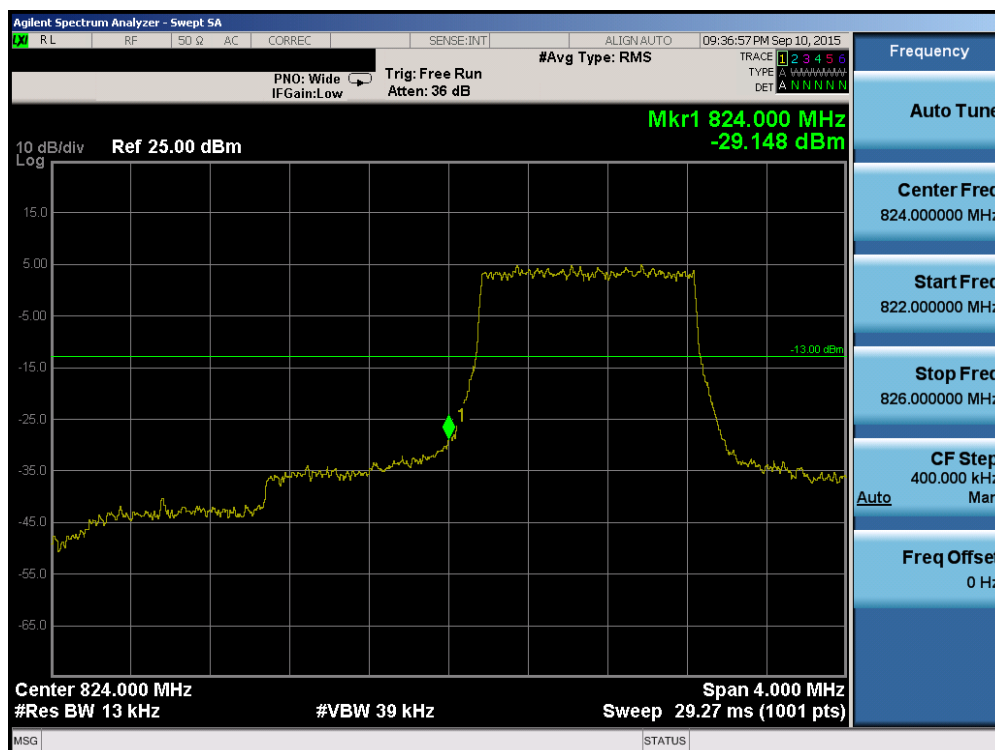
Plot 6-112. Lower Band Edge Plot (Band 5/26 – 1.4MHz QPSK – RB Size 6)
