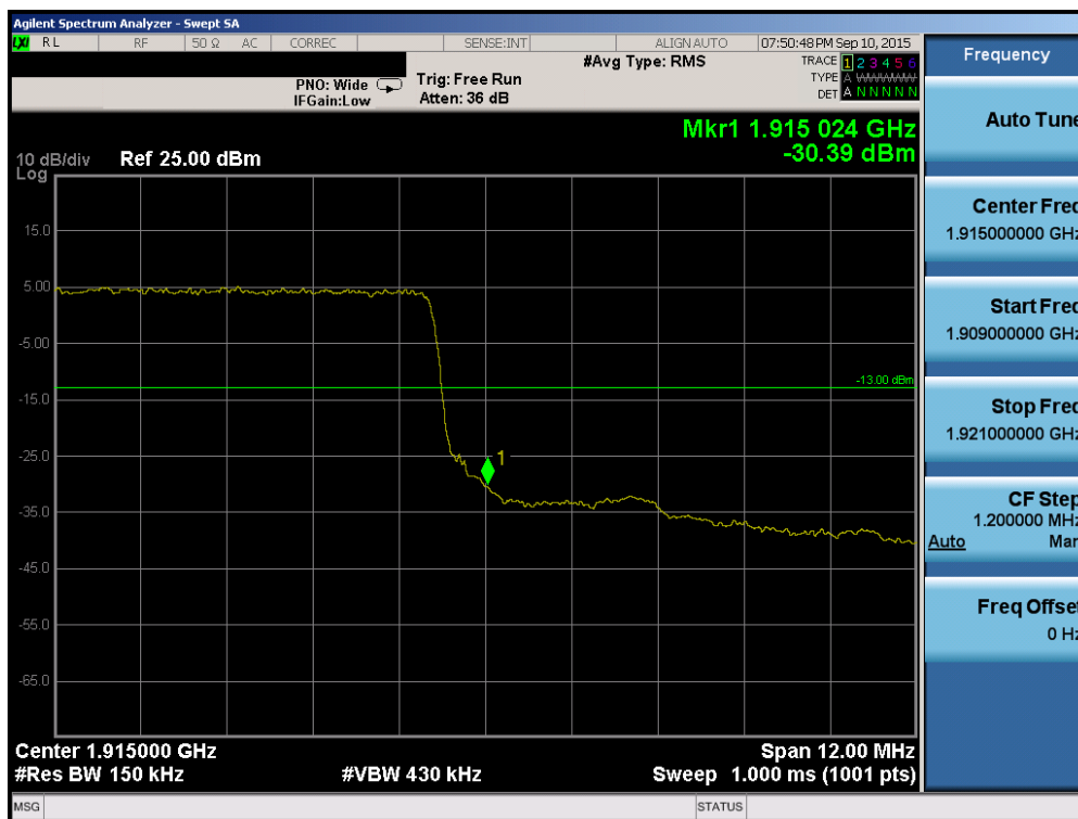
Plot 6-170. Upper Band Edge Plot (Band 2/25 – 15.0MHz QPSK – RB Size 75)
