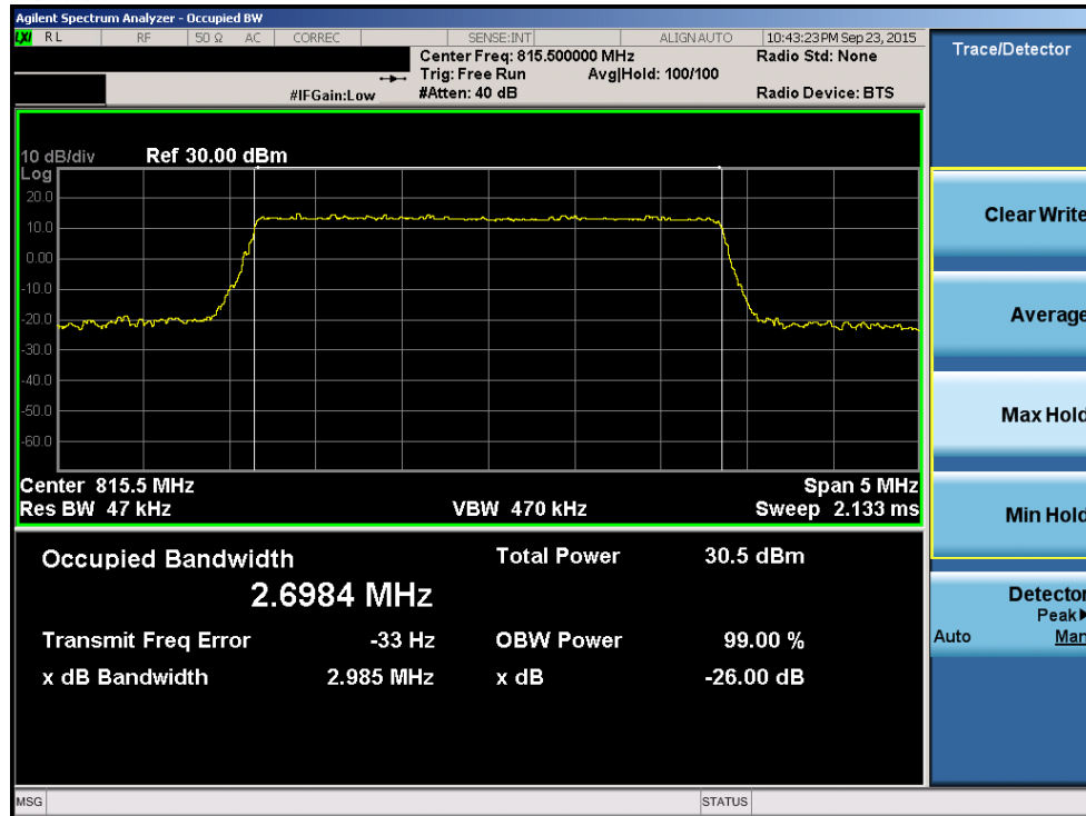
Plot 8-7. Occupied Bandwidth Plot (3MHz 16-QAM – RB Size 15– Low Channel)
