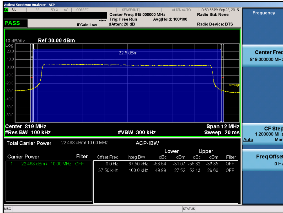
Plot 8-15. Channel Edge Plot (10MHz QPSK – RB Size 50)
