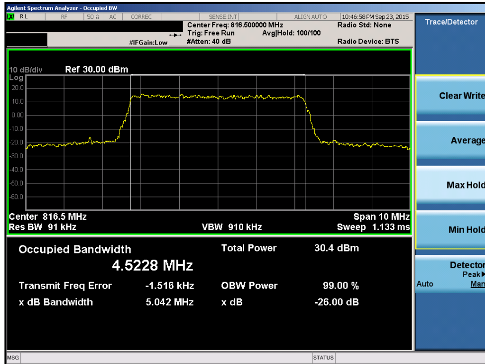
Plot 8-11. Occupied Bandwidth Plot (5MHz 16-QAM – RB Size 25– Low Channel))
