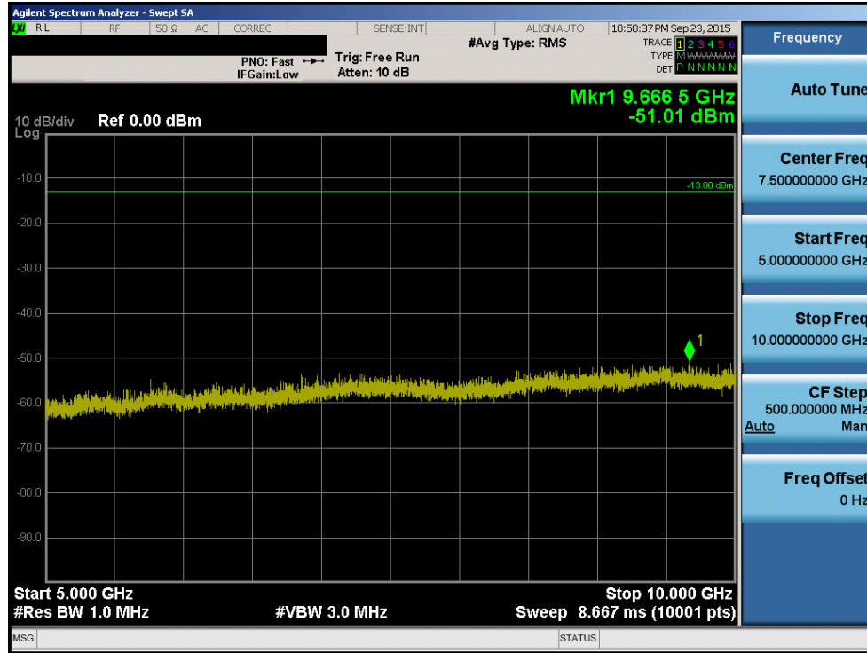
Plot 8-17. Conducted Spurious Plot (10MHz QPSK – RB Size 1, RB Offset 0)
