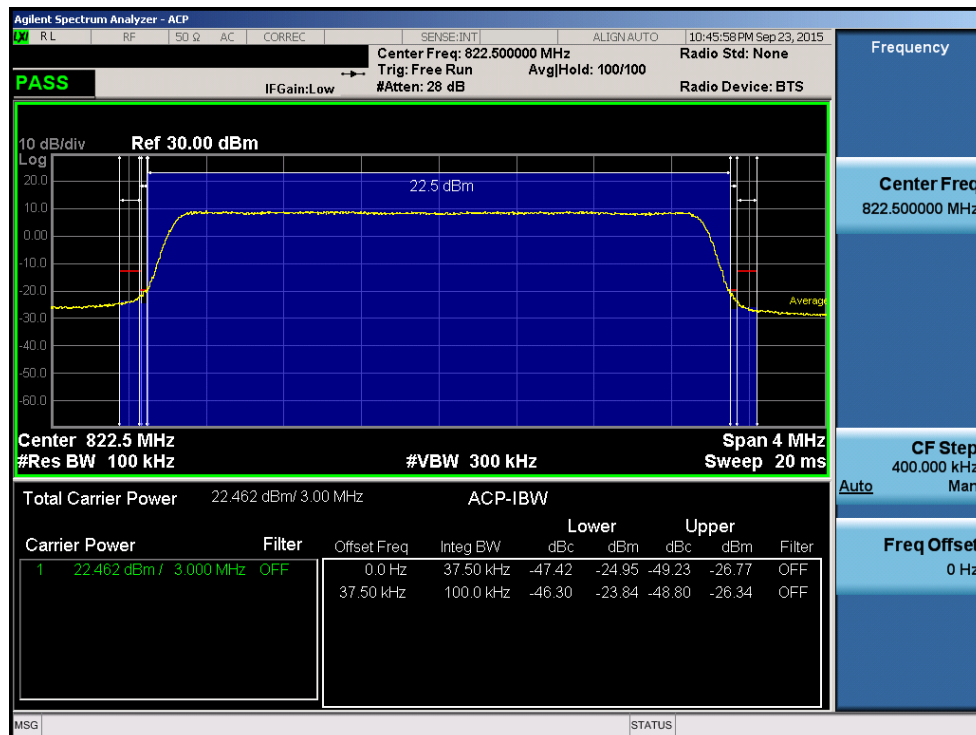
Plot 8-8. Channel Edge Plot (3MHz QPSK – RB Size 15 – High Channel)
