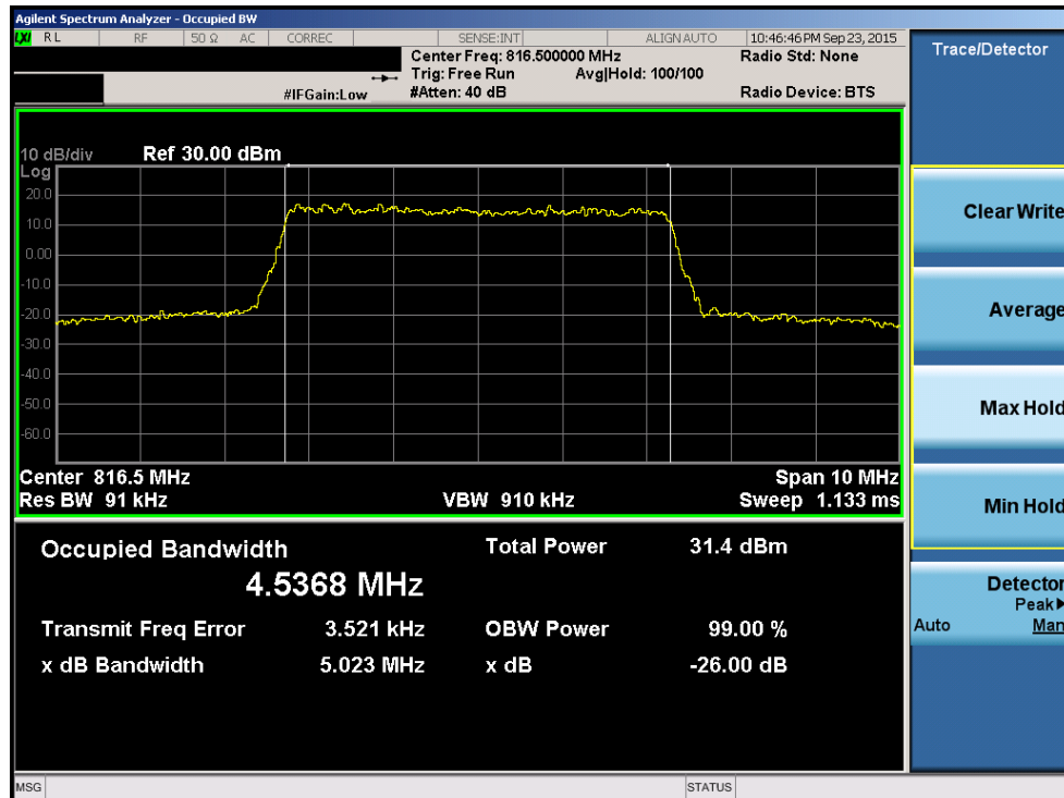
Plot 8-10. Occupied Bandwidth Plot (5MHz QPSK – RB Size 25– Low Channel)
