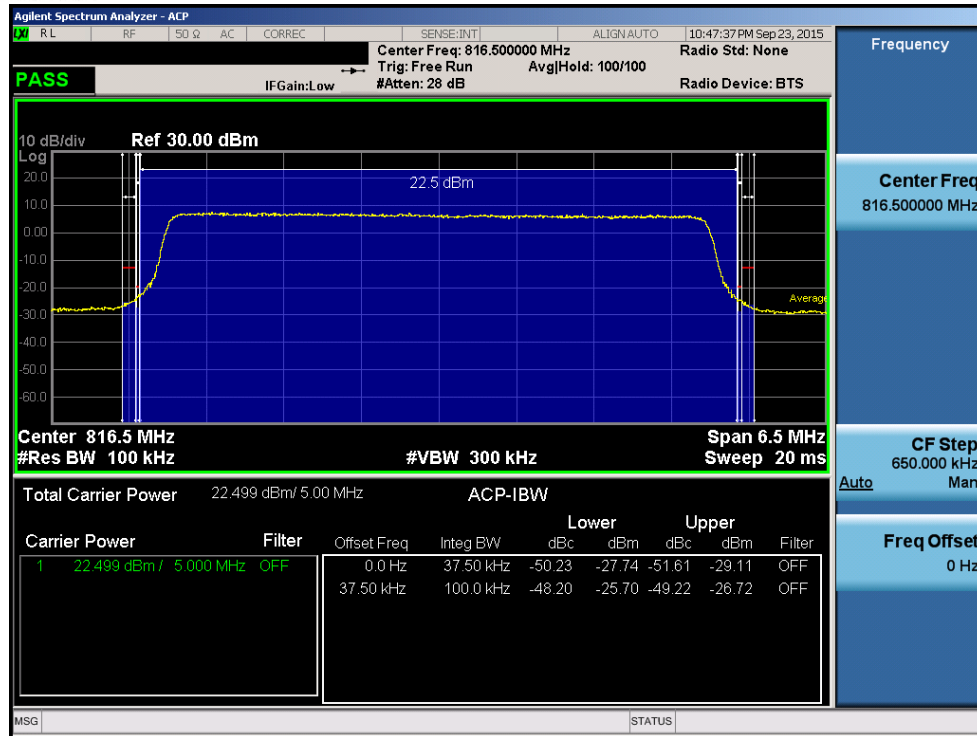
Plot 8-9. Channel Edge Plot (5MHz QPSK – RB Size 25– Low Channel)
