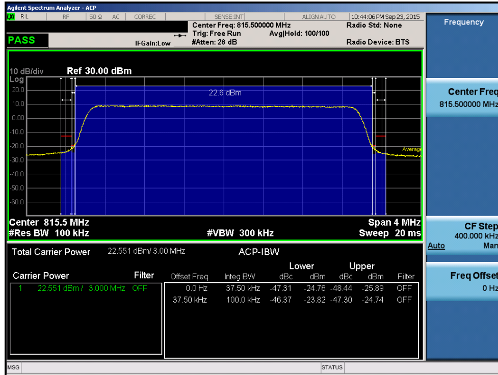
Plot 8-5. Channel Edge Plot (3MHz QPSK – RB Size 15– Low Channel)
