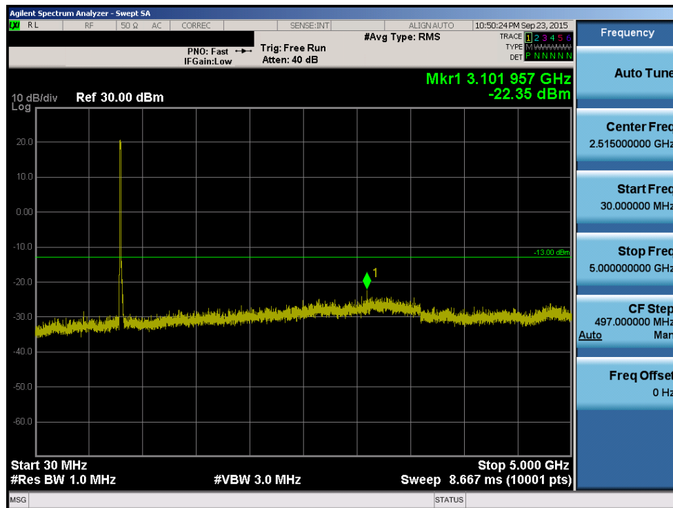
Plot 8-16. Conducted Spurious Plot (10MHz QPSK – RB Size 1, RB Offset 0)
