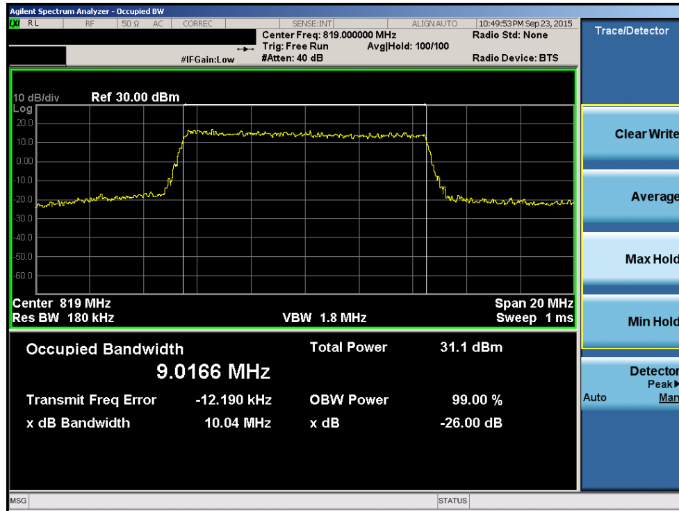
Plot 8-13. Occupied Bandwidth Plot (10MHz QPSK – RB Size 50)
