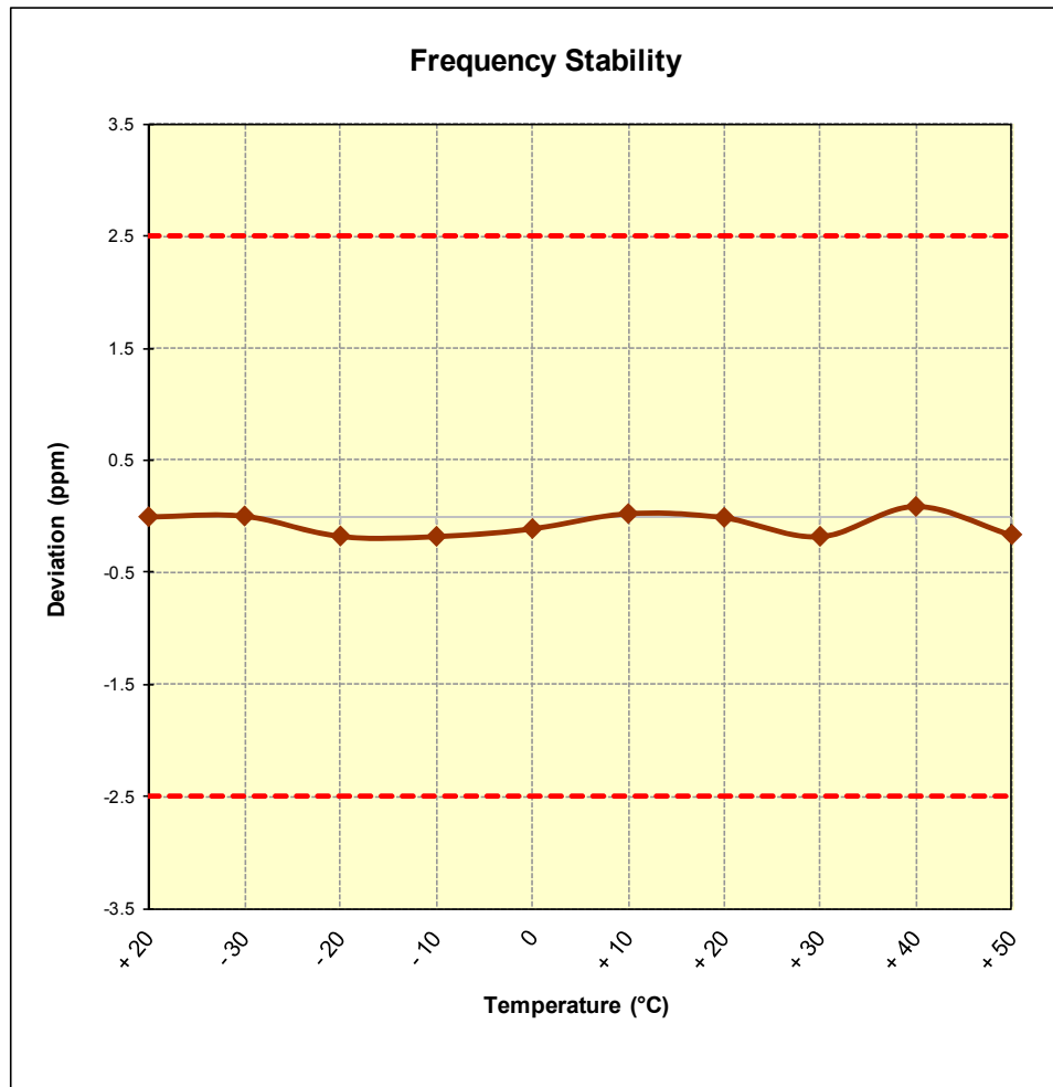
Figure 6-1. CDMA BC10 Frequency Stability Graph (Ch. 476)
