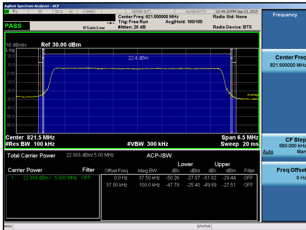
Plot 8-12. Channel Edge Plot (5MHz QPSK – RB Size 25 – High Channel)
