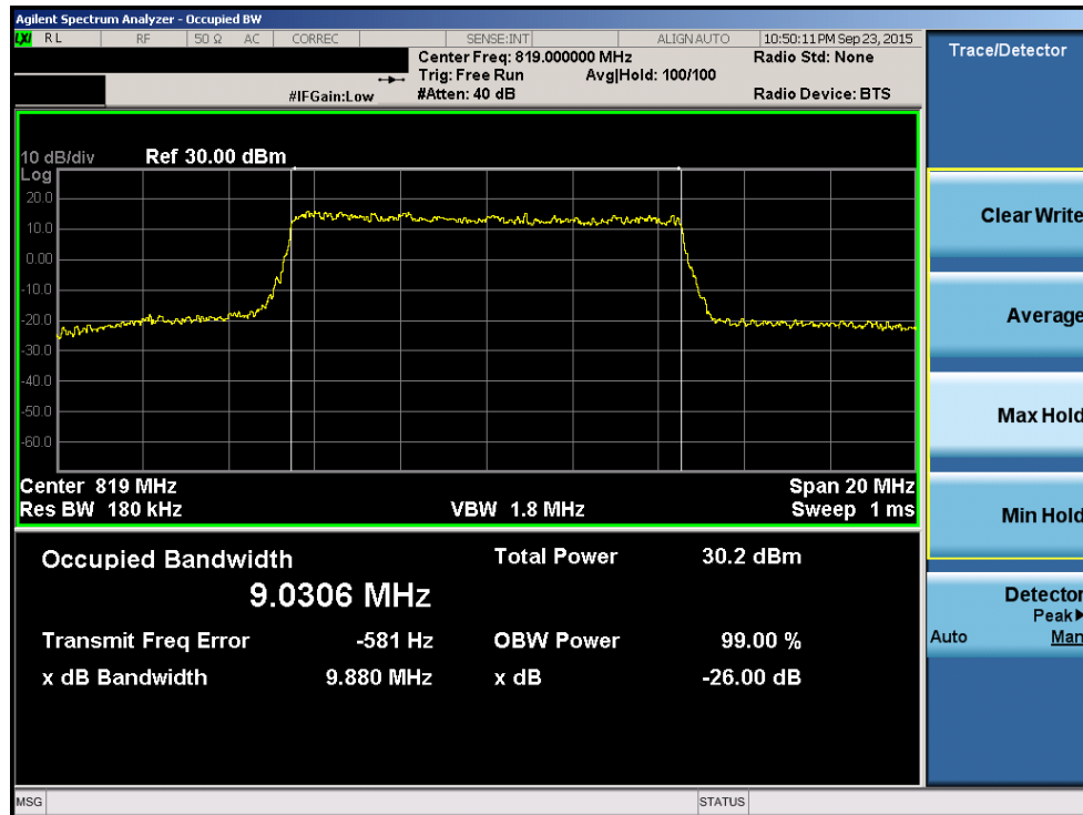
Plot 8-14. Occupied Bandwidth Plot (10MHz 16-QAM – RB Size 50)
