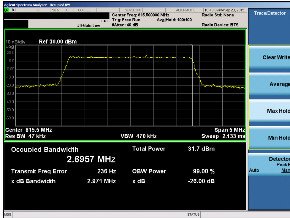
Plot 8-6. Occupied Bandwidth Plot (3MHz QPSK – RB Size 15– Low Channel)
