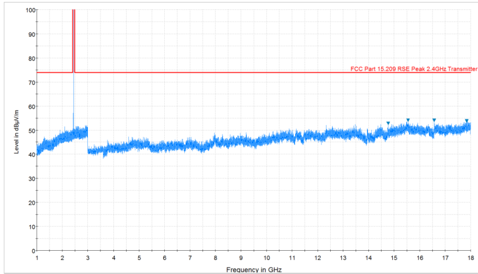
Plot 6-44. Radiated Spurious Plot above 1GHz (BT – Ch. 39, Ant. Pol. H)
