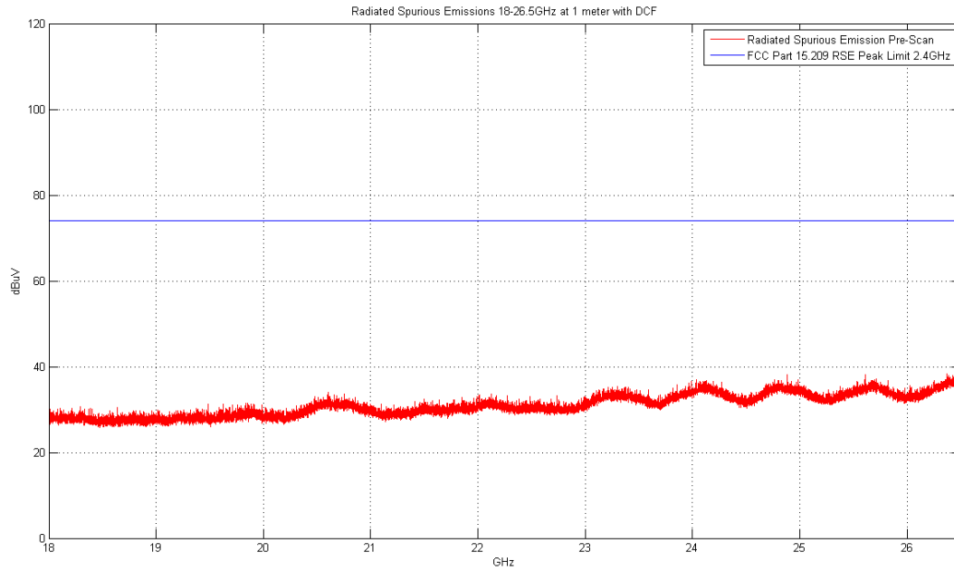
Plot 6-48. Radiated Spurious Plot above 18GHz (Pol. H)
