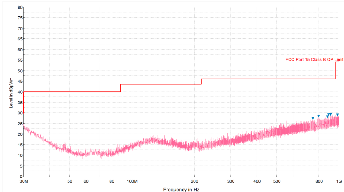
Plot 6-52. Radiated Spurious Plot below 1GHz (Pol. H)
