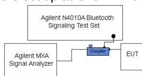
Figure 6-2. Test Instrument & Measurement Setup
