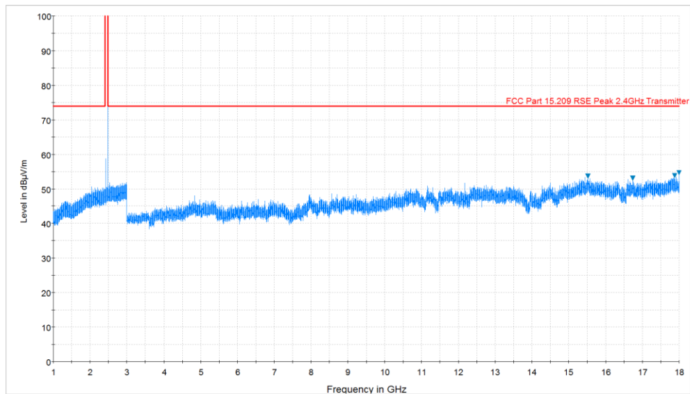
Plot 6-47. Radiated Spurious Plot above 1GHz (BT – Ch. 78, Ant. Pol. V)
