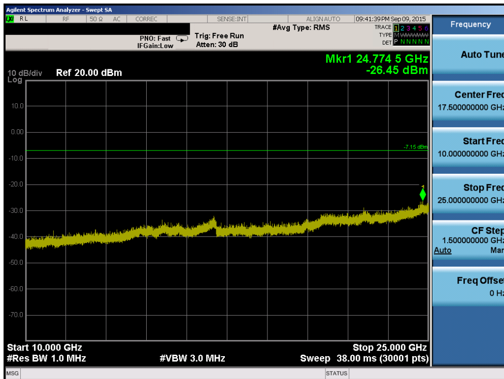
Plot 6-39. Conducted Spurious Plot (Bluetooth, 3Mbps – Ch. 39)
