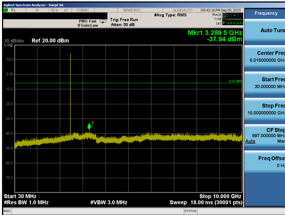
Plot 6-40. Conducted Spurious Plot (Bluetooth, 3Mbps – Ch. 78)
