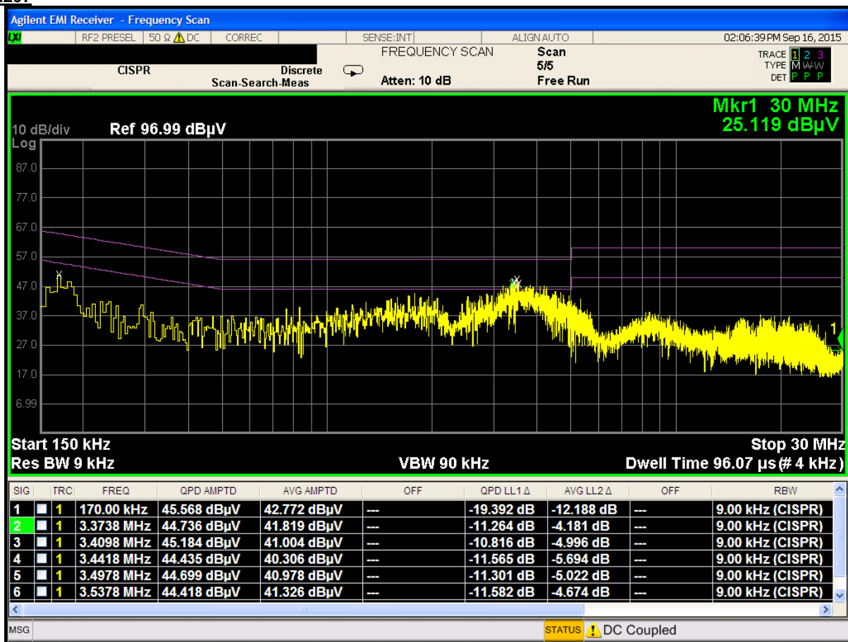
Plot 6-55. Line-Conducted Test Plot (N)
