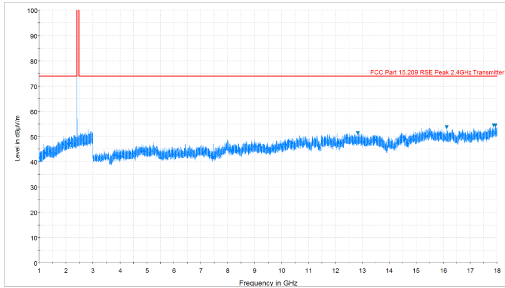
Plot 6-42. Radiated Spurious Plot above 1GHz (BT – Ch. 0, Ant. Pol. H)
