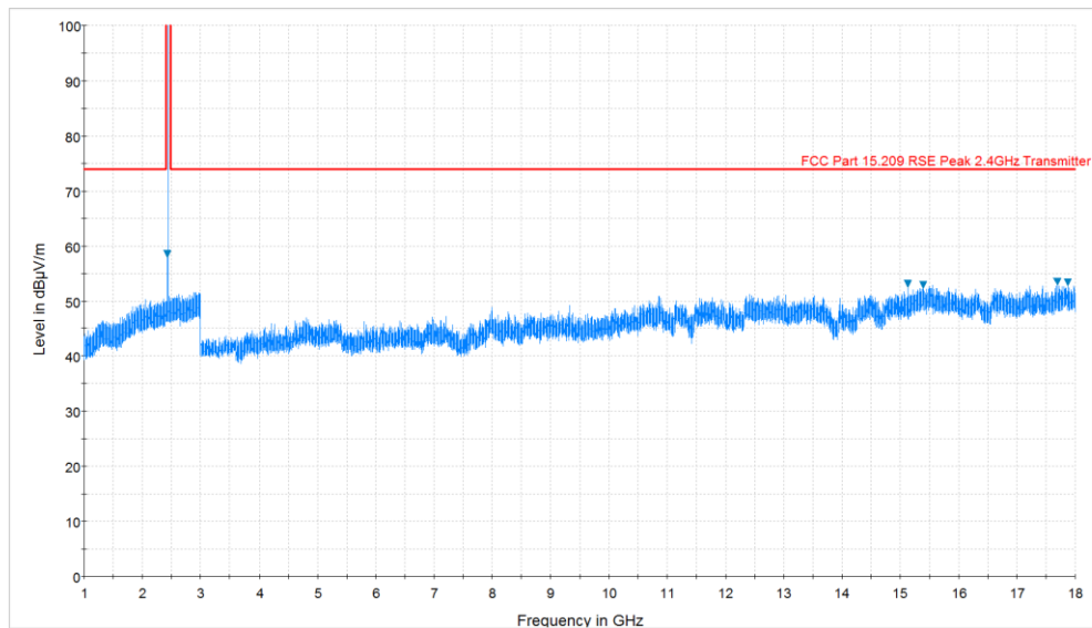
Plot 6-45. Radiated Spurious Plot above 1GHz (BT – Ch. 39, Ant. Pol. V)
