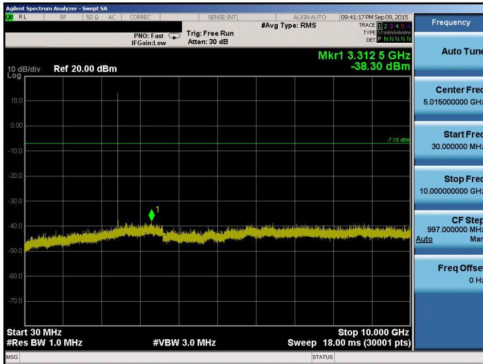
Plot 6-38. Conducted Spurious Plot (Bluetooth, 3Mbps – Ch. 39)
