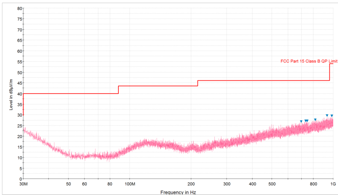
Plot 6-53. Radiated Spurious Plot below 1GHz (Pol. V)
