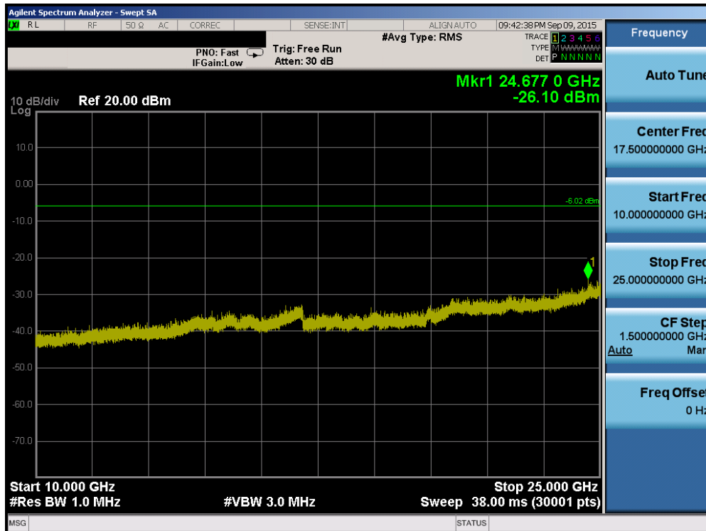
Plot 6-41. Conducted Spurious Plot (Bluetooth, 3Mbps – Ch. 78)
