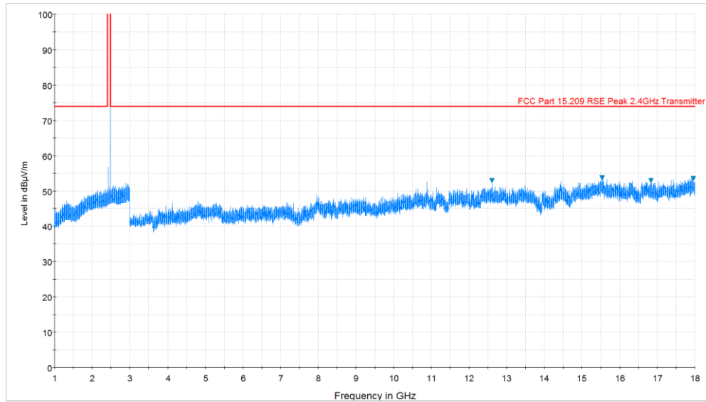
Plot 6-46. Radiated Spurious Plot above 1GHz (BT – Ch. 78, Ant. Pol. H)
