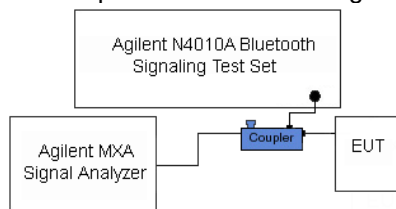
Figure 6-1. Test Instrument & Measurement Setup
