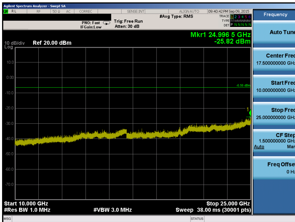
Plot 6-37. Conducted Spurious Plot (Bluetooth, 3Mbps – Ch. 0)
