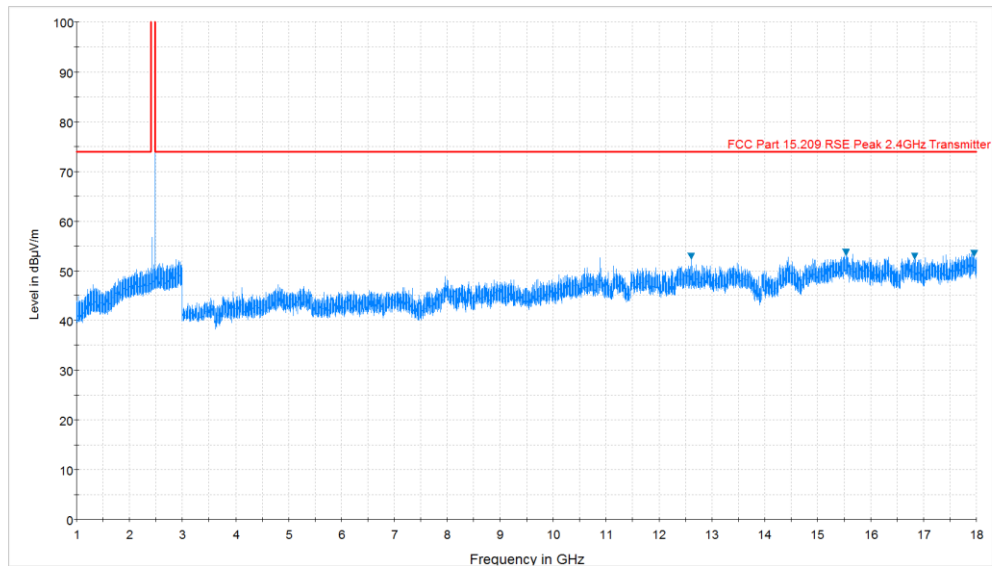
Plot 6-43. Radiated Spurious Plot above 1GHz (BT – Ch. 0, Ant. Pol. V)
