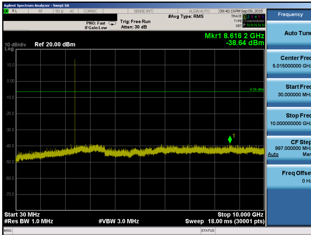
Plot 6-36. Conducted Spurious Plot (Bluetooth, 3Mbps – Ch. 0)
