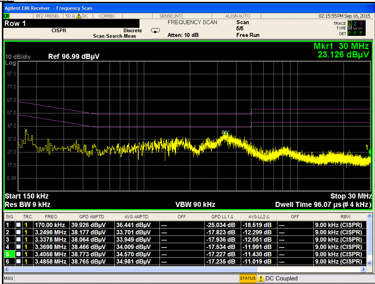
Plot 6-54. Line-Conducted Test Plot (L1)
