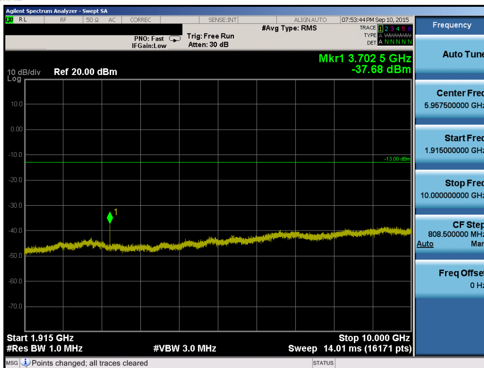
Plot 6-69. Conducted Spurious Plot (Band 2/25 – 20.0MHz QPSK – RB Size 1, RB Offset 0 – Low Channel)
