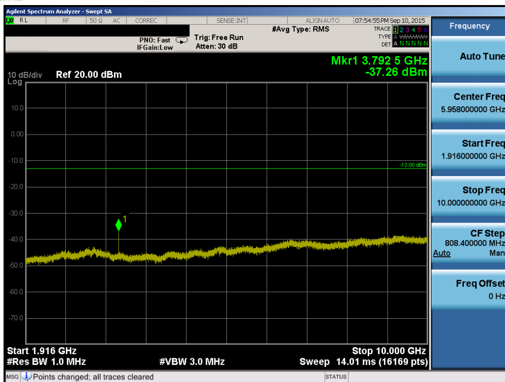
Plot 6-75. Conducted Spurious Plot (Band 2/25 – 20.0MHz QPSK – RB Size 1, RB Offset 0 – High Channel)
