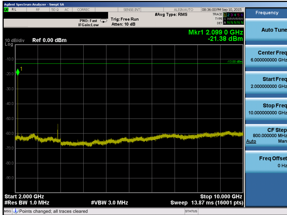
Plot 6-43. Conducted Spurious Plot (Band 12/17 – 10.0MHz QPSK – RB Size 1, RB Offset 0 – Low Channel)
