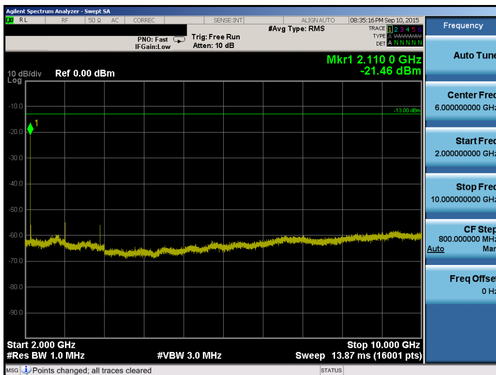
Plot 6-46. Conducted Spurious Plot (Band 12/17 – 10.0MHz QPSK – RB Size 1, RB Offset 0 – Mid Channel)
