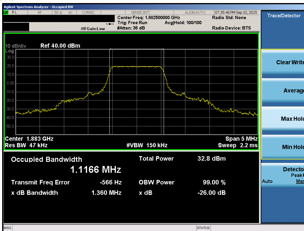
Plot 6-29. Occupied Bandwidth Plot (Band 2/25 – 1.4MHz QPSK – RB Size 6)
