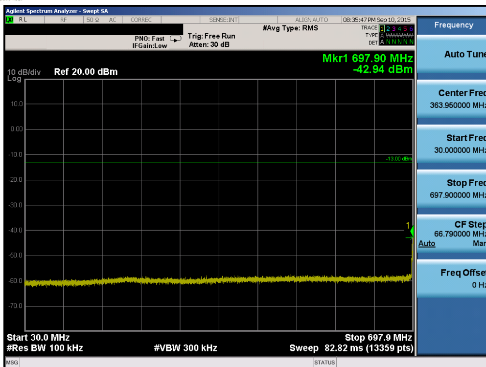
Plot 6-41. Conducted Spurious Plot (Band 12/17 – 10.0MHz QPSK – RB Size 1, RB Offset 0– Low Channel)
