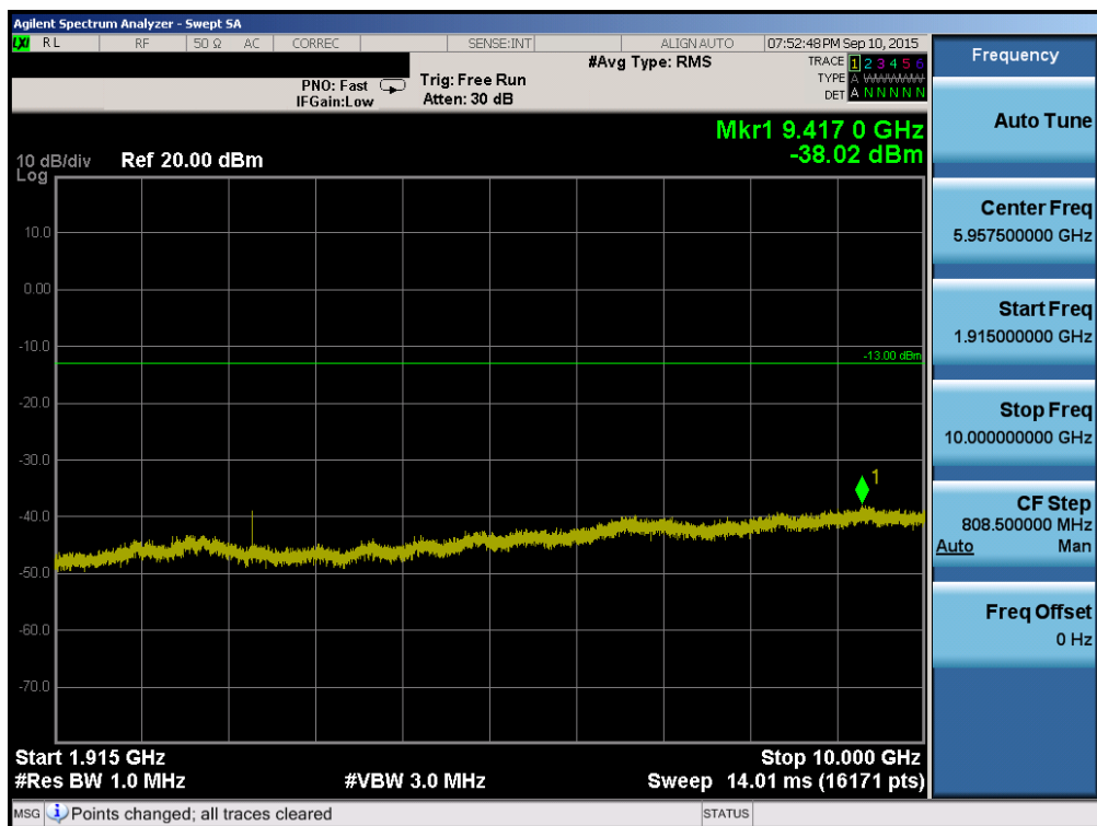
Plot 6-72. Conducted Spurious Plot (Band 2/25 – 20.0MHz QPSK – RB Size 1, RB Offset 0 – Mid Channel)
