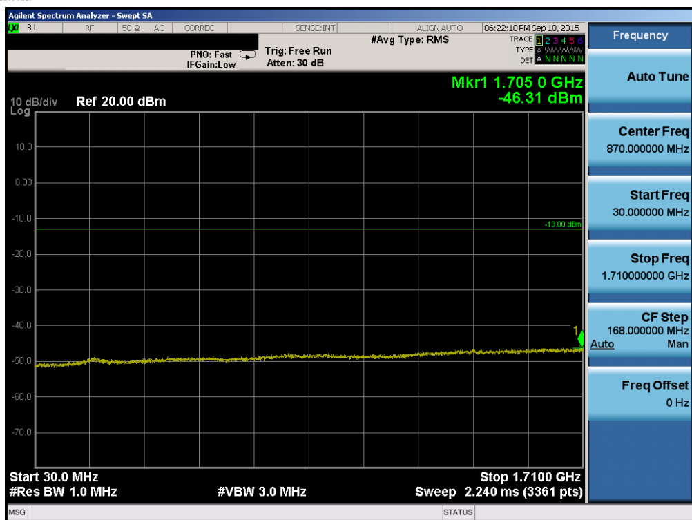
Plot 6-65. Conducted Spurious Plot (Band 4 – 20.0MHz QPSK – RB Size 1, RB Offset 0 – High Channel)
