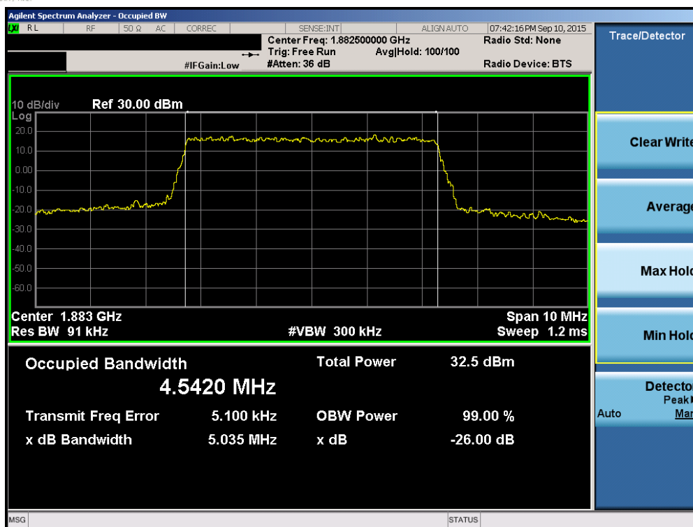
Plot 6-33. Occupied Bandwidth Plot (Band 2/25 – 5.0MHz QPSK – RB Size 25)
