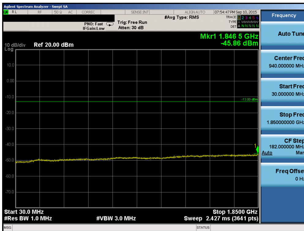
Plot 6-74. Conducted Spurious Plot (Band 2/25 – 20.0MHz QPSK – RB Size 1, RB Offset 0 – High Channel)
