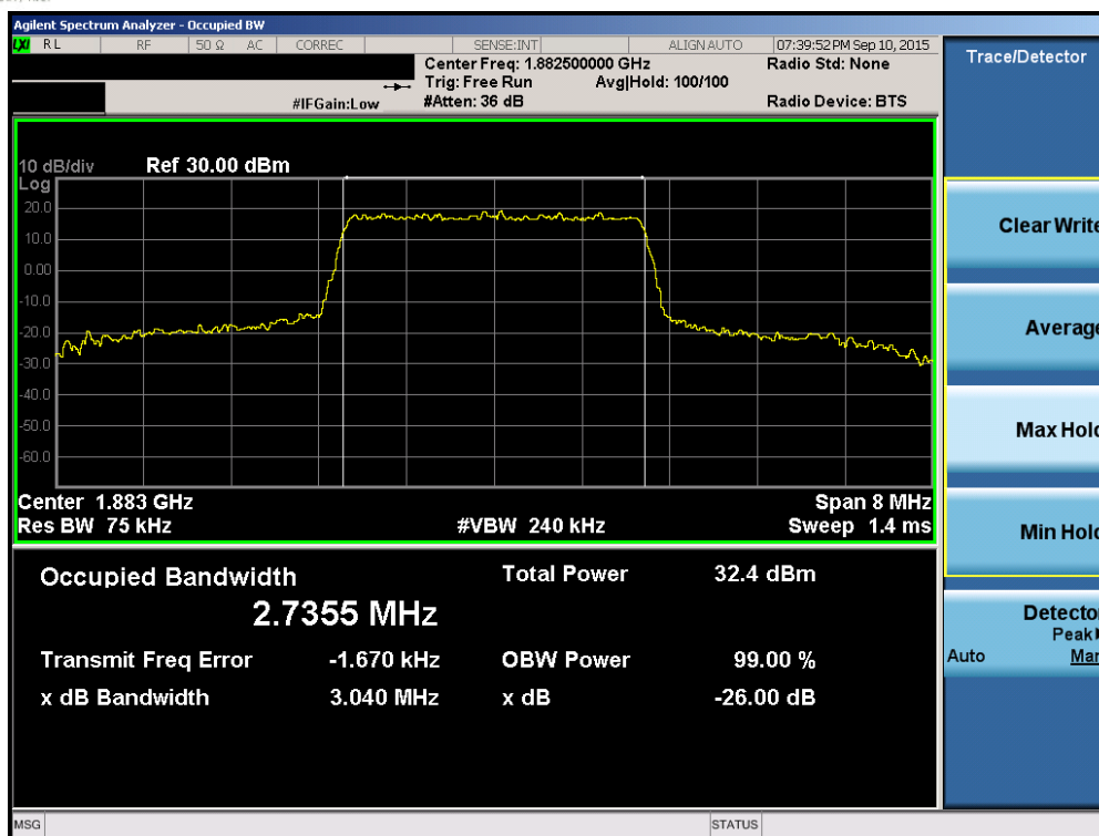
Plot 6-31. Occupied Bandwidth Plot (Band 2/25 – 3.0MHz QPSK – RB Size 15)
