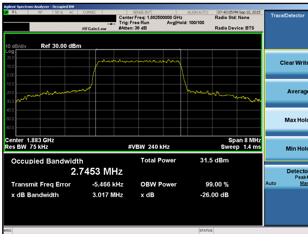
Plot 6-32. Occupied Bandwidth Plot (Band 2/25 – 3.0MHz 16-QAM – RB Size 15)
