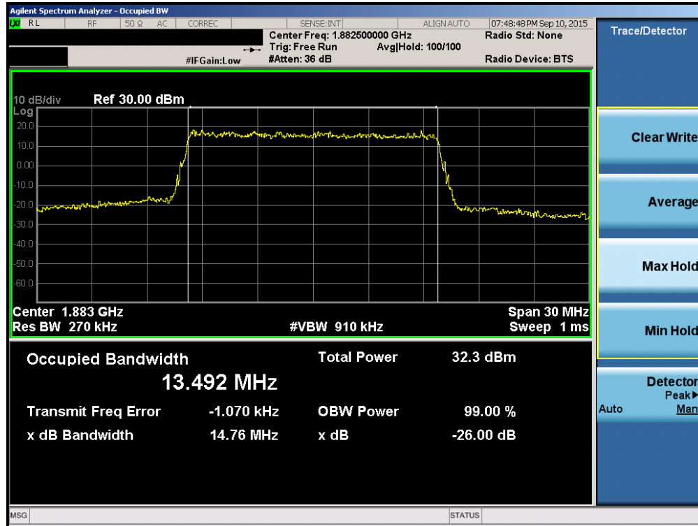
Plot 6-37. Occupied Bandwidth Plot (Band 2/25 – 15.0MHz QPSK – RB Size 75)
