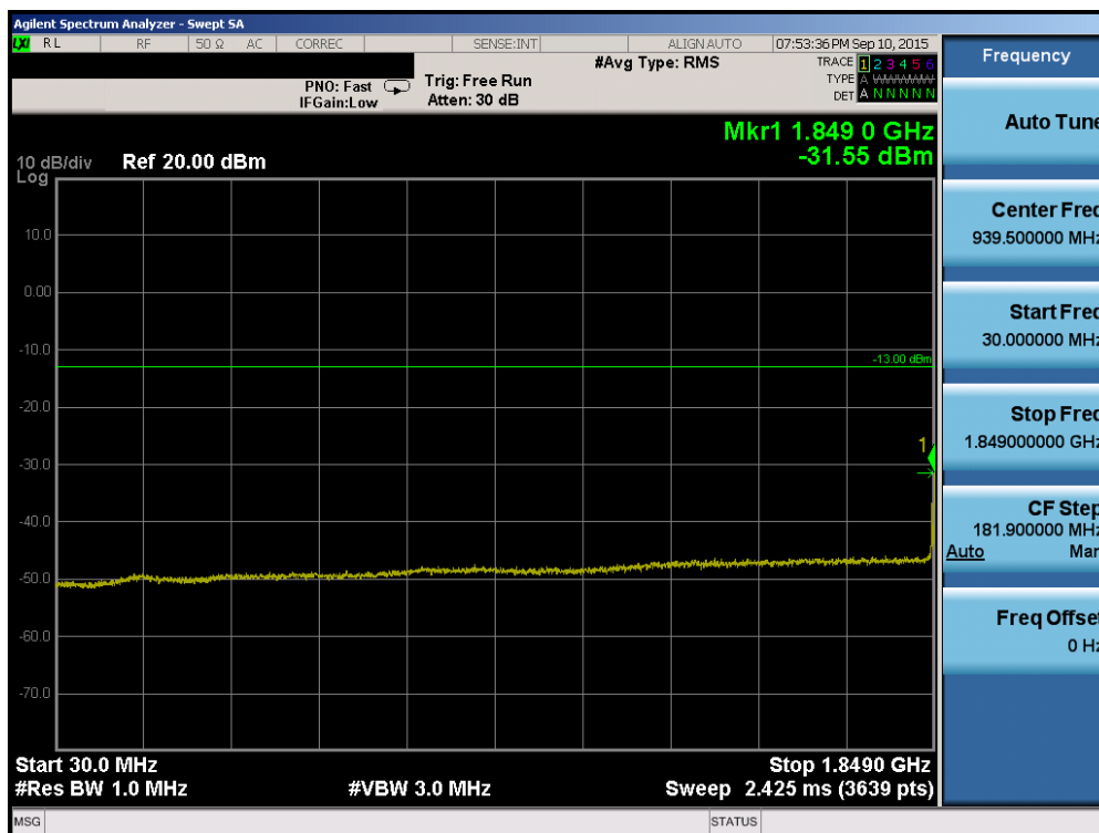
Plot 6-68. Conducted Spurious Plot (Band 2/25 – 20.0MHz QPSK – RB Size 1, RB Offset 0– Low Channel)
