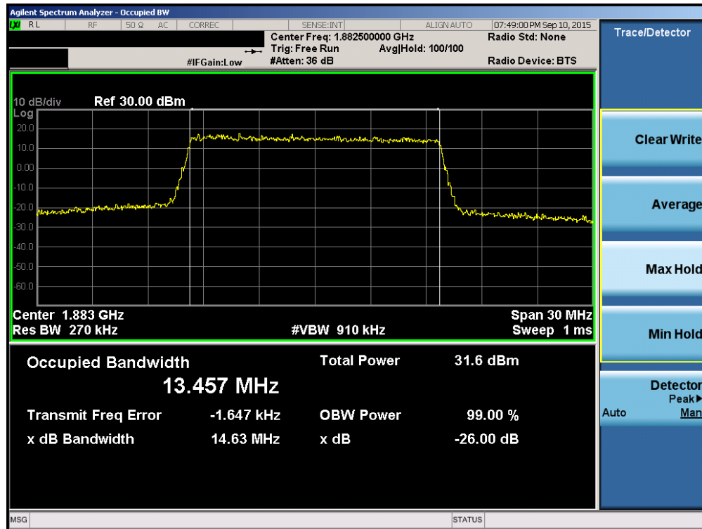
Plot 6-38. Occupied Bandwidth Plot (Band 2/25 – 15.0MHz 16-QAM – RB Size 75)
