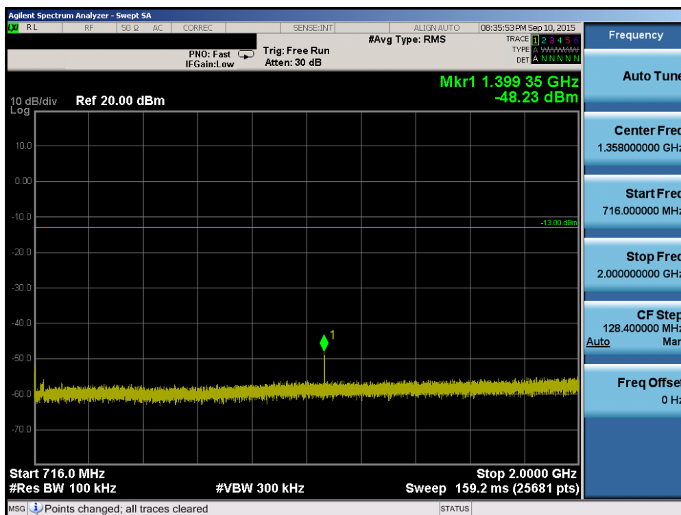
Plot 6-42. Conducted Spurious Plot (Band 12/17 – 10.0MHz QPSK – RB Size 1, RB Offset 0 – Low Channel)
