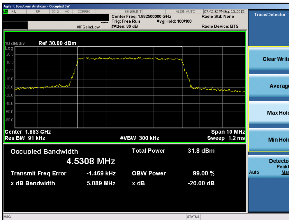
Plot 6-34. Occupied Bandwidth Plot (Band 2/25 – 5.0MHz 16-QAM – RB Size 25)
