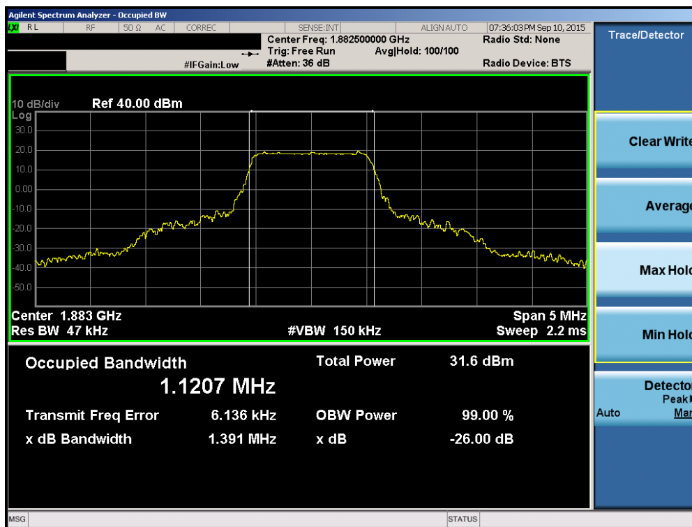
Plot 6-30. Occupied Bandwidth Plot (Band 2/25 – 1.4MHz 16-QAM – RB Size 6)
