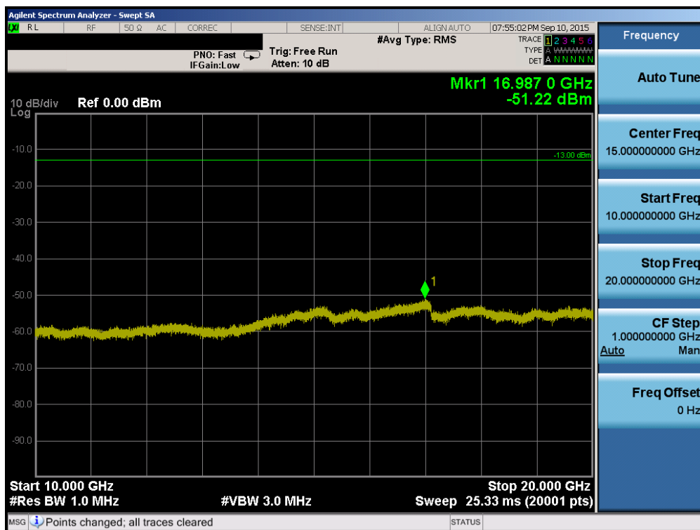
Plot 6-76. Conducted Spurious Plot (Band 2/25 – 20.0MHz QPSK – RB Size 1, RB Offset 0 – High Channel)
