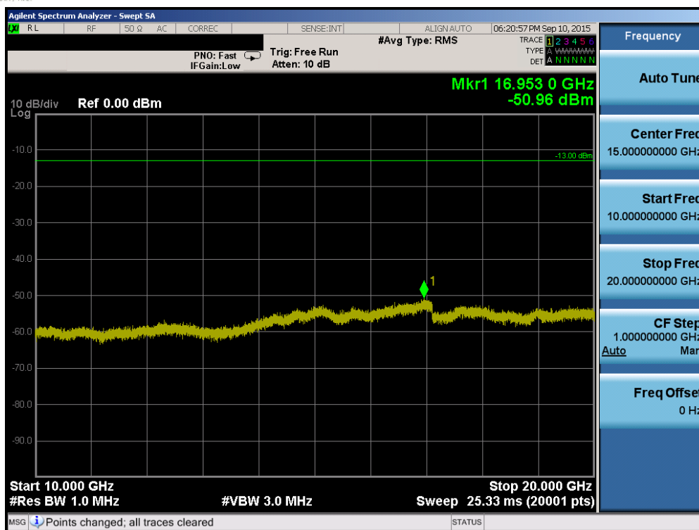
Plot 6-61. Conducted Spurious Plot (Band 4 – 20.0MHz QPSK – RB Size 1, RB Offset 0 – Low Channel)
