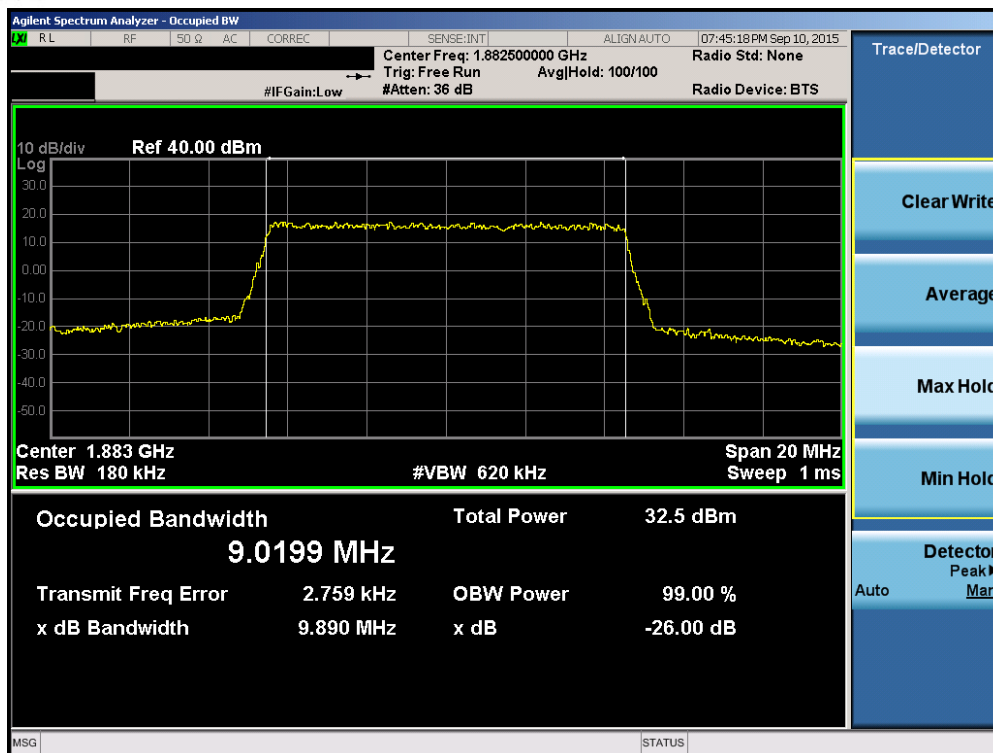
Plot 6-35. Occupied Bandwidth Plot (Band 2/25 – 10.0MHz QPSK – RB Size 50)
