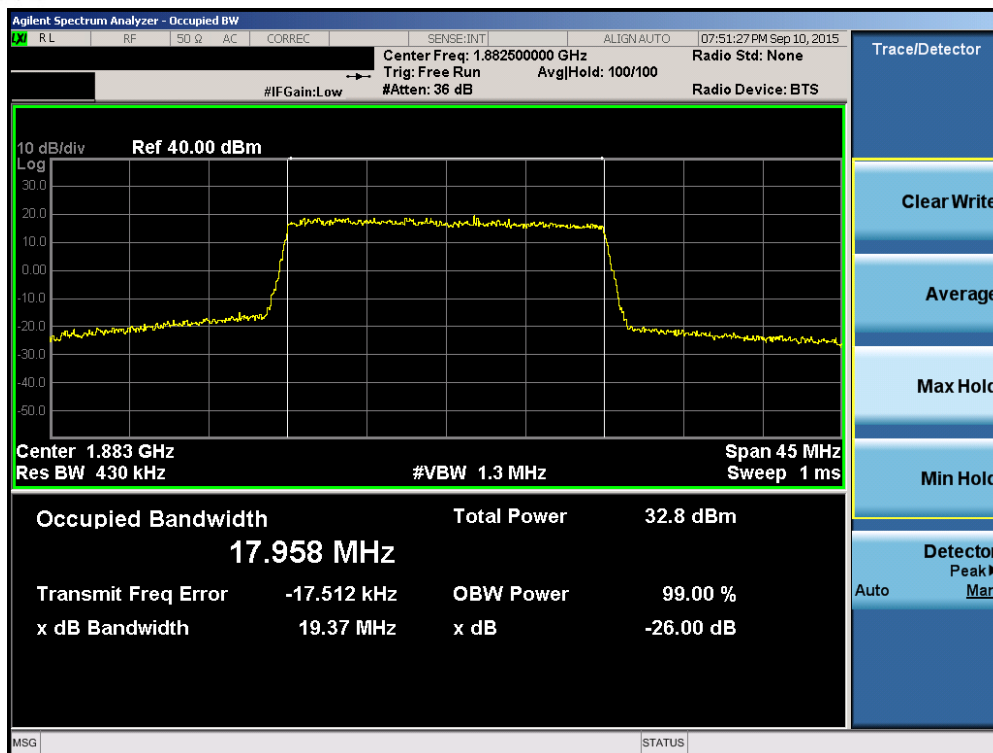
Plot 6-39. Occupied Bandwidth Plot (Band 2/25 – 20.0MHz QPSK – RB Size 100)
