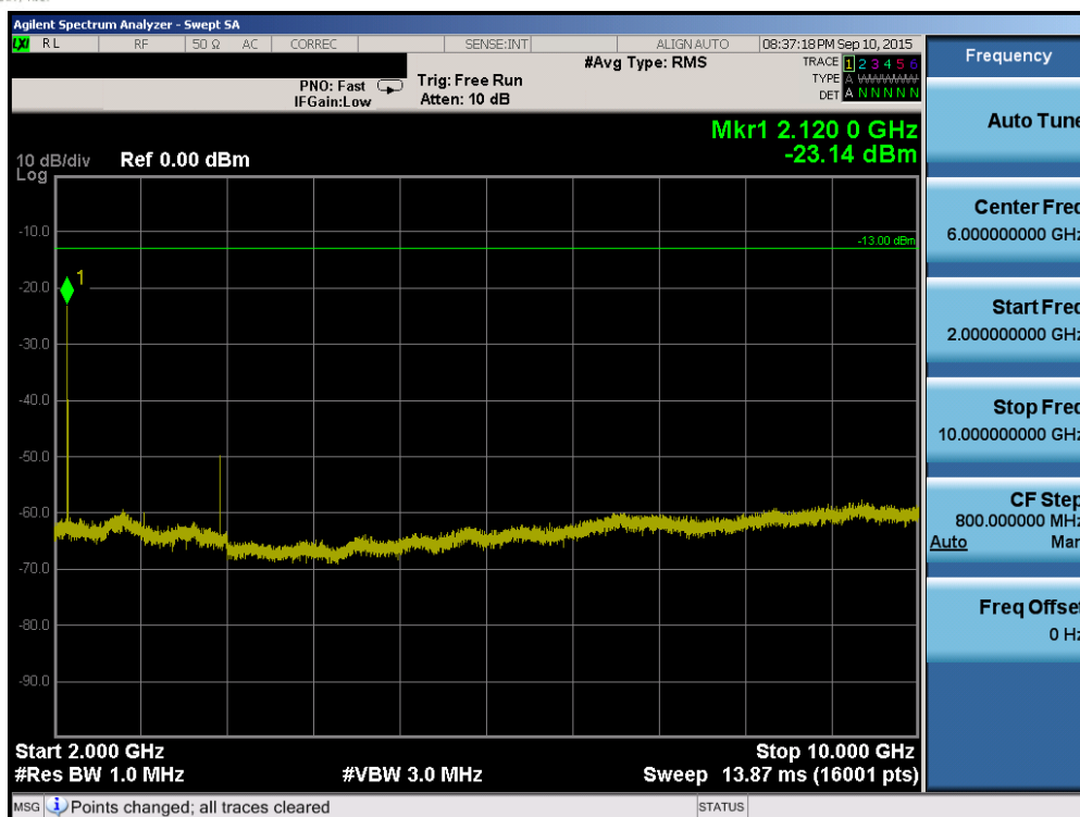
Plot 6-49. Conducted Spurious Plot (Band 12/17 – 10.0MHz QPSK – RB Size 1, RB Offset 0 – High Channel)
