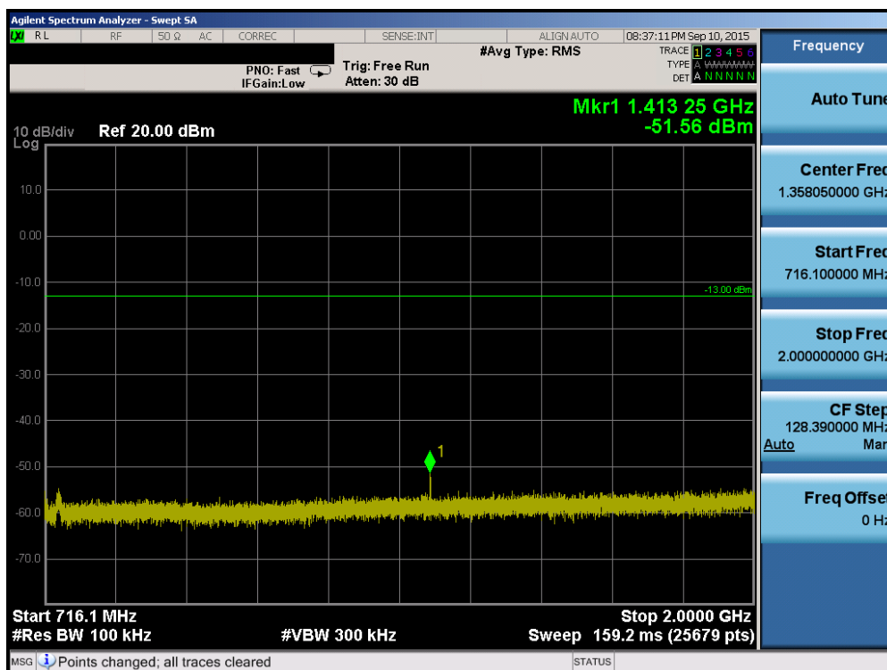
Plot 6-48. Conducted Spurious Plot (Band 12/17 – 10.0MHz QPSK – RB Size 1, RB Offset 0 – High Channel)
