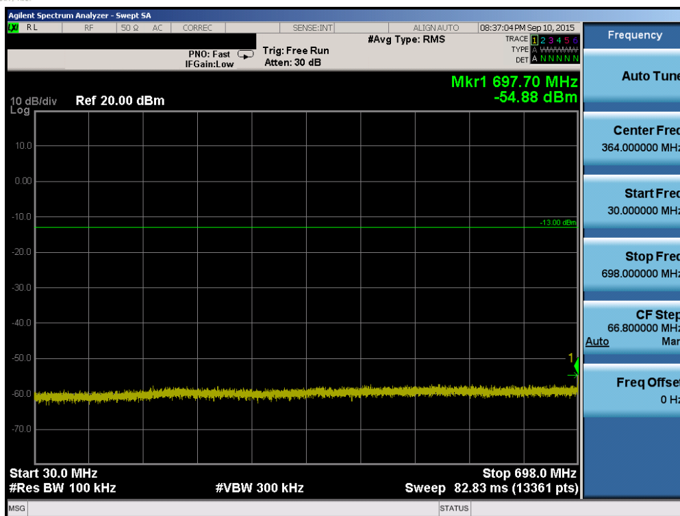
Plot 6-47. Conducted Spurious Plot (Band 12/17 – 10.0MHz QPSK – RB Size 1, RB Offset 0 – High Channel)
