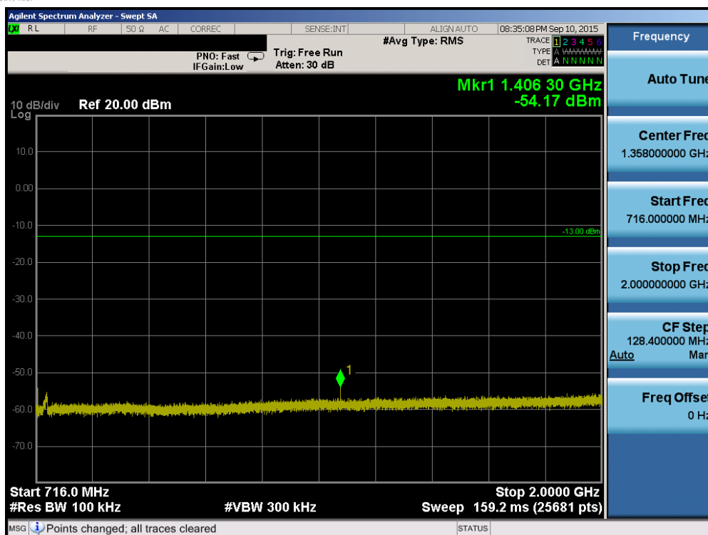
Plot 6-45. Conducted Spurious Plot (Band 12/17 – 10.0MHz QPSK – RB Size 1, RB Offset 0 – Mid Channel)
