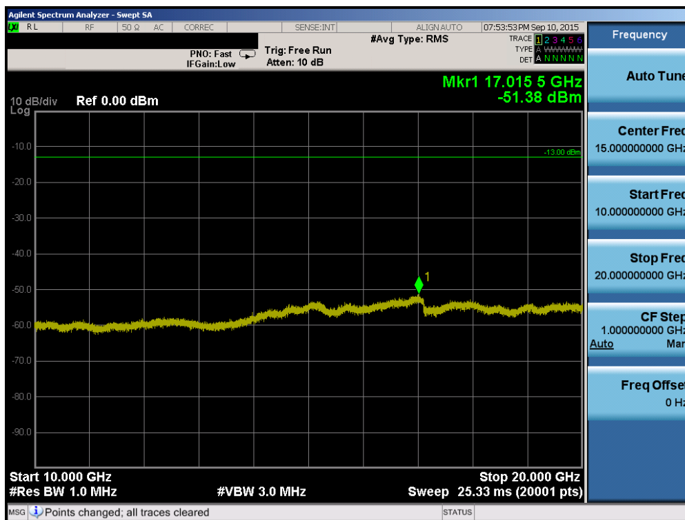
Plot 6-70. Conducted Spurious Plot (Band 2/25 – 20.0MHz QPSK – RB Size 1, RB Offset 0 – Low Channel)
