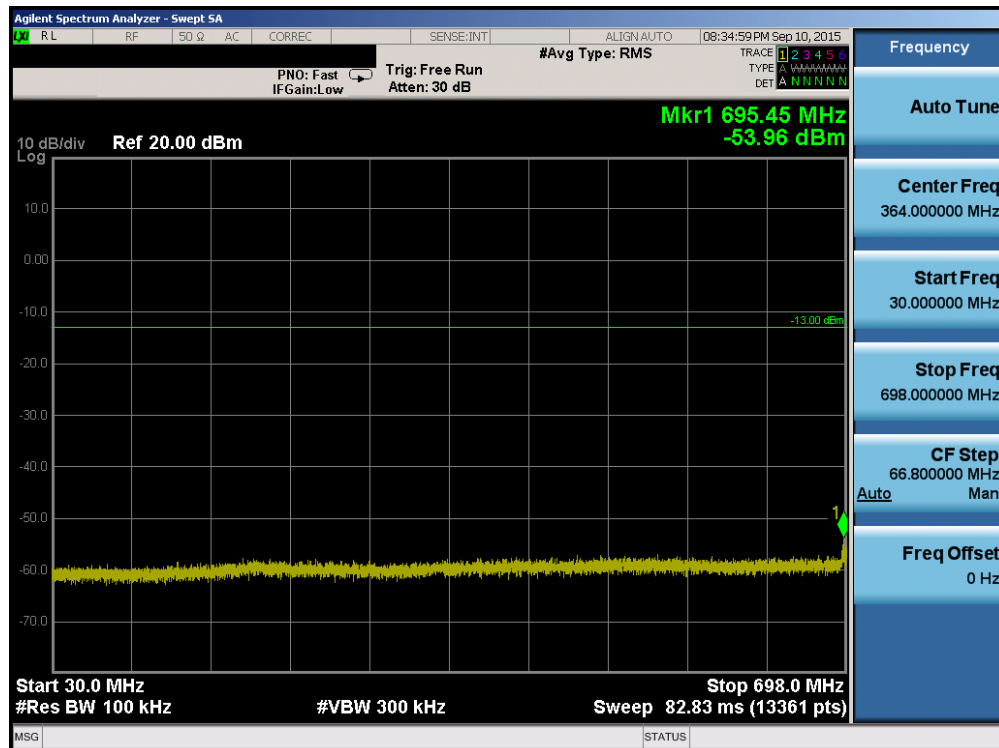
Plot 6-44. Conducted Spurious Plot (Band 12/17 – 10.0MHz QPSK – RB Size 1, RB Offset 0 – Mid Channel)
