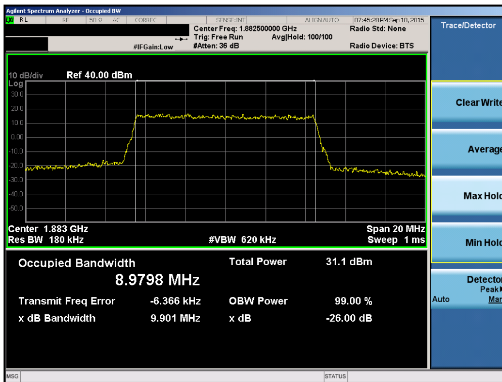
Plot 6-36. Occupied Bandwidth Plot (Band 2/25 – 10.0MHz 16-QAM – RB Size 50)
