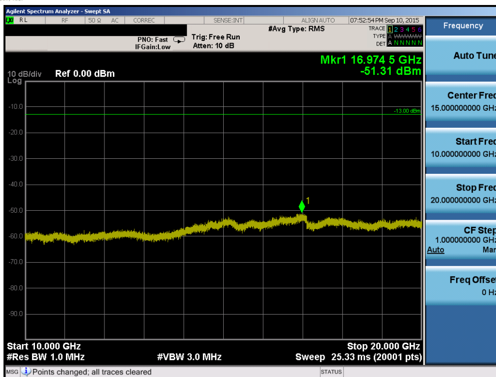
Plot 6-73. Conducted Spurious Plot (Band 2/25 – 20.0MHz QPSK – RB Size 1, RB Offset 0 – Mid Channel)
