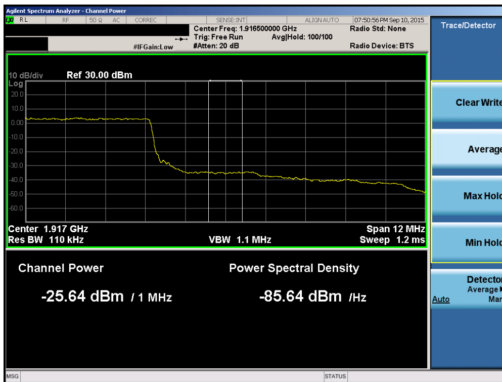
Plot 6-148. Upper Extended Band Edge Plot (Band 2/25 – 15.0MHz QPSK – RB Size 75)
