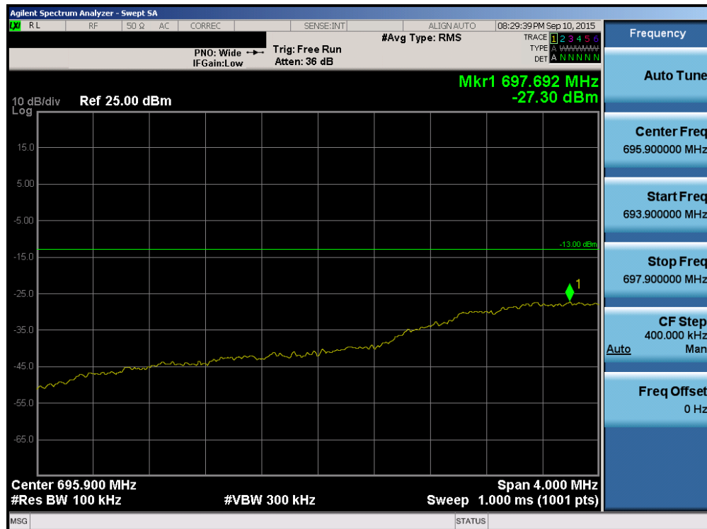
Plot 6-82. Lower Extended Band Edge Plot (Band 12 – 3.0MHz QPSK – RB Size 15)
