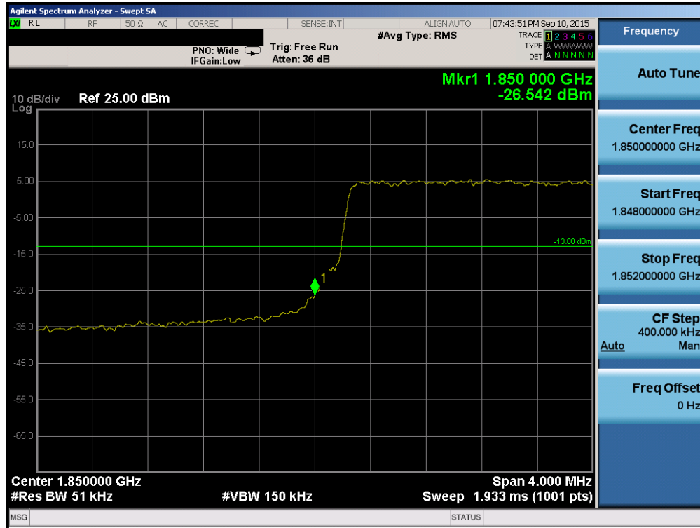
Plot 6-137. Lower Band Edge Plot (Band 2/25 – 5.0MHz QPSK – RB Size 25)
