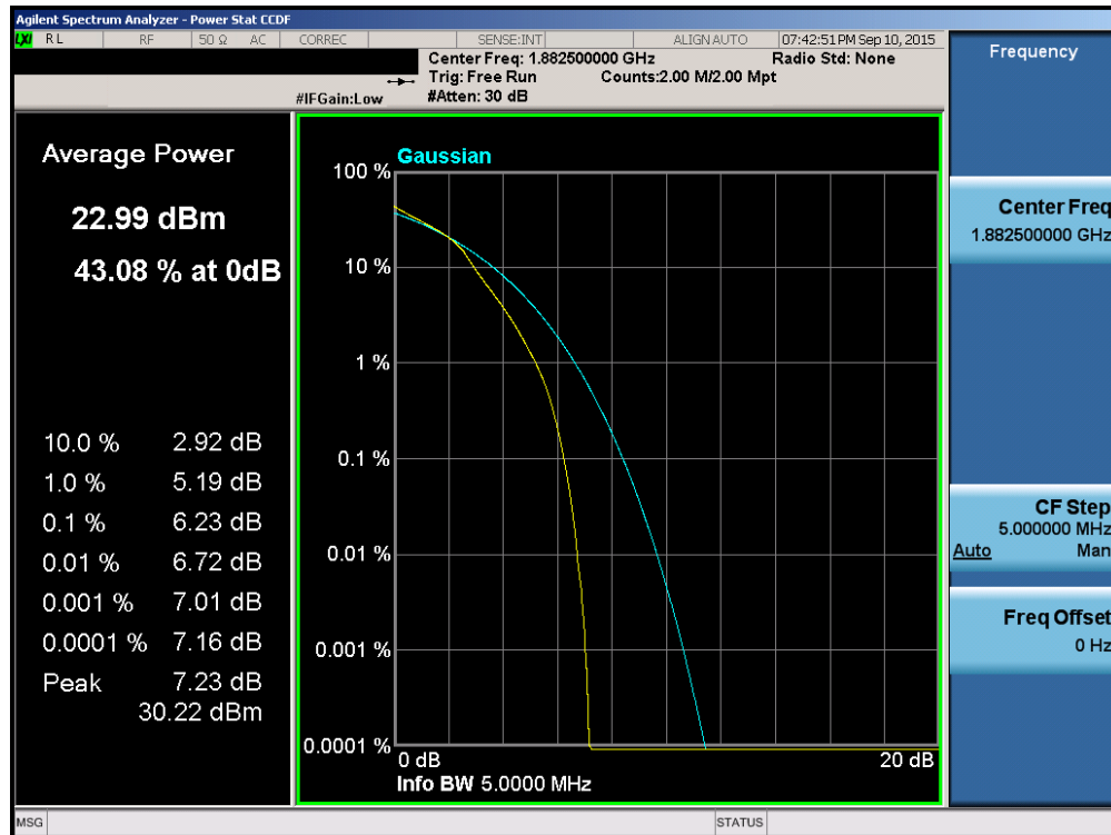
Plot 6-158. PAR Plot (Band 2/25 – 5.0MHz 16-QAM – RB Size 25)
