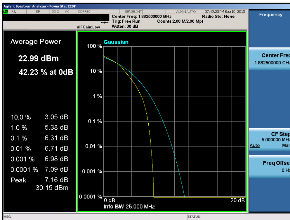
Plot 6-162. PAR Plot (Band 2/25 – 15.0MHz 16-QAM – RB Size 75)
