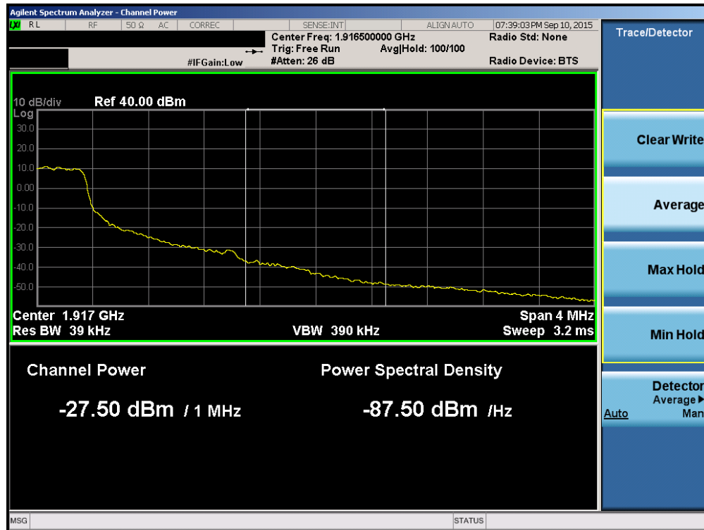
Plot 6-132. Upper Extended Band Edge Plot (Band 2/25 – 1.4MHz QPSK – RB Size 6)
