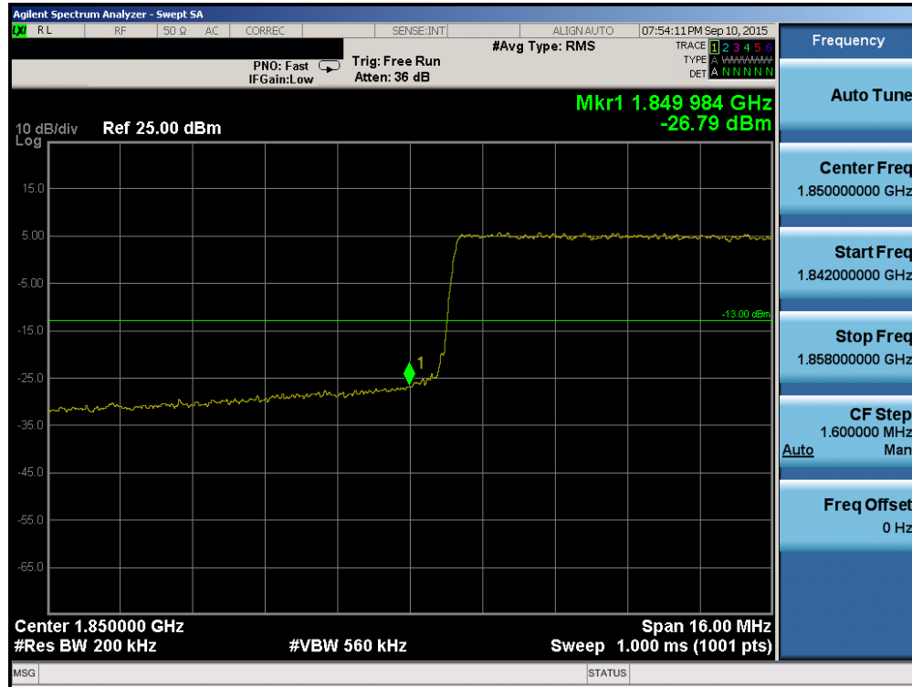
Plot 6-149. Lower Band Edge Plot (Band 2/25 – 20.0MHz QPSK – RB Size 100)
