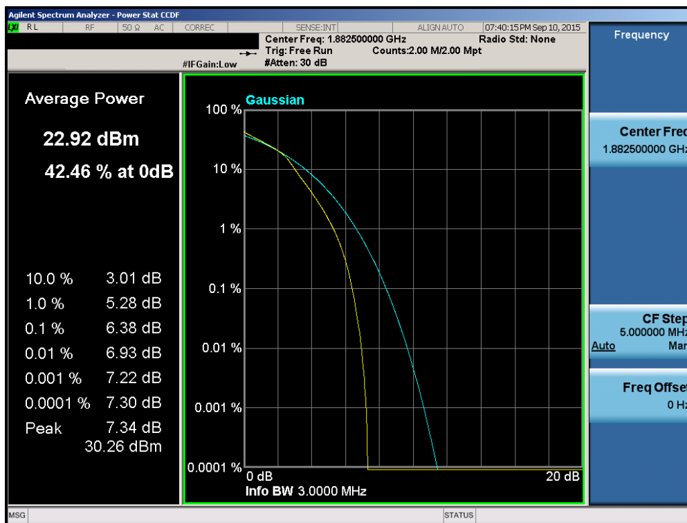
Plot 6-156. PAR Plot (Band 2/25 – 3.0MHz 16-QAM – RB Size 15)
