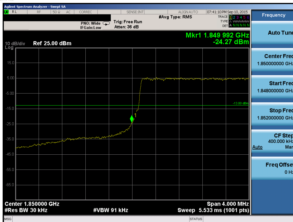
Plot 6-133. Lower Band Edge Plot (Band 2/25 – 3.0MHz QPSK – RB Size 15)
