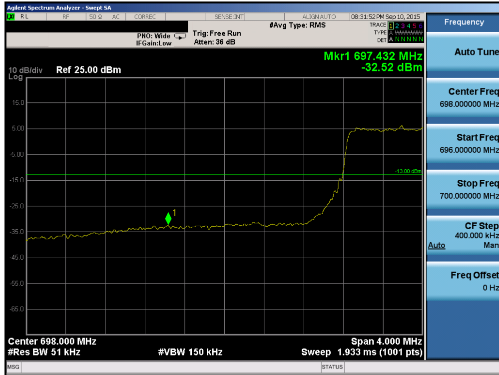
Plot 6-85. Lower Band Edge Plot (Band 12/17 – 5.0MHz QPSK – RB Size 25)
