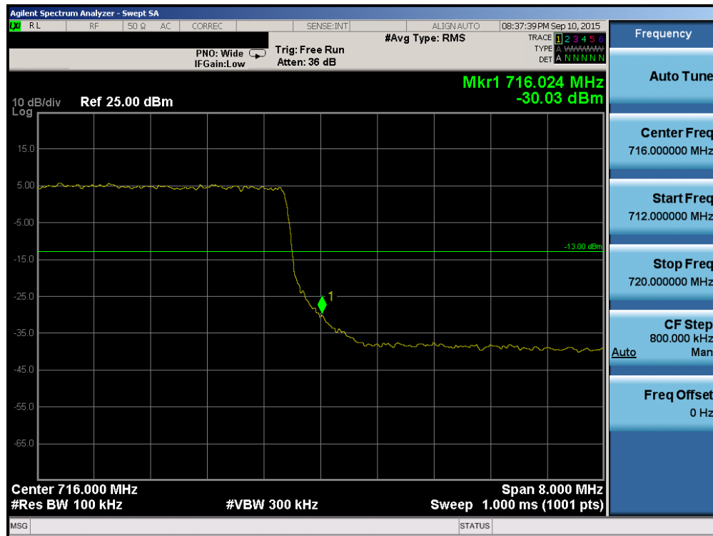
Plot 6-90. Upper Band Edge Plot (Band 12/17 – 10.0MHz QPSK – RB Size 50)
