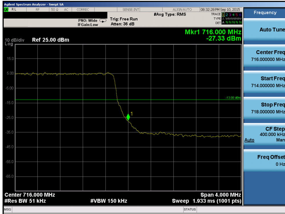
Plot 6-87. Upper Band Edge Plot (Band 12/17 - 5.0MHz QPSK - RB Size 25)
