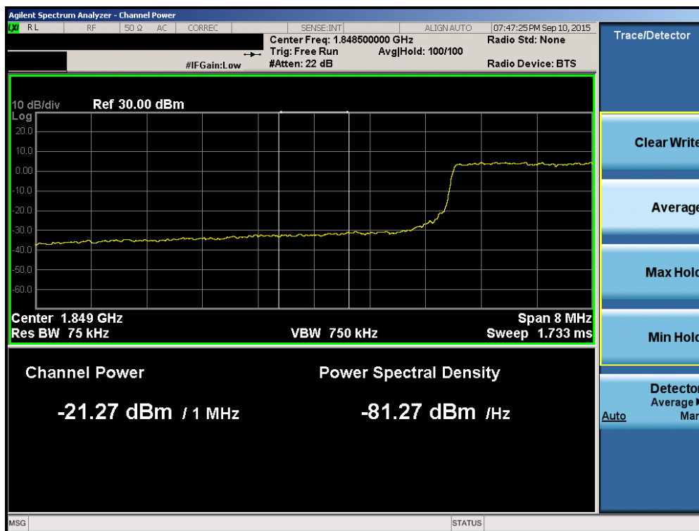
Plot 6-142. Lower Extended Band Edge Plot (Band 2/25 – 10.0MHz QPSK – RB Size 50)
