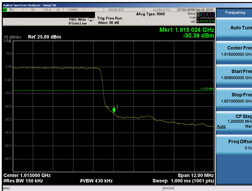
Plot 6-147. Upper Band Edge Plot (Band 2/25 – 15.0MHz QPSK – RB Size 75)
