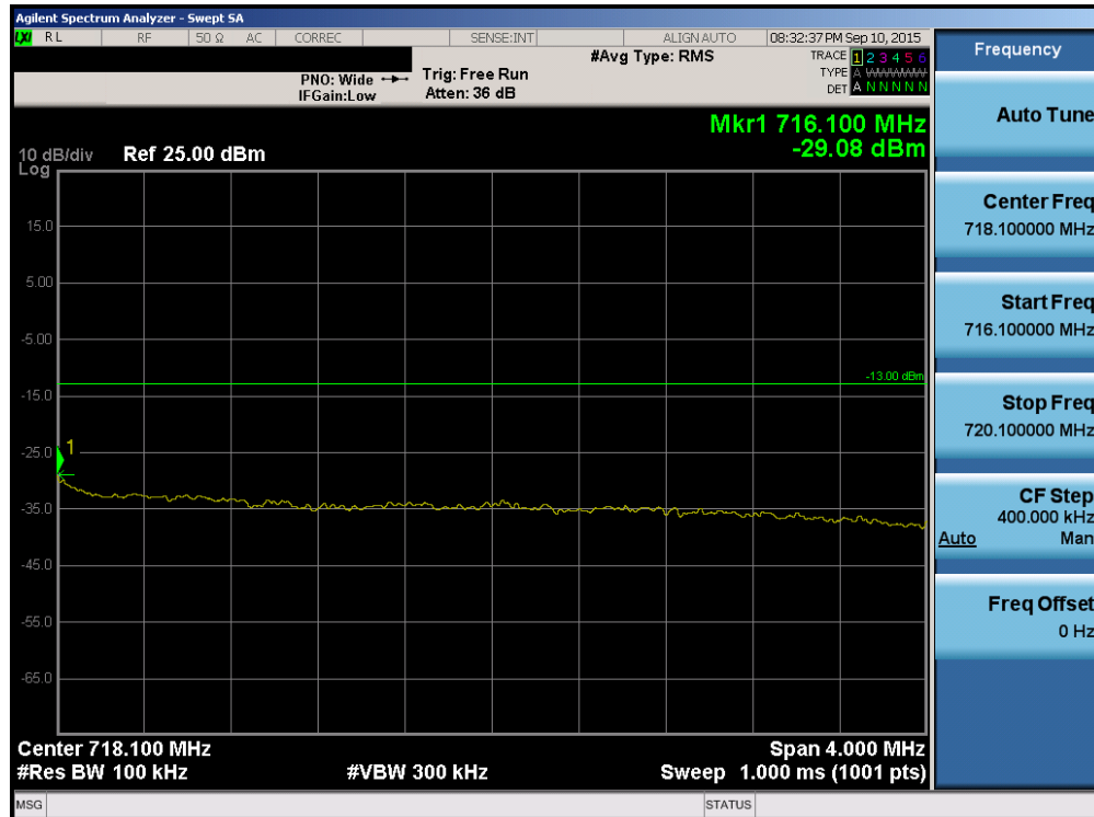
Plot 6-88. Upper Extended Band Edge Plot (Band 12/17 - 5.0MHz QPSK - RB Size 25)
