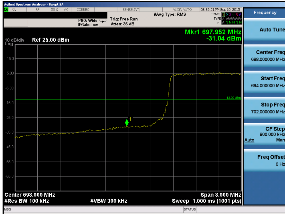
Plot 6-89. Lower Band Edge Plot (Band 12/17 – 10.0MHz QPSK – RB Size 50)
