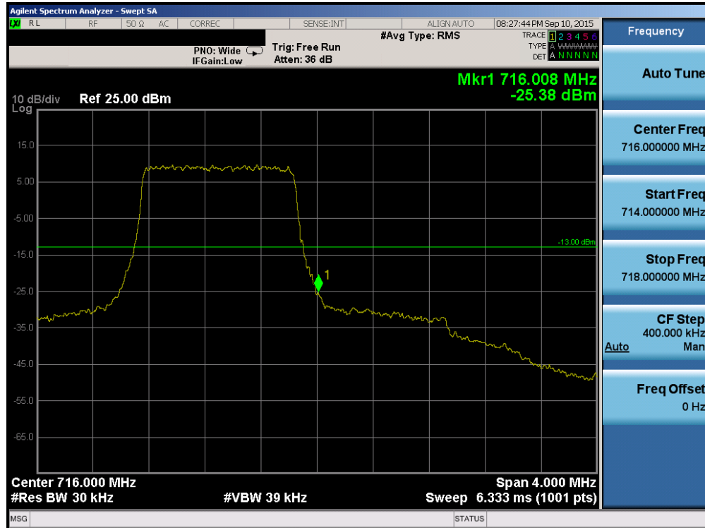
Plot 6-79. Upper Band Edge Plot (Band 12 – 1.4MHz QPSK – RB Size 6)
