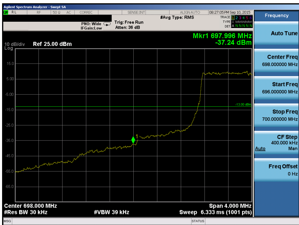
Plot 6-77. Lower Band Edge Plot (Band 12 – 1.4MHz QPSK – RB Size 6)
