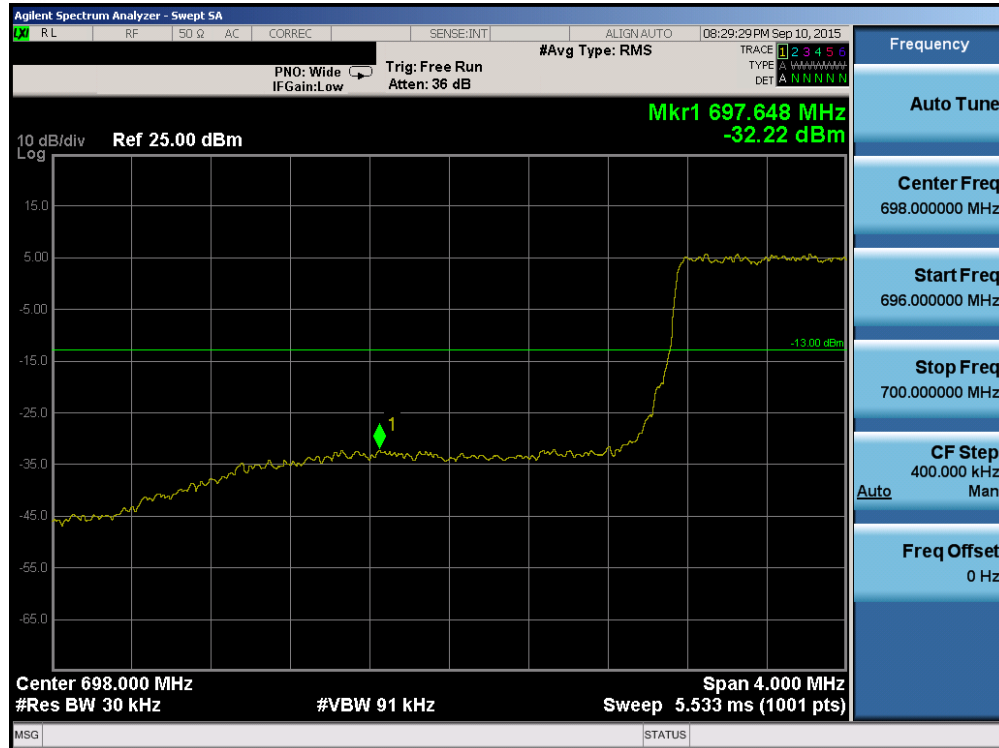
Plot 6-81. Lower Band Edge Plot (Band 12 – 3.0MHz QPSK – RB Size 15)
