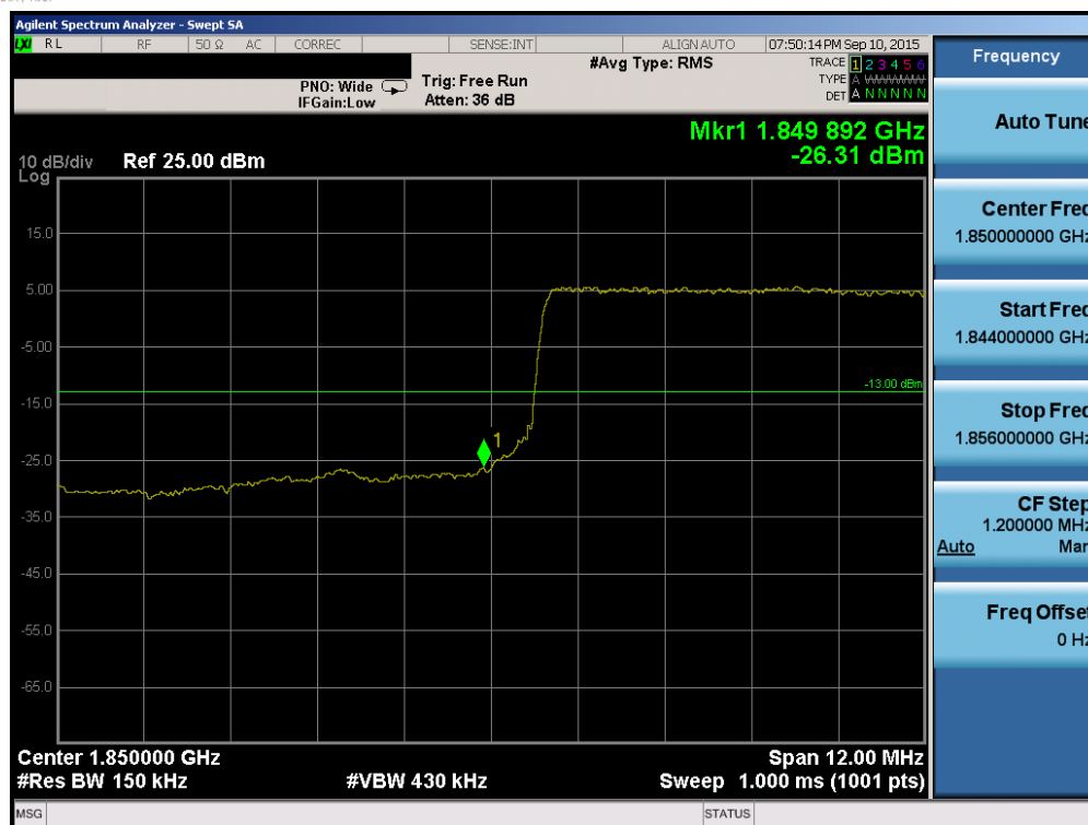
Plot 6-145. Lower Band Edge Plot (Band 2/25 – 15.0MHz QPSK – RB Size 75)
