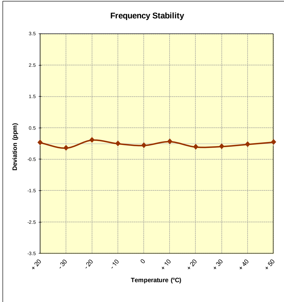
Figure 6-8. Frequency Stability Graph (Band 5)
