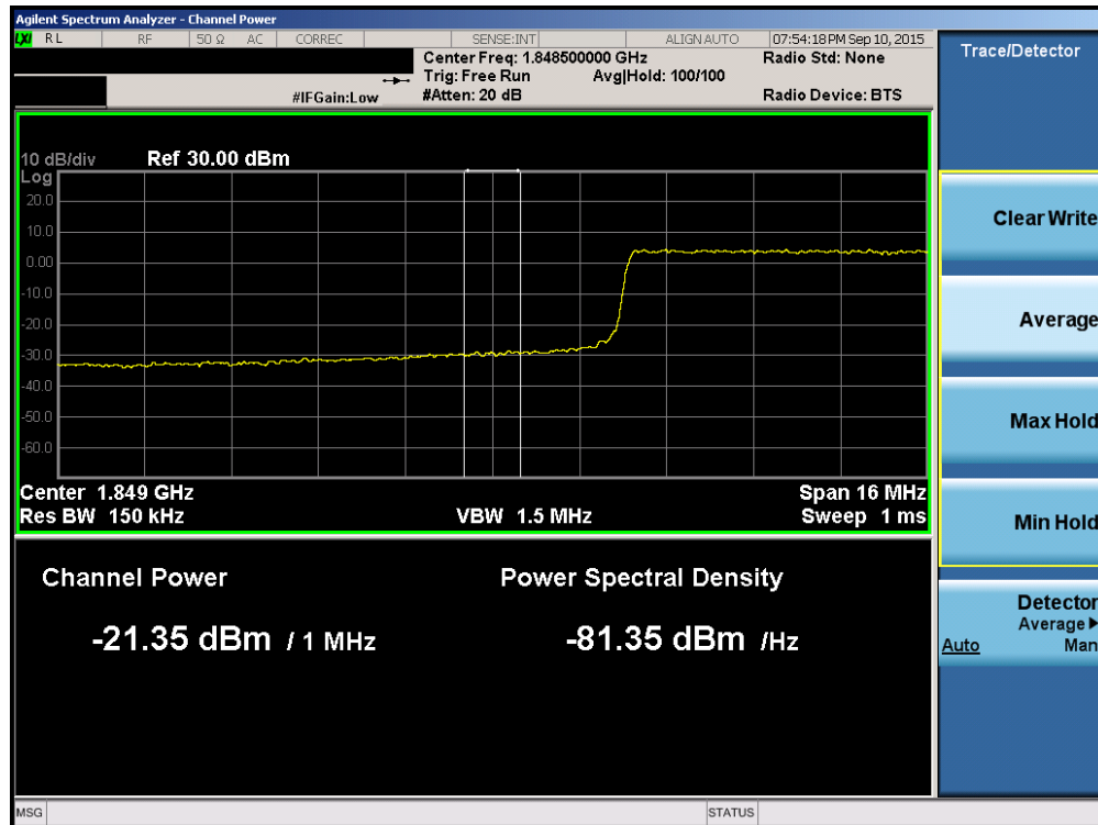
Plot 6-150. Lower Extended Band Edge Plot (Band 2/25 – 20.0MHz QPSK – RB Size 100)
