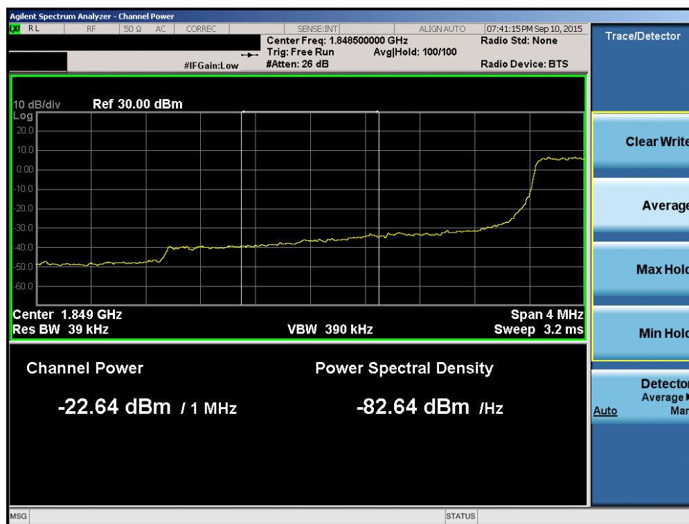
Plot 6-134. Lower Extended Band Edge Plot (Band 2/25 – 3.0MHz QPSK – RB Size 15)
