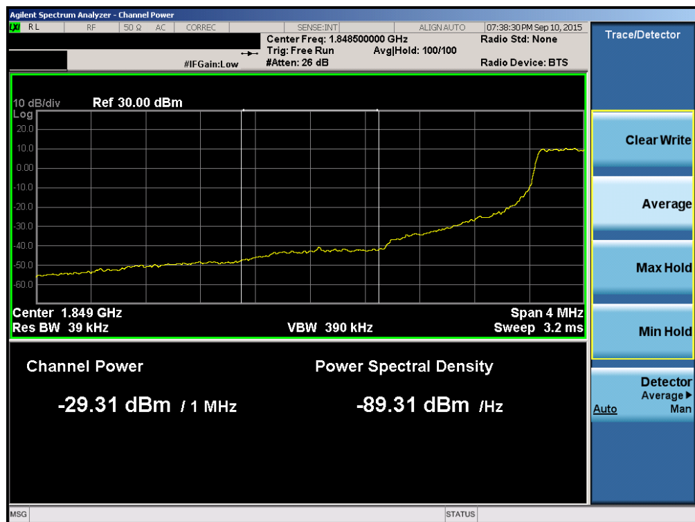
Plot 6-130. Lower Extended Band Edge Plot (Band 2/25 – 1.4MHz QPSK – RB Size 6)
