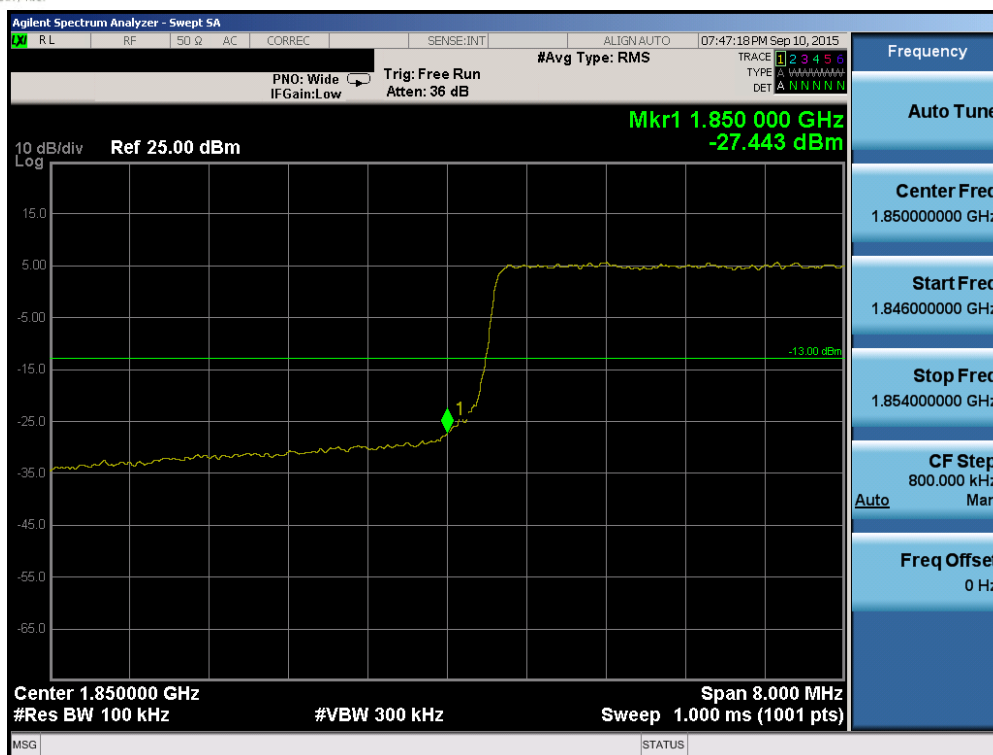
Plot 6-141. Lower Band Edge Plot (Band 2/25 – 10.0MHz QPSK – RB Size 50)
