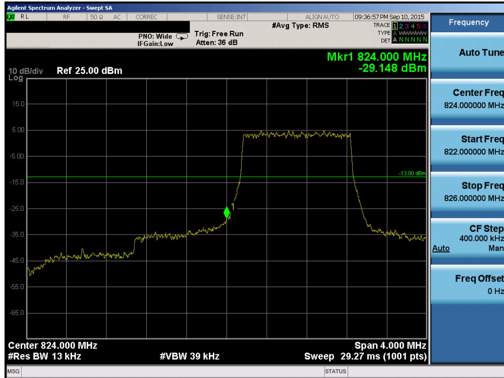
Plot 6-91. Lower Band Edge Plot (Band 5 – 1.4MHz QPSK – RB Size 6)
