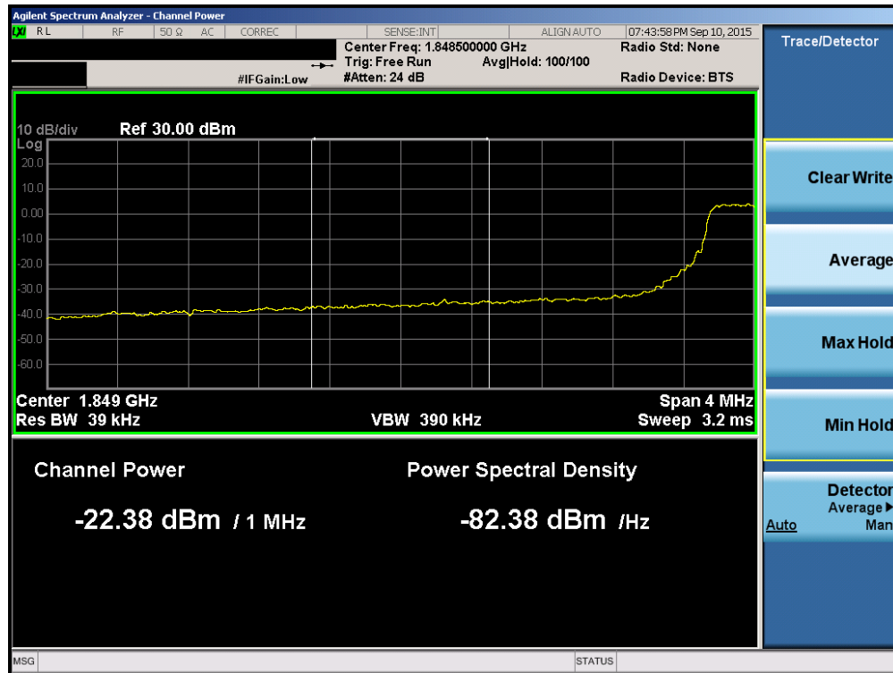
Plot 6-138. Lower Extended Band Edge Plot (Band 2/25 – 5.0MHz QPSK – RB Size 25)
