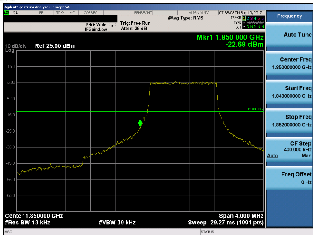
Plot 6-129. Lower Band Edge Plot (Band 2/25 – 1.4MHz QPSK – RB Size 6)
