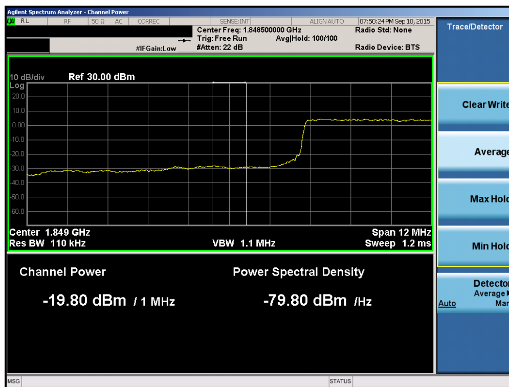
Plot 6-146. Lower Extended Band Edge Plot (Band 2/25 – 15.0MHz QPSK – RB Size 75)
