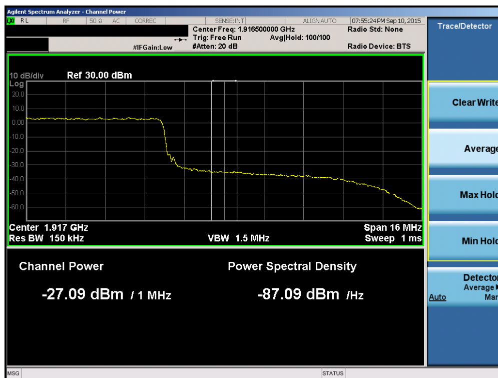
Plot 6-152. Upper Extended Band Edge Plot (Band 2/25 – 20.0MHz QPSK – RB Size 100)
