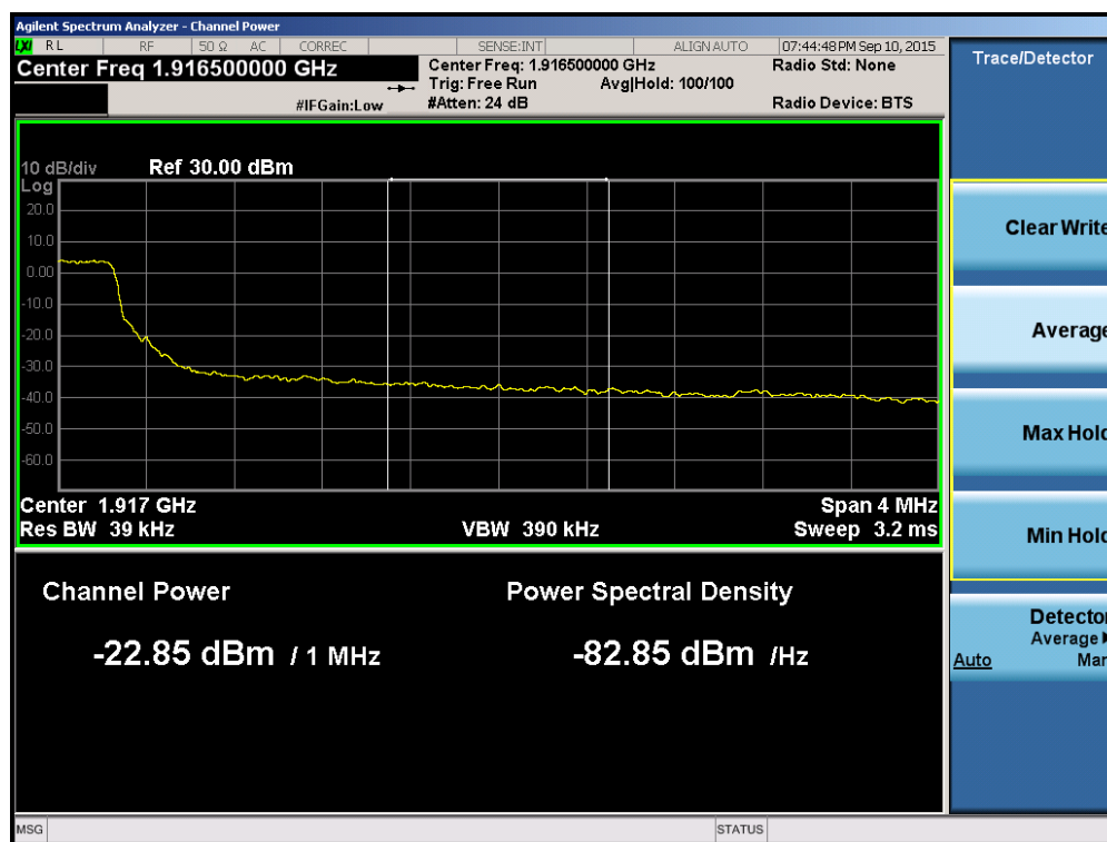
Plot 6-140. Upper Extended Band Edge Plot (Band 2/25 – 5.0MHz QPSK – RB Size 25)
