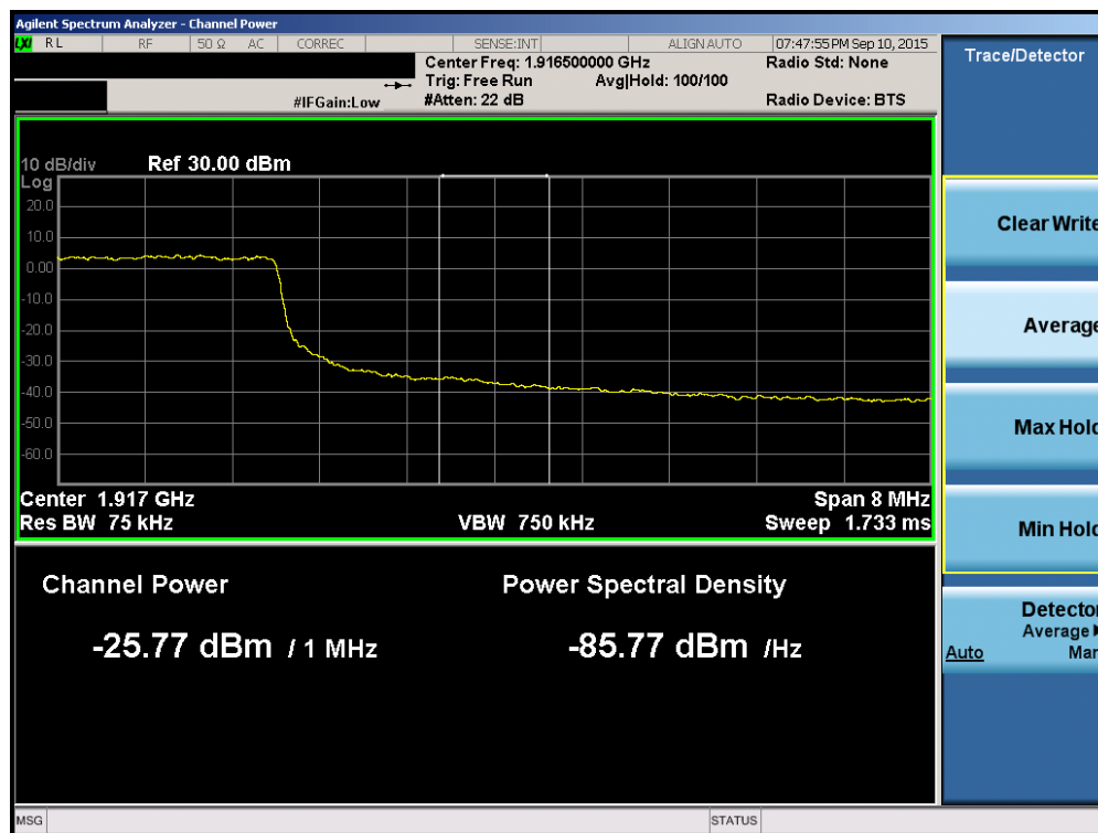
Plot 6-144. Upper Extended Band Edge Plot (Band 2/25 – 10.0MHz QPSK – RB Size 50)
