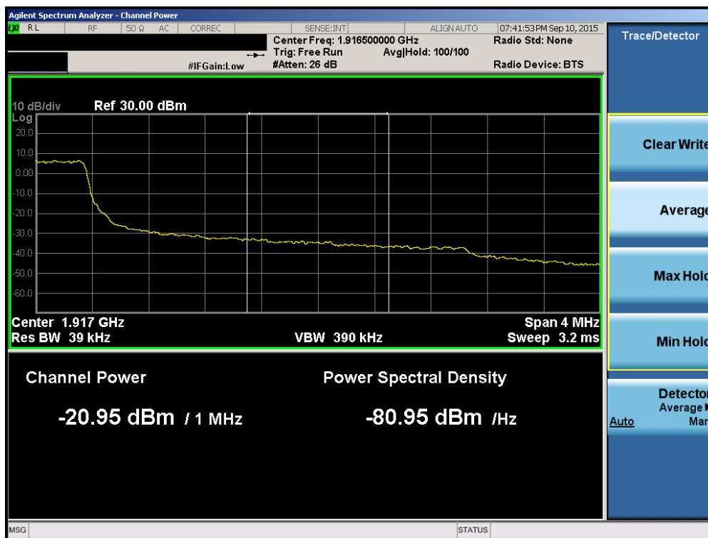
Plot 6-136. Upper Extended Band Edge Plot (Band 2/25 – 3.0MHz QPSK – RB Size 15)
