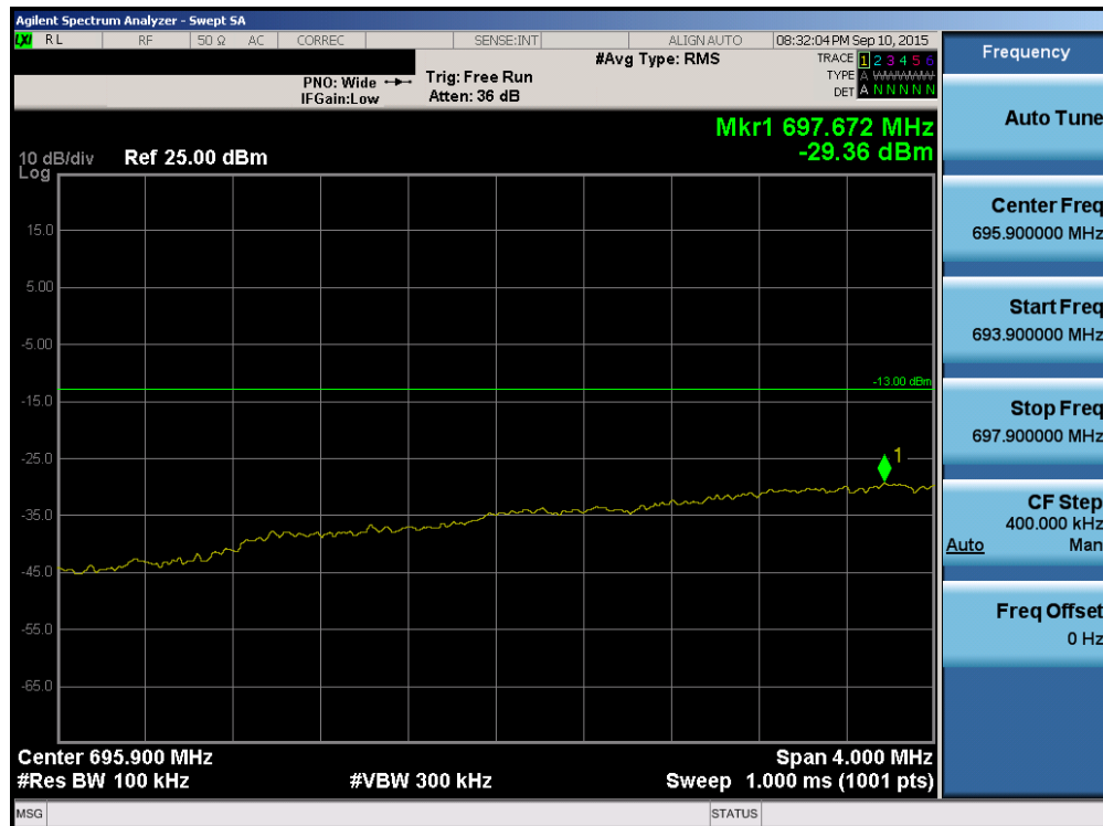
Plot 6-86. Lower Extended Band Edge Plot (Band 12/17 – 5.0MHz QPSK – RB Size 25)
