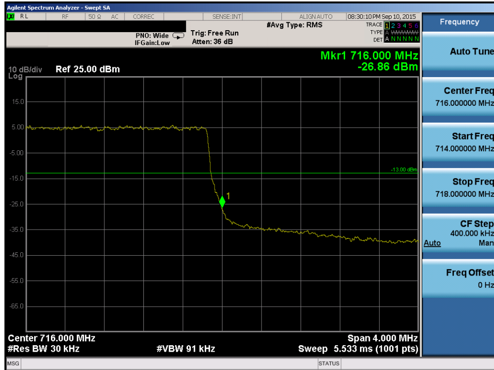
Plot 6-83. Upper Band Edge Plot (Band 12 – 3.0MHz QPSK – RB Size 15)
