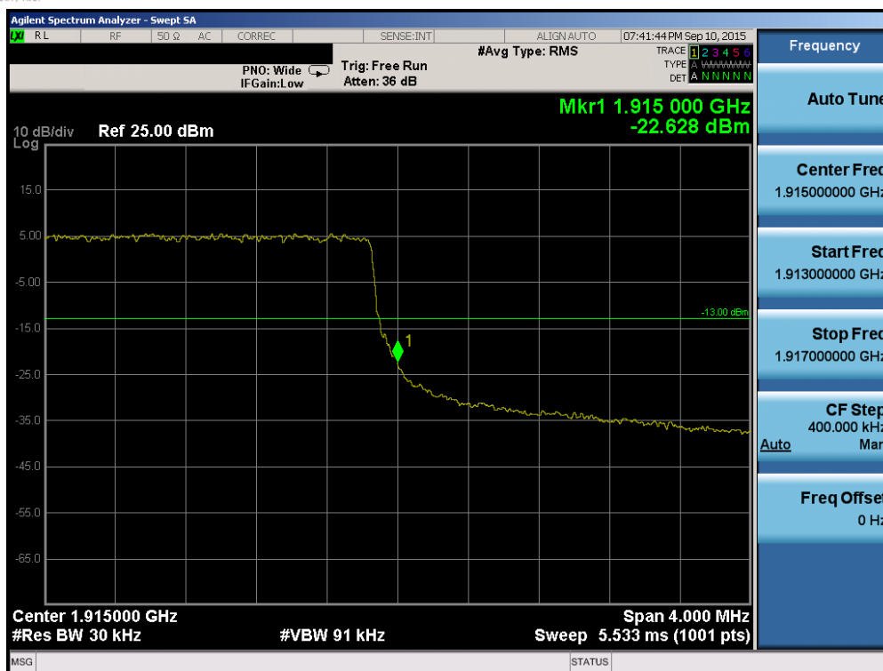
Plot 6-135. Upper Band Edge Plot (Band 2/25 – 3.0MHz QPSK – RB Size 15)
