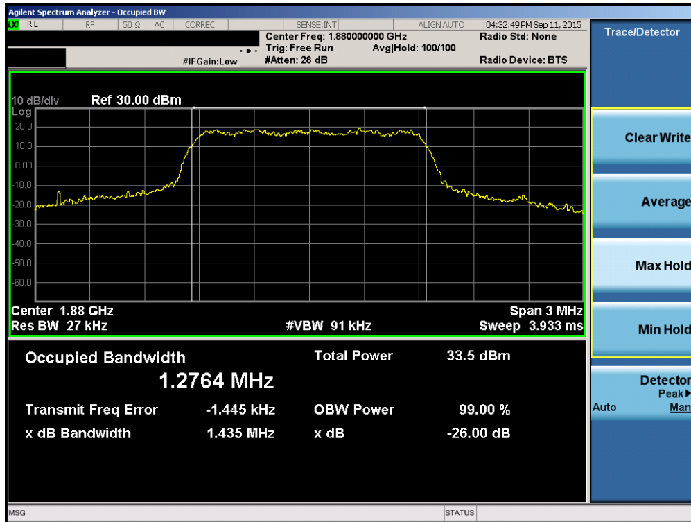
Plot 6-2. Occupied Bandwidth Plot (PCS CDMA/EvDO Mode – Ch. 600)
