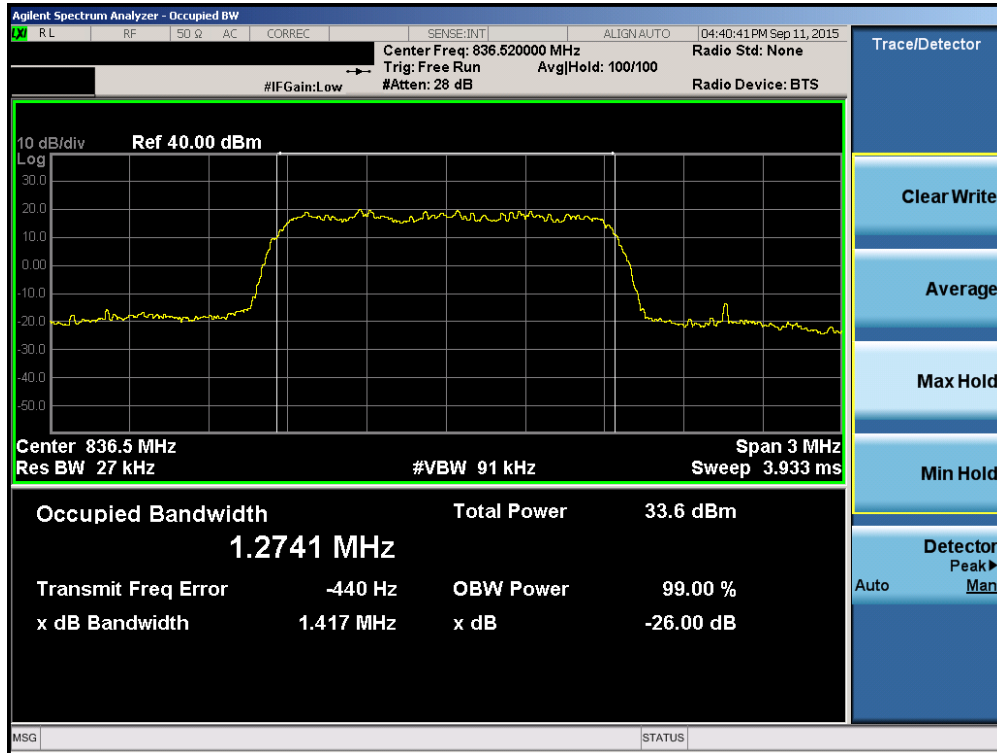
Plot 6-1. Occupied Bandwidth Plot (Cellular CDMA/EvDO Mode – Ch. 384)
