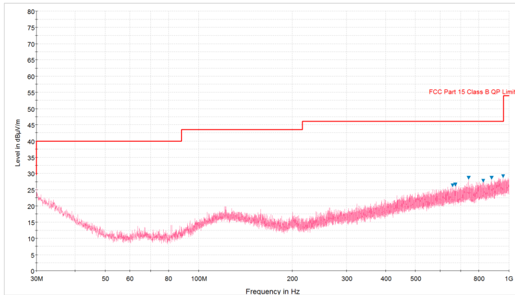
Plot 6-92. Radiated Spurious Plot below 1GHz (802.11a – U3 Ch. 157, Ant. Pol. V)
