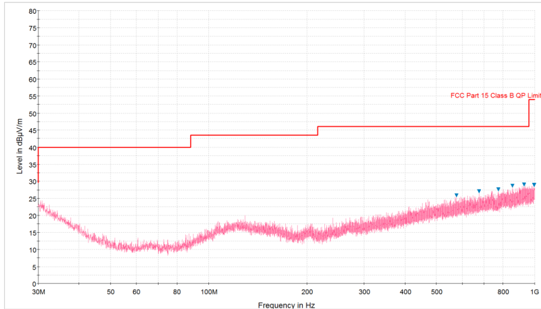
Plot 6-91. Radiated Spurious Plot below 1GHz (802.11a – U3 Ch. 157, Ant. Pol. H)
