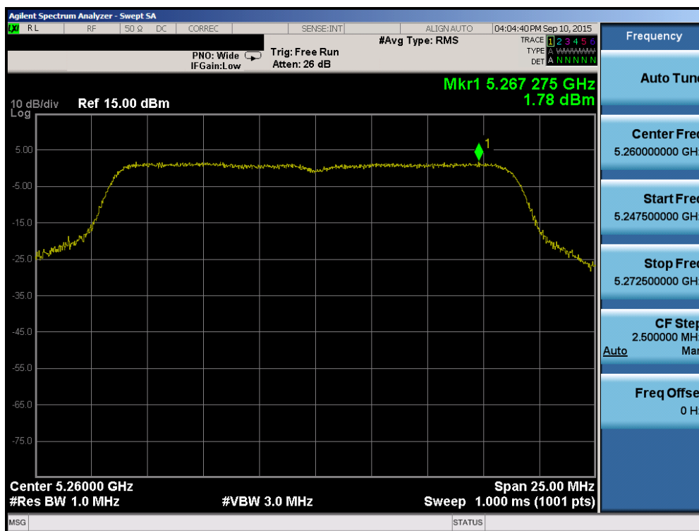
Plot 6-45. Power Spectral Density Plot (20MHz BW 802.11n (UNII Band 2A) – Ch. 52)
