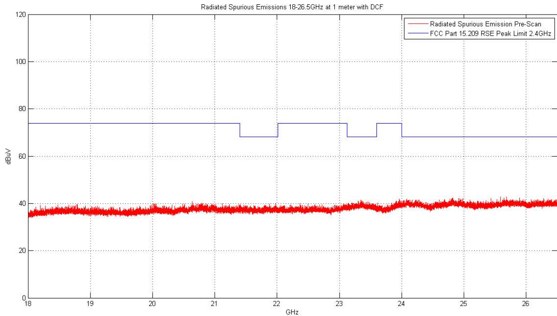
Plot 7-48. Radiated Spurious Plot above 18GHz (Pol. H)
