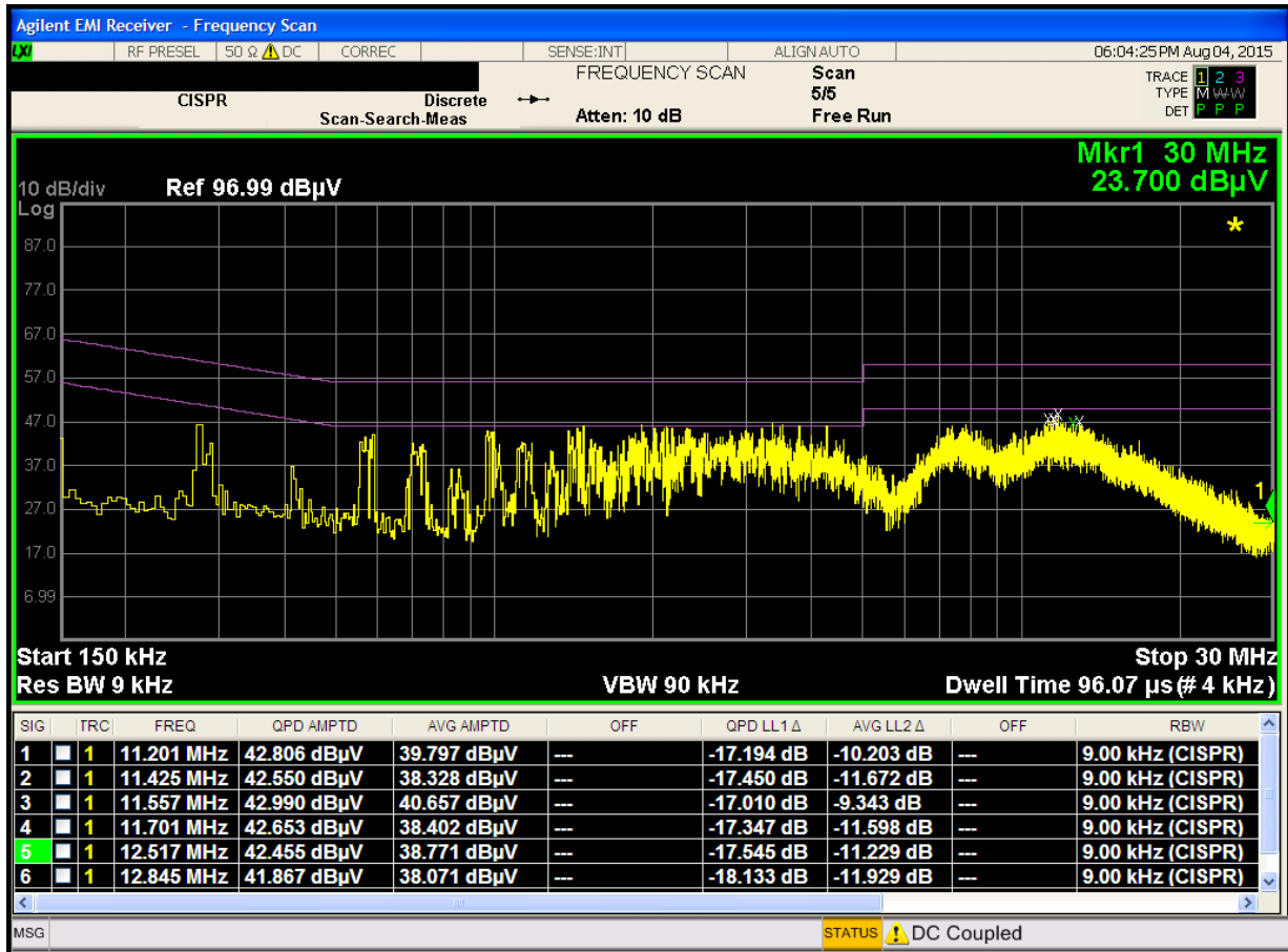
Plot 7-54. Line-Conducted Test Plot (L1)
