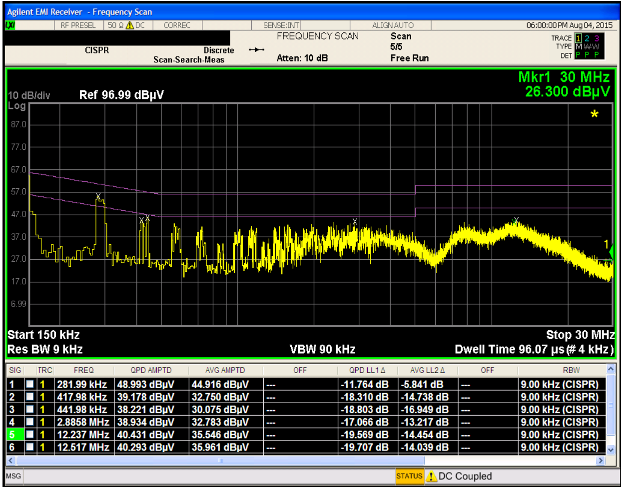
Plot 7-55. Line-Conducted Test Plot (N)
