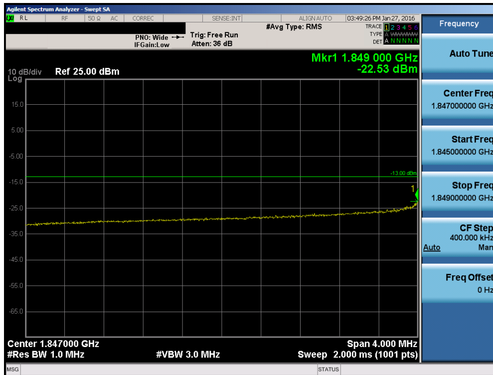
Plot 7-105. Lower Extended Band Edge Plot (Band 2 – 10.0MHz QPSK – RB Size 50)
