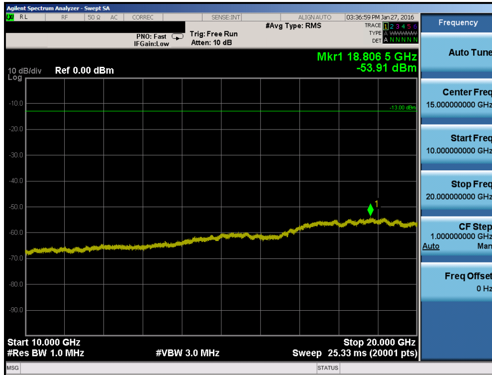
Plot 7-53. Conducted Spurious Plot (Band 2 – 20.0MHz QPSK – RB Size 1, RB Offset 0 – Low Channel)
