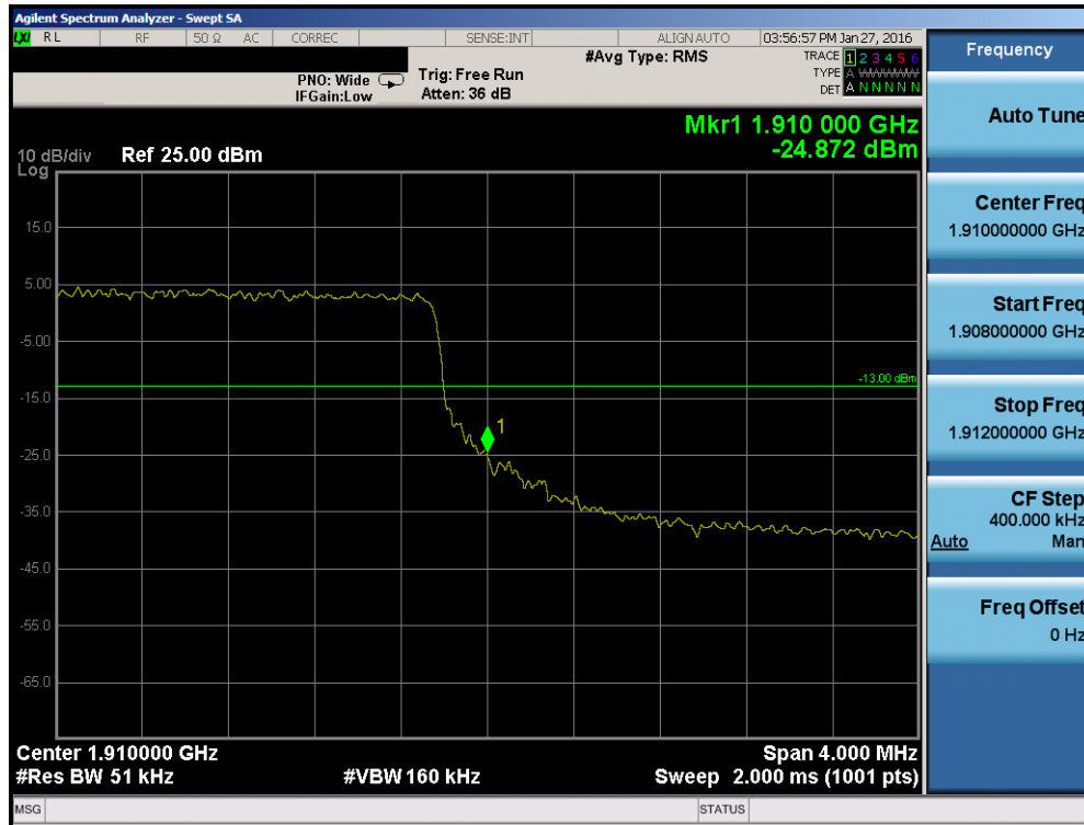
Plot 7-102. Upper Band Edge Plot (Band 2 – 5.0MHz QPSK – RB Size 25)
