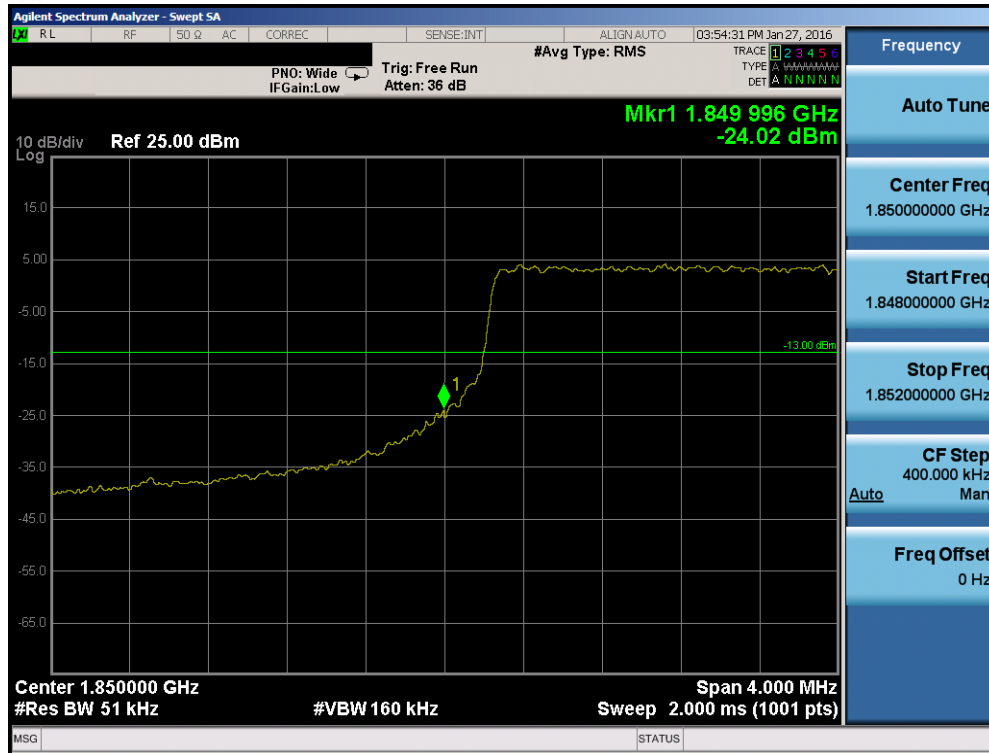
Plot 7-100. Lower Band Edge Plot (Band 2 – 5.0MHz QPSK – RB Size 25)
