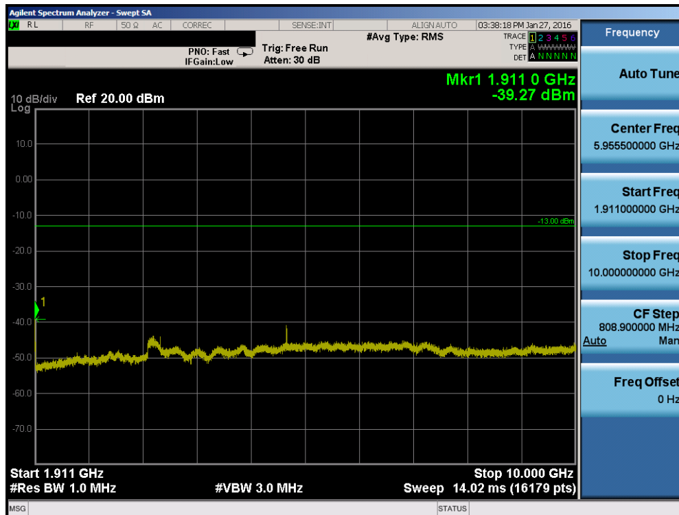
Plot 7-58. Conducted Spurious Plot (Band 2 – 20.0MHz QPSK – RB Size 1, RB Offset 0 – High Channel)
