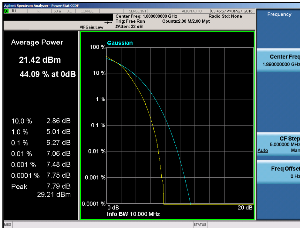
Plot 7-123. PAR Plot (Band 2 – 10.0MHz 16-QAM – RB Size 50)
