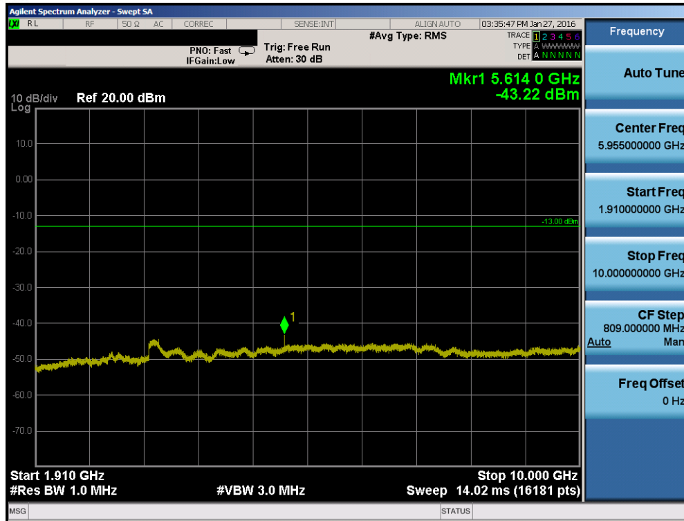
Plot 7-55. Conducted Spurious Plot (Band 2 – 20.0MHz QPSK – RB Size 1, RB Offset 0 – Mid Channel)
