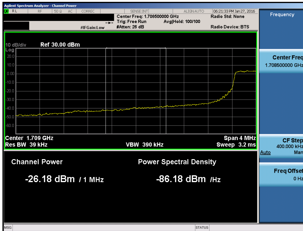
Plot 7-73. Lower Extended Band Edge Plot (Band 4 – 3.0MHz QPSK – RB Size 15)
