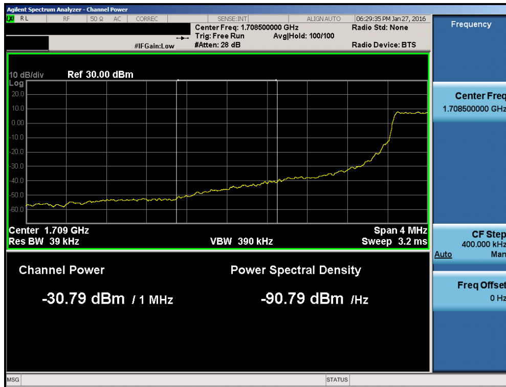
Plot 7-69. Lower Extended Band Edge Plot (Band 4 – 1.4MHz QPSK – RB Size 6)
