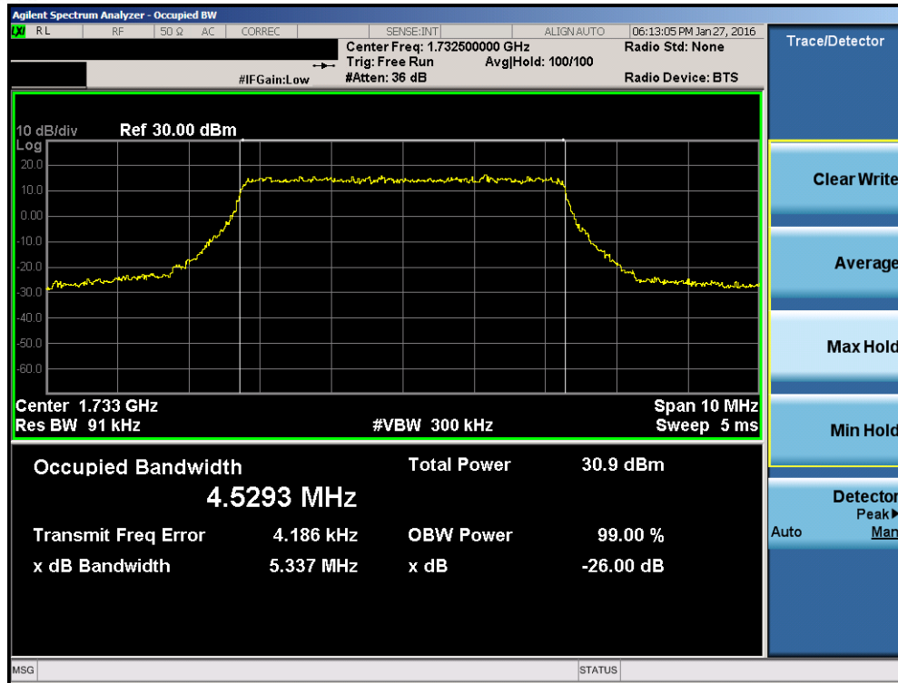
Plot 7-13. Occupied Bandwidth Plot (Band 4 – 5.0MHz QPSK – RB Size 25)
