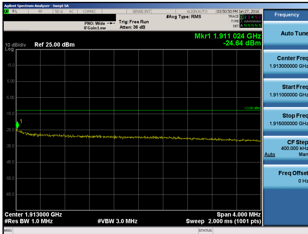
Plot 7-107. Upper Extended Band Edge Plot (Band 2 – 10.0MHz QPSK – RB Size 50)
