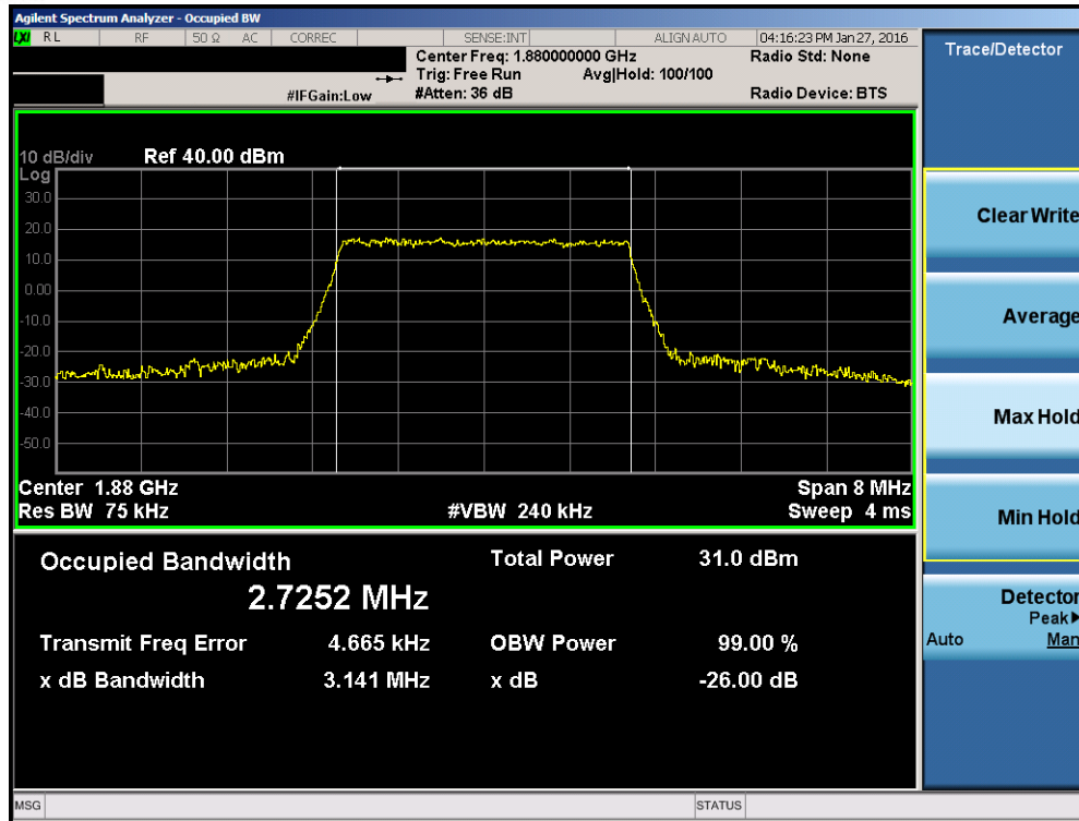
Plot 7-23. Occupied Bandwidth Plot (Band 2 – 3.0MHz QPSK – RB Size 15)
