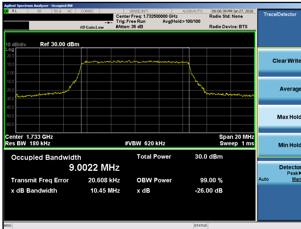
Plot 7-16. Occupied Bandwidth Plot (Band 4 – 10.0MHz 16-QAM – RB Size 50)
