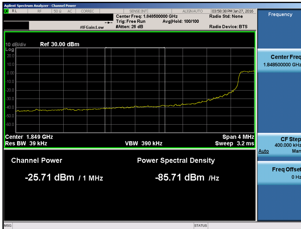
Plot 7-101. Lower Extended Band Edge Plot (Band 2 – 5.0MHz QPSK – RB Size 25)
