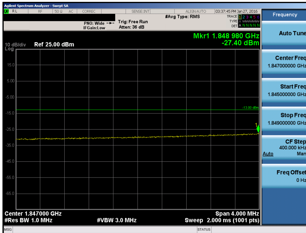
Plot 7-113. Lower Extended Band Edge Plot (Band 2 – 20.0MHz QPSK – RB Size 100)
