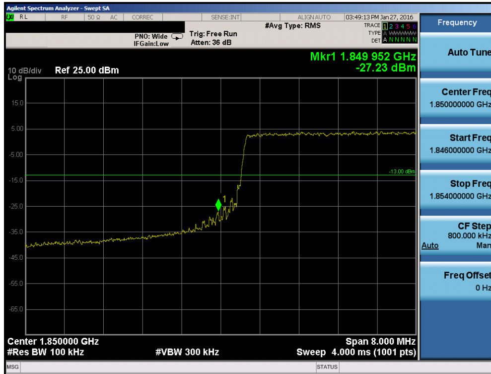
Plot 7-104. Lower Band Edge Plot (Band 2 – 10.0MHz QPSK – RB Size 50)
