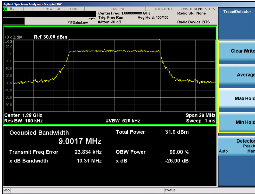
Plot 7-27. Occupied Bandwidth Plot (Band 2 – 10.0MHz QPSK – RB Size 50)
