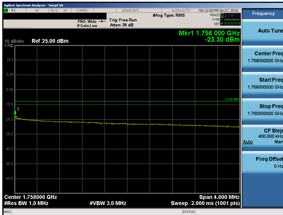
Plot 7-83. Upper Extended Band Edge Plot (Band 4 – 10.0MHz QPSK – RB Size 50)
