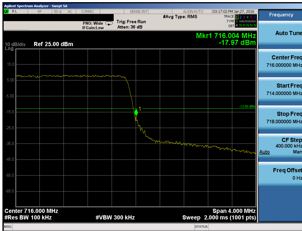
Plot 7-63. Upper Band Edge Plot (Band 12 – 3.0MHz QPSK – RB Size 15)
