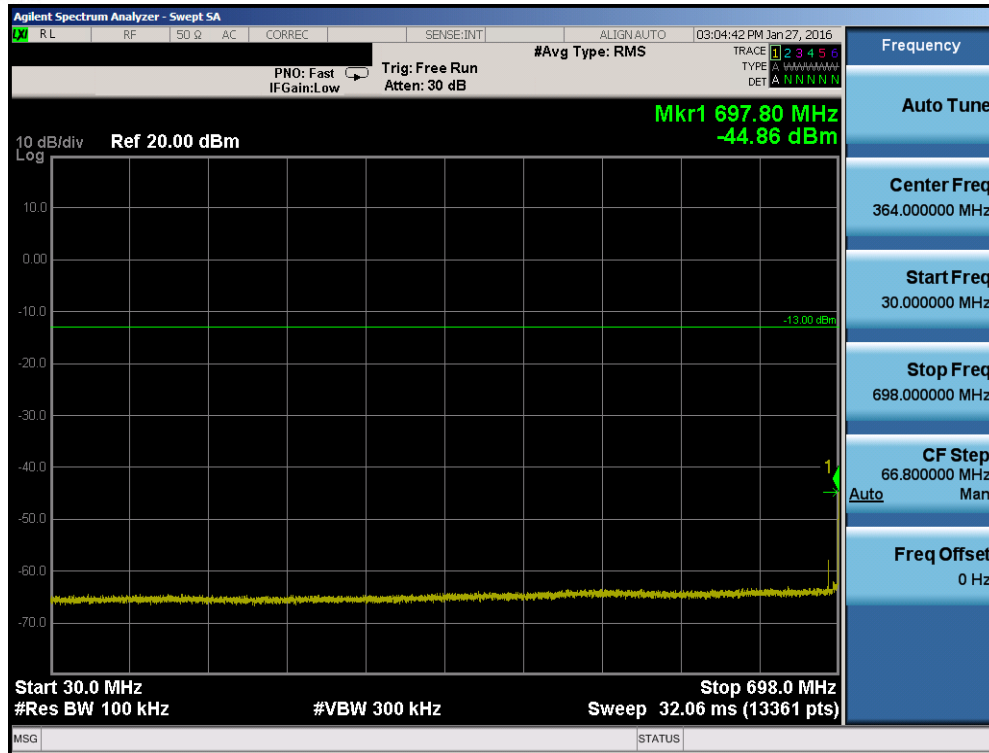
Plot 7-39. Conducted Spurious Plot (Band 12 – 10.0MHz QPSK – RB Size 1, RB Offset 0 – High Channel)
