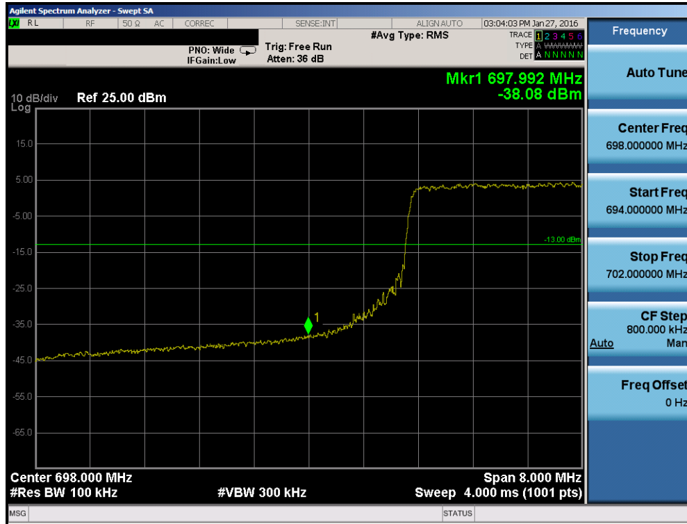
Plot 7-66. Lower Band Edge Plot (Band 12 – 10.0MHz QPSK – RB Size 50)
