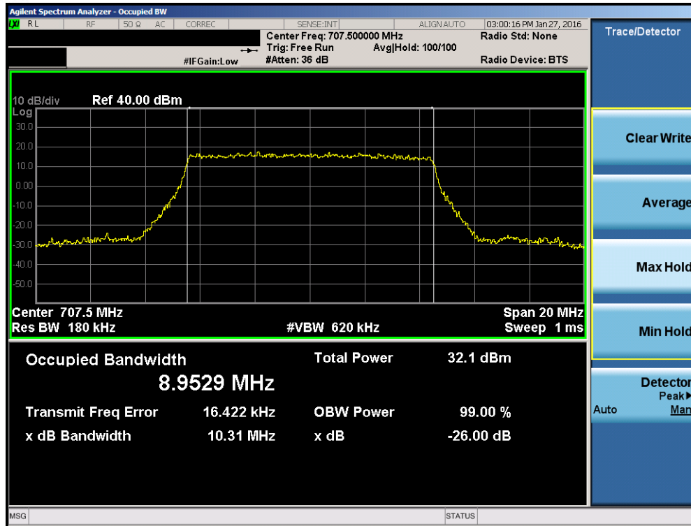
Plot 7-7. Occupied Bandwidth Plot (Band 12 – 10.0MHz QPSK – RB Size 50)
