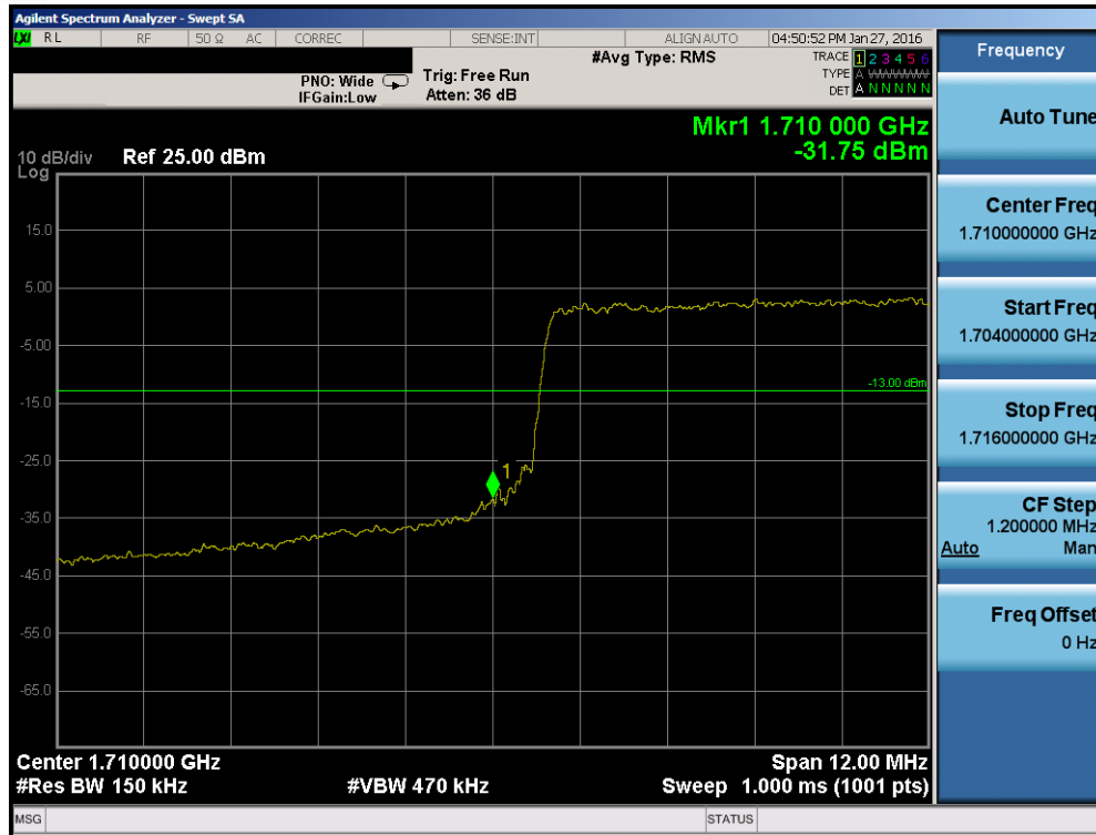
Plot 7-84. Lower Band Edge Plot (Band 4 – 15.0MHz QPSK – RB Size 75)
