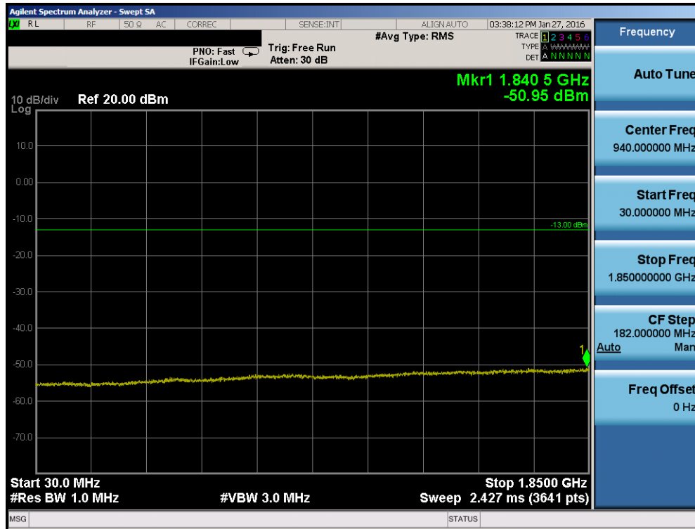
Plot 7-57. Conducted Spurious Plot (Band 2 – 20.0MHz QPSK – RB Size 1, RB Offset 0 – High Channel)
