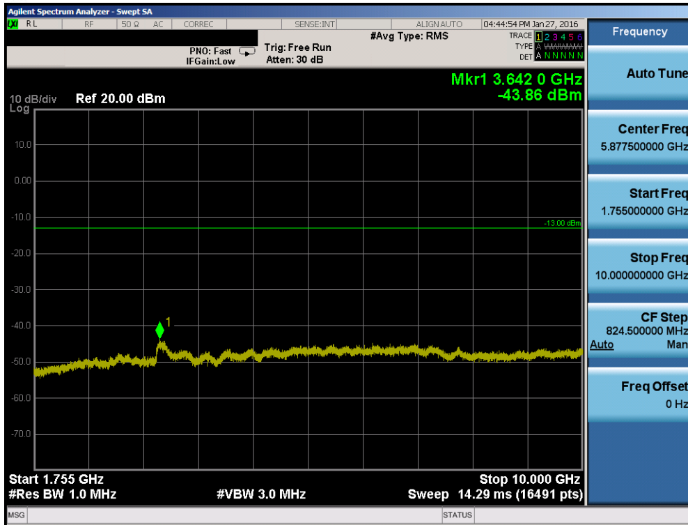
Plot 7-43. Conducted Spurious Plot (Band 4 – 20.0MHz QPSK – RB Size 1, RB Offset 0 – Low Channel)
