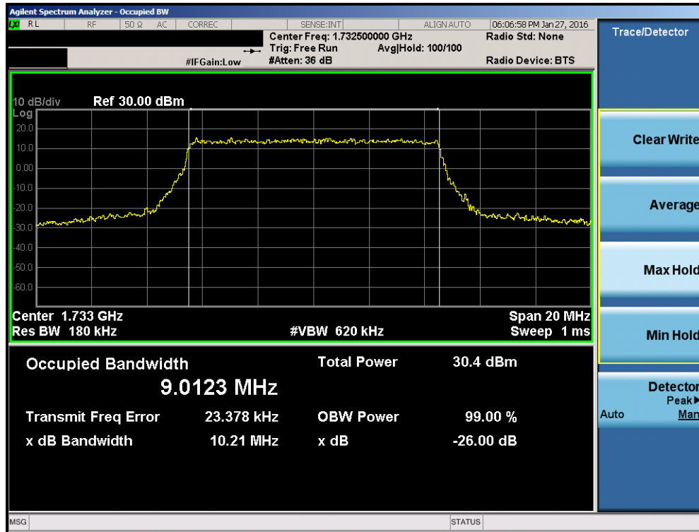
Plot 7-15. Occupied Bandwidth Plot (Band 4 – 10.0MHz QPSK – RB Size 50)
