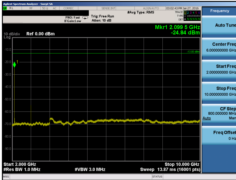
Plot 7-35. Conducted Spurious Plot (Band 12 – 10.0MHz QPSK – RB Size 1, RB Offset 0 – Low Channel)
