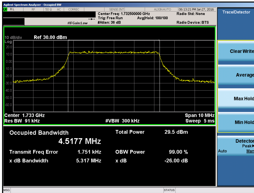
Plot 7-14. Occupied Bandwidth Plot (Band 4 – 5.0MHz 16-QAM – RB Size 25)
