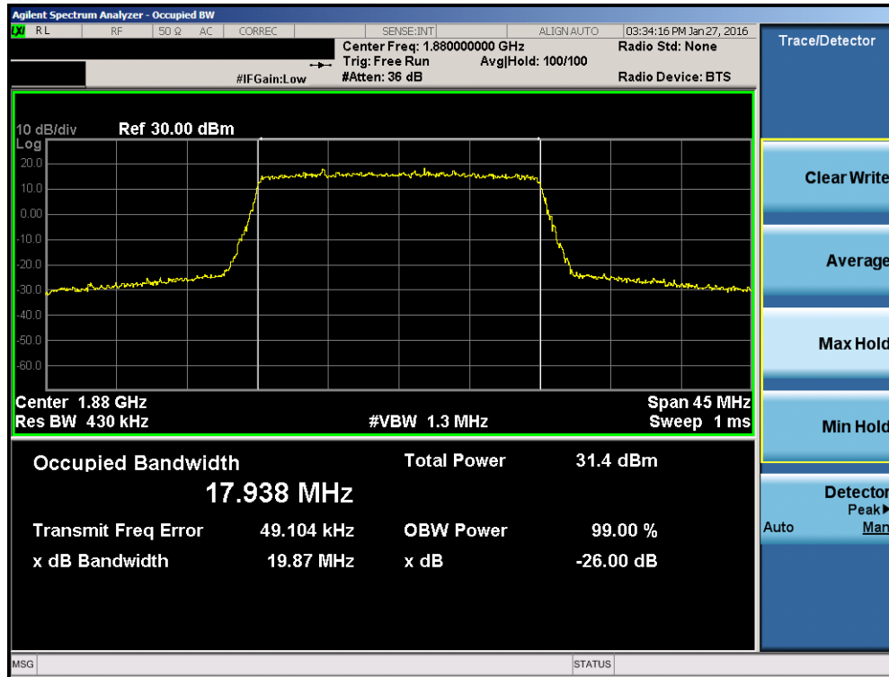
Plot 7-31. Occupied Bandwidth Plot (Band 2 – 20.0MHz QPSK – RB Size 100)
