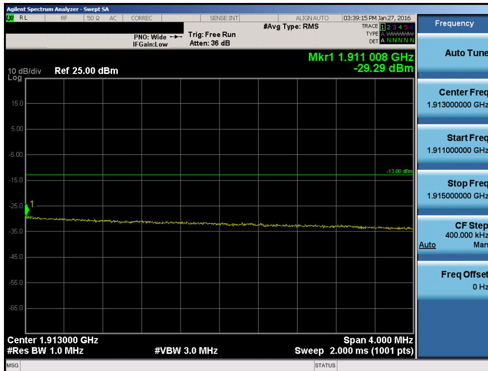
Plot 7-115. Upper Extended Band Edge Plot (Band 2 – 20.0MHz QPSK – RB Size 100)
