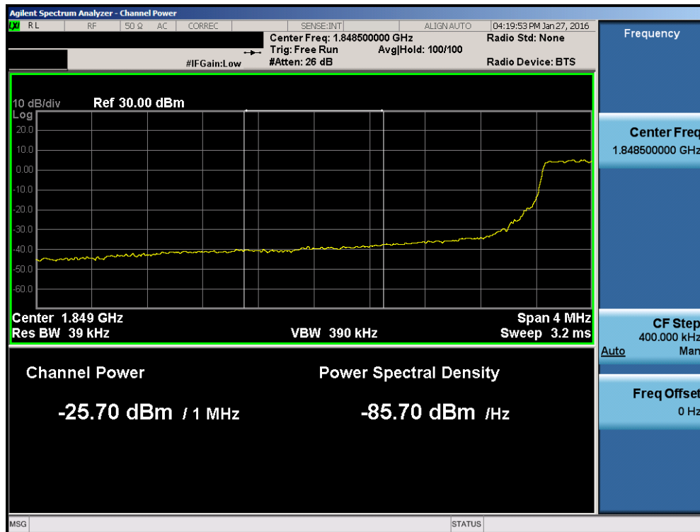
Plot 7-97. Lower Extended Band Edge Plot (Band 2 – 3.0MHz QPSK – RB Size 15)
