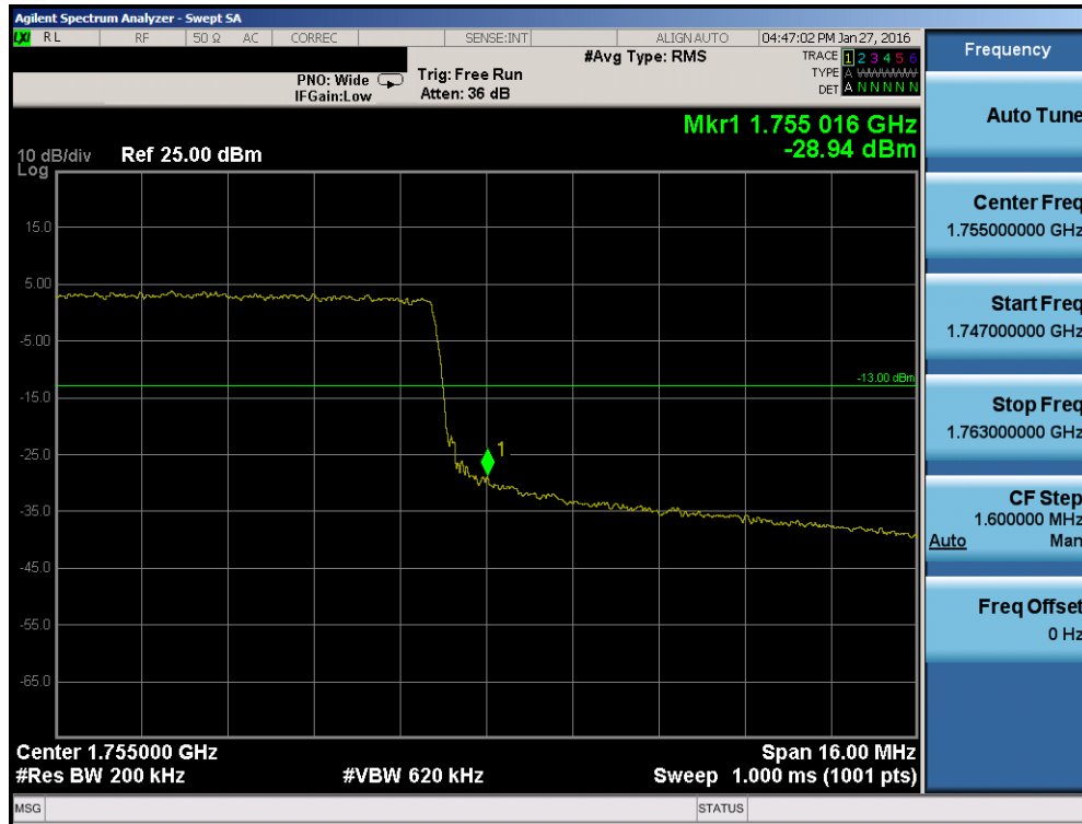
Plot 7-90. Upper Band Edge Plot (Band 4 – 20.0MHz QPSK – RB Size 100)
