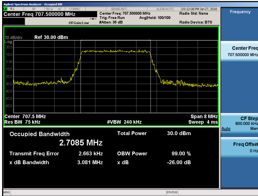
Plot 7-3. Occupied Bandwidth Plot (Band 12 – 3.0MHz QPSK – RB Size 15)
