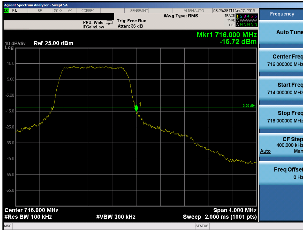
Plot 7-61. Upper Band Edge Plot (Band 12 – 1.4MHz QPSK – RB Size 6)
