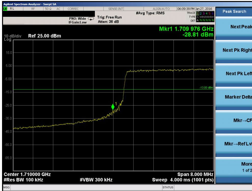
Plot 7-80. Lower Band Edge Plot (Band 4 – 10.0MHz QPSK – RB Size 50)
