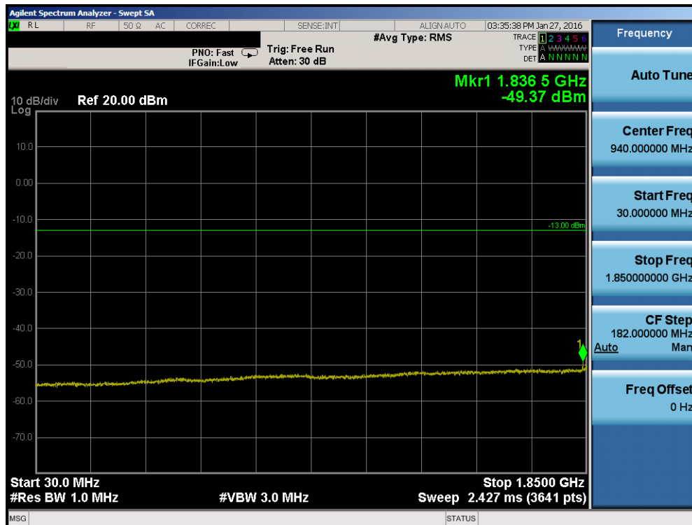
Plot 7-54. Conducted Spurious Plot (Band 2 – 20.0MHz QPSK – RB Size 1, RB Offset 0 – Mid Channel)
