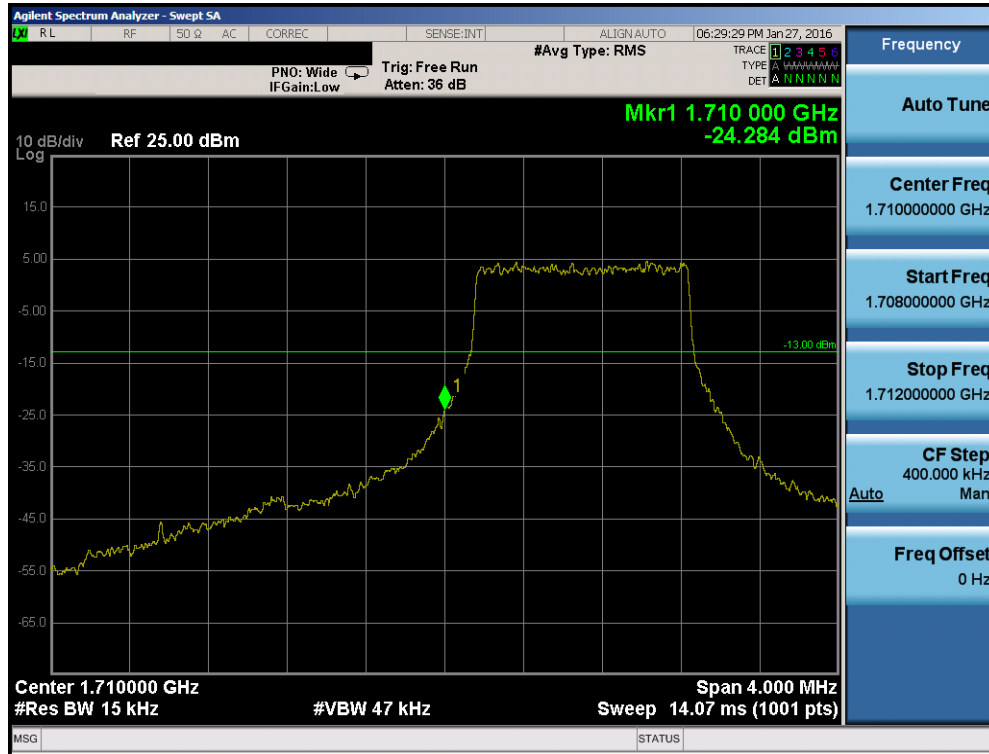
Plot 7-68. Lower Band Edge Plot (Band 4 – 1.4MHz QPSK – RB Size 6)
