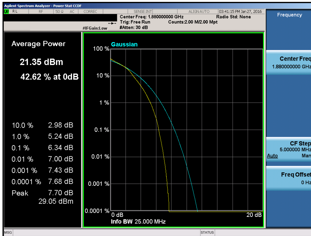
Plot 7-125. PAR Plot (Band 2 – 15.0MHz 16-QAM – RB Size 75)
