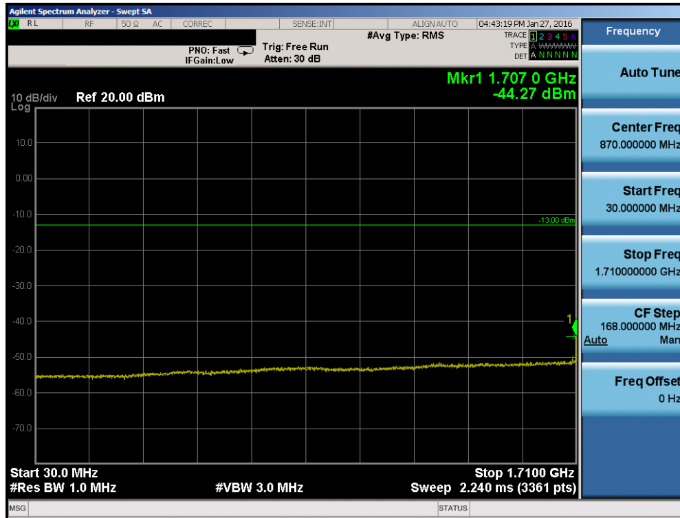
Plot 7-45. Conducted Spurious Plot (Band 4 – 20.0MHz QPSK – RB Size 1, RB Offset 0 – Mid Channel)
