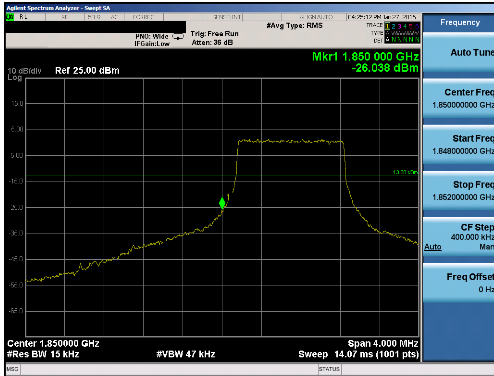
Plot 7-92. Lower Band Edge Plot (Band 2 – 1.4MHz QPSK – RB Size 6)
