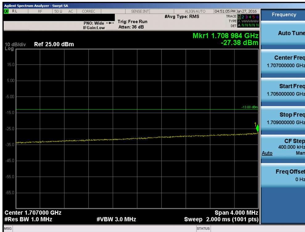
Plot 7-85. Lower Extended Band Edge Plot (Band 4 – 15.0MHz QPSK – RB Size 75)
