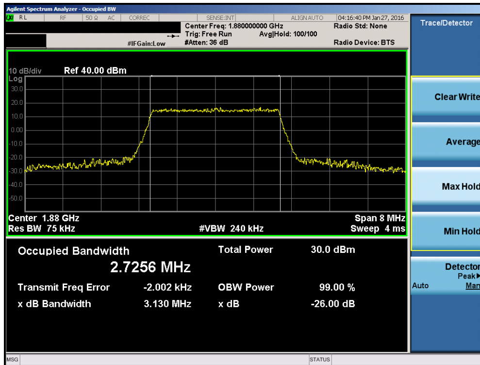
Plot 7-24. Occupied Bandwidth Plot (Band 2 – 3.0MHz 16-QAM – RB Size 15)
