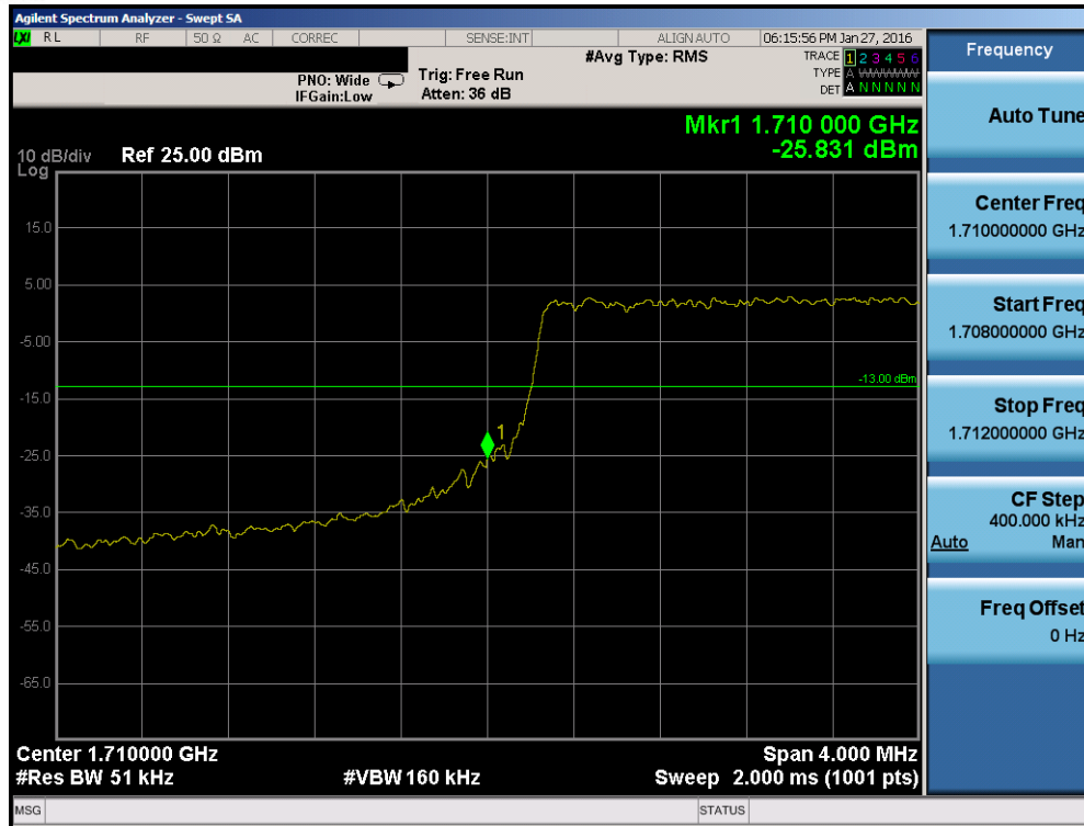
Plot 7-76. Lower Band Edge Plot (Band 4 – 5.0MHz QPSK – RB Size 25)
