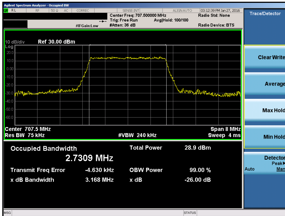
Plot 7-4. Occupied Bandwidth Plot (Band 12 – 3.0MHz 16-QAM – RB Size 15)
