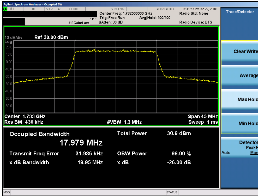
Plot 7-19. Occupied Bandwidth Plot (Band 4 – 20.0MHz QPSK – RB Size 100)
