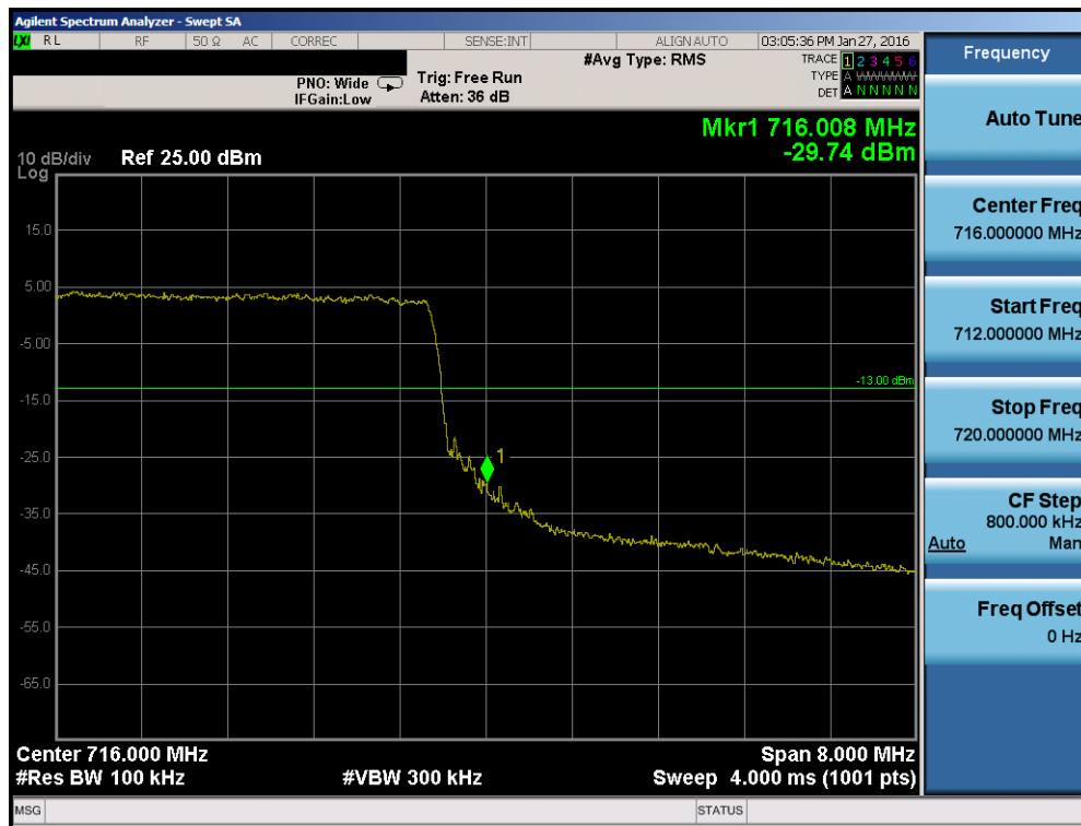
Plot 7-67. Upper Band Edge Plot (Band 12 – 10.0MHz QPSK – RB Size 50)
