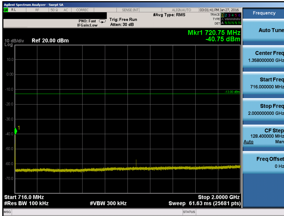
Plot 7-37. Conducted Spurious Plot (Band 12 – 10.0MHz QPSK – RB Size 1, RB Offset 0 – Mid Channel)
