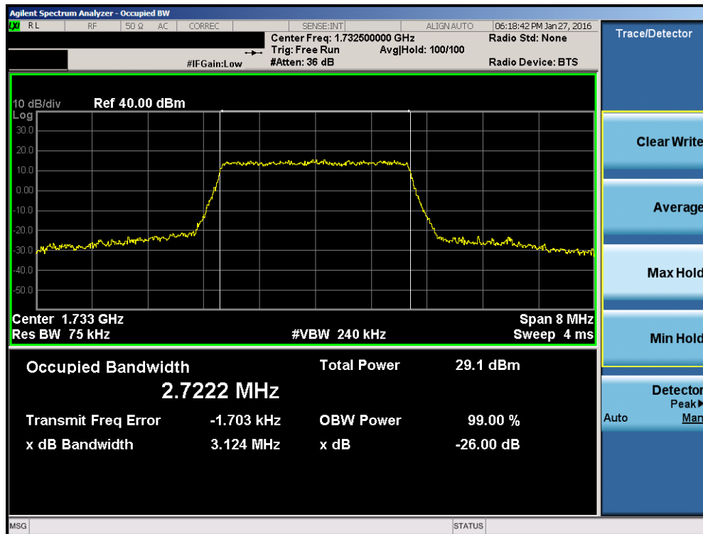
Plot 7-12. Occupied Bandwidth Plot (Band 4 – 3.0MHz 16-QAM – RB Size 15)
