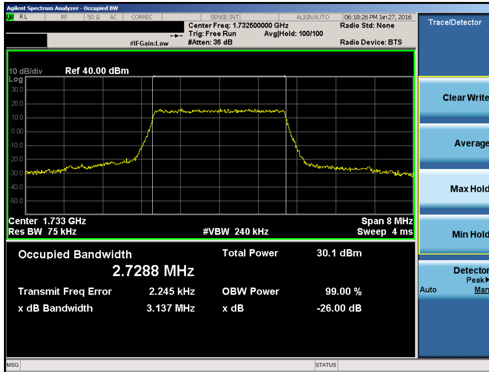
Plot 7-11. Occupied Bandwidth Plot (Band 4 – 3.0MHz QPSK – RB Size 15)
