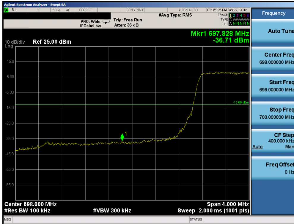
Plot 7-62. Lower Band Edge Plot (Band 12 – 3.0MHz QPSK – RB Size 15)
