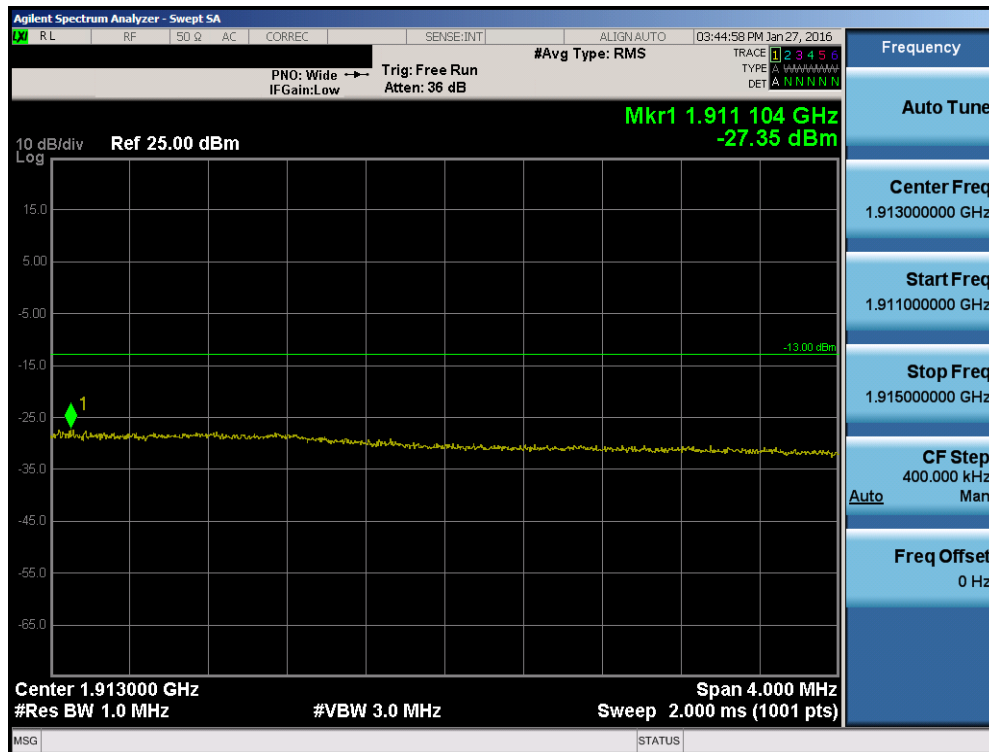
Plot 7-111. Upper Extended Band Edge Plot (Band 2 – 15.0MHz QPSK – RB Size 75)
