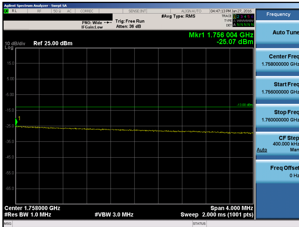
Plot 7-91. Upper Extended Band Edge Plot (Band 4 – 20.0MHz QPSK – RB Size 100)
