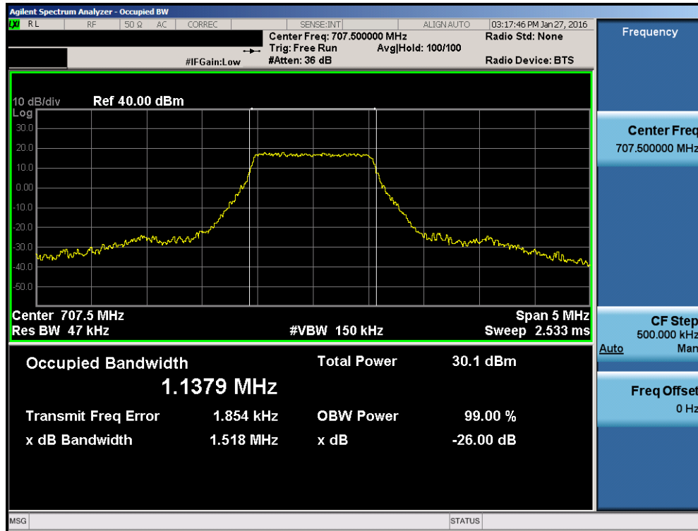
Plot 7-1. Occupied Bandwidth Plot (Band 12 – 1.4MHz QPSK – RB Size 6)
