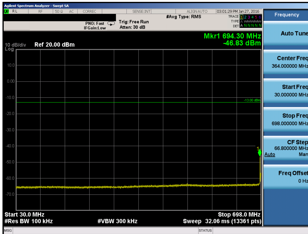
Plot 7-36. Conducted Spurious Plot (Band 12 – 10.0MHz QPSK – RB Size 1, RB Offset 0 – Mid Channel)
