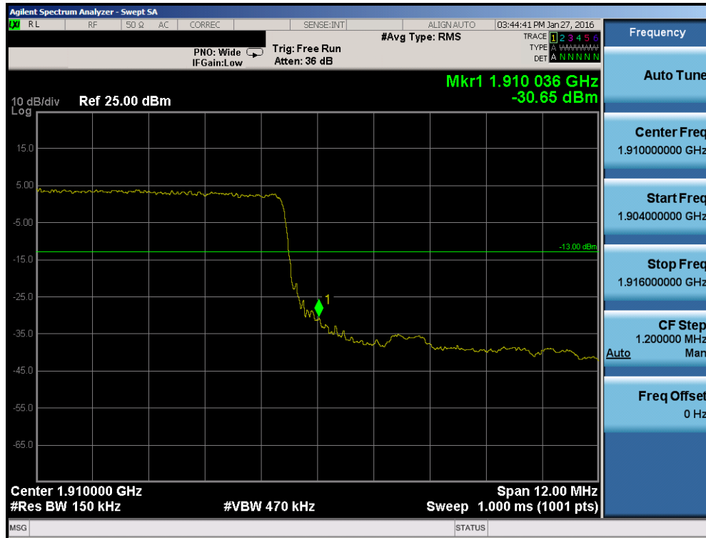
Plot 7-110. Upper Band Edge Plot (Band 2 – 15.0MHz QPSK – RB Size 75)
