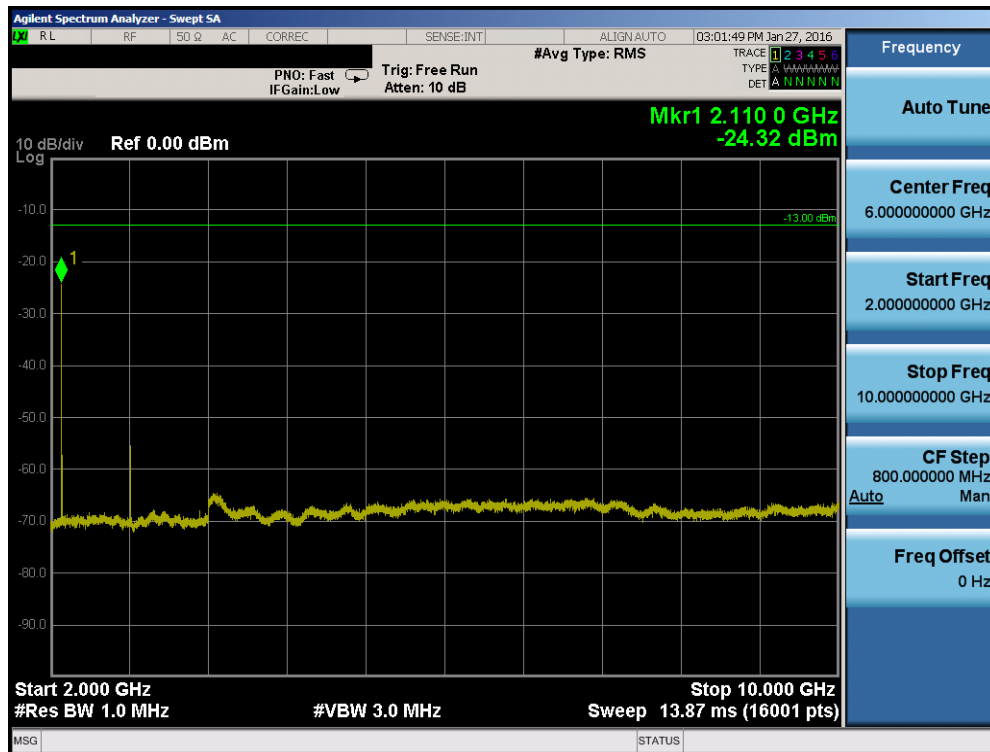
Plot 7-38. Conducted Spurious Plot (Band 12 – 10.0MHz QPSK – RB Size 1, RB Offset 0 – Mid Channel)
