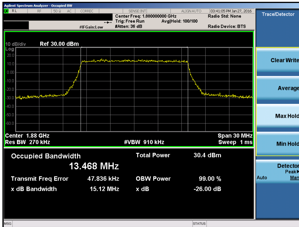
Plot 7-30. Occupied Bandwidth Plot (Band 2 – 15.0MHz 16-QAM – RB Size 75)
