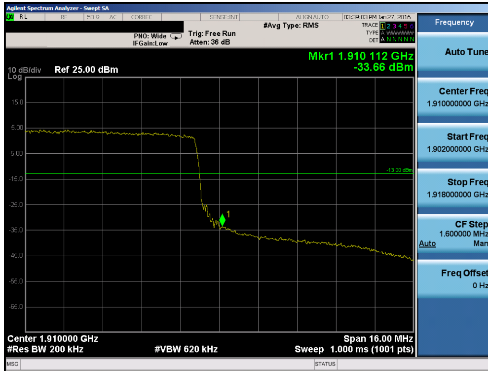
Plot 7-114. Upper Band Edge Plot (Band 2 – 20.0MHz QPSK – RB Size 100)
