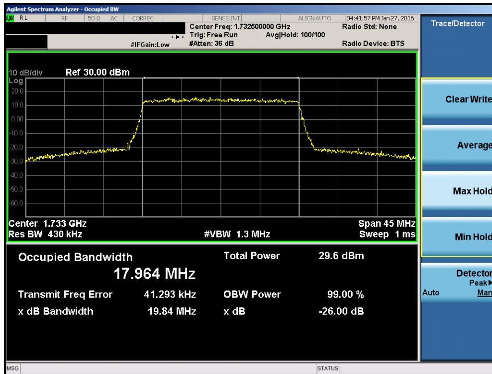
Plot 7-20. Occupied Bandwidth Plot (Band 4 – 20.0MHz 16-QAM – RB Size 100)
