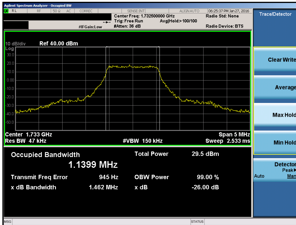
Plot 7-10. Occupied Bandwidth Plot (Band 4 – 1.4MHz 16-QAM – RB Size 6)
