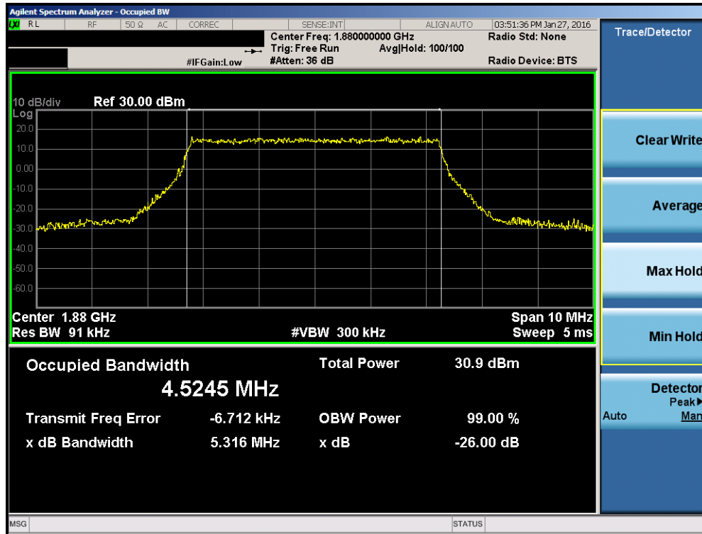
Plot 7-25. Occupied Bandwidth Plot (Band 2 – 5.0MHz QPSK – RB Size 25)
