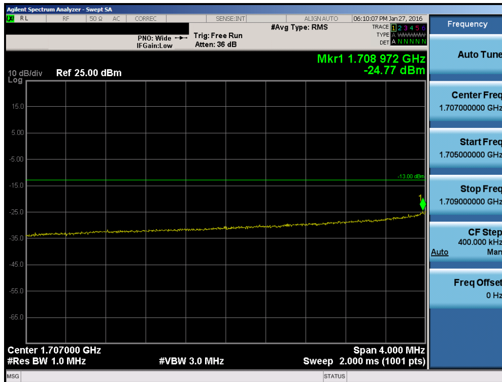
Plot 7-81. Lower Extended Band Edge Plot (Band 4 – 10.0MHz QPSK – RB Size 50)
