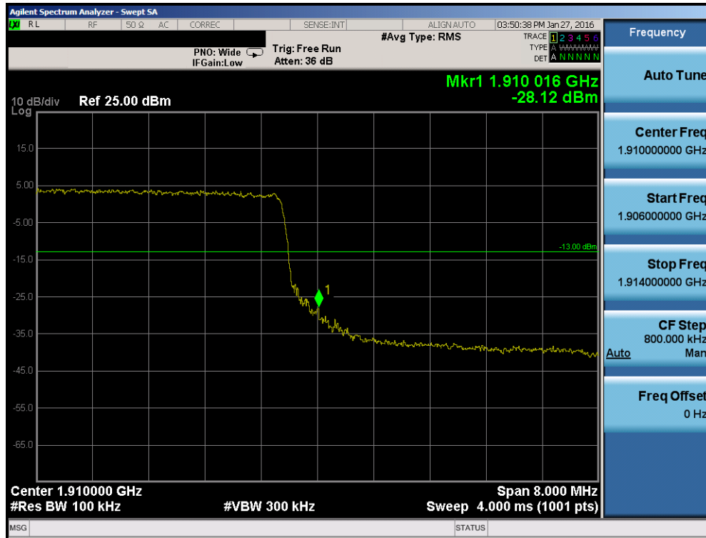
Plot 7-106. Upper Band Edge Plot (Band 2 – 10.0MHz QPSK – RB Size 50)
