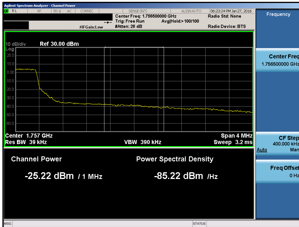
Plot 7-75. Upper Extended Band Edge Plot (Band 4 – 3.0MHz QPSK – RB Size 15)
