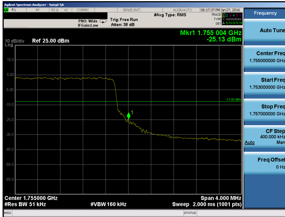
Plot 7-78. Upper Band Edge Plot (Band 4 – 5.0MHz QPSK – RB Size 25)
