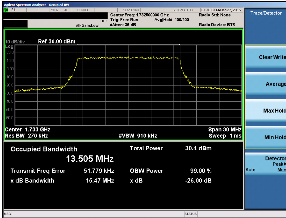
Plot 7-17. Occupied Bandwidth Plot (Band 4 – 15.0MHz QPSK – RB Size 75)
