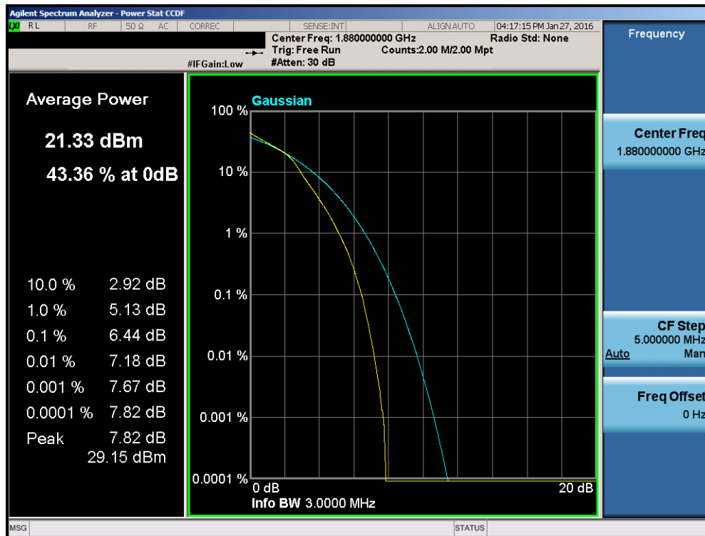
Plot 7-119. PAR Plot (Band 2 – 3.0MHz 16-QAM – RB Size 15)
