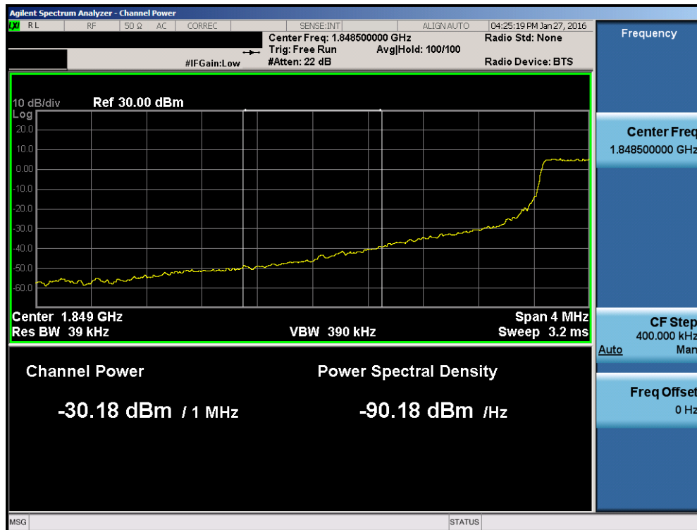
Plot 7-93. Lower Extended Band Edge Plot (Band 2 – 1.4MHz QPSK – RB Size 6)
