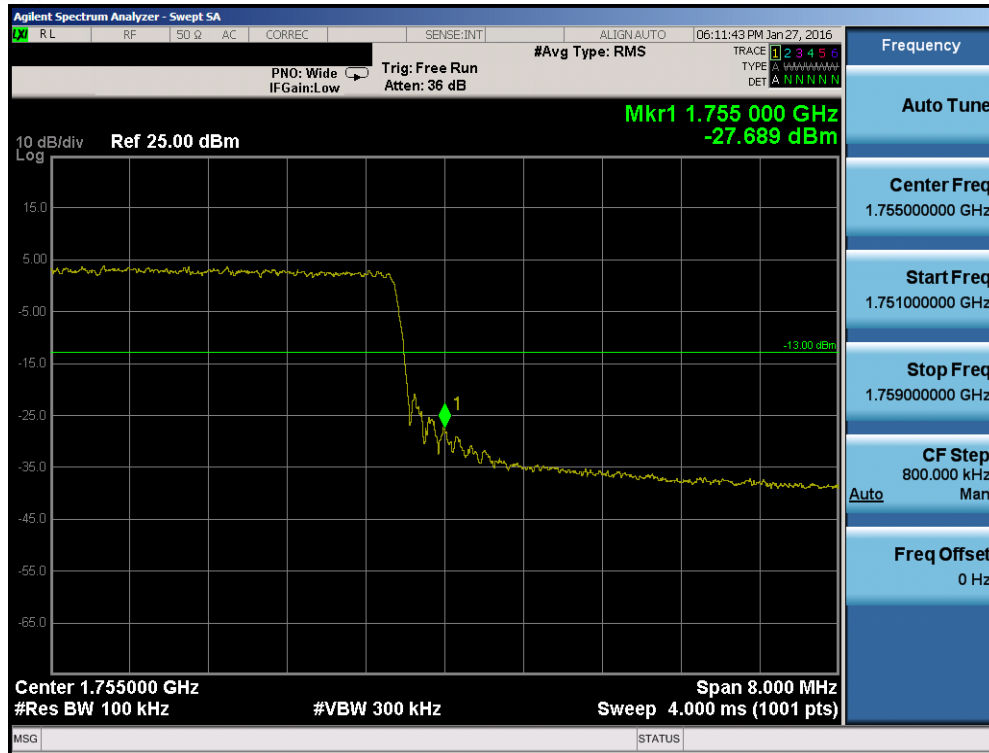
Plot 7-82. Upper Band Edge Plot (Band 4 – 10.0MHz QPSK – RB Size 50)
