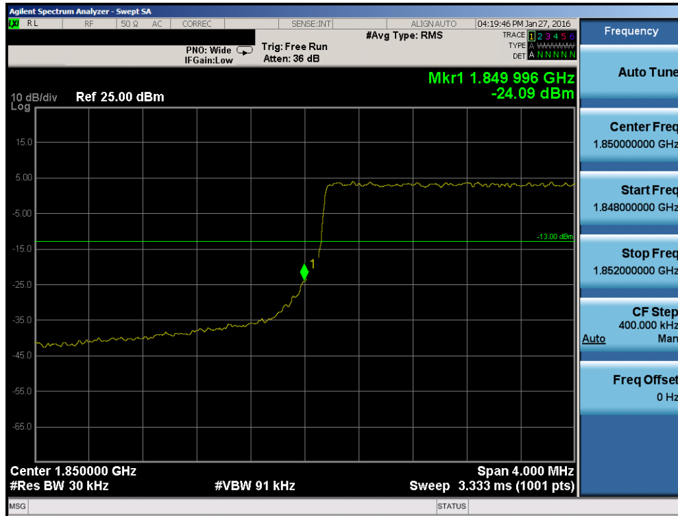
Plot 7-96. Lower Band Edge Plot (Band 2 – 3.0MHz QPSK – RB Size 15)
