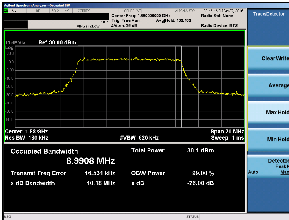
Plot 7-28. Occupied Bandwidth Plot (Band 2 – 10.0MHz 16-QAM – RB Size 50)
