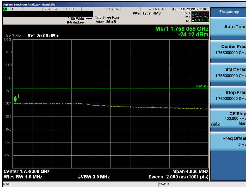
Plot 7-87. Upper Extended Band Edge Plot (Band 4 – 15.0MHz QPSK – RB Size 75)
