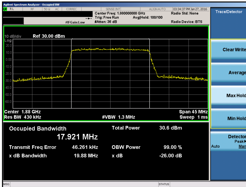
Plot 7-32. Occupied Bandwidth Plot (Band 2 – 20.0MHz 16-QAM – RB Size 100)
