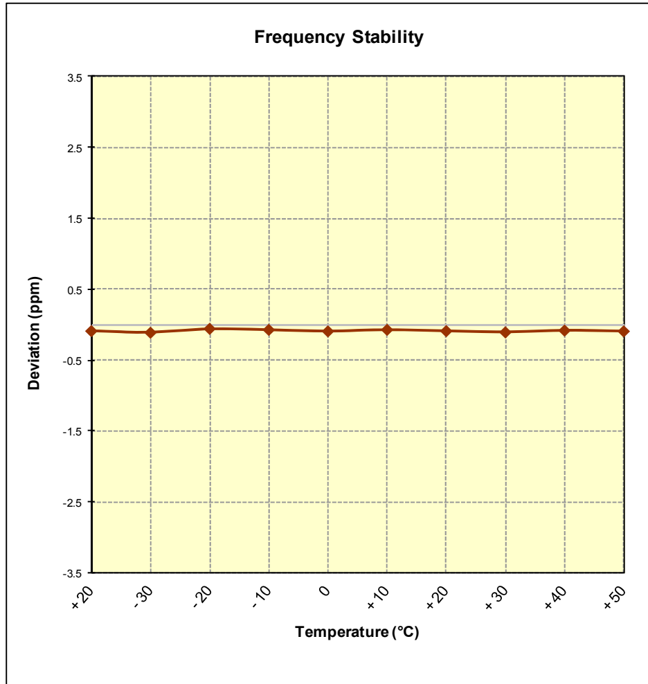
Figure 7-10. Frequency Stability Graph (Band 2)
