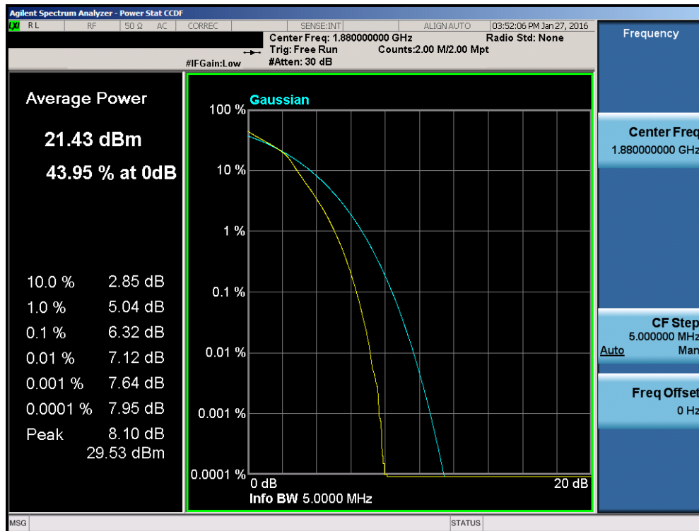
Plot 7-121. PAR Plot (Band 2 – 5.0MHz 16-QAM – RB Size 25)
