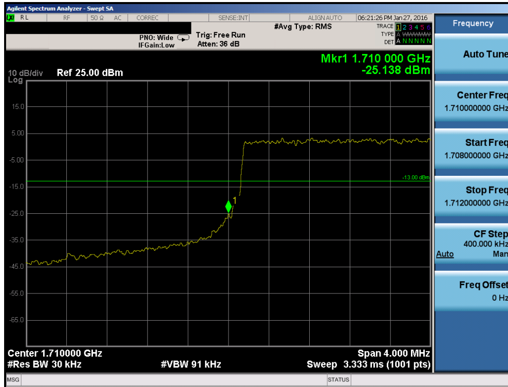
Plot 7-72. Lower Band Edge Plot (Band 4 – 3.0MHz QPSK – RB Size 15)
