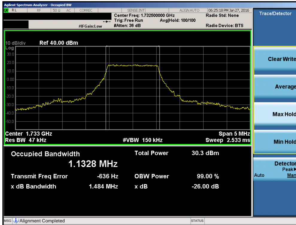
Plot 7-9. Occupied Bandwidth Plot (Band 4 – 1.4MHz QPSK – RB Size 6)
