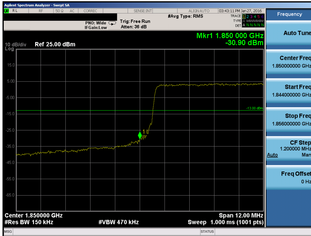
Plot 7-108. Lower Band Edge Plot (Band 2 – 15.0MHz QPSK – RB Size 75)
