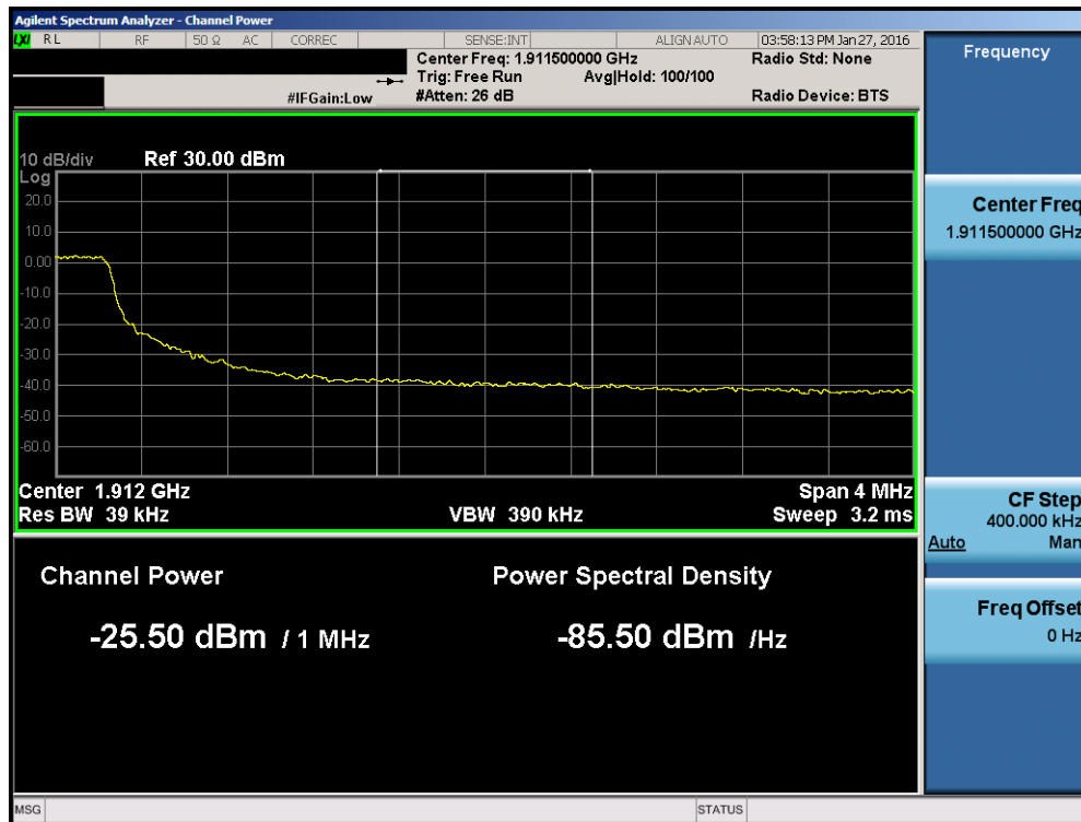
Plot 7-103. Upper Extended Band Edge Plot (Band 2 – 5.0MHz QPSK – RB Size 25)
