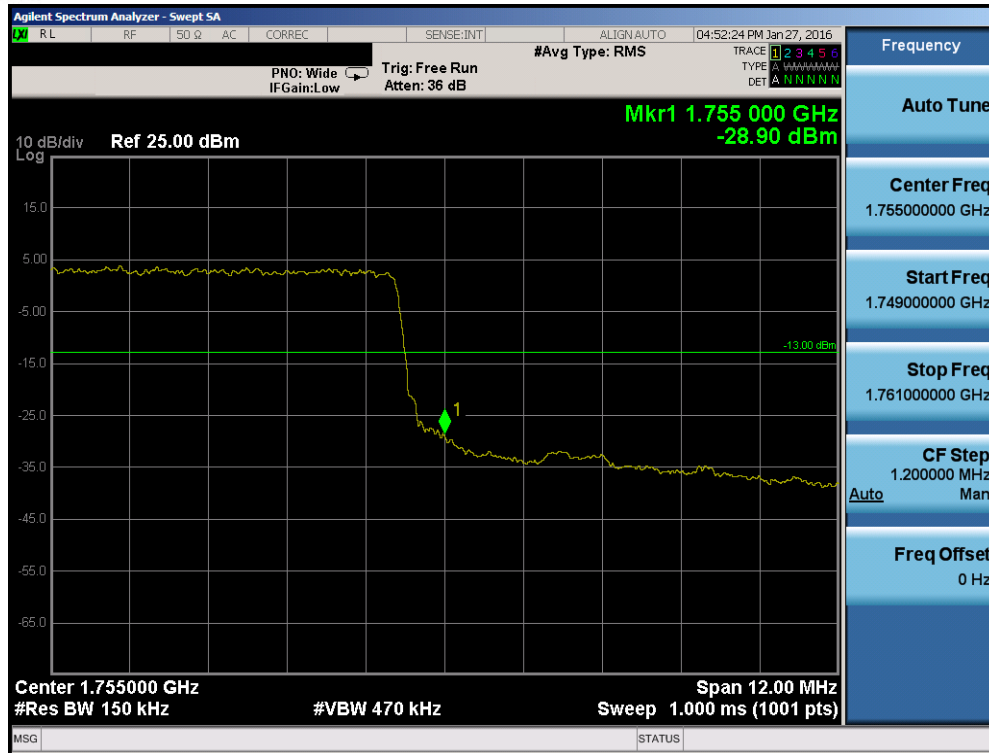
Plot 7-86. Upper Band Edge Plot (Band 4 – 15.0MHz QPSK – RB Size 75)
