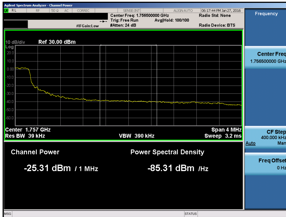
Plot 7-79. Upper Extended Band Edge Plot (Band 4 – 5.0MHz QPSK – RB Size 25)
