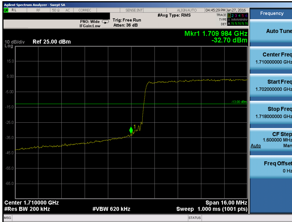
Plot 7-88. Lower Band Edge Plot (Band 4 – 20.0MHz QPSK – RB Size 100)
