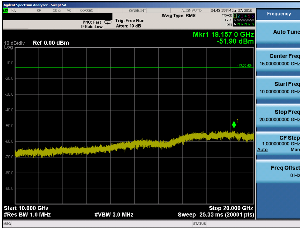
Plot 7-47. Conducted Spurious Plot (Band 4 – 20.0MHz QPSK – RB Size 1, RB Offset 0 – Mid Channel)
