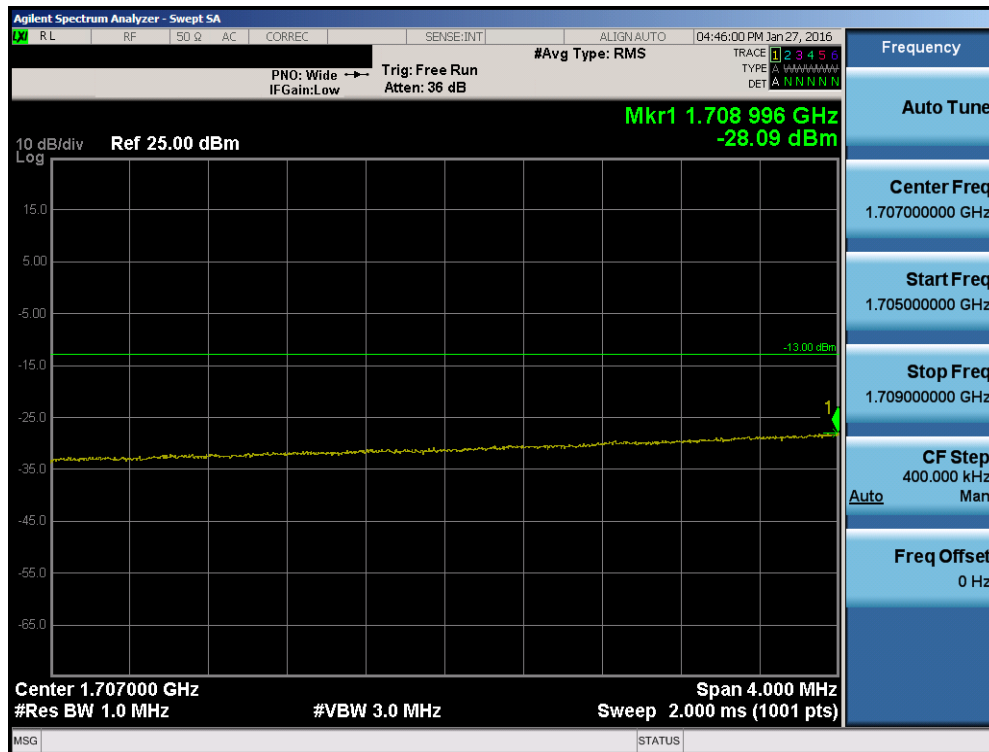
Plot 7-89. Lower Extended Band Edge Plot (Band 4 – 20.0MHz QPSK – RB Size 100)
