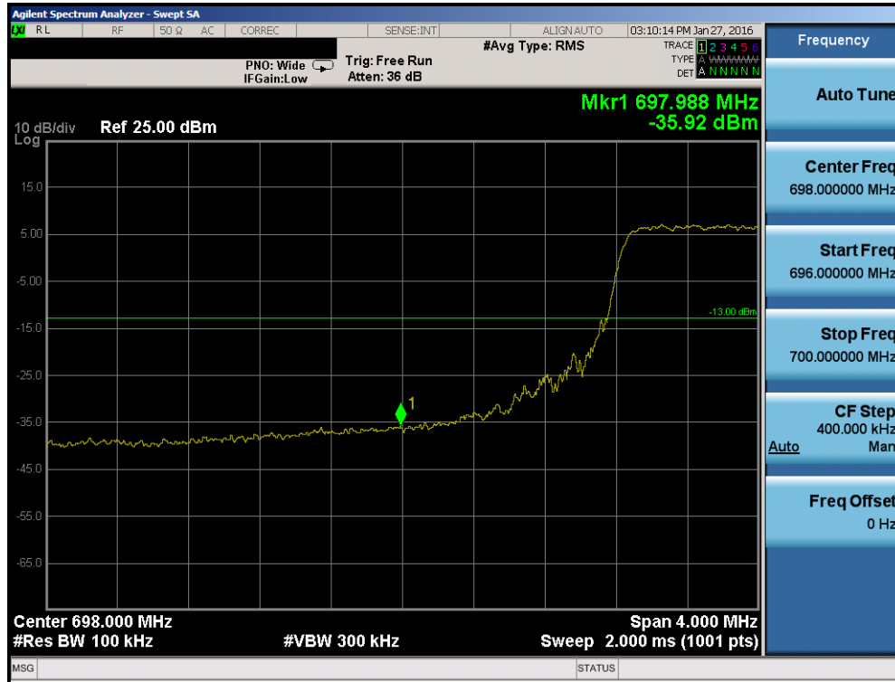
Plot 7-64. Lower Band Edge Plot (Band 12 – 5.0MHz QPSK – RB Size 25)
