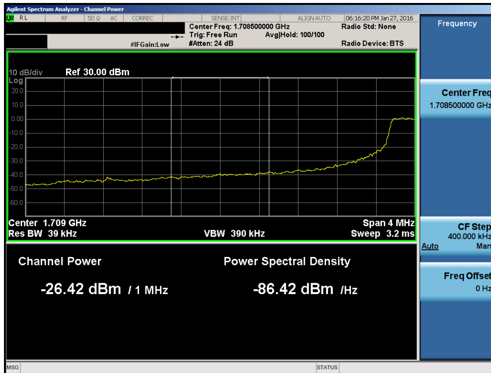
Plot 7-77. Lower Extended Band Edge Plot (Band 4 – 5.0MHz QPSK – RB Size 25)
