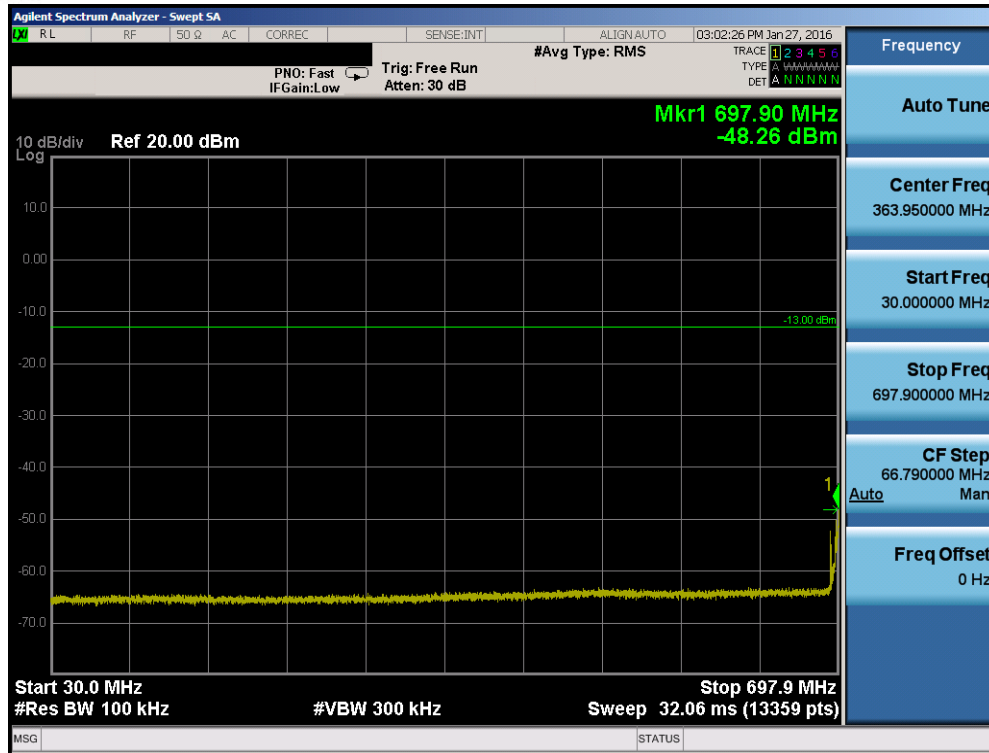
Plot 7-33. Conducted Spurious Plot (Band 12 – 10.0MHz QPSK – RB Size 1, RB Offset 0– Low Channel)
