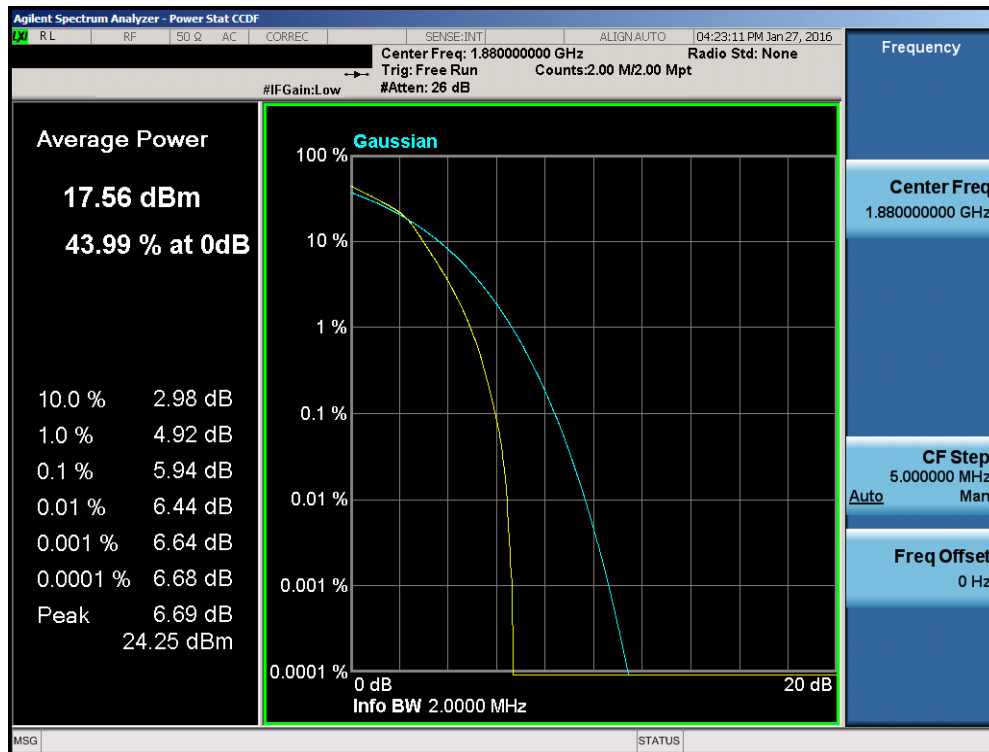
Plot 7-117. PAR Plot (Band 2 – 1.4MHz 16-QAM – RB Size 6)
