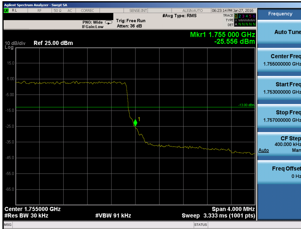
Plot 7-74. Upper Band Edge Plot (Band 4 – 3.0MHz QPSK – RB Size 15)
