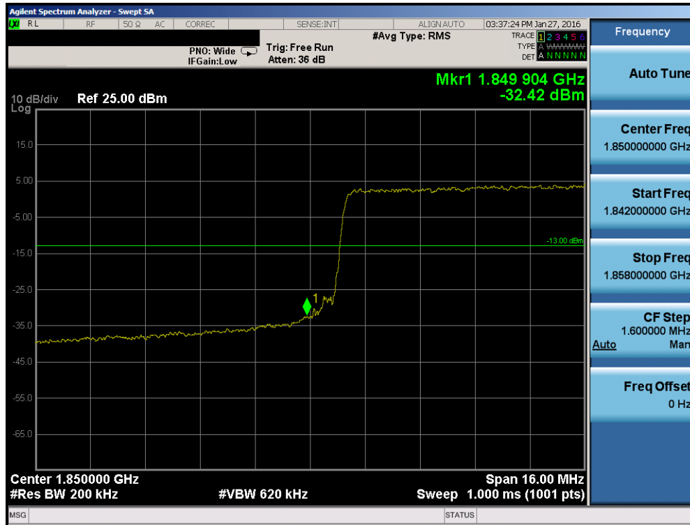
Plot 7-112. Lower Band Edge Plot (Band 2 – 20.0MHz QPSK – RB Size 100)
