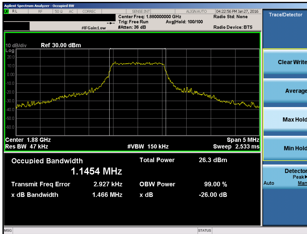
Plot 7-22. Occupied Bandwidth Plot (Band 2 – 1.4MHz 16-QAM – RB Size 6)
