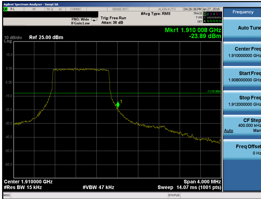
Plot 7-94. Upper Band Edge Plot (Band 2 – 1.4MHz QPSK – RB Size 6)
