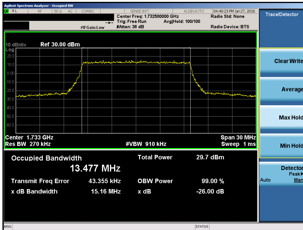
Plot 7-18. Occupied Bandwidth Plot (Band 4 – 15.0MHz 16-QAM – RB Size 75)
