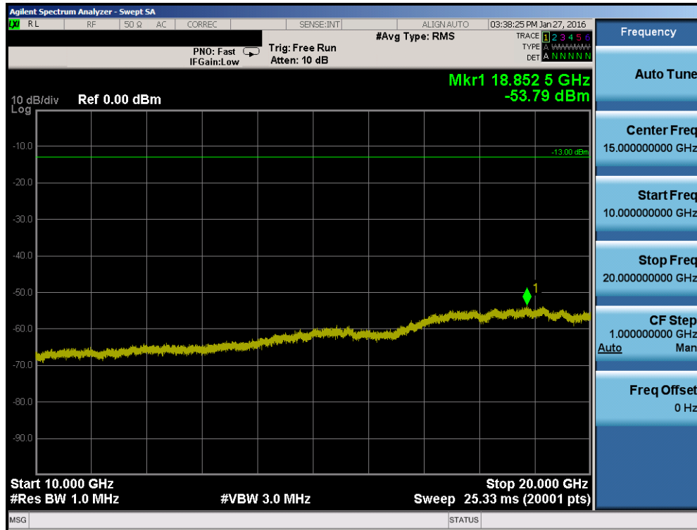
Plot 7-59. Conducted Spurious Plot (Band 2 – 20.0MHz QPSK – RB Size 1, RB Offset 0 – High Channel)
