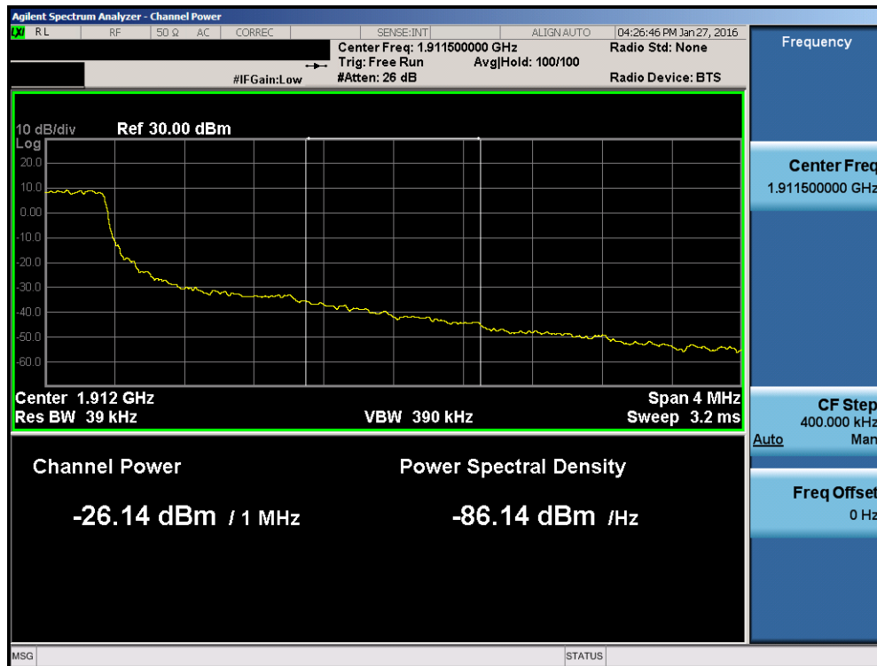
Plot 7-95. Upper Extended Band Edge Plot (Band 2 – 1.4MHz QPSK – RB Size 6)
