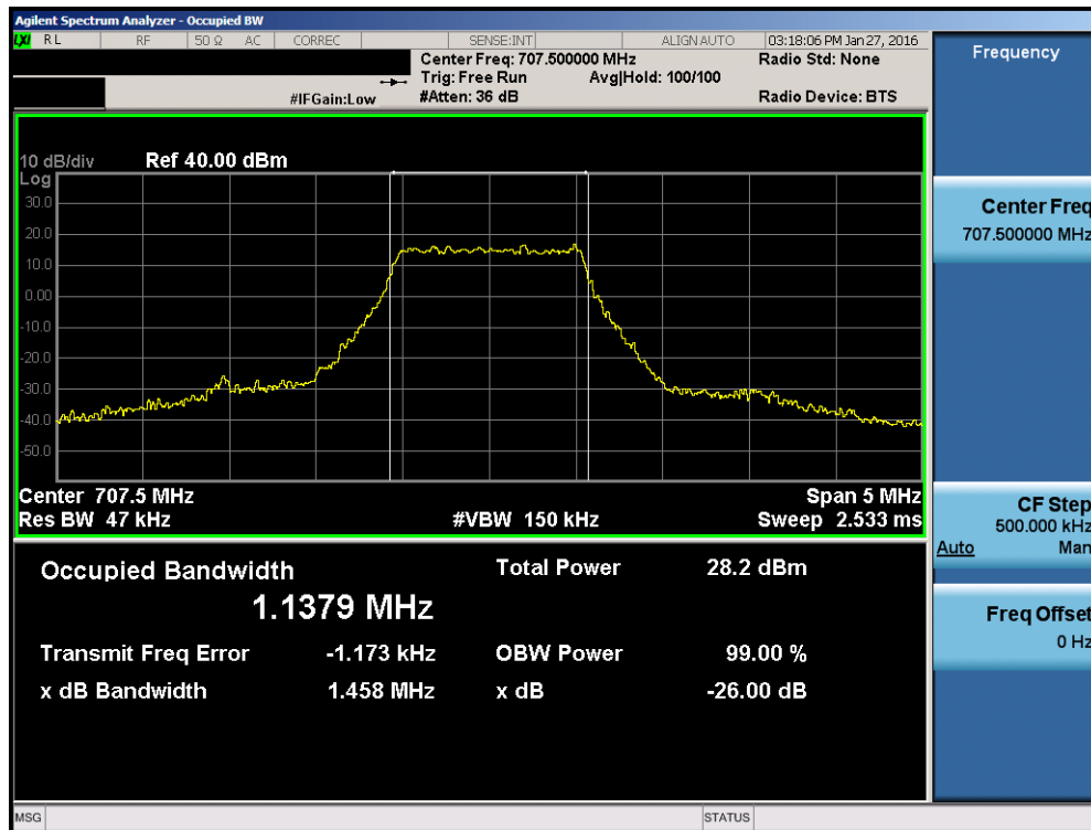
Plot 7-2. Occupied Bandwidth Plot (Band 12 – 1.4MHz 16-QAM – RB Size 6)
