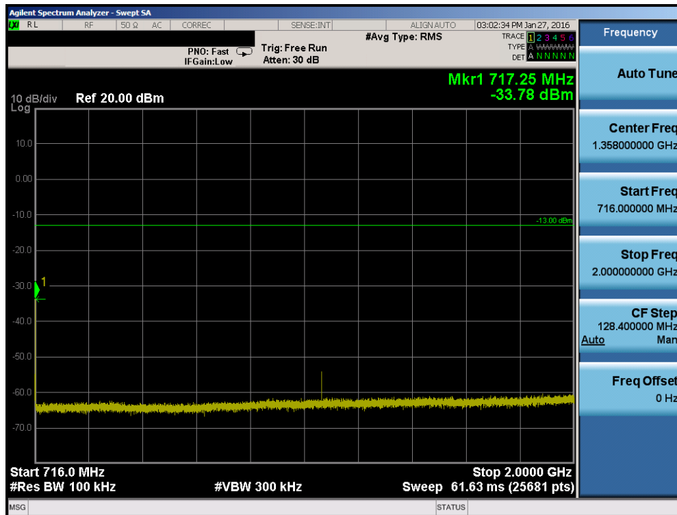
Plot 7-34. Conducted Spurious Plot (Band 12 – 10.0MHz QPSK – RB Size 1, RB Offset 0 – Low Channel)
