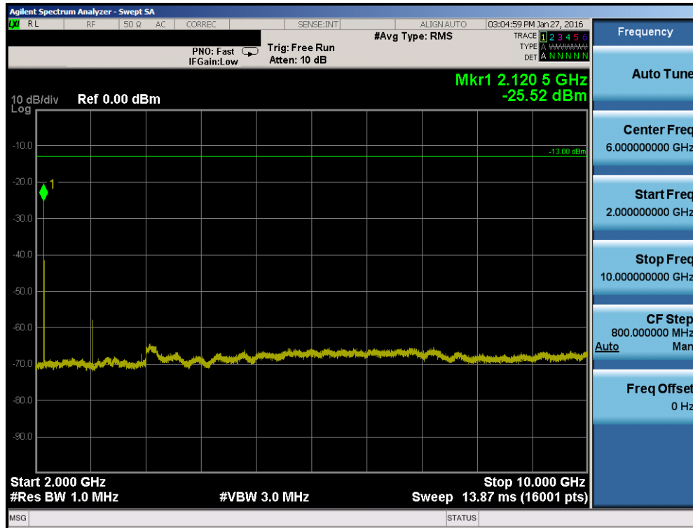
Plot 7-41. Conducted Spurious Plot (Band 12 – 10.0MHz QPSK – RB Size 1, RB Offset 0 – High Channel)
