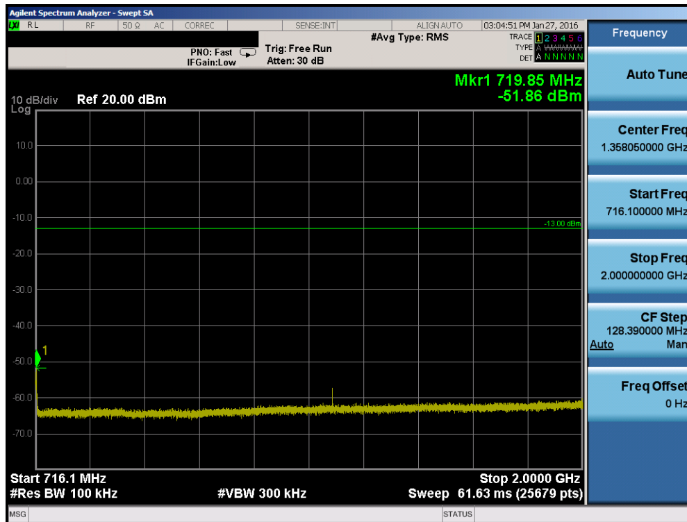
Plot 7-40. Conducted Spurious Plot (Band 12 – 10.0MHz QPSK – RB Size 1, RB Offset 0 – High Channel)
