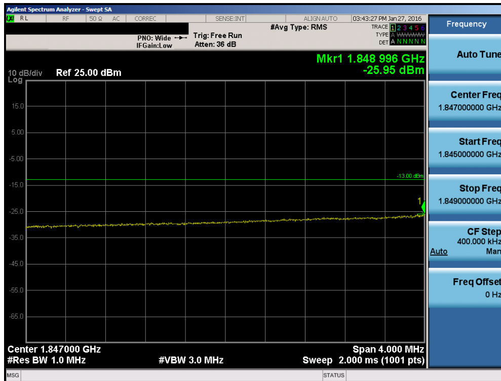
Plot 7-109. Lower Extended Band Edge Plot (Band 2 – 15.0MHz QPSK – RB Size 75)
