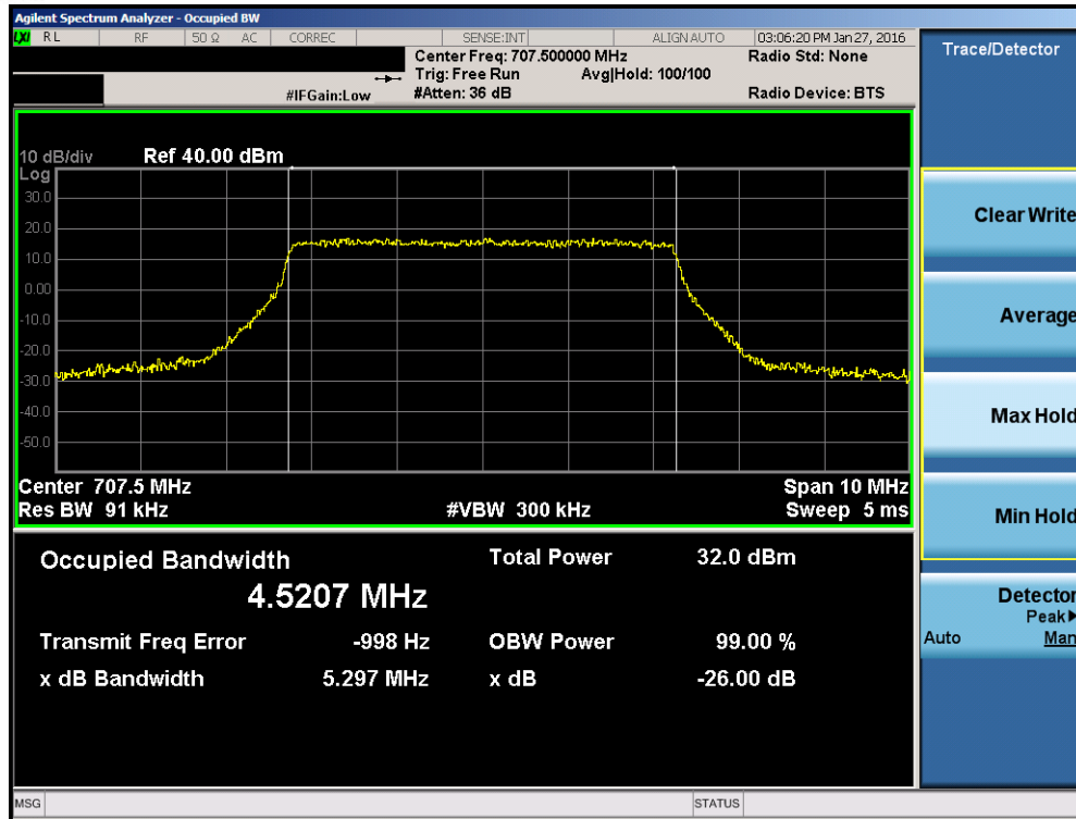
Plot 7-5. Occupied Bandwidth Plot (Band 12 – 5.0MHz QPSK – RB Size 25)
