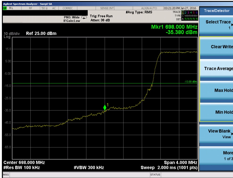
Plot 7-60. Lower Band Edge Plot (Band 12 – 1.4MHz QPSK – RB Size 6)
