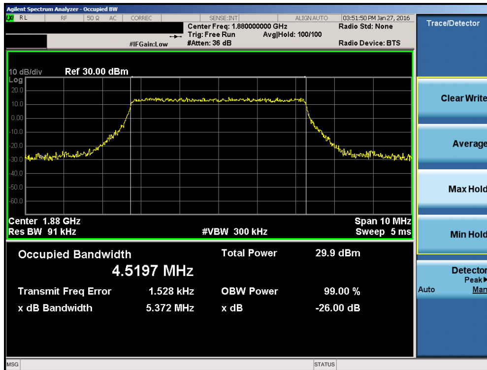
Plot 7-26. Occupied Bandwidth Plot (Band 2 – 5.0MHz 16-QAM – RB Size 25)
