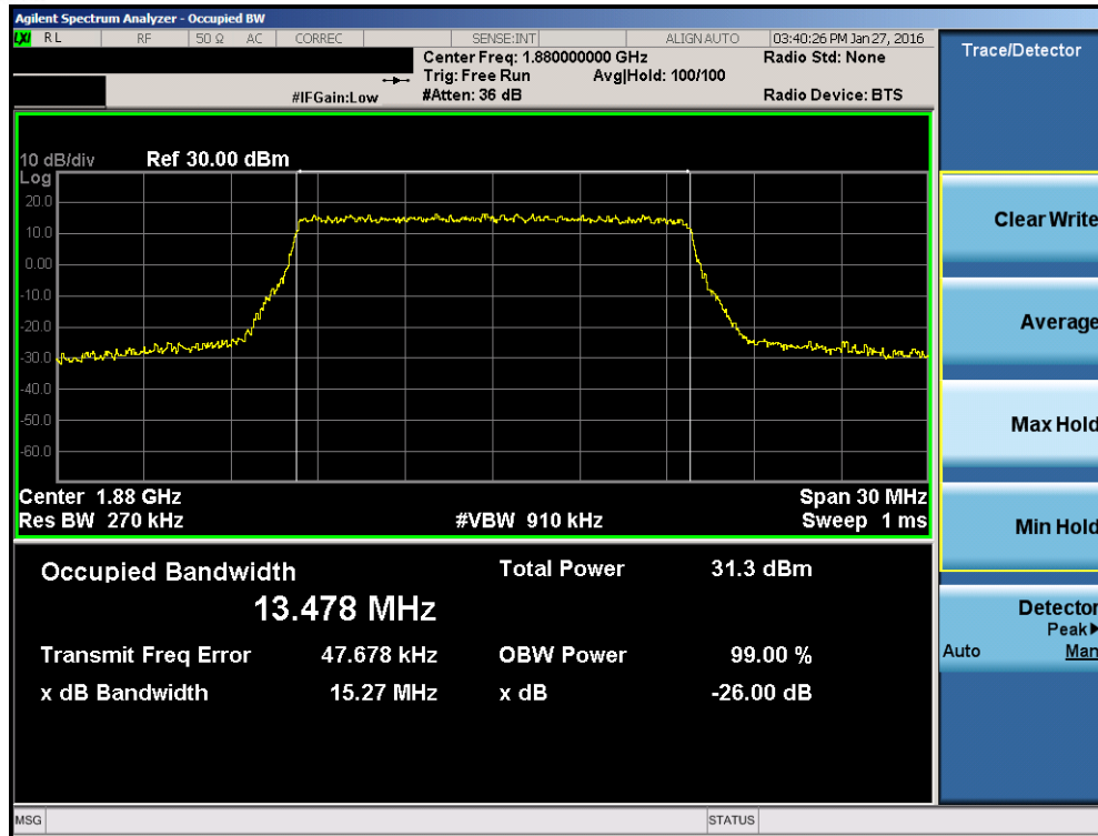
Plot 7-29. Occupied Bandwidth Plot (Band 2 – 15.0MHz QPSK – RB Size 75)
