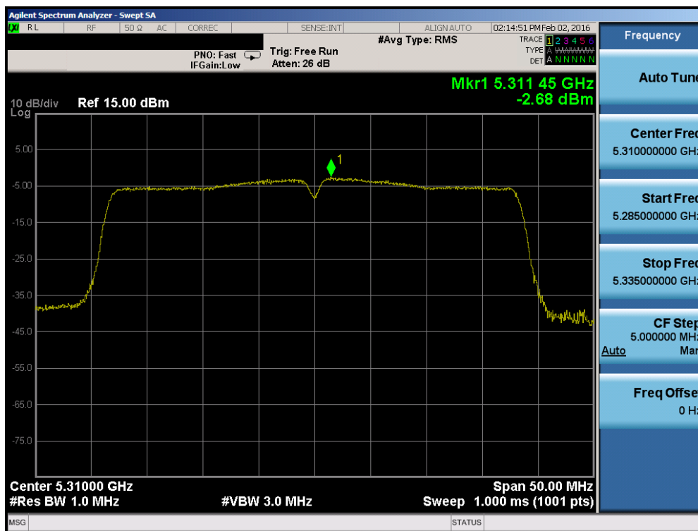
Plot 7-49. Power Spectral Density Plot (40MHz BW 802.11n (UNII Band 2A) – Ch. 62)
