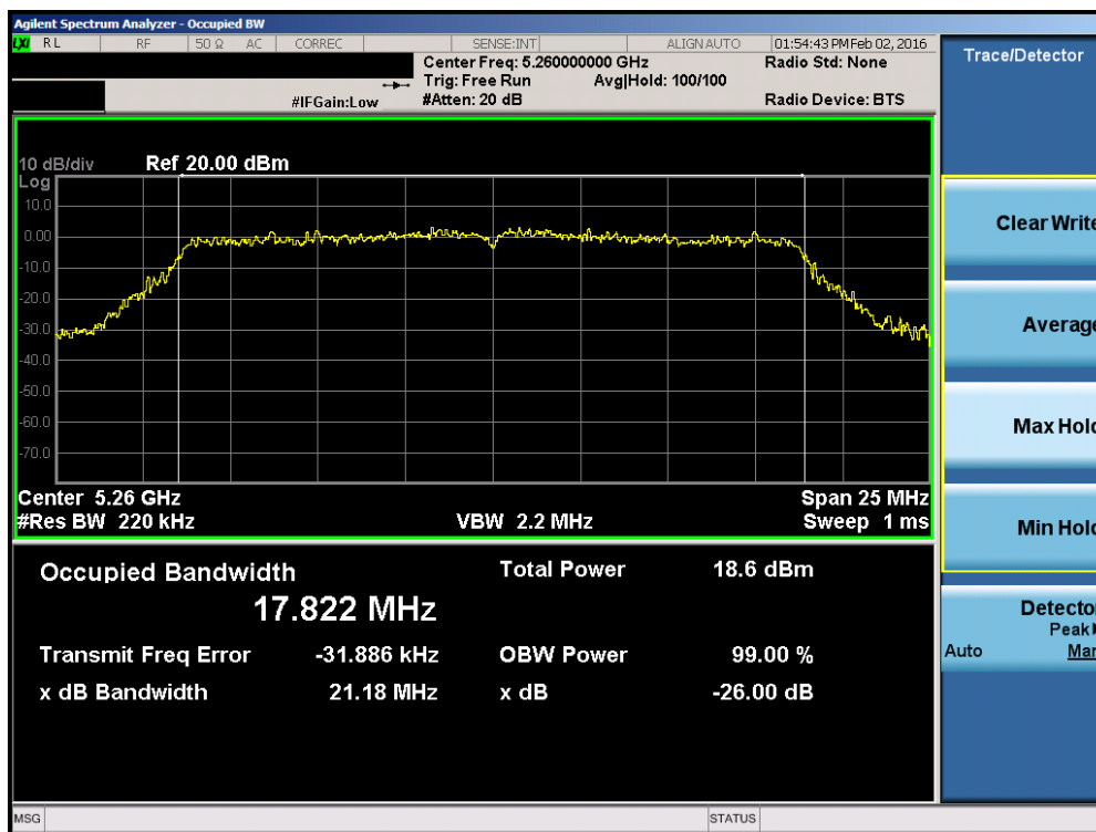
Plot 7-12. 26dB Bandwidth Plot (20MHz BW 802.11n (UNII Band 2A) – Ch. 52)
