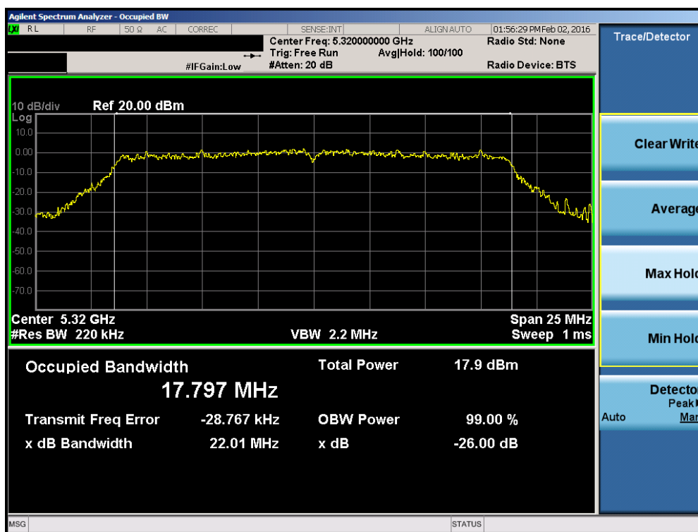
Plot 7-14. 26dB Bandwidth Plot (20MHz BW 802.11n (UNII Band 2A) – Ch. 64)
