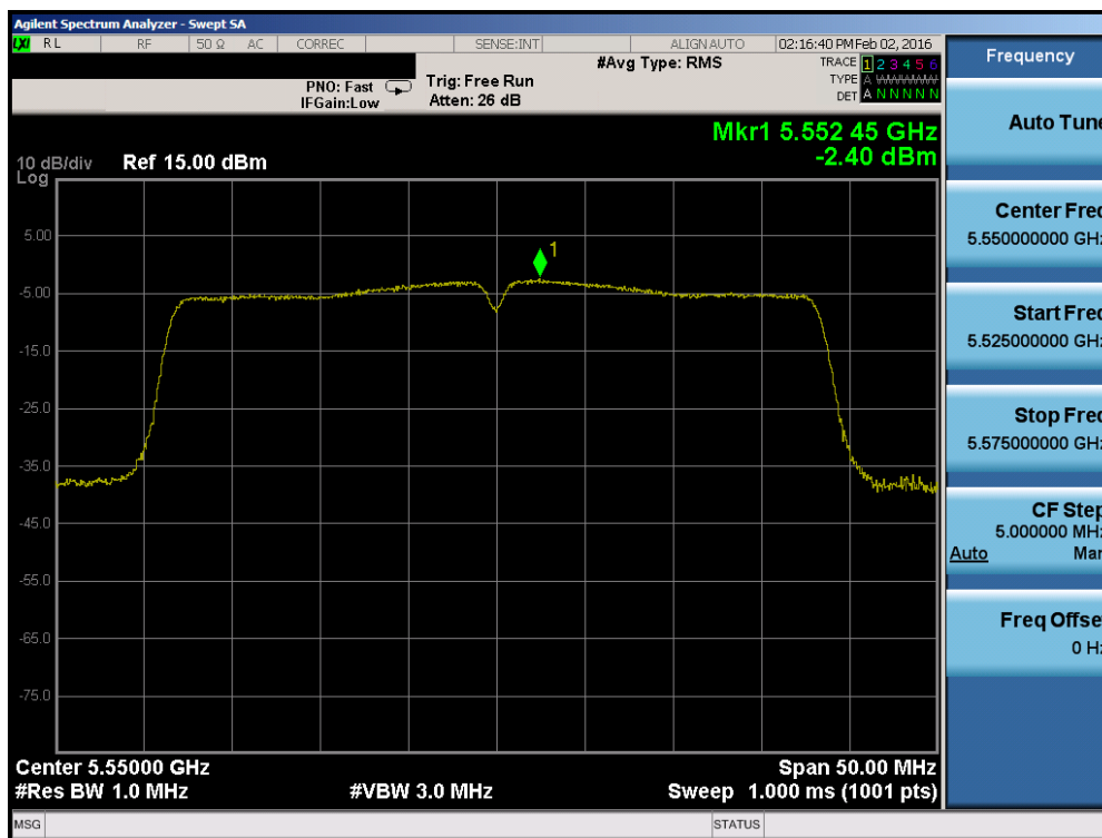
Plot 7-57. Power Spectral Density Plot (40MHz BW 802.11n (UNII Band 2C) – Ch. 110)
