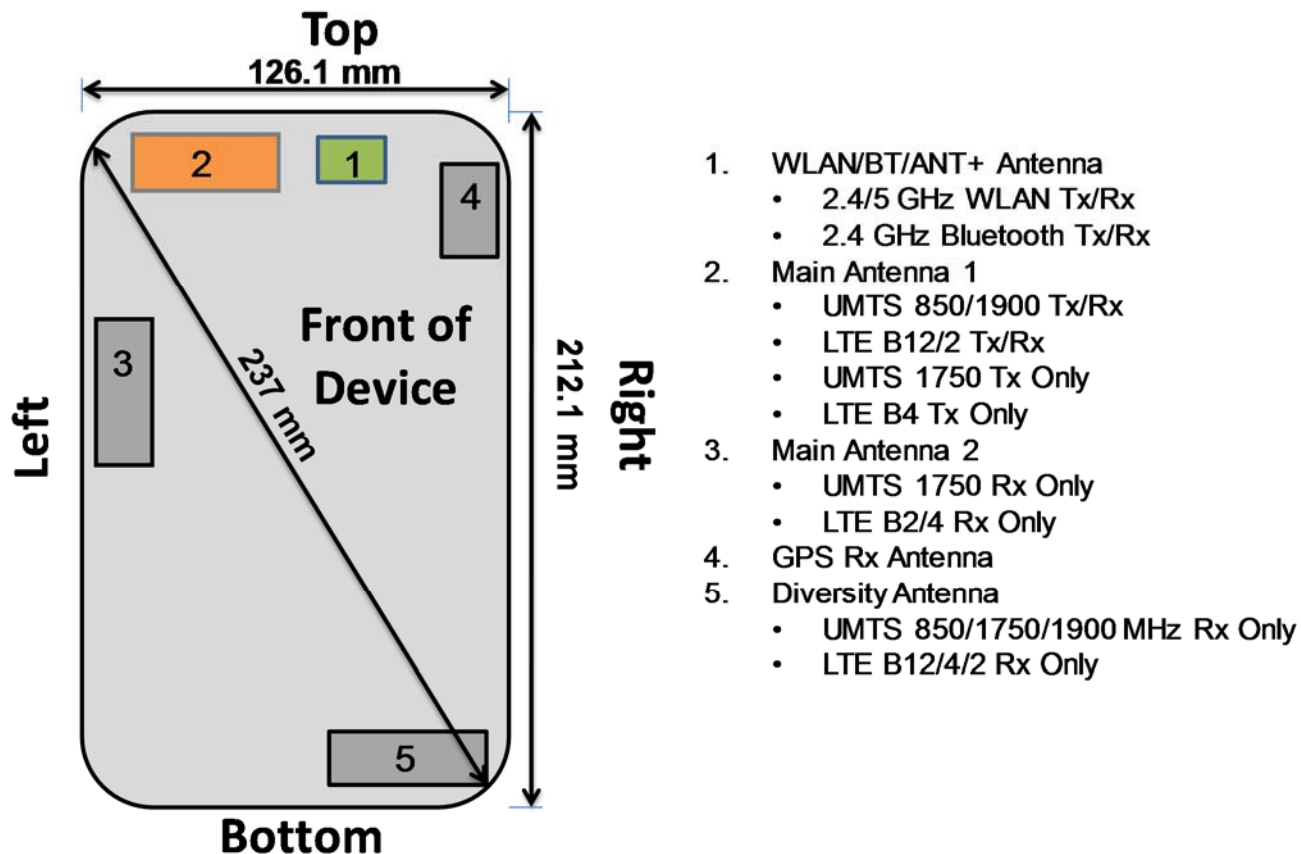
Figure F-1 DUT Antenna Locations
